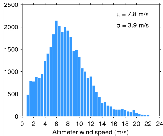
Figure 33. Histogram of flag-valid wind over oceans and lakes for 27/07/2015. The mean ( \mu ) and standard deviation ( \sigma ) are also shown. Note that values larger than 24 m/s are excluded from the histogram for the sake of readability but not from the computation of \mu and \sigma .
