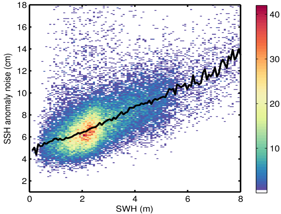
Figure 9. 2D histogram showing flag-valid SSH anomaly noise as a function of SWH for 27/07/2015. The black line denotes the median SSH anomaly as a function of SWH.
