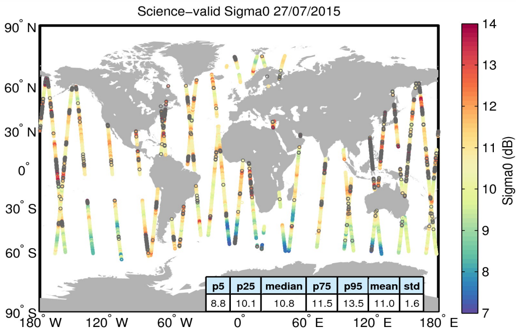
Figure 27. Geographical distribution of science-valid sigma0 data over oceans and lakes for 27/07/2015. The statistical values shown in the table refer to the sigma0 in dB and are calculated over all measurements shown in the figure. Gray circles denote records that have been rejected based on the editing criteria described in Table 4.
