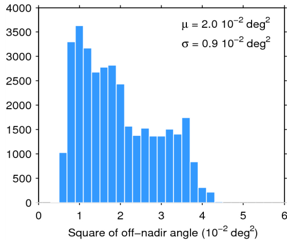
Figure 39. Histogram of flag-valid mispointing over oceans and lakes for 27/07/2015. The mean ( \mu ) and standard deviation ( \sigma ) are also shown. Note that values larger than 6 \cdot 10^{-2} \text{ deg}^2 are excluded from the histogram for the sake of readability but not from the computation of \mu and \sigma .
