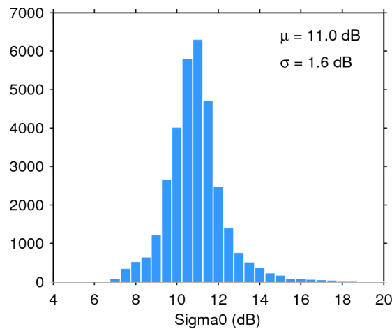
Figure 28. Histogram of science-valid sigma0 over oceans and lakes for 27/07/2015. The mean ( \mu ) and standard deviation ( \sigma ) are also shown. Note that values outside [4 20] dB are excluded from the histogram for the sake of readability but not from the computation of \mu and \sigma .
