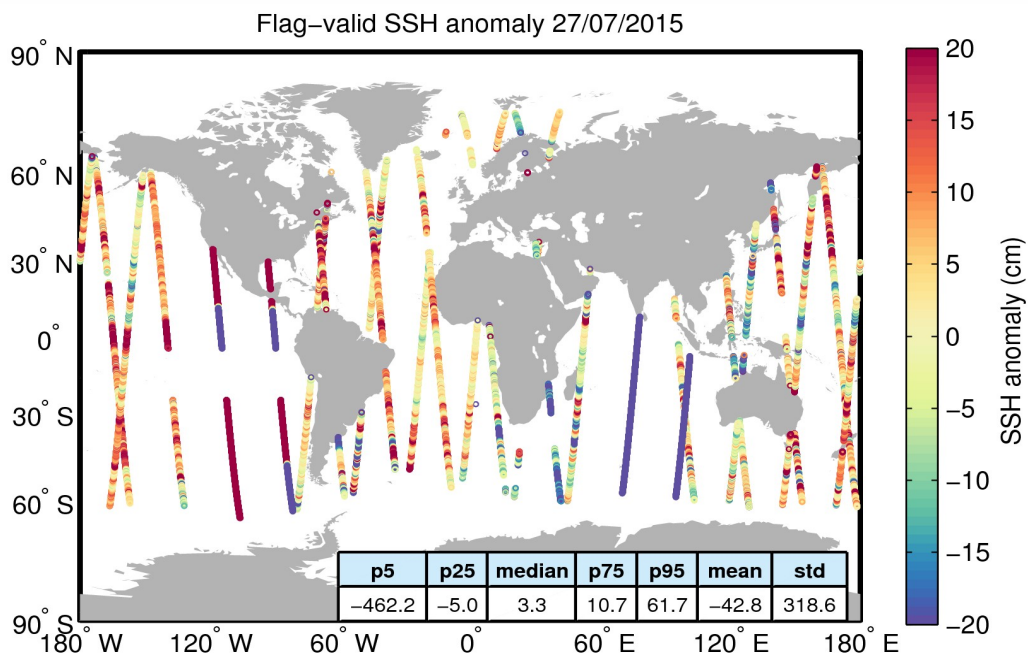
Figure 5. Geographical distribution of flag-valid 1-Hz SSH anomaly data over oceans and lakes for 27/07/2015. The statistical values shown in the table refer to the SSH anomaly in cm and are calculated over all measurements shown in the figure.
