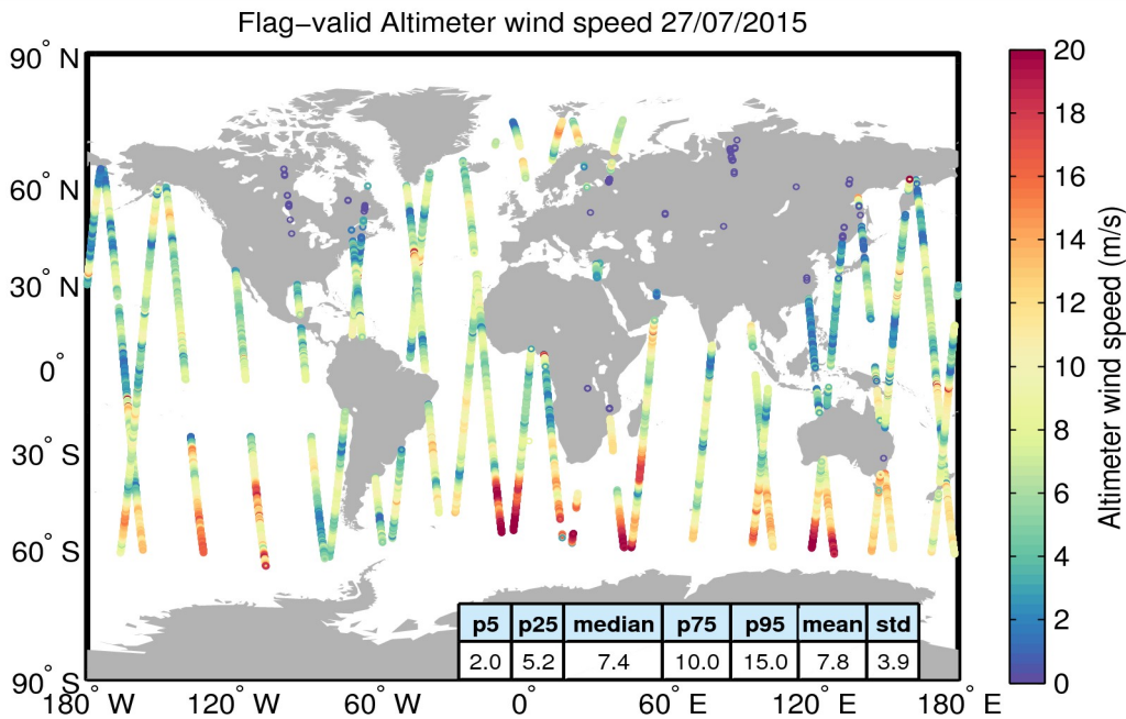
Figure 31. Geographical distribution of flag-valid wind data over oceans and lakes for 27/07/2015. The statistical values shown in the table refer to the wind in m/s and are calculated over all measurements shown in the figure.
