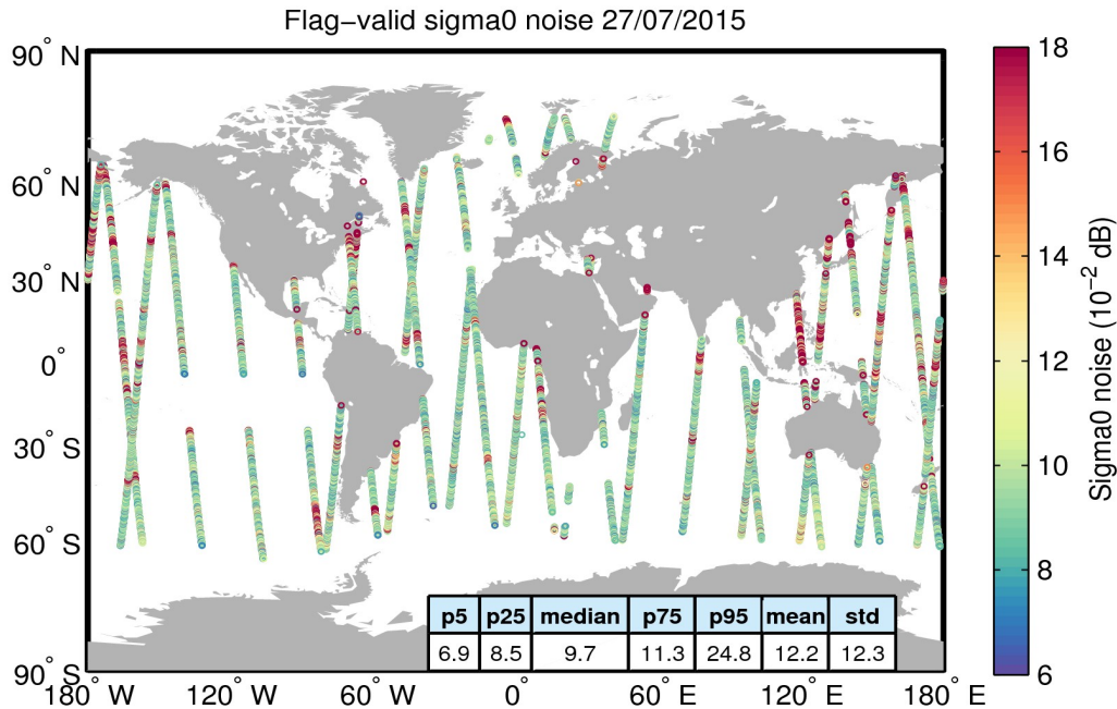
Figure 26. Geographical distribution of flag-valid 20-Hz sigma0 measurement noise over oceans and lakes for 27/07/2015. The statistical values shown in the table refer to the sigma0 noise and are calculated over all measurements shown in the figure.
