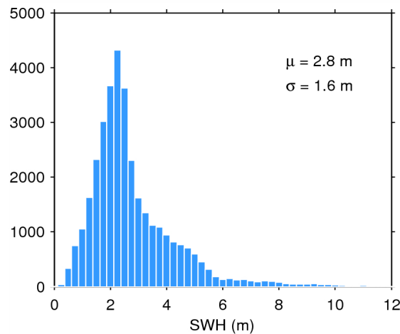
Figure 17. Histogram of flag-valid SWH over oceans and lakes for 27/07/2015. The mean ( \mu ) and standard deviation ( \sigma ) are also shown. Note that values larger than 12 m are excluded from the histogram for the sake of readability but not from the computation of \mu and \sigma .
