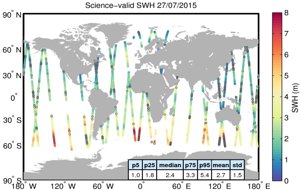
Figure 19. Geographical distribution of science-valid SWH data over oceans and lakes for 27/07/2015. The statistical values shown in the table refer to the SWH in m and are calculated over all measurements shown in the figure. Gray circles denote records that have been rejected based on the editing criteria described in Table 3.
