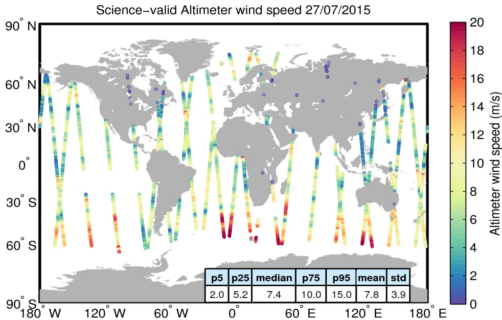
Figure 34. Geographical distribution of science-valid wind data over oceans and lakes for 27/07/2015. The statistical values shown in the table refer to the wind in m/s and are calculated over all measurements shown in the figure. Gray circles denote records that have been rejected based on the editing criteria described in Table 5.
