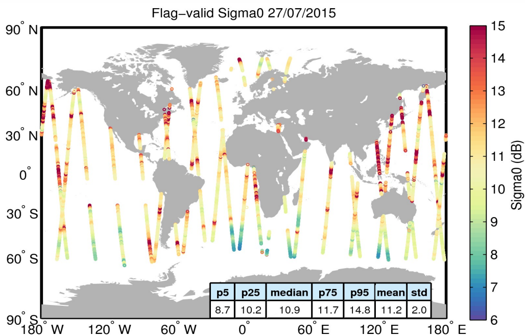
Figure 23. Geographical distribution of flag-valid sigma0 data over oceans and lakes for 27/07/2015. The statistical values shown in the table refer to the sigma0 in dB and are calculated over all measurements shown in the figure.
