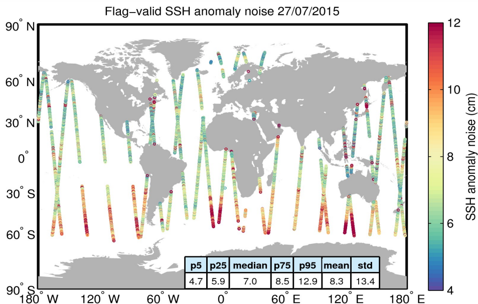
Figure 8. Geographical distribution of flag-valid 20-Hz SSH anomaly measurement noise over oceans and lakes for 27/07/2015. The statistical values shown in the table refer to the SSH anomaly noise and are calculated over all measurements shown in the figure.
