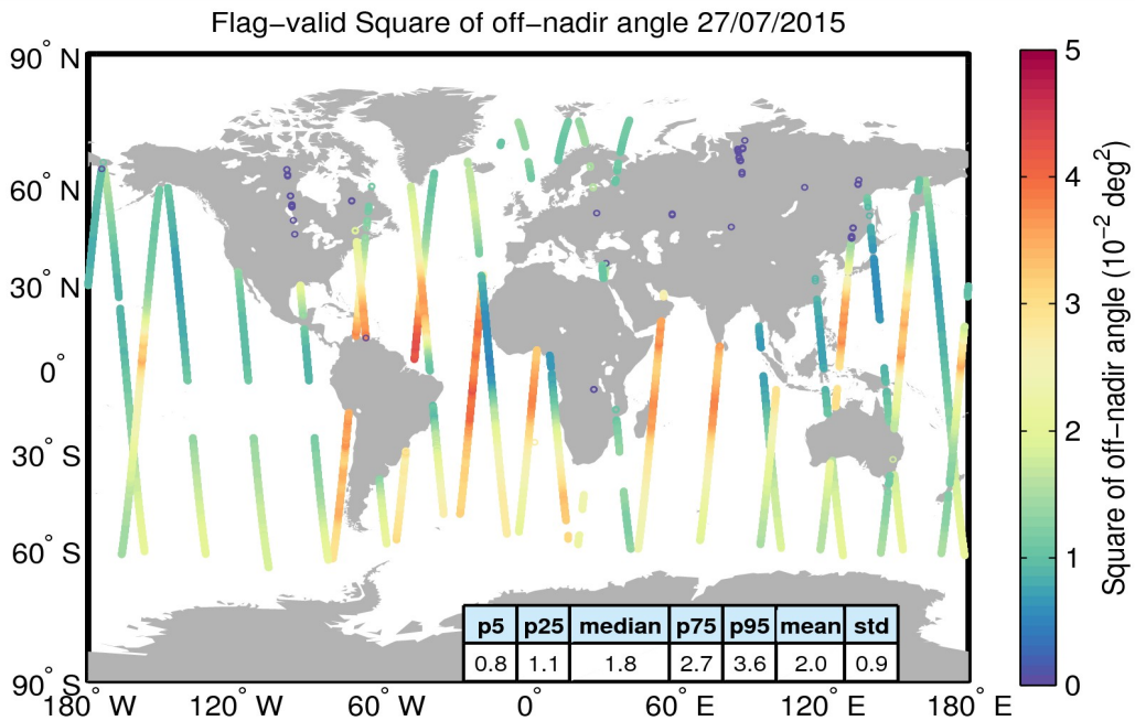
Figure 37. Geographical distribution of flag-valid mispointing data over oceans and lakes for 27/07/2015. The statistical values shown in the table refer to the mispointing in 10^{-2} \text{ deg}^2 and are calculated over all measurements shown in the figure.
