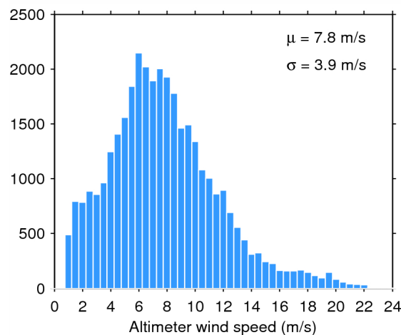
Figure 35. Histogram of science-valid wind over oceans and lakes for 27/07/2015. The mean ( \mu ) and standard deviation ( \sigma ) are also shown. Note that values larger than 24 m/s are excluded from the histogram for the sake of readability but not from the computation of \mu and \sigma .
