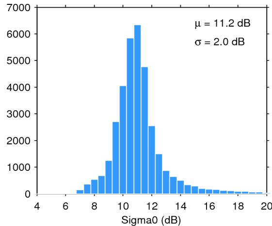
Figure 25. Histogram of flag-valid sigma0 over oceans and lakes for 27/07/2015. The mean ( \mu ) and standard deviation ( \sigma ) are also shown. Note that values outside [4 20] dB are excluded from the histogram for the sake of readability but not from the computation of \mu and \sigma .
