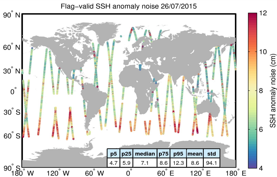
Figure 8. Geographical distribution of flag-valid 20-Hz SSH anomaly measurement noise over oceans and lakes for 26/07/2015. The statistical values shown in the table refer to the SSH anomaly noise and are calculated over all measurements shown in the figure.
