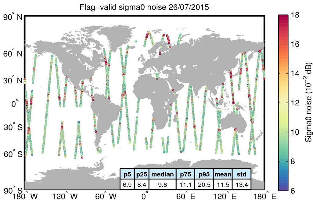
Figure 26. Geographical distribution of flag-valid 20-Hz sigma0 measurement noise over oceans and lakes for 26/07/2015. The statistical values shown in the table refer to the sigma0 noise and are calculated over all measurements shown in the figure.
