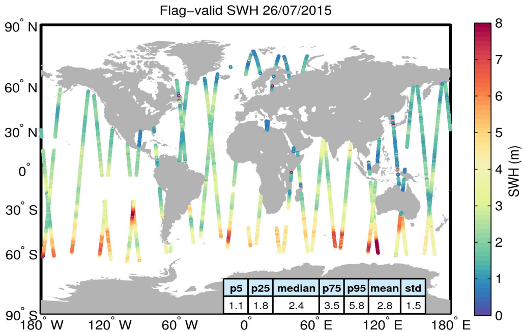
Figure 15. Geographical distribution of flag-valid SWH data over oceans and lakes for 26/07/2015. The statistical values shown in the table refer to the SWH in m and are calculated over all measurements shown in the figure.
