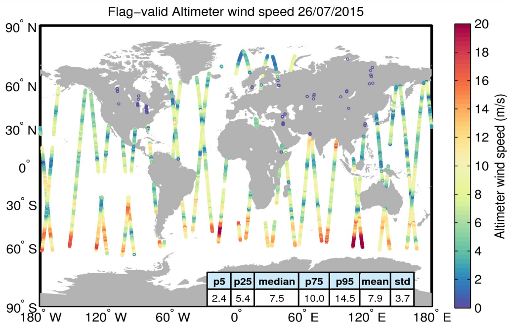
Figure 31. Geographical distribution of flag-valid wind data over oceans and lakes for 26/07/2015. The statistical values shown in the table refer to the wind in m/s and are calculated over all measurements shown in the figure.
