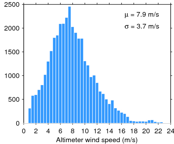
Figure 33. Histogram of flag-valid wind over oceans and lakes for 26/07/2015. The mean ( \mu ) and standard deviation ( \sigma ) are also shown. Note that values larger than 24 m/s are excluded from the histogram for the sake of readability but not from the computation of \mu and \sigma .
