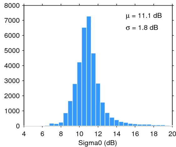
Figure 25. Histogram of flag-valid sigma0 over oceans and lakes for 26/07/2015. The mean ( \mu ) and standard deviation ( \sigma ) are also shown. Note that values outside [4 20] dB are excluded from the histogram for the sake of readability but not from the computation of \mu and \sigma .
