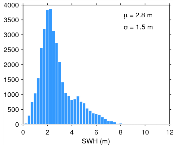
Figure 20. Histogram of science-valid SWH over oceans and lakes for 26/07/2015. The mean ( \mu ) and standard deviation ( \sigma ) are also shown. Note that values larger than 12 m are excluded from the histogram for the sake of readability but not from the computation of \mu and \sigma .
