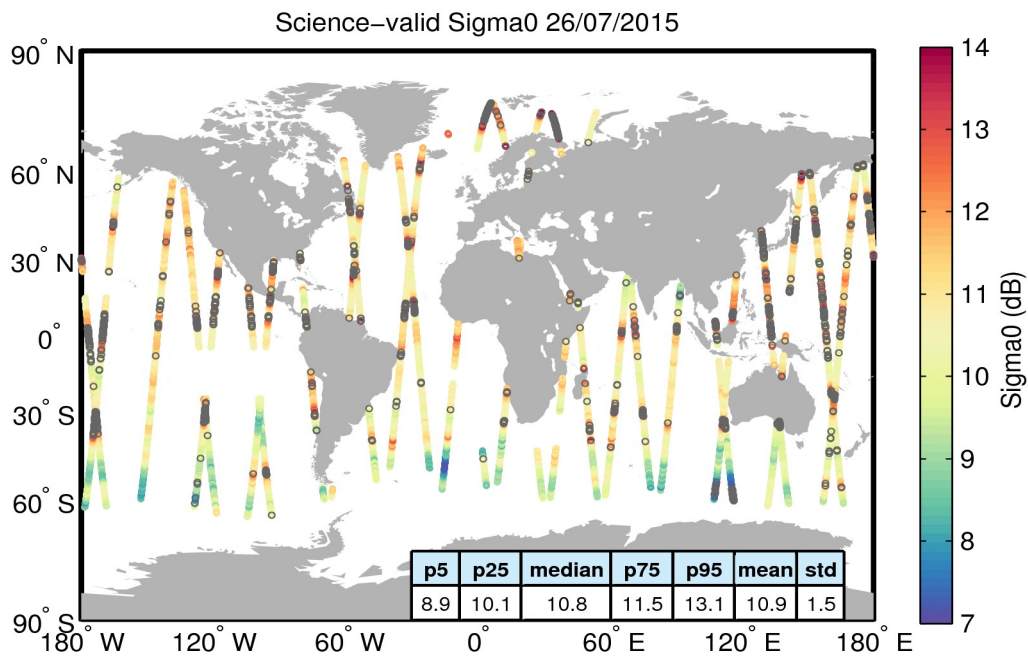
Figure 27. Geographical distribution of science-valid sigma0 data over oceans and lakes for 26/07/2015. The statistical values shown in the table refer to the sigma0 in dB and are calculated over all measurements shown in the figure. Gray circles denote records that have been rejected based on the editing criteria described in Table 4.
