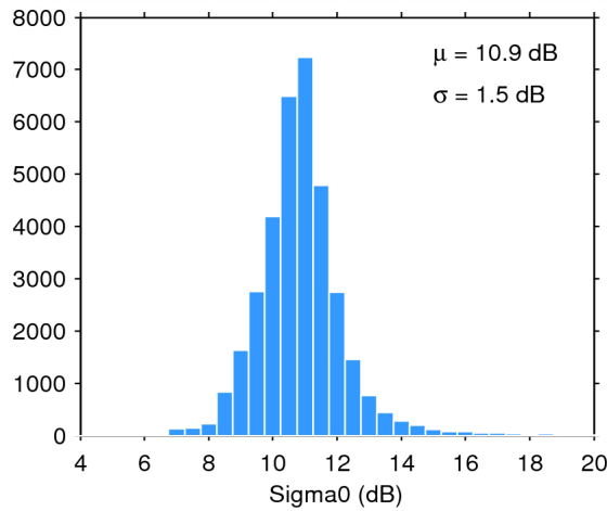
Figure 28. Histogram of science-valid sigma0 over oceans and lakes for 26/07/2015. The mean ( \mu ) and standard deviation ( \sigma ) are also shown. Note that values outside [4 20] dB are excluded from the histogram for the sake of readability but not from the computation of \mu and \sigma .
