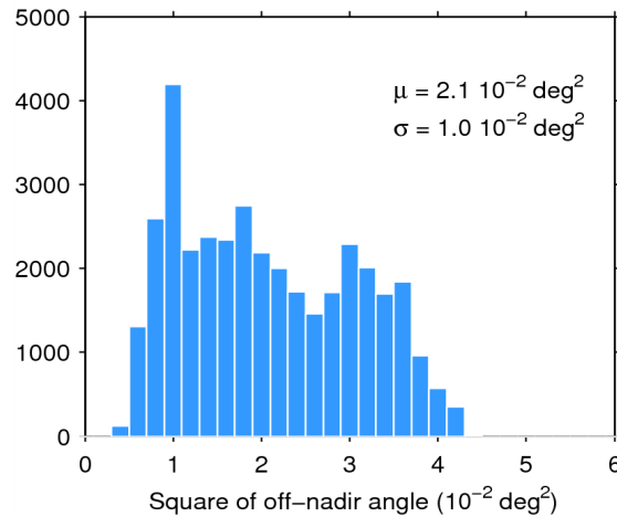
Figure 39. Histogram of flag-valid mispointing over oceans and lakes for 26/07/2015. The mean ( \mu ) and standard deviation ( \sigma ) are also shown. Note that values larger than 6 \cdot 10^{-2} \text{ deg}^2 are excluded from the histogram for the sake of readability but not from the computation of \mu and \sigma .
