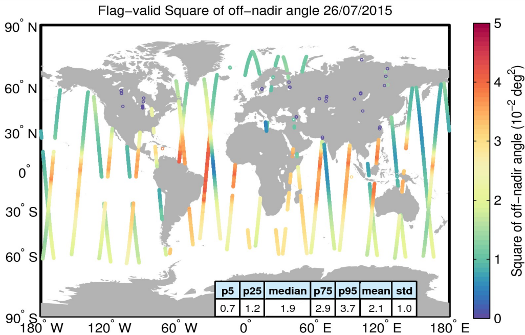
Figure 37. Geographical distribution of flag-valid mispointing data over oceans and lakes for 26/07/2015. The statistical values shown in the table refer to the mispointing in 10^{-2} \text{ deg}^2 and are calculated over all measurements shown in the figure.
