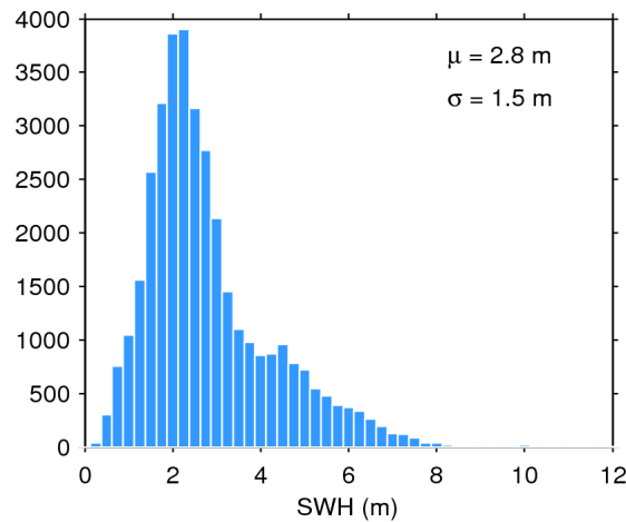
Figure 17. Histogram of flag-valid SWH over oceans and lakes for 26/07/2015. The mean ( \mu ) and standard deviation ( \sigma ) are also shown. Note that values larger than 12 m are excluded from the histogram for the sake of readability but not from the computation of \mu and \sigma .
