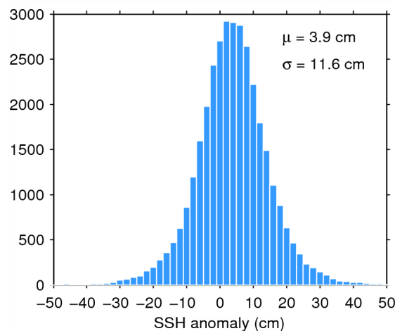
Figure 11. Histogram of science-valid SSH anomaly over oceans and lakes for 26/07/2015. The mean ( \mu ) and standard deviation ( \sigma ) are also shown. Note that values outside [-50 50] cm are excluded from the histogram for the sake of readability but not from the computation of \mu and \sigma .
