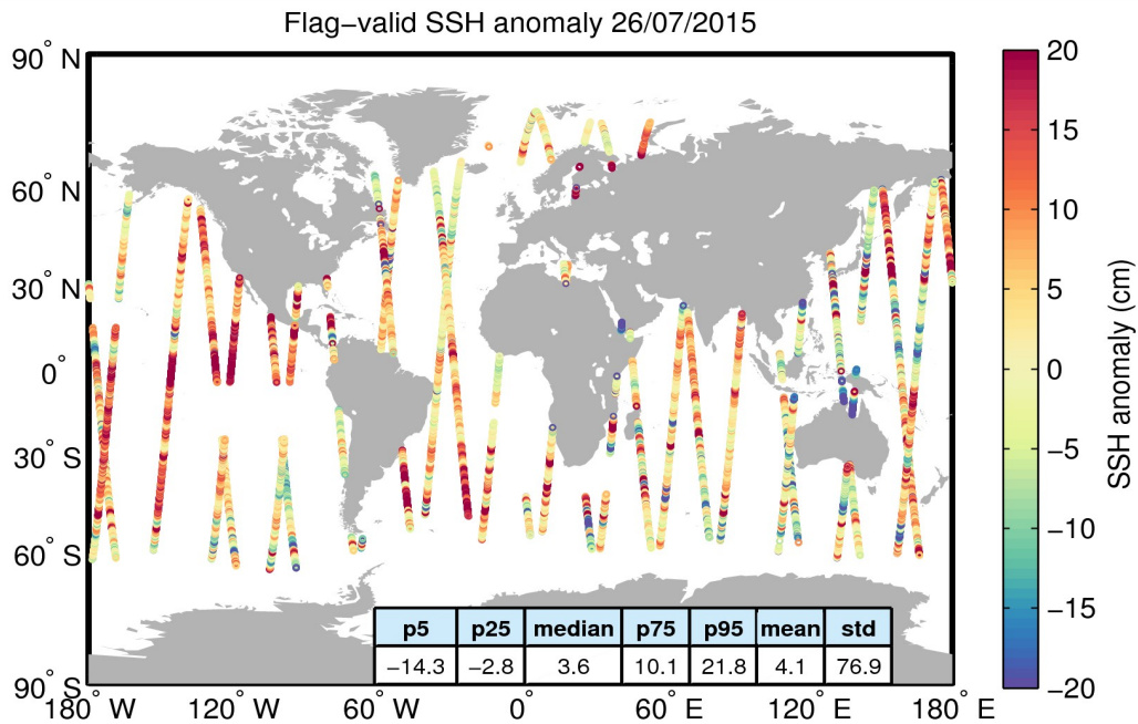
Figure 5. Geographical distribution of flag-valid 1-Hz SSH anomaly data over oceans and lakes for 26/07/2015. The statistical values shown in the table refer to the SSH anomaly in cm and are calculated over all measurements shown in the figure.
