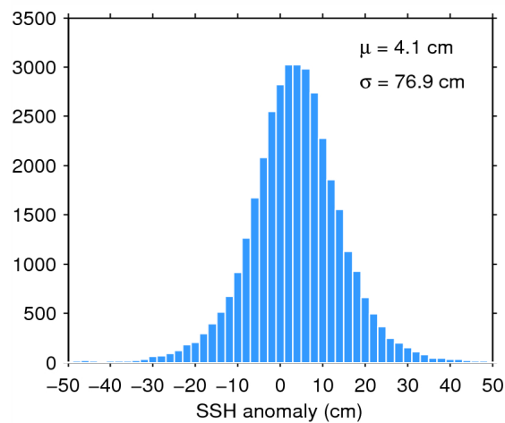
Figure 7. Histogram of flag-valid SSH anomaly over oceans and lakes for 26/07/2015. The mean ( \mu ) and standard deviation ( \sigma ) are also shown. Note that values outside [-50 50] cm are excluded from the histogram for the sake of readability but not from the computation of \mu and \sigma .
