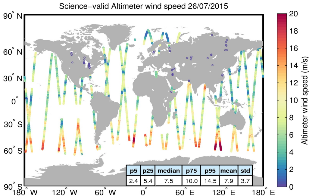
Figure 34. Geographical distribution of science-valid wind data over oceans and lakes for 26/07/2015. The statistical values shown in the table refer to the wind in m/s and are calculated over all measurements shown in the figure. Gray circles denote records that have been rejected based on the editing criteria described in Table 5.
