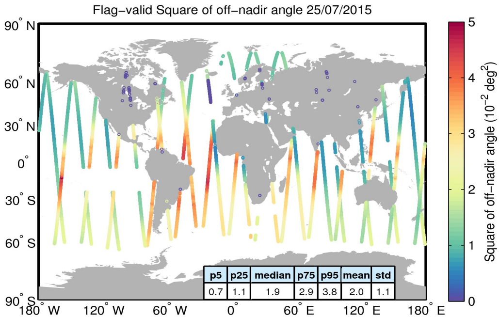
Figure 37. Geographical distribution of flag-valid mispointing data over oceans and lakes for 25/07/2015. The statistical values shown in the table refer to the mispointing in 10^{-2} deg 2 and are calculated over all measurements shown in the figure.
