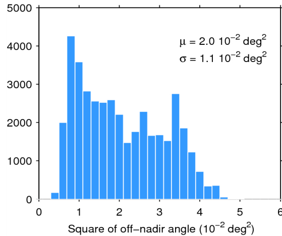
Figure 39. Histogram of flag-valid mispointing over oceans and lakes for 25/07/2015. The mean ( \mu ) and standard deviation ( \sigma ) are also shown. Note that values larger than 6 \cdot 10^{-2} \text{ deg}^2 are excluded from the histogram for the sake of readability but not from the computation of \mu and \sigma .
