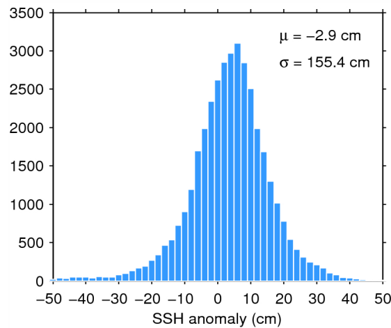
Figure 7. Histogram of flag-valid SSH anomaly over oceans and lakes for 25/07/2015. The mean ( \mu ) and standard deviation ( \sigma ) are also shown. Note that values outside [-50\ 50] cm are excluded from the histogram for the sake of readability but not from the computation of \mu and \sigma .
