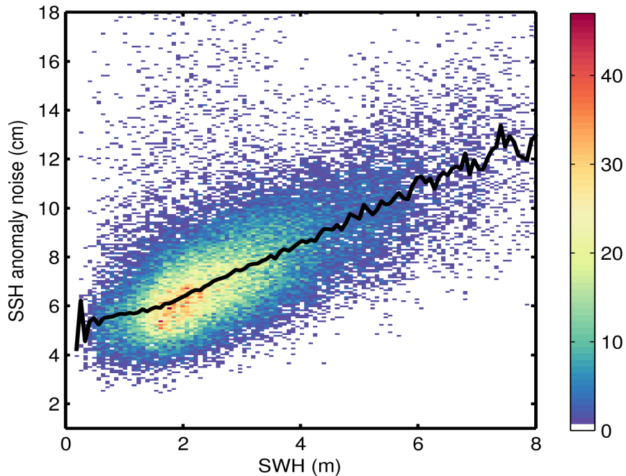
Figure 9. 2D histogram showing flag-valid SSH anomaly noise as a function of SWH for 25/07/2015. The black line denotes the median SSH anomaly as a function of SWH.
