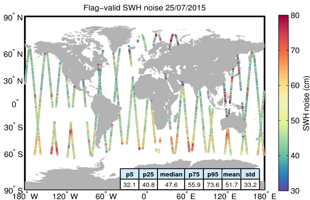
Figure 18. Geographical distribution of flag-valid 20-Hz SWH measurement noise over oceans and lakes for 25/07/2015. The statistical values shown in the figure refer to the SWH noise and are calculated over all measurements shown in the figure.
