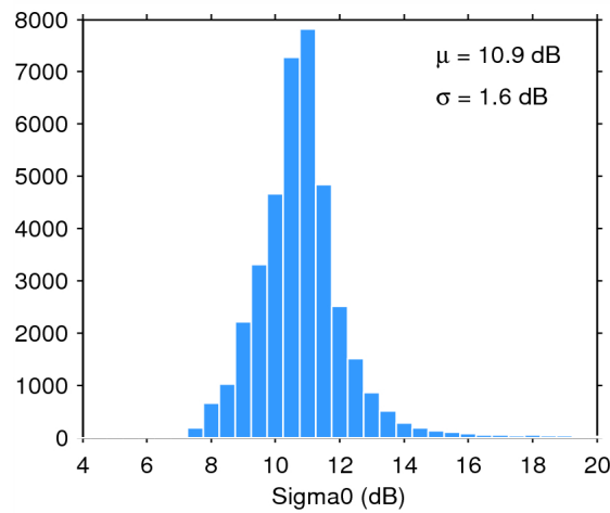
Figure 28. Histogram of science-valid sigma0 over oceans and lakes for 25/07/2015. The mean ( \mu ) and standard deviation ( \sigma ) are also shown. Note that values outside [4 20] dB are excluded from the histogram for the sake of readability but not from the computation of \mu and \sigma .
