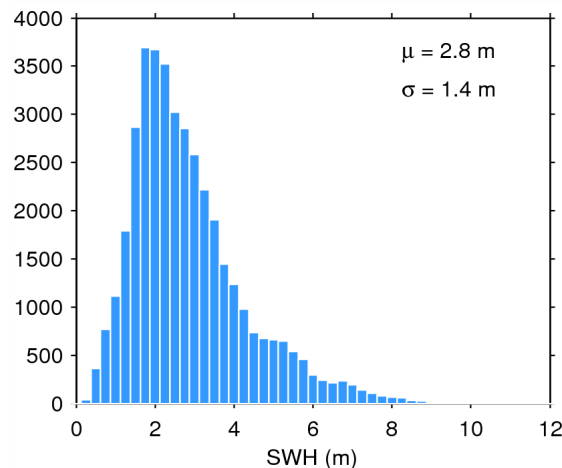
Figure 20. Histogram of science-valid SWH over oceans and lakes for 25/07/2015. The mean ( \mu ) and standard deviation ( \sigma ) are also shown. Note that values larger than 12 m are excluded from the histogram for the sake of readability but not from the computation of \mu and \sigma .
