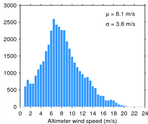
Figure 35. Histogram of science-valid wind over oceans and lakes for 25/07/2015. The mean ( \mu ) and standard deviation ( \sigma ) are also shown. Note that values larger than 24 m/s are excluded from the histogram for the sake of readability but not from the computation of \mu and \sigma .
