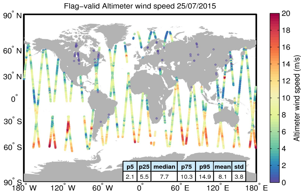
Figure 31. Geographical distribution of flag-valid wind data over oceans and lakes for 25/07/2015. The statistical values shown in the table refer to the wind in m/s and are calculated over all measurements shown in the figure.
