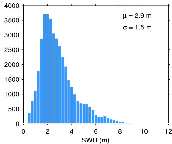
Figure 17. Histogram of flag-valid SWH over oceans and lakes for 25/07/2015. The mean ( \mu ) and standard deviation ( \sigma ) are also shown. Note that values larger than 12 m are excluded from the histogram for the sake of readability but not from the computation of \mu and \sigma .
