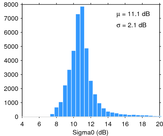
Figure 25. Histogram of flag-valid sigma0 over oceans and lakes for 25/07/2015. The mean ( \mu ) and standard deviation ( \sigma ) are also shown. Note that values outside [4 20] dB are excluded from the histogram for the sake of readability but not from the computation of \mu and \sigma .
