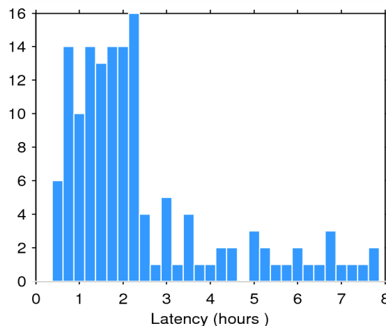
Figure 2. Histogram of the data latency for 25/07/2015. The y-axis denotes the number of files that are made available with a delay of x-hours with respect to the mean time of the records stored in the file.
