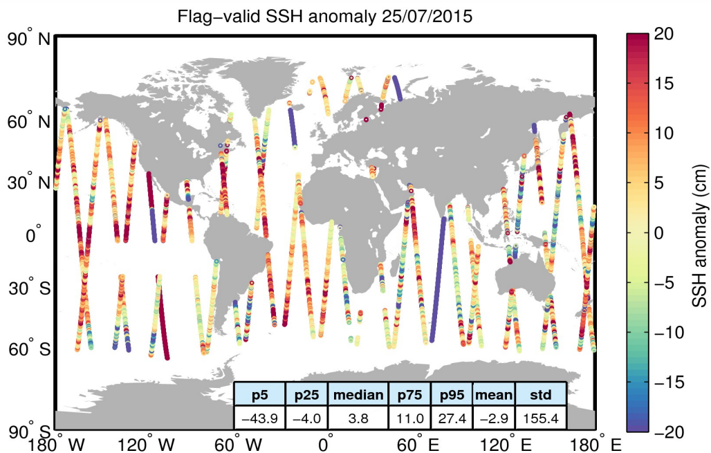
Figure 5. Geographical distribution of flag-valid 1-Hz SSH anomaly data over oceans and lakes for 25/07/2015. The statistical values shown in the table refer to the SSH anomaly in cm and are calculated over all measurements shown in the figure.
