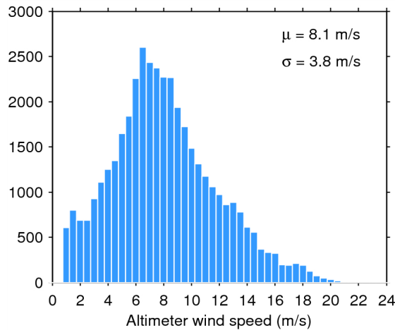
Figure 33. Histogram of flag-valid wind over oceans and lakes for 25/07/2015. The mean ( \mu ) and standard deviation ( \sigma ) are also shown. Note that values larger than 24 m/s are excluded from the histogram for the sake of readability but not from the computation of \mu and \sigma .
