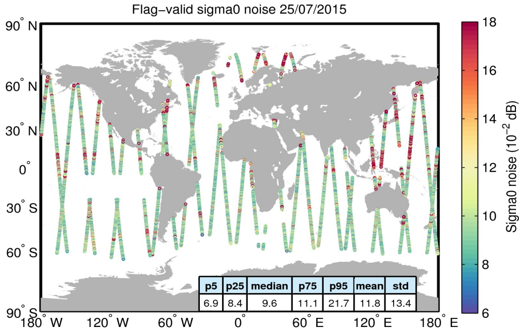
Figure 26. Geographical distribution of flag-valid 20-Hz sigma0 measurement noise over oceans and lakes for 25/07/2015. The statistical values shown in the table refer to the sigma0 noise and are calculated over all measurements shown in the figure.
