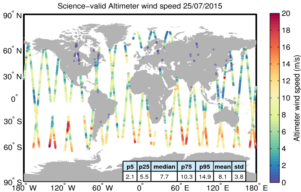
Figure 34. Geographical distribution of science-valid wind data over oceans and lakes for 25/07/2015. The statistical values shown in the table refer to the wind in m/s and are calculated over all measurements shown in the figure. Gray circles denote records that have been rejected based on the editing criteria described in Table 5.
