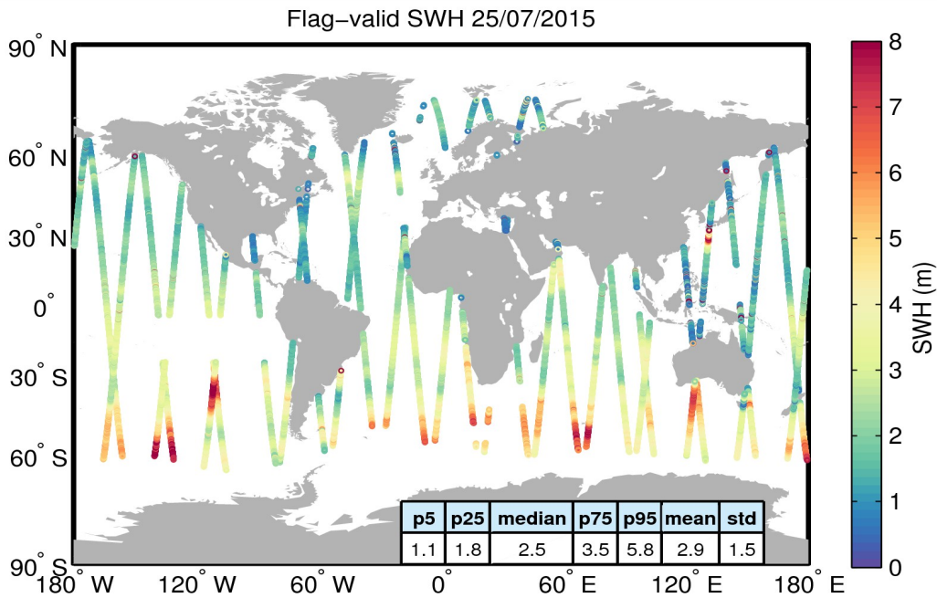
Figure 15. Geographical distribution of flag-valid SWH data over oceans and lakes for 25/07/2015. The statistical values shown in the table refer to the SWH in m and are calculated over all measurements shown in the figure.
