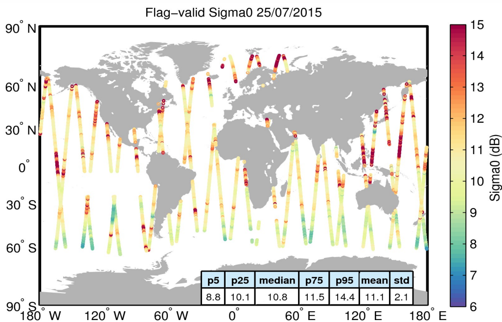
Figure 23. Geographical distribution of flag-valid sigma0 data over oceans and lakes for 25/07/2015. The statistical values shown in the table refer to the sigma0 in dB and are calculated over all measurements shown in the figure.
