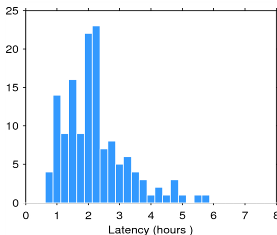
Figure 2. Histogram of the data latency for 22/07/2015. The y-axis denotes the number of files that are made available with a delay of x-hours with respect to the mean time of the records stored in the file.
