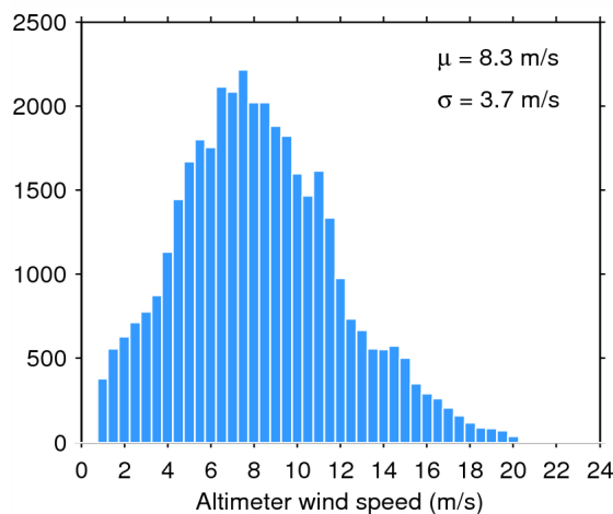
Figure 35. Histogram of science-valid wind over oceans and lakes for 21/07/2015. The mean ( \mu ) and standard deviation ( \sigma ) are also shown. Note that values larger than 24 m/s are excluded from the histogram for the sake of readability but not from the computation of \mu and \sigma .
