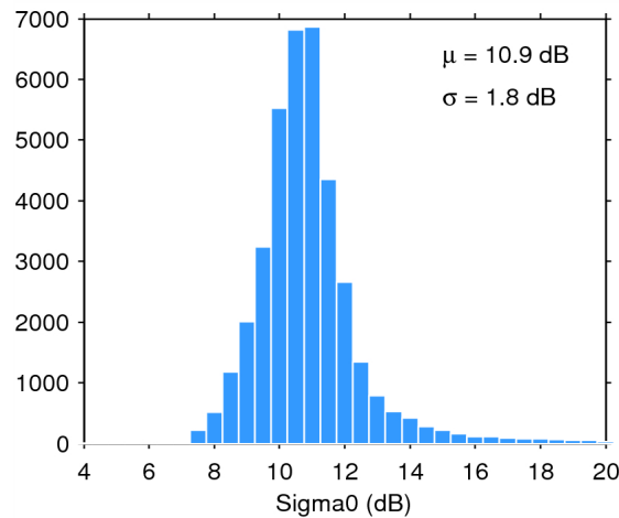
Figure 25. Histogram of flag-valid sigma0 over oceans and lakes for 21/07/2015. The mean ( \mu ) and standard deviation ( \sigma ) are also shown. Note that values outside [4 20] dB are excluded from the histogram for the sake of readability but not from the computation of \mu and \sigma .
