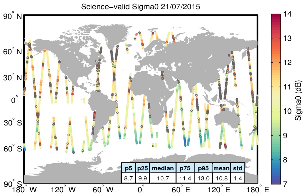
Figure 27. Geographical distribution of science-valid sigma0 data over oceans and lakes for 21/07/2015. The statistical values shown in the table refer to the sigma0 in dB and are calculated over all measurements shown in the figure. Gray circles denote records that have been rejected based on the editing criteria described in Table 4.
