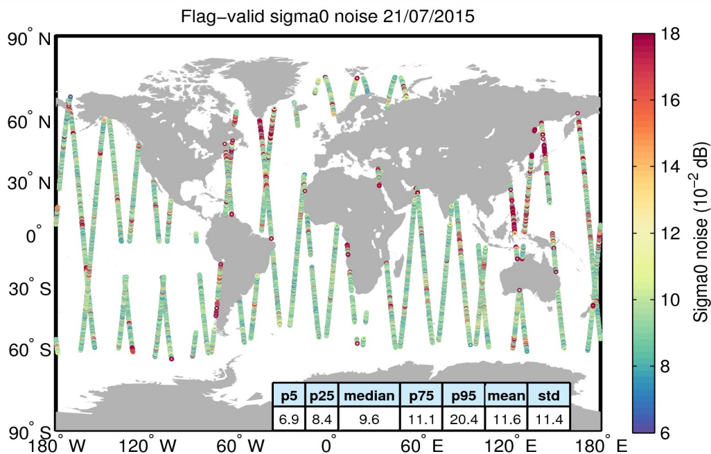
Figure 26. Geographical distribution of flag-valid 20-Hz sigma0 measurement noise over oceans and lakes for 21/07/2015. The statistical values shown in the table refer to the sigma0 noise and are calculated over all measurements shown in the figure.
