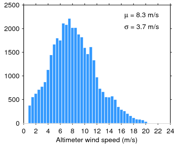
Figure 33. Histogram of flag-valid wind over oceans and lakes for 21/07/2015. The mean ( \mu ) and standard deviation ( \sigma ) are also shown. Note that values larger than 24 m/s are excluded from the histogram for the sake of readability but not from the computation of \mu and \sigma .
