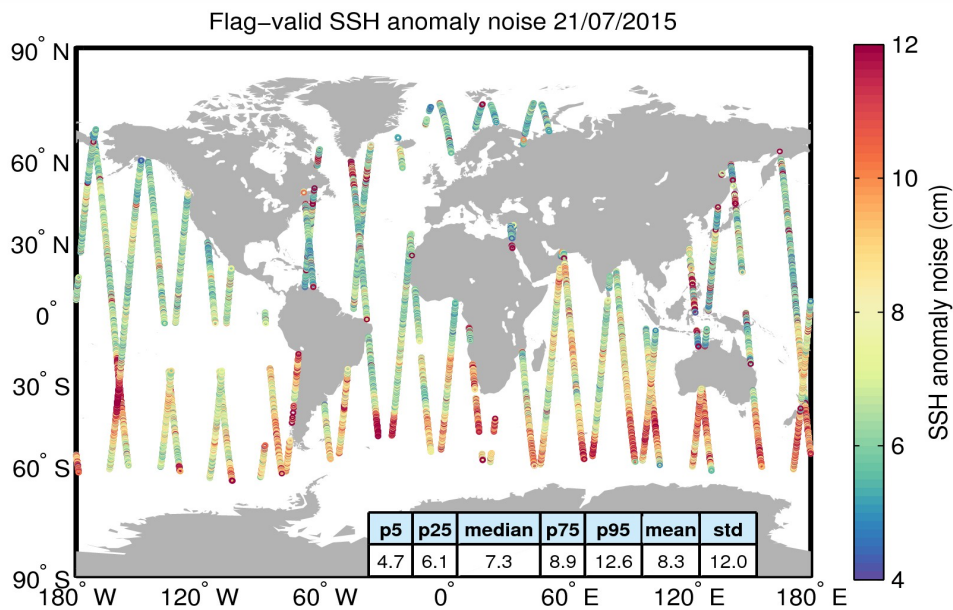
Figure 8. Geographical distribution of flag-valid 20-Hz SSH anomaly measurement noise over oceans and lakes for 21/07/2015. The statistical values shown in the table refer to the SSH anomaly noise and are calculated over all measurements shown in the figure.
