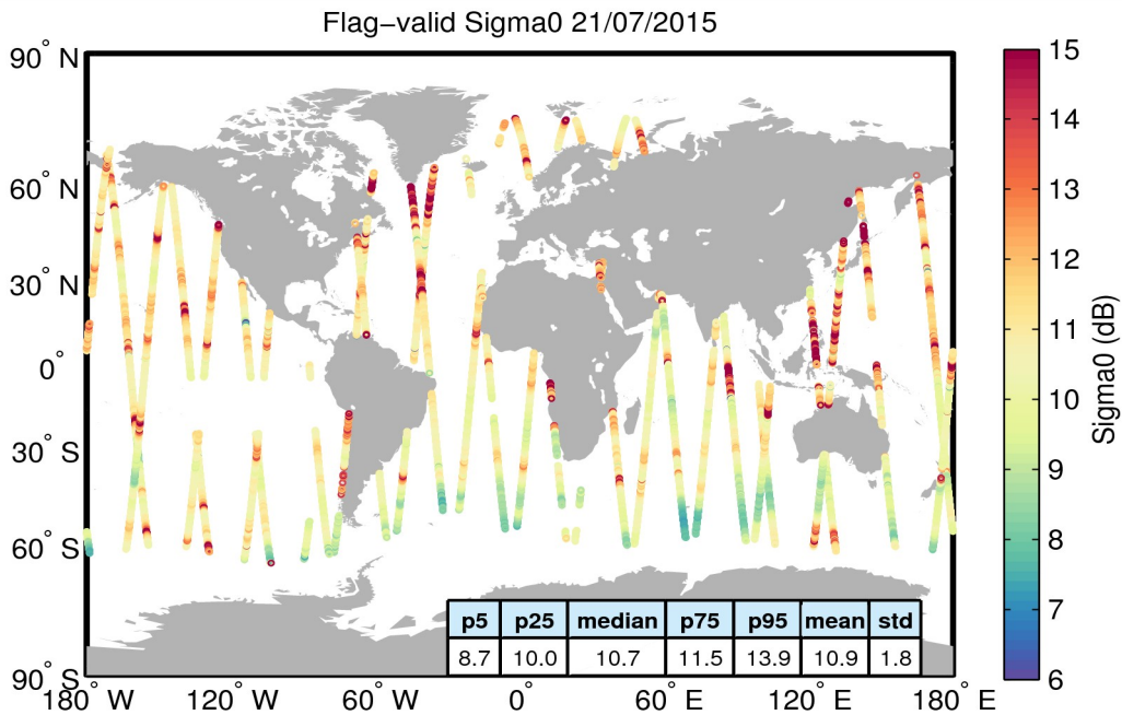
Figure 23. Geographical distribution of flag-valid sigma0 data over oceans and lakes for 21/07/2015. The statistical values shown in the table refer to the sigma0 in dB and are calculated over all measurements shown in the figure.
