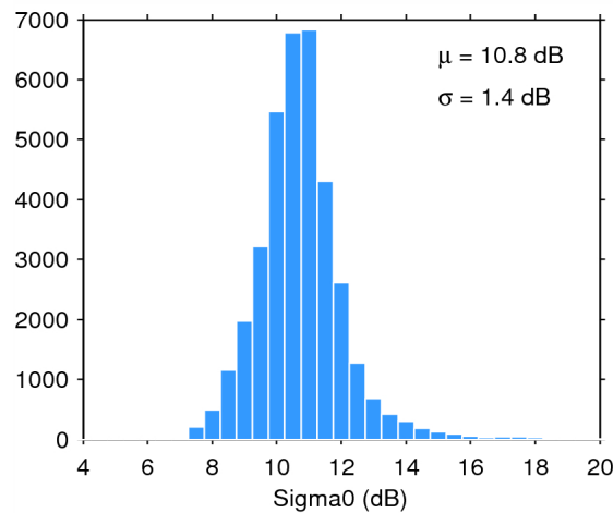
Figure 28. Histogram of science-valid sigma0 over oceans and lakes for 21/07/2015. The mean ( \mu ) and standard deviation ( \sigma ) are also shown. Note that values outside [4 20] dB are excluded from the histogram for the sake of readability but not from the computation of \mu and \sigma .
