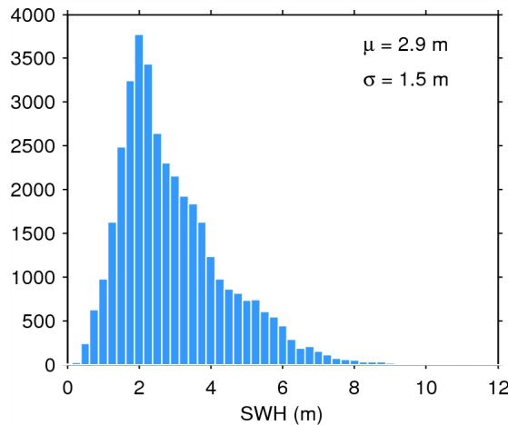
Figure 20. Histogram of science-valid SWH over oceans and lakes for 21/07/2015. The mean ( \mu ) and standard deviation ( \sigma ) are also shown. Note that values larger than 12 m are excluded from the histogram for the sake of readability but not from the computation of \mu and \sigma .
