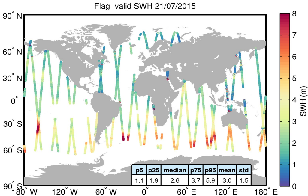
Figure 15. Geographical distribution of flag-valid SWH data over oceans and lakes for 21/07/2015. The statistical values shown in the table refer to the SWH in m and are calculated over all measurements shown in the figure.
