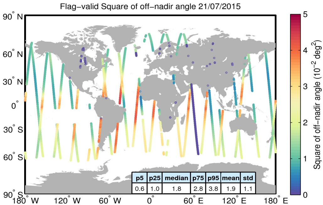
Figure 37. Geographical distribution of flag-valid mispointing data over oceans and lakes for 21/07/2015. The statistical values shown in the table refer to the mispointing in 10^{-2} \text{deg}^2 and are calculated over all measurements shown in the figure.
