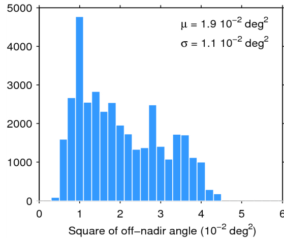
Figure 39. Histogram of flag-valid mispointing over oceans and lakes for 21/07/2015. The mean ( \mu ) and standard deviation ( \sigma ) are also shown. Note that values larger than 6 \cdot 10^{-2} \text{ deg}^2 are excluded from the histogram for the sake of readability but not from the computation of \mu and \sigma .
