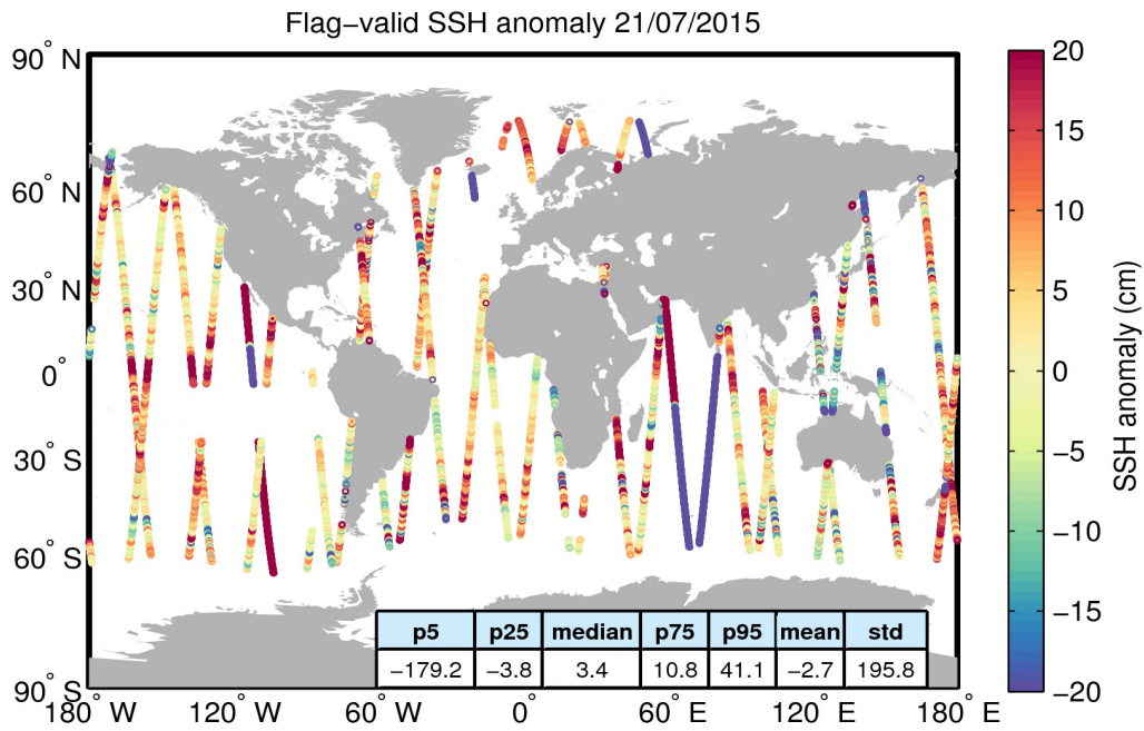
Figure 5. Geographical distribution of flag-valid 1-Hz SSH anomaly data over oceans and lakes for 21/07/2015. The statistical values shown in the table refer to the SSH anomaly in cm and are calculated over all measurements shown in the figure.
