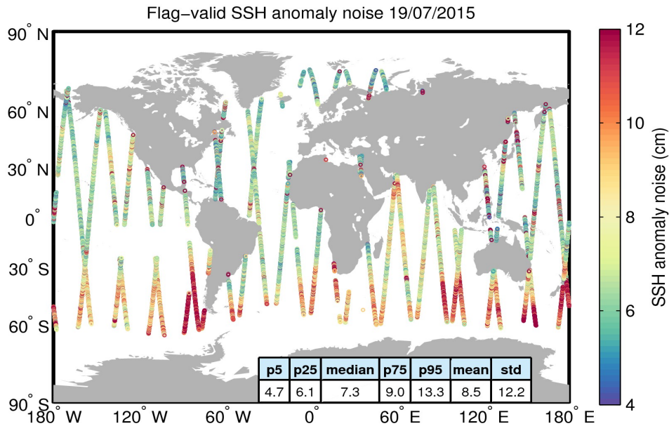
Figure 8. Geographical distribution of flag-valid 20-Hz SSH anomaly measurement noise over oceans and lakes for 19/07/2015. The statistical values shown in the table refer to the SSH anomaly noise and are calculated over all measurements shown in the figure.
