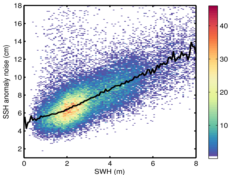
Figure 9. 2D histogram showing flag-valid SSH anomaly noise as a function of SWH for 19/07/2015. The black line denotes the median SSH anomaly as a function of SWH.
