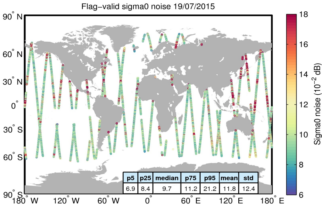
Figure 26. Geographical distribution of flag-valid 20-Hz sigma0 measurement noise over oceans and lakes for 19/07/2015. The statistical values shown in the table refer to the sigma0 noise and are calculated over all measurements shown in the figure.
