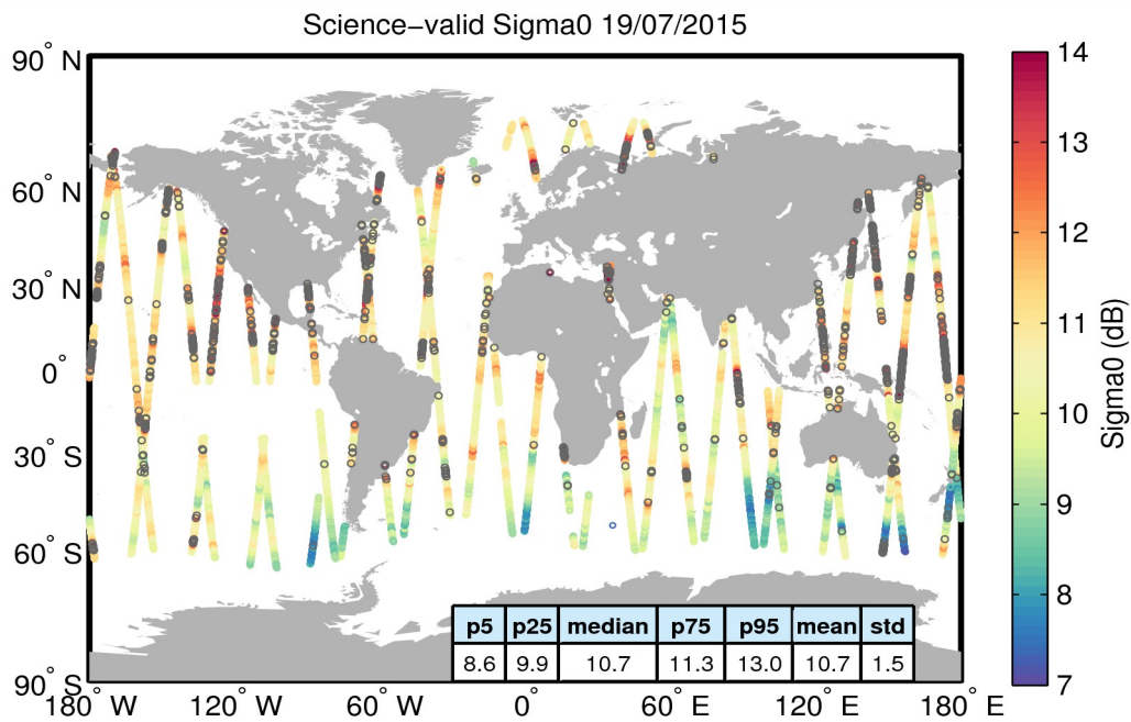
Figure 27. Geographical distribution of science-valid sigma0 data over oceans and lakes for 19/07/2015. The statistical values shown in the table refer to the sigma0 in dB and are calculated over all measurements shown in the figure. Gray circles denote records that have been rejected based on the editing criteria described in Table 4.
