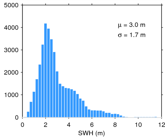
Figure 17. Histogram of flag-valid SWH over oceans and lakes for 19/07/2015. The mean ( \mu ) and standard deviation ( \sigma ) are also shown. Note that values larger than 12 m are excluded from the histogram for the sake of readability but not from the computation of \mu and \sigma .
