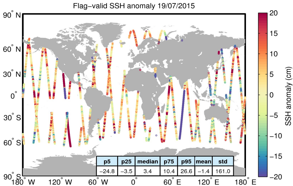
Figure 5. Geographical distribution of flag-valid 1-Hz SSH anomaly data over oceans and lakes for 19/07/2015. The statistical values shown in the table refer to the SSH anomaly in cm and are calculated over all measurements shown in the figure.
