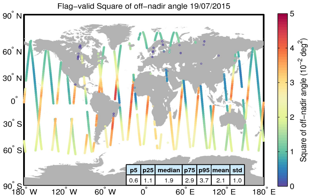
Figure 37. Geographical distribution of flag-valid mispointing data over oceans and lakes for 19/07/2015. The statistical values shown in the table refer to the mispointing in 10^{-2} \text{ deg}^2 and are calculated over all measurements shown in the figure.
