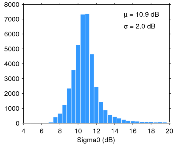
Figure 25. Histogram of flag-valid sigma0 over oceans and lakes for 19/07/2015. The mean ( \mu ) and standard deviation ( \sigma ) are also shown. Note that values outside [4 20] dB are excluded from the histogram for the sake of readability but not from the computation of \mu and \sigma .
