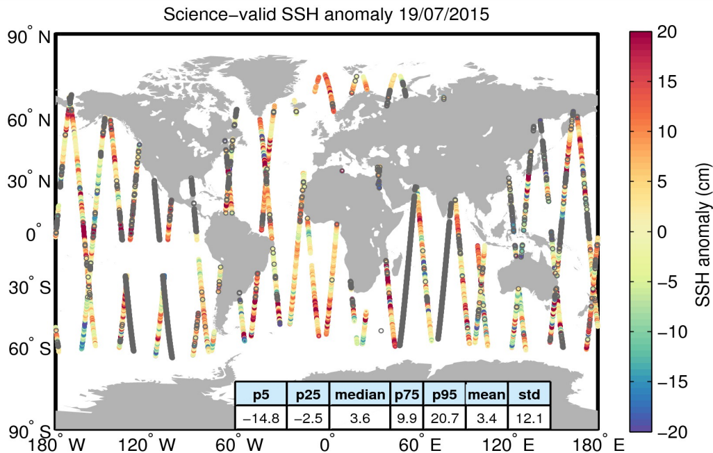
Figure 10. Geographical distribution of science-valid SSH anomaly data over oceans and lakes for 19/07/2015. The statistical values shown in the table refer to the SSH anomaly in cm and are calculated over all measurements shown in the figure. Gray circles denote records that have been rejected based on the editing criteria described in Table 2.
