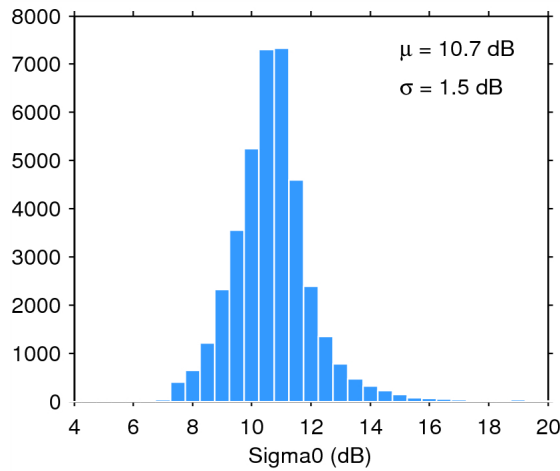
Figure 28. Histogram of science-valid sigma0 over oceans and lakes for 19/07/2015. The mean ( \mu ) and standard deviation ( \sigma ) are also shown. Note that values outside [4 20] dB are excluded from the histogram for the sake of readability but not from the computation of \mu and \sigma .
