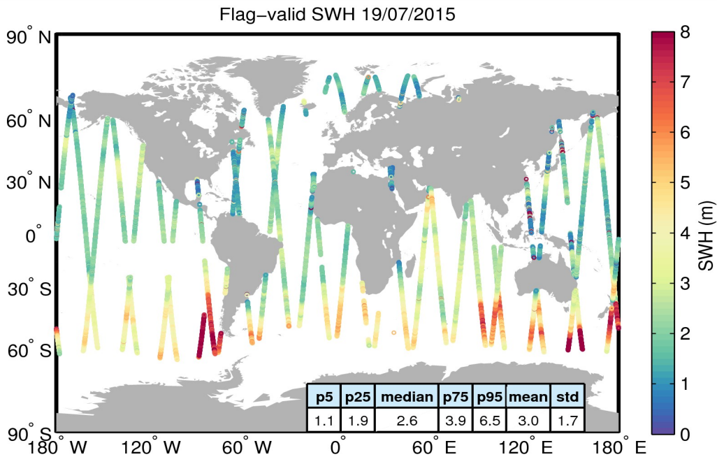
Figure 15. Geographical distribution of flag-valid SWH data over oceans and lakes for 19/07/2015. The statistical values shown in the table refer to the SWH in m and are calculated over all measurements shown in the figure.
