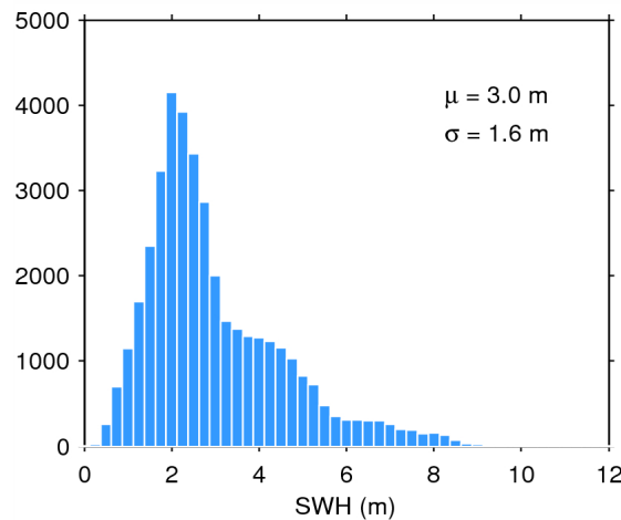
Figure 20. Histogram of science-valid SWH over oceans and lakes for 19/07/2015. The mean ( \mu ) and standard deviation ( \sigma ) are also shown. Note that values larger than 12 m are excluded from the histogram for the sake of readability but not from the computation of \mu and \sigma .
