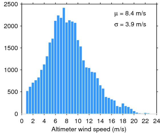
Figure 33. Histogram of flag-valid wind over oceans and lakes for 19/07/2015. The mean ( \mu ) and standard deviation ( \sigma ) are also shown. Note that values larger than 24 m/s are excluded from the histogram for the sake of readability but not from the computation of \mu and \sigma .
