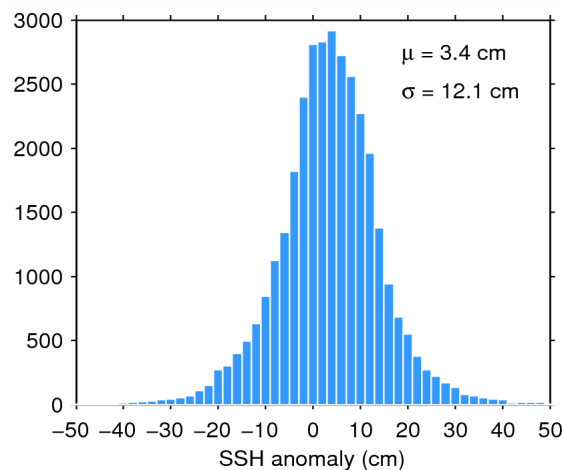
Figure 11. Histogram of science-valid SSH anomaly over oceans and lakes for 19/07/2015. The mean ( \mu ) and standard deviation ( \sigma ) are also shown. Note that values outside [-50 50] cm are excluded from the histogram for the sake of readability but not from the computation of \mu and \sigma .
