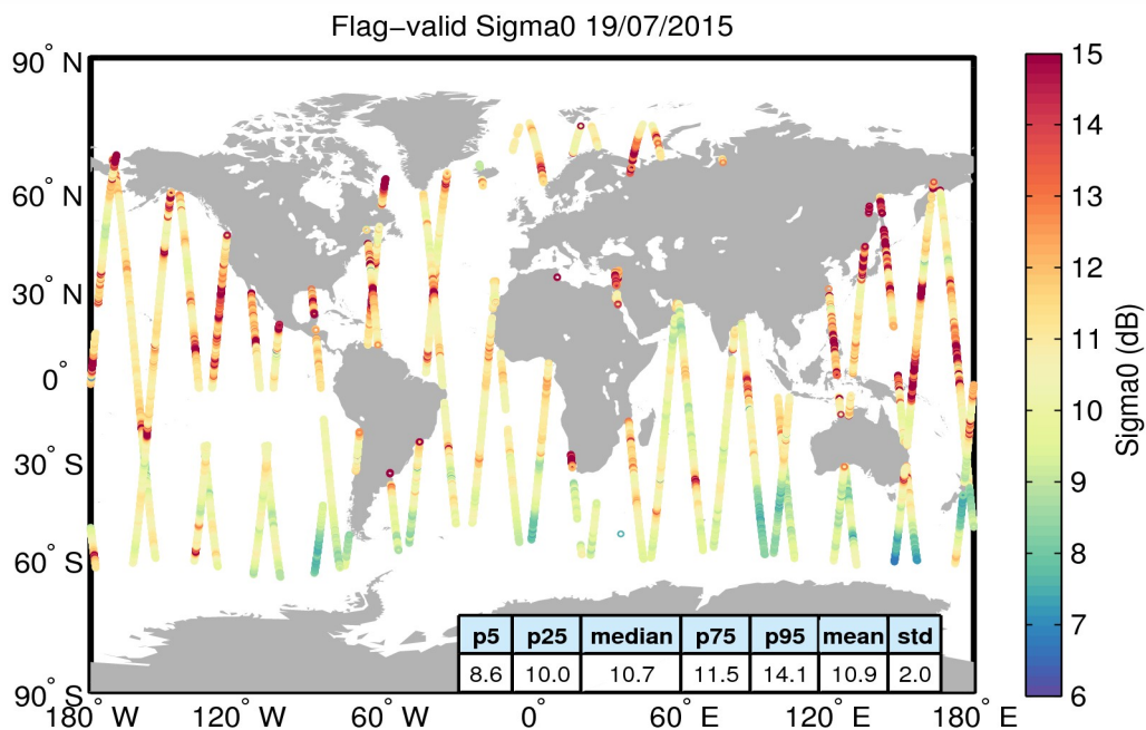
Figure 23. Geographical distribution of flag-valid sigma0 data over oceans and lakes for 19/07/2015. The statistical values shown in the table refer to the sigma0 in dB and are calculated over all measurements shown in the figure.
