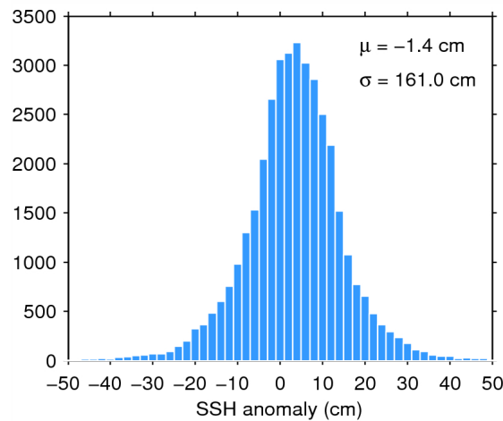
Figure 7. Histogram of flag-valid SSH anomaly over oceans and lakes for 19/07/2015. The mean ( \mu ) and standard deviation ( \sigma ) are also shown. Note that values outside [-50 50] cm are excluded from the histogram for the sake of readability but not from the computation of \mu and \sigma .
