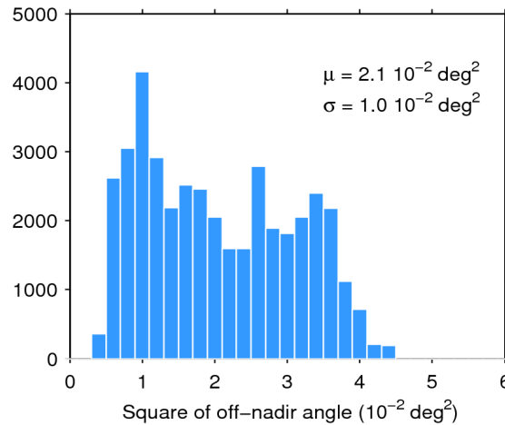
Figure 39. Histogram of flag-valid mispointing over oceans and lakes for 19/07/2015. The mean ( \mu ) and standard deviation ( \sigma ) are also shown. Note that values larger than 6 \cdot 10^{-2} \text{ deg}^2 are excluded from the histogram for the sake of readability but not from the computation of \mu and \sigma .
