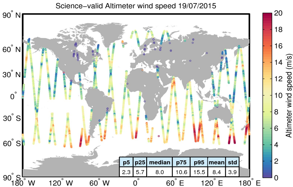
Figure 34. Geographical distribution of science-valid wind data over oceans and lakes for 19/07/2015. The statistical values shown in the table refer to the wind in m/s and are calculated over all measurements shown in the figure. Gray circles denote records that have been rejected based on the editing criteria described in Table 5.
