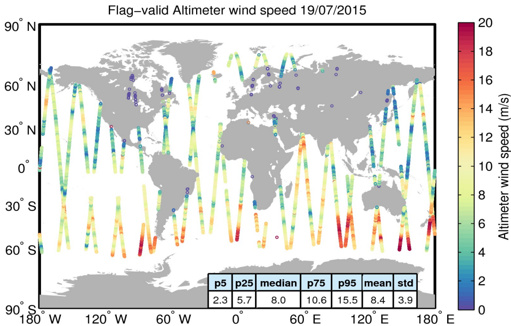
Figure 31. Geographical distribution of flag-valid wind data over oceans and lakes for 19/07/2015. The statistical values shown in the table refer to the wind in m/s and are calculated over all measurements shown in the figure.
