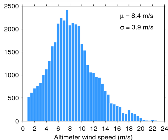
Figure 35. Histogram of science-valid wind over oceans and lakes for 19/07/2015. The mean ( \mu ) and standard deviation ( \sigma ) are also shown. Note that values larger than 24 m/s are excluded from the histogram for the sake of readability but not from the computation of \mu and \sigma .
