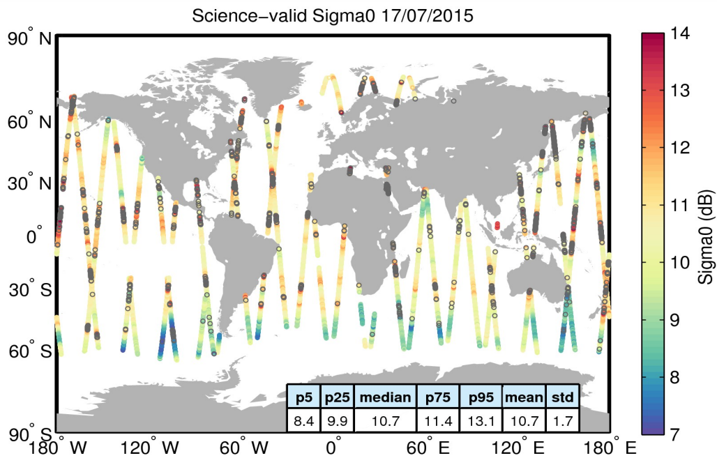
Figure 27. Geographical distribution of science-valid sigma0 data over oceans and lakes for 17/07/2015. The statistical values shown in the table refer to the sigma0 in dB and are calculated over all measurements shown in the figure. Gray circles denote records that have been rejected based on the editing criteria described in Table 4.
