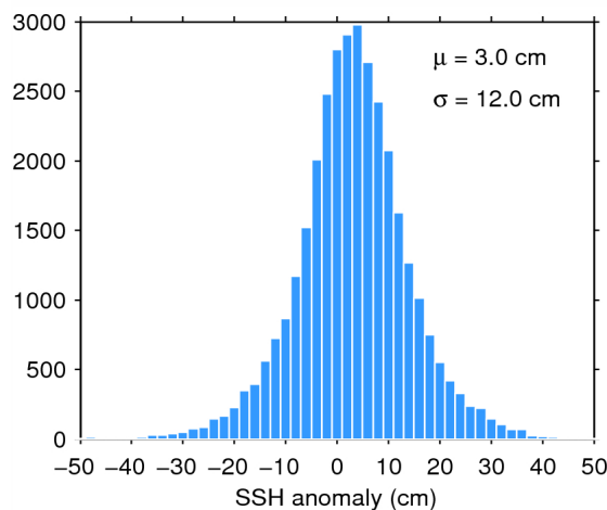
Figure 11. Histogram of science-valid SSH anomaly over oceans and lakes for 17/07/2015. The mean ( \mu ) and standard deviation ( \sigma ) are also shown. Note that values outside [-50 50] cm are excluded from the histogram for the sake of readability but not from the computation of \mu and \sigma .
