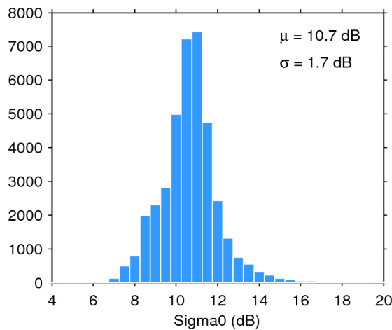
Figure 28. Histogram of science-valid sigma0 over oceans and lakes for 17/07/2015. The mean ( \mu ) and standard deviation ( \sigma ) are also shown. Note that values outside [4 20] dB are excluded from the histogram for the sake of readability but not from the computation of \mu and \sigma .
