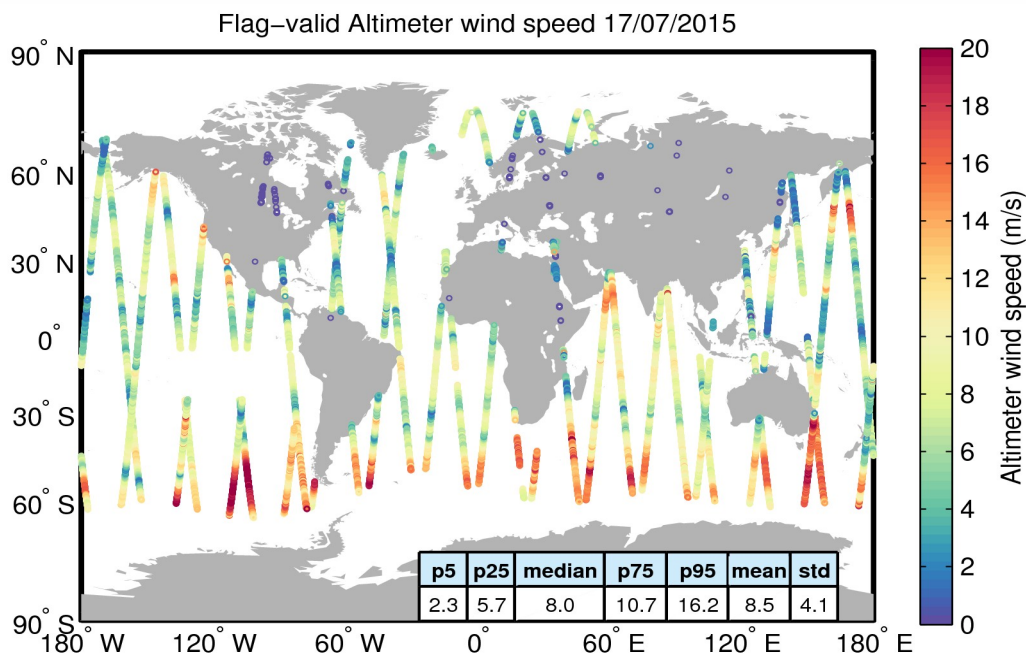
Figure 31. Geographical distribution of flag-valid wind data over oceans and lakes for 17/07/2015. The statistical values shown in the table refer to the wind in m/s and are calculated over all measurements shown in the figure.
