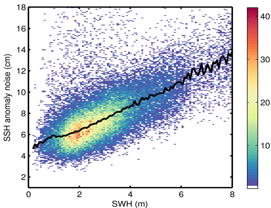
Figure 9. 2D histogram showing flag-valid SSH anomaly noise as a function of SWH for 17/07/2015. The black line denotes the median SSH anomaly as a function of SWH.
