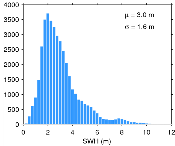
Figure 17. Histogram of flag-valid SWH over oceans and lakes for 17/07/2015. The mean ( \mu ) and standard deviation ( \sigma ) are also shown. Note that values larger than 12 m are excluded from the histogram for the sake of readability but not from the computation of \mu and \sigma .
