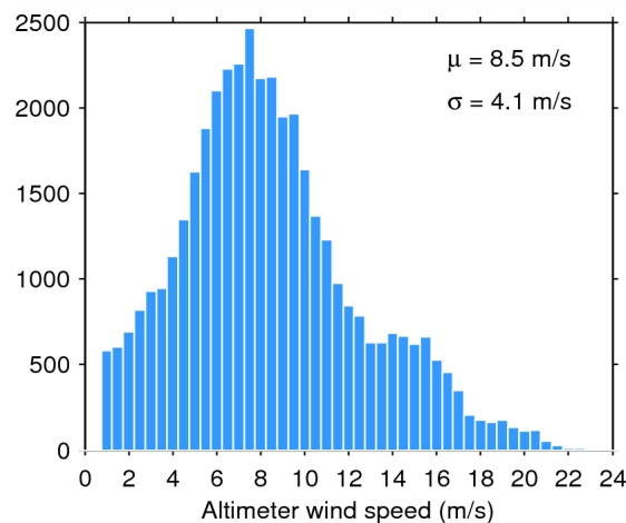
Figure 35. Histogram of science-valid wind over oceans and lakes for 17/07/2015. The mean ( \mu ) and standard deviation ( \sigma ) are also shown. Note that values larger than 24 m/s are excluded from the histogram for the sake of readability but not from the computation of \mu and \sigma .
