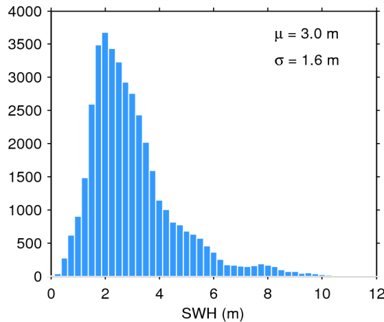
Figure 20. Histogram of science-valid SWH over oceans and lakes for 17/07/2015. The mean ( \mu ) and standard deviation ( \sigma ) are also shown. Note that values larger than 12 m are excluded from the histogram for the sake of readability but not from the computation of \mu and \sigma .
