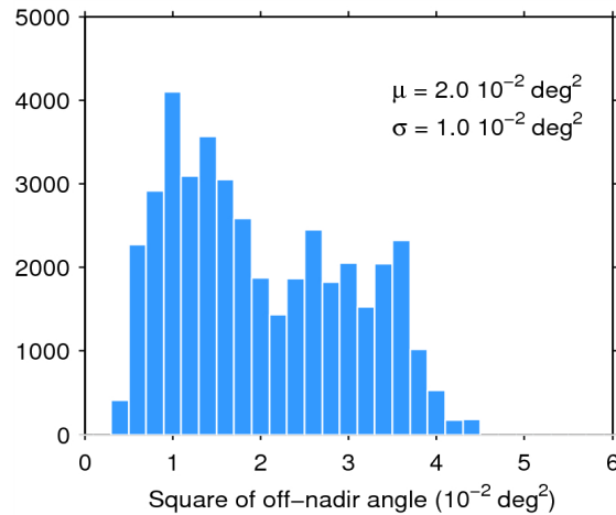
Figure 39. Histogram of flag-valid mispointing over oceans and lakes for 17/07/2015. The mean ( \mu ) and standard deviation ( \sigma ) are also shown. Note that values larger than 6 \cdot 10^{-2} \text{ deg}^2 are excluded from the histogram for the sake of readability but not from the computation of \mu and \sigma .
