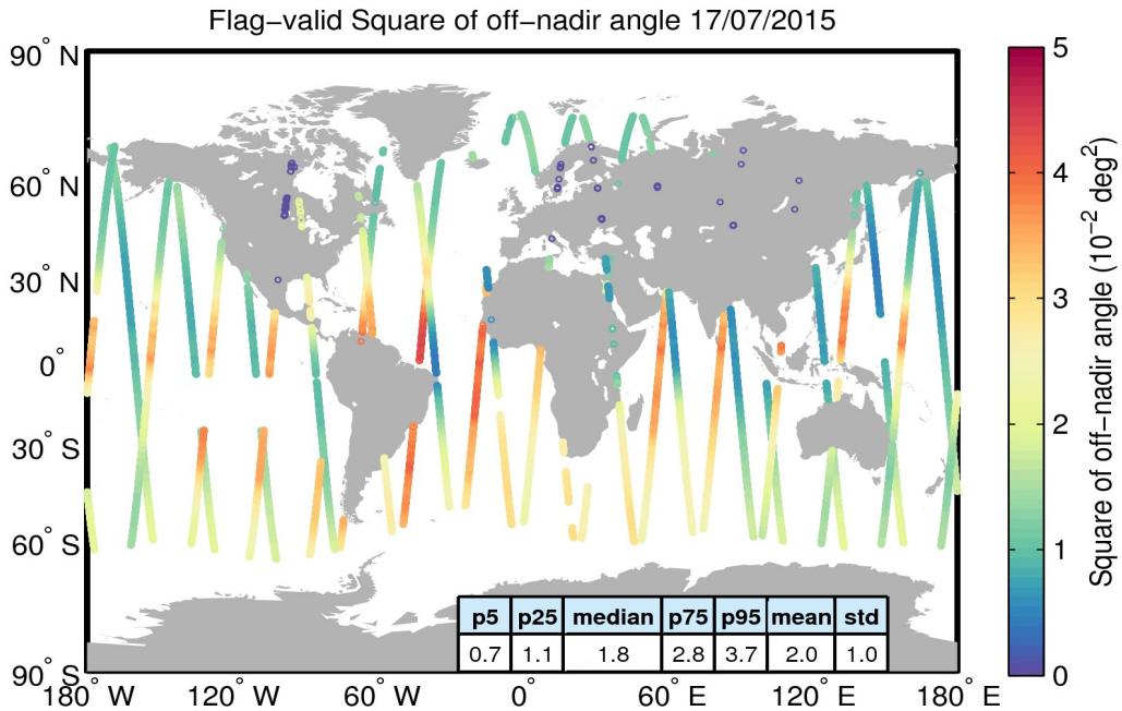
Figure 37. Geographical distribution of flag-valid mispointing data over oceans and lakes for 17/07/2015. The statistical values shown in the table refer to the mispointing in 10^{-2} \text{deg}^2 and are calculated over all measurements shown in the figure.
