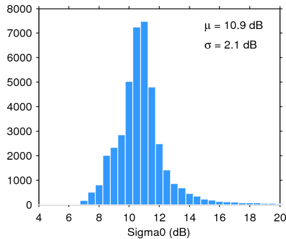
Figure 25. Histogram of flag-valid sigma0 over oceans and lakes for 17/07/2015. The mean ( \mu ) and standard deviation ( \sigma ) are also shown. Note that values outside [4 20] dB are excluded from the histogram for the sake of readability but not from the computation of \mu and \sigma .
