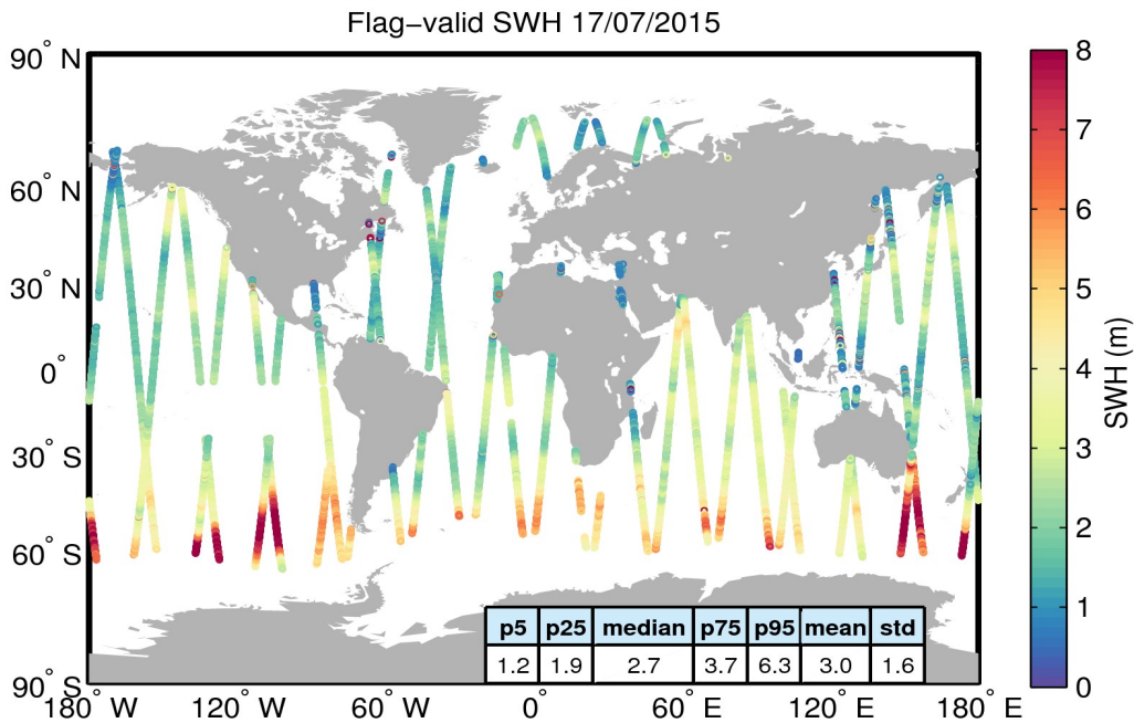
Figure 15. Geographical distribution of flag-valid SWH data over oceans and lakes for 17/07/2015. The statistical values shown in the table refer to the SWH in m and are calculated over all measurements shown in the figure.
