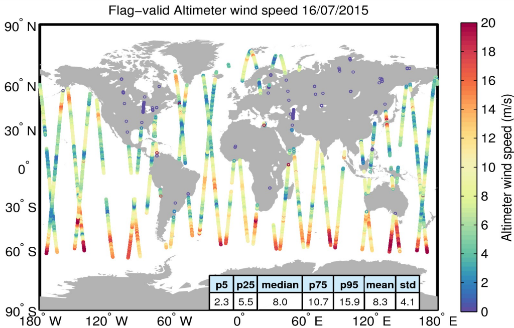
Figure 31. Geographical distribution of flag-valid wind data over oceans and lakes for 16/07/2015. The statistical values shown in the table refer to the wind in m/s and are calculated over all measurements shown in the figure.
