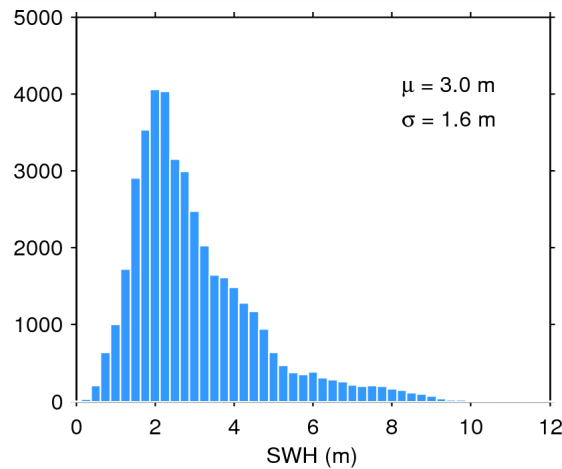
Figure 17. Histogram of flag-valid SWH over oceans and lakes for 15/07/2015. The mean ( \mu ) and standard deviation ( \sigma ) are also shown. Note that values larger than 12 m are excluded from the histogram for the sake of readability but not from the computation of \mu and \sigma .
