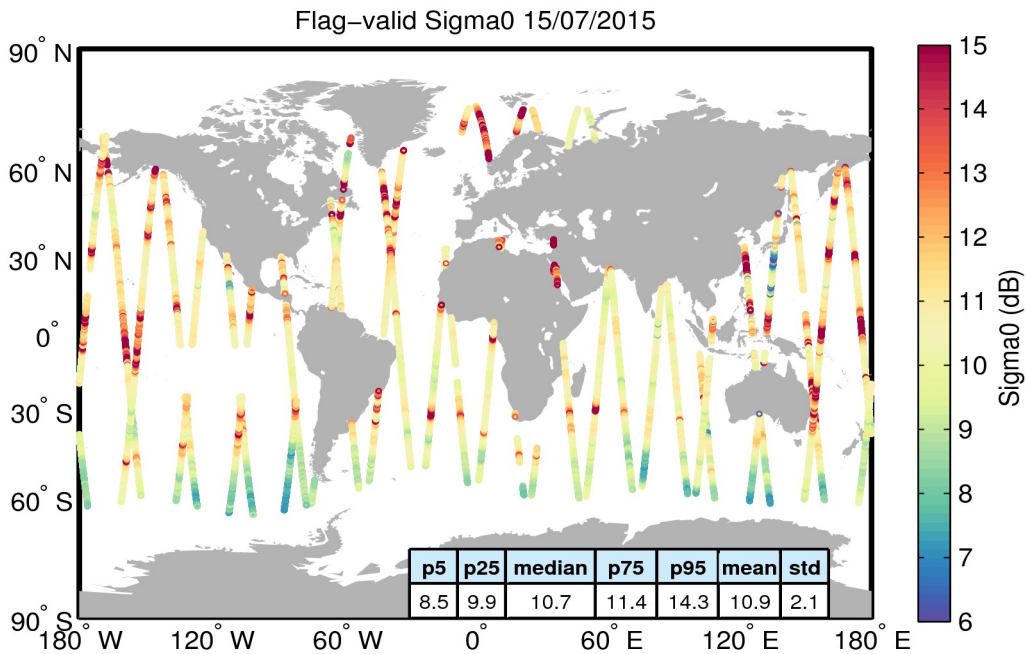
Figure 23. Geographical distribution of flag-valid sigma0 data over oceans and lakes for 15/07/2015. The statistical values shown in the table refer to the sigma0 in dB and are calculated over all measurements shown in the figure.
