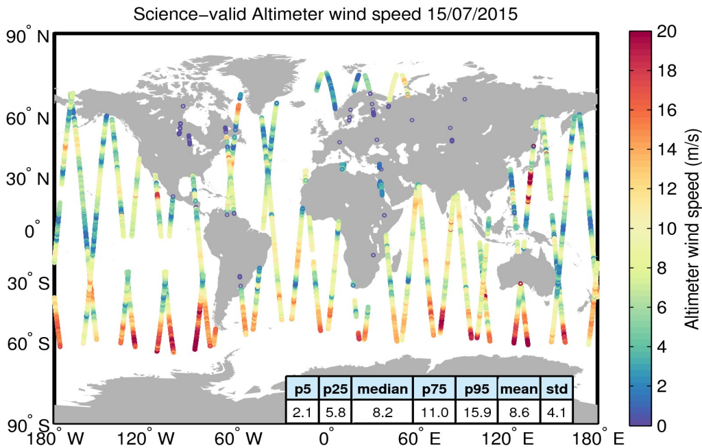
Figure 34. Geographical distribution of science-valid wind data over oceans and lakes for 15/07/2015. The statistical values shown in the table refer to the wind in m/s and are calculated over all measurements shown in the figure. Gray circles denote records that have been rejected based on the editing criteria described in Table 5.
