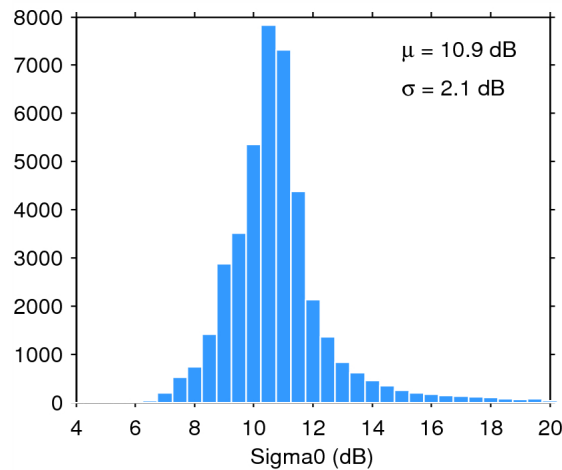
Figure 25. Histogram of flag-valid sigma0 over oceans and lakes for 15/07/2015. The mean ( \mu ) and standard deviation ( \sigma ) are also shown. Note that values outside [4 20] dB are excluded from the histogram for the sake of readability but not from the computation of \mu and \sigma .
