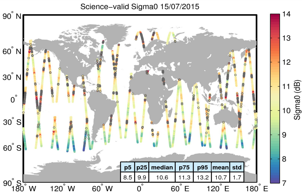
Figure 27. Geographical distribution of science-valid sigma0 data over oceans and lakes for 15/07/2015. The statistical values shown in the table refer to the sigma0 in dB and are calculated over all measurements shown in the figure. Gray circles denote records that have been rejected based on the editing criteria described in Table 4.
