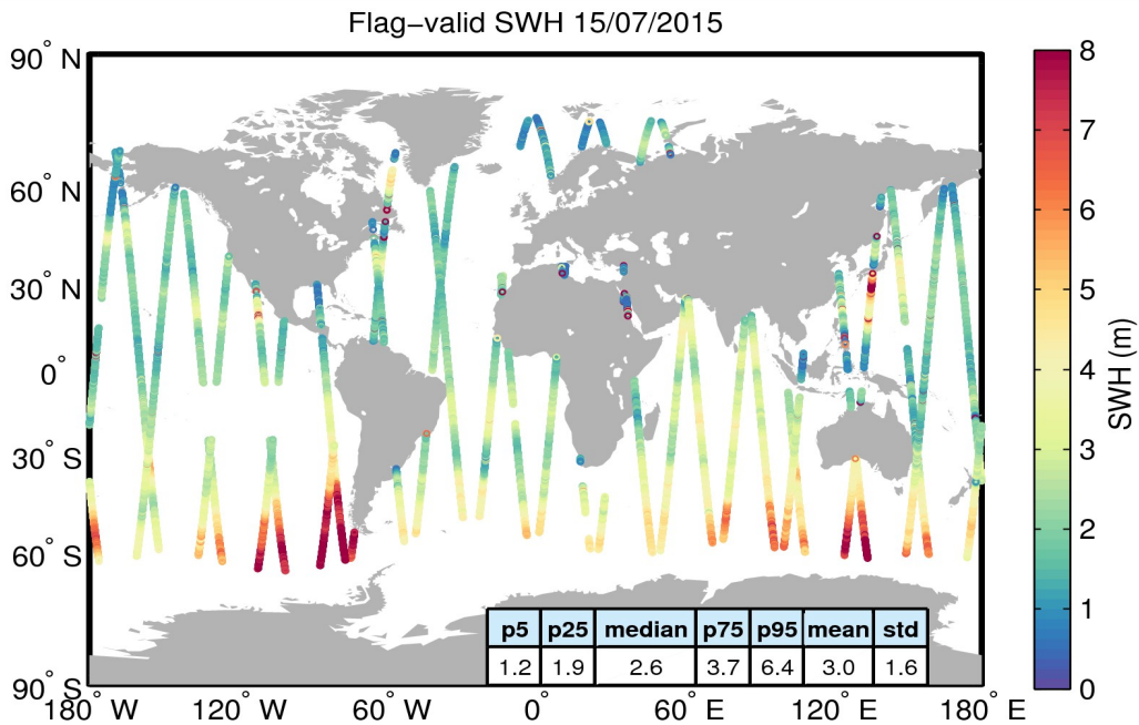
Figure 15. Geographical distribution of flag-valid SWH data over oceans and lakes for 15/07/2015. The statistical values shown in the table refer to the SWH in m and are calculated over all measurements shown in the figure.
