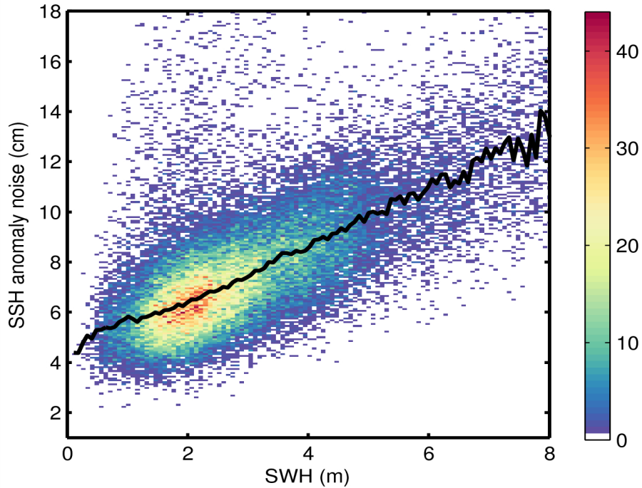
Figure 9. 2D histogram showing flag-valid SSH anomaly noise as a function of SWH for 15/07/2015. The black line denotes the median SSH anomaly as a function of SWH.
