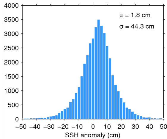
Figure 7. Histogram of flag-valid SSH anomaly over oceans and lakes for 15/07/2015. The mean ( \mu ) and standard deviation ( \sigma ) are also shown. Note that values outside [-50\ 50] cm are excluded from the histogram for the sake of readability but not from the computation of \mu and \sigma .
