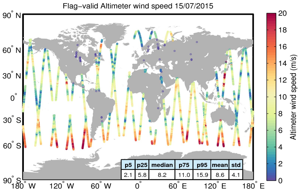
Figure 31. Geographical distribution of flag-valid wind data over oceans and lakes for 15/07/2015. The statistical values shown in the table refer to the wind in m/s and are calculated over all measurements shown in the figure.
