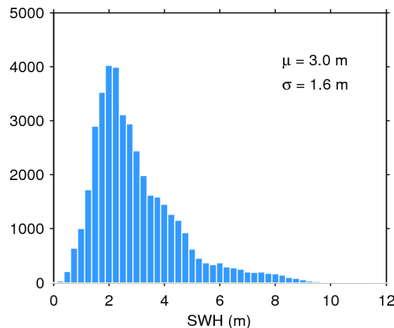
Figure 20. Histogram of science-valid SWH over oceans and lakes for 15/07/2015. The mean ( \mu ) and standard deviation ( \sigma ) are also shown. Note that values larger than 12 m are excluded from the histogram for the sake of readability but not from the computation of \mu and \sigma .
