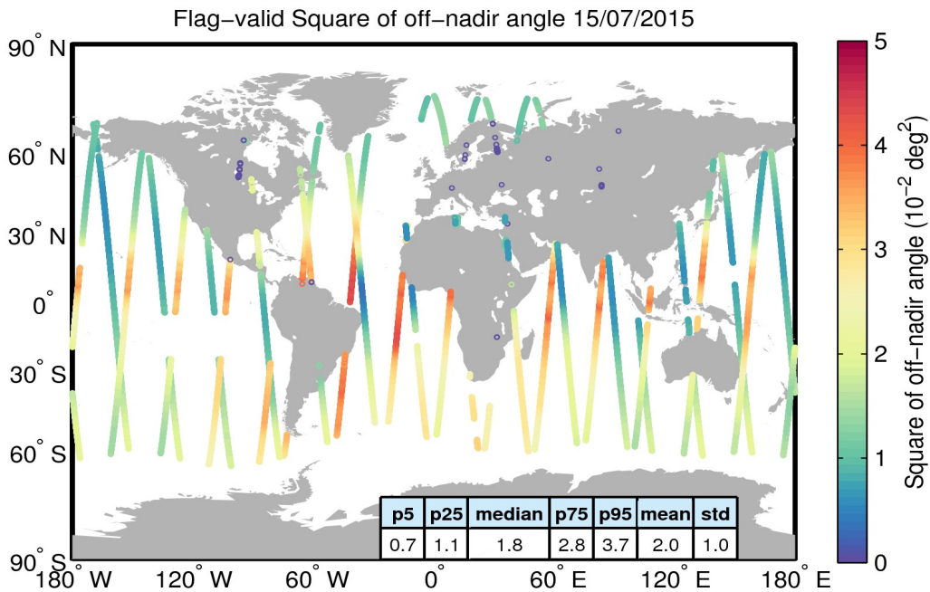
Figure 37. Geographical distribution of flag-valid mispointing data over oceans and lakes for 15/07/2015. The statistical values shown in the table refer to the mispointing in 10^{-2} \text{ deg}^2 and are calculated over all measurements shown in the figure.
