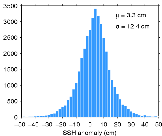
Figure 11. Histogram of science-valid SSH anomaly over oceans and lakes for 15/07/2015. The mean ( \mu ) and standard deviation ( \sigma ) are also shown. Note that values outside [-50 50] cm are excluded from the histogram for the sake of readability but not from the computation of \mu and \sigma .
