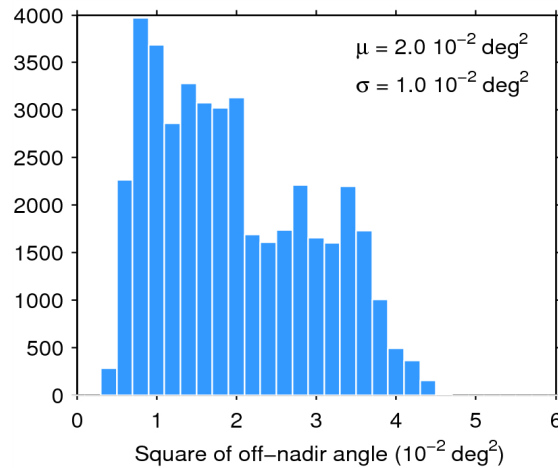
Figure 39. Histogram of flag-valid mispointing over oceans and lakes for 15/07/2015. The mean ( \mu ) and standard deviation ( \sigma ) are also shown. Note that values larger than 6 \cdot 10^{-2} \text{ deg}^2 are excluded from the histogram for the sake of readability but not from the computation of \mu and \sigma .
