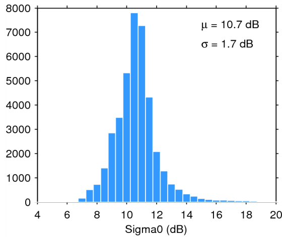
Figure 28. Histogram of science-valid sigma0 over oceans and lakes for 15/07/2015. The mean ( \mu ) and standard deviation ( \sigma ) are also shown. Note that values outside [4 20] dB are excluded from the histogram for the sake of readability but not from the computation of \mu and \sigma .
