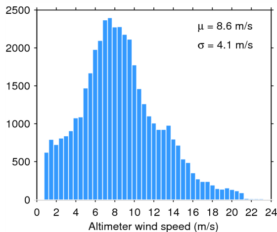
Figure 35. Histogram of science-valid wind over oceans and lakes for 15/07/2015. The mean ( \mu ) and standard deviation ( \sigma ) are also shown. Note that values larger than 24 m/s are excluded from the histogram for the sake of readability but not from the computation of \mu and \sigma .
