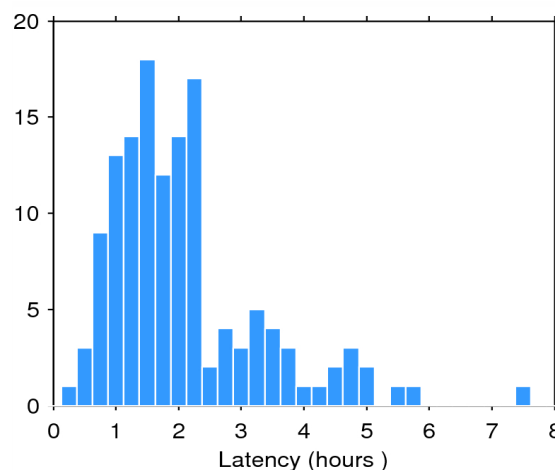
Figure 2. Histogram of the data latency for 15/07/2015. The y-axis denotes the number of files that are made available with a delay of x-hours with respect to the mean time of the records stored in the file.
