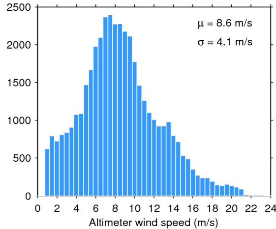
Figure 33. Histogram of flag-valid wind over oceans and lakes for 15/07/2015. The mean ( \mu ) and standard deviation ( \sigma ) are also shown. Note that values larger than 24 m/s are excluded from the histogram for the sake of readability but not from the computation of \mu and \sigma .
