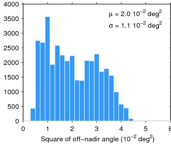
Figure 39. Histogram of flag-valid mispointing over oceans and lakes for 14/07/2015. The mean ( \mu ) and standard deviation ( \sigma ) are also shown. Note that values larger than 6 \cdot 10^{-2} \text{ deg}^2 are excluded from the histogram for the sake of readability but not from the computation of \mu and \sigma .
