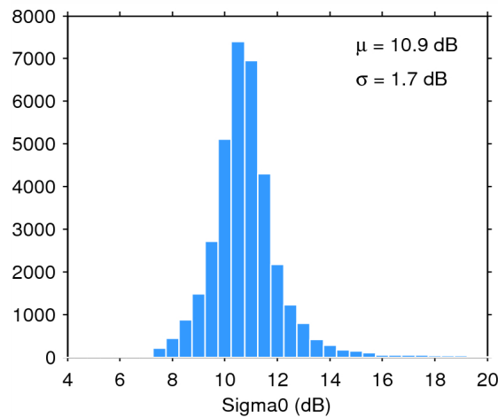
Figure 28. Histogram of science-valid sigma0 over oceans and lakes for 14/07/2015. The mean ( \mu ) and standard deviation ( \sigma ) are also shown. Note that values outside [4 20] dB are excluded from the histogram for the sake of readability but not from the computation of \mu and \sigma .
