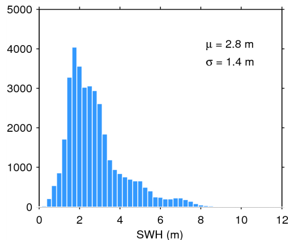
Figure 20. Histogram of science-valid SWH over oceans and lakes for 14/07/2015. The mean ( \mu ) and standard deviation ( \sigma ) are also shown. Note that values larger than 12 m are excluded from the histogram for the sake of readability but not from the computation of \mu and \sigma .
