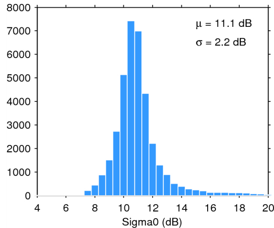
Figure 25. Histogram of flag-valid sigma0 over oceans and lakes for 14/07/2015. The mean ( \mu ) and standard deviation ( \sigma ) are also shown. Note that values outside [4 20] dB are excluded from the histogram for the sake of readability but not from the computation of \mu and \sigma .
