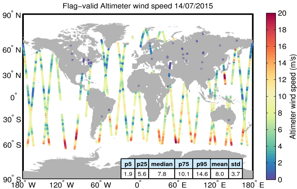
Figure 31. Geographical distribution of flag-valid wind data over oceans and lakes for 14/07/2015. The statistical values shown in the table refer to the wind in m/s and are calculated over all measurements shown in the figure.
