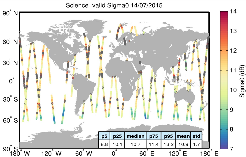
Figure 27. Geographical distribution of science-valid sigma0 data over oceans and lakes for 14/07/2015. The statistical values shown in the table refer to the sigma0 in dB and are calculated over all measurements shown in the figure. Gray circles denote records that have been rejected based on the editing criteria described in Table 4.
