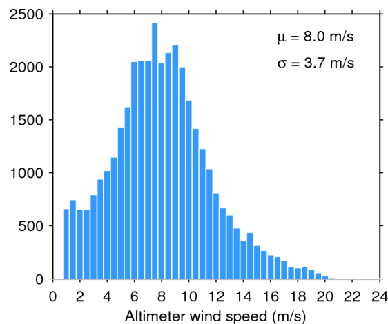
Figure 35. Histogram of science-valid wind over oceans and lakes for 14/07/2015. The mean ( \mu ) and standard deviation ( \sigma ) are also shown. Note that values larger than 24 m/s are excluded from the histogram for the sake of readability but not from the computation of \mu and \sigma .
