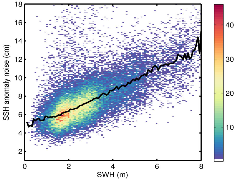
Figure 9. 2D histogram showing flag-valid SSH anomaly noise as a function of SWH for 14/07/2015. The black line denotes the median SSH anomaly as a function of SWH.
