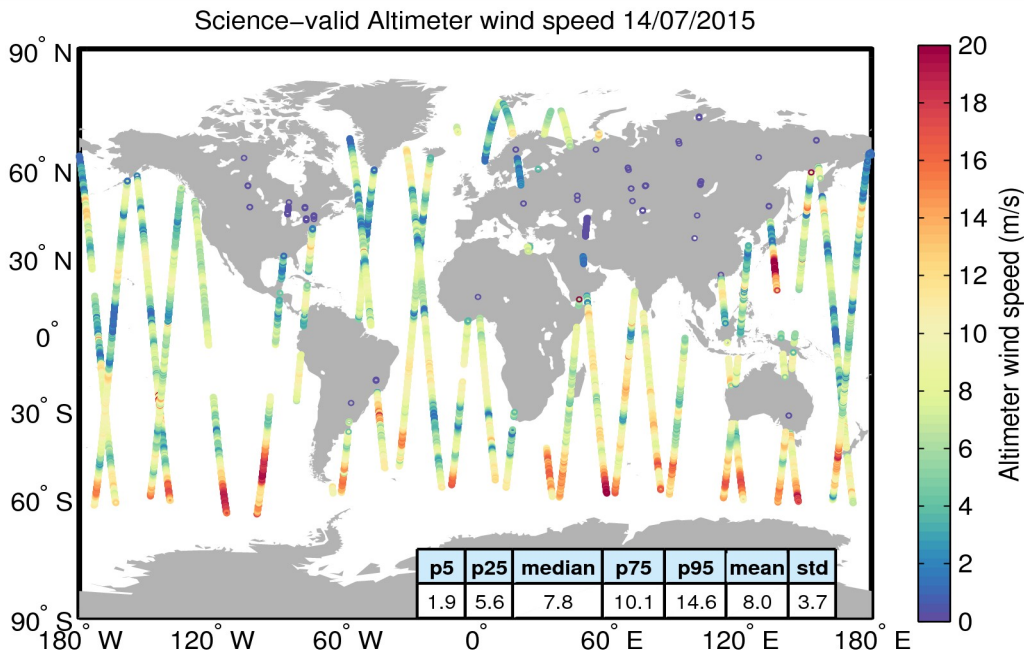
Figure 34. Geographical distribution of science-valid wind data over oceans and lakes for 14/07/2015. The statistical values shown in the table refer to the wind in m/s and are calculated over all measurements shown in the figure. Gray circles denote records that have been rejected based on the editing criteria described in Table 5.
