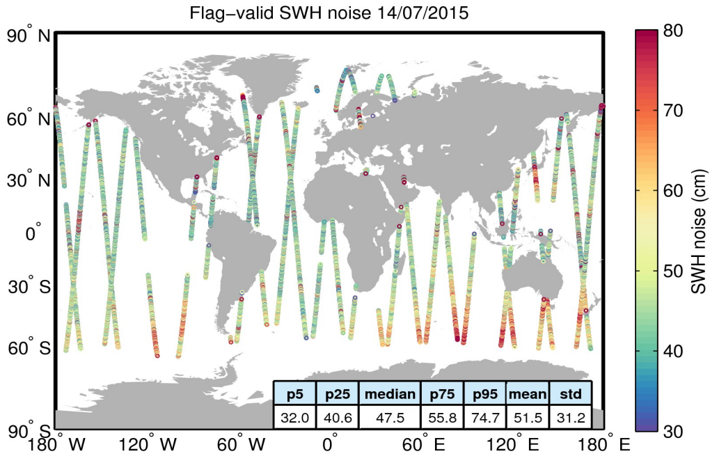
Figure 18. Geographical distribution of flag-valid 20-Hz SWH measurement noise over oceans and lakes for 14/07/2015. The statistical values shown in the figure refer to the SWH noise and are calculated over all measurements shown in the figure.
