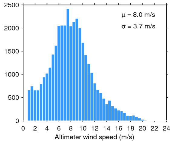
Figure 33. Histogram of flag-valid wind over oceans and lakes for 14/07/2015. The mean ( \mu ) and standard deviation ( \sigma ) are also shown. Note that values larger than 24 m/s are excluded from the histogram for the sake of readability but not from the computation of \mu and \sigma .
