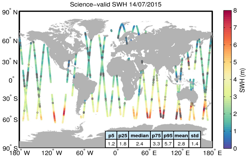
Figure 19. Geographical distribution of science-valid SWH data over oceans and lakes for 14/07/2015. The statistical values shown in the table refer to the SWH in m and are calculated over all measurements shown in the figure. Gray circles denote records that have been rejected based on the editing criteria described in Table 3.
