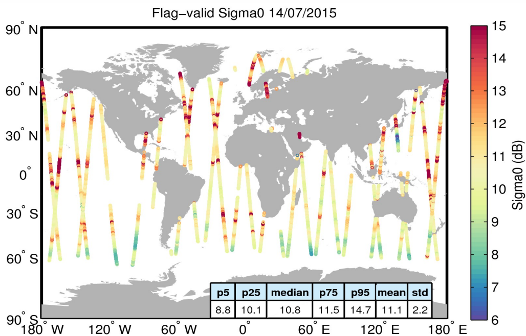
Figure 23. Geographical distribution of flag-valid sigma0 data over oceans and lakes for 14/07/2015. The statistical values shown in the table refer to the sigma0 in dB and are calculated over all measurements shown in the figure.
