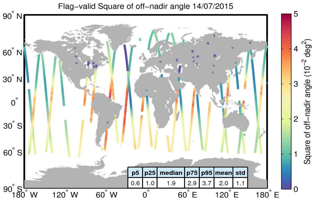
Figure 37. Geographical distribution of flag-valid mispointing data over oceans and lakes for 14/07/2015. The statistical values shown in the table refer to the mispointing in 10^{-2} \text{deg}^2 and are calculated over all measurements shown in the figure.
