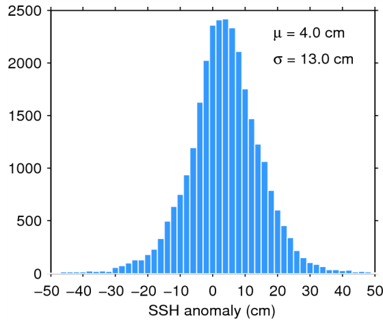
Figure 11. Histogram of science-valid SSH anomaly over oceans and lakes for 14/07/2015. The mean ( \mu ) and standard deviation ( \sigma ) are also shown. Note that values outside [-50 50] cm are excluded from the histogram for the sake of readability but not from the computation of \mu and \sigma .
