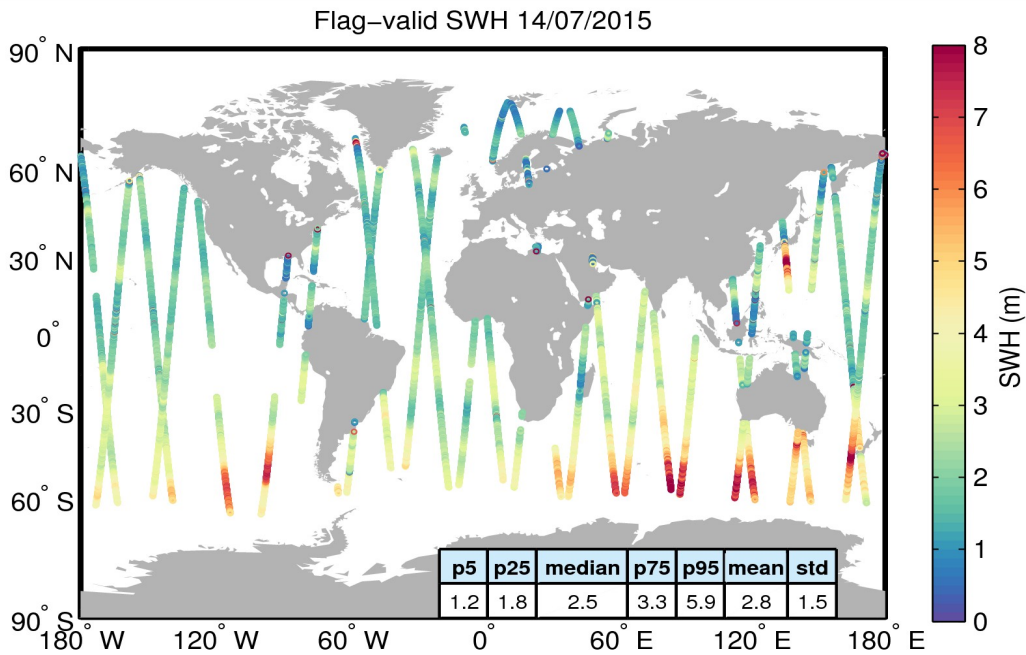
Figure 15. Geographical distribution of flag-valid SWH data over oceans and lakes for 14/07/2015. The statistical values shown in the table refer to the SWH in m and are calculated over all measurements shown in the figure.
