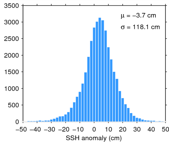
Figure 7. Histogram of flag-valid SSH anomaly over oceans and lakes for 14/07/2015. The mean ( \mu ) and standard deviation ( \sigma ) are also shown. Note that values outside [-50\ 50] cm are excluded from the histogram for the sake of readability but not from the computation of \mu and \sigma .
