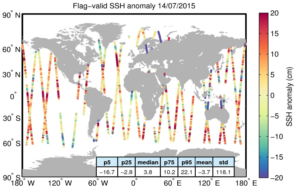
Figure 5. Geographical distribution of flag-valid 1-Hz SSH anomaly data over oceans and lakes for 14/07/2015. The statistical values shown in the table refer to the SSH anomaly in cm and are calculated over all measurements shown in the figure.
