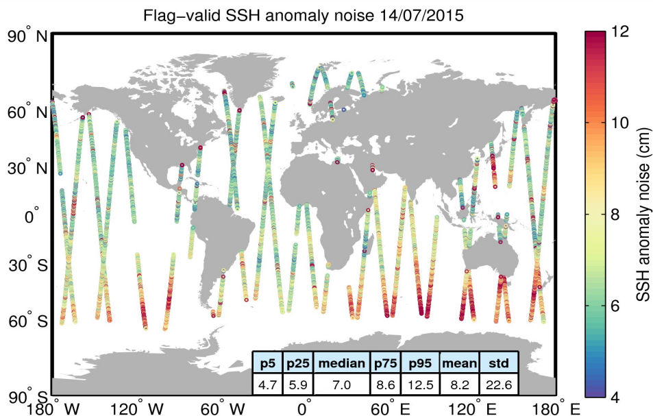
Figure 8. Geographical distribution of flag-valid 20-Hz SSH anomaly measurement noise over oceans and lakes for 14/07/2015. The statistical values shown in the table refer to the SSH anomaly noise and are calculated over all measurements shown in the figure.
