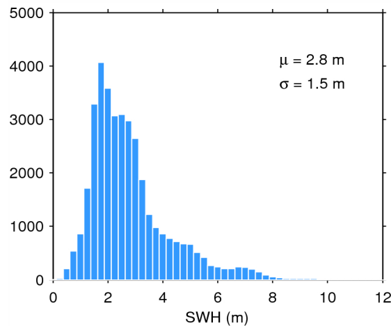
Figure 17. Histogram of flag-valid SWH over oceans and lakes for 14/07/2015. The mean ( \mu ) and standard deviation ( \sigma ) are also shown. Note that values larger than 12 m are excluded from the histogram for the sake of readability but not from the computation of \mu and \sigma .
