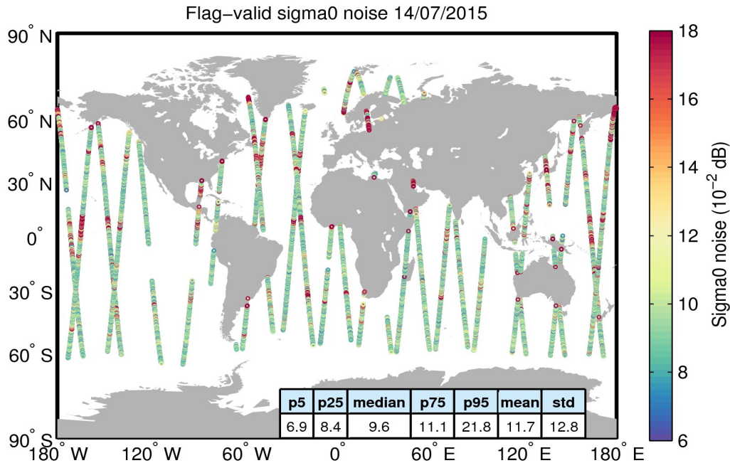
Figure 26. Geographical distribution of flag-valid 20-Hz sigma0 measurement noise over oceans and lakes for 14/07/2015. The statistical values shown in the table refer to the sigma0 noise and are calculated over all measurements shown in the figure.
