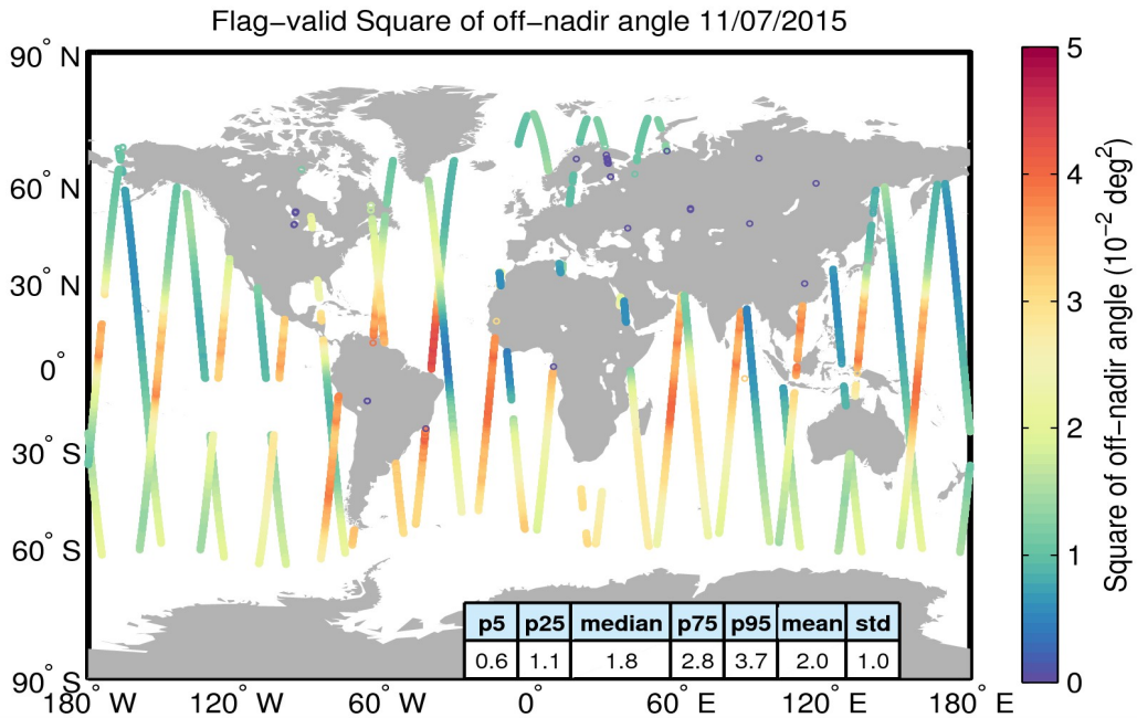
Figure 37. Geographical distribution of flag-valid mispointing data over oceans and lakes for 11/07/2015. The statistical values shown in the table refer to the mispointing in 10^{-2} \text{deg}^2 and are calculated over all measurements shown in the figure.
