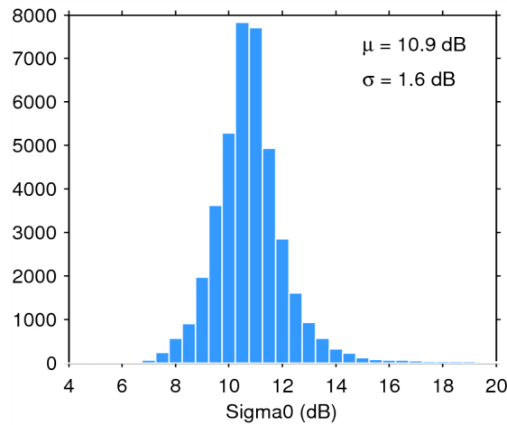
Figure 28. Histogram of science-valid sigma0 over oceans and lakes for 11/07/2015. The mean ( \mu ) and standard deviation ( \sigma ) are also shown. Note that values outside [4 20] dB are excluded from the histogram for the sake of readability but not from the computation of \mu and \sigma .
