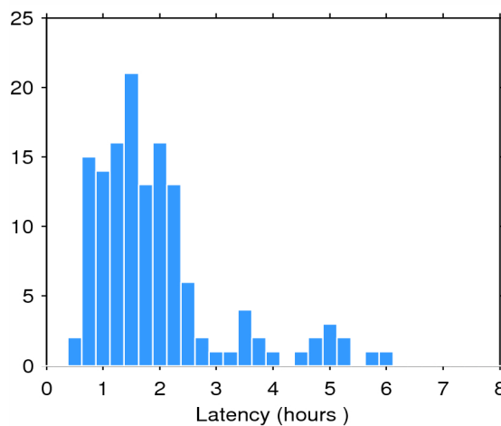
Figure 2. Histogram of the data latency for 11/07/2015. The y-axis denotes the number of files that are made available with a delay of x-hours with respect to the mean time of the records stored in the file.
