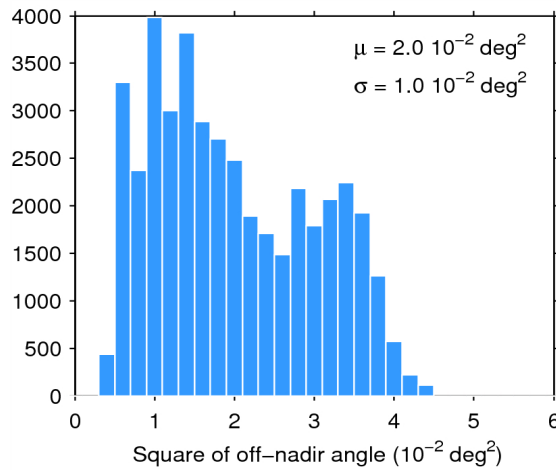
Figure 39. Histogram of flag-valid mispointing over oceans and lakes for 11/07/2015. The mean ( \mu ) and standard deviation ( \sigma ) are also shown. Note that values larger than 6 \cdot 10^{-2} \text{ deg}^2 are excluded from the histogram for the sake of readability but not from the computation of \mu and \sigma .
