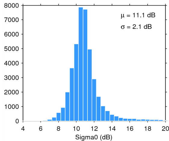
Figure 25. Histogram of flag-valid sigma0 over oceans and lakes for 11/07/2015. The mean ( \mu ) and standard deviation ( \sigma ) are also shown. Note that values outside [4 20] dB are excluded from the histogram for the sake of readability but not from the computation of \mu and \sigma .
