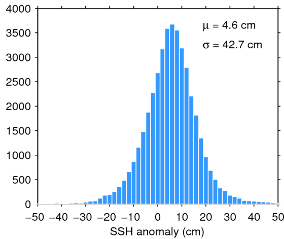
Figure 7. Histogram of flag-valid SSH anomaly over oceans and lakes for 11/07/2015. The mean ( \mu ) and standard deviation ( \sigma ) are also shown. Note that values outside [-50\ 50] cm are excluded from the histogram for the sake of readability but not from the computation of \mu and \sigma .
