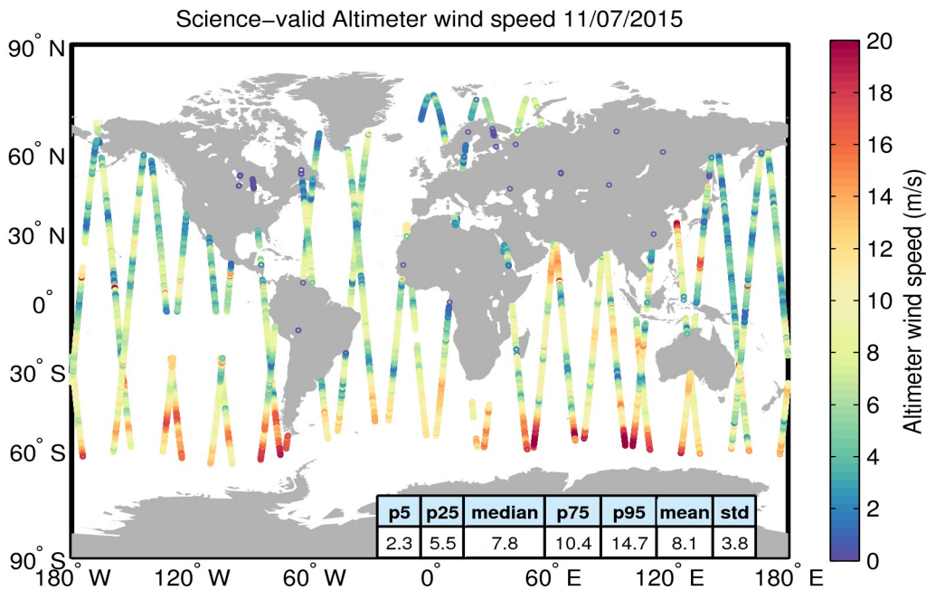
Figure 34. Geographical distribution of science-valid wind data over oceans and lakes for 11/07/2015. The statistical values shown in the table refer to the wind in m/s and are calculated over all measurements shown in the figure. Gray circles denote records that have been rejected based on the editing criteria described in Table 5.
