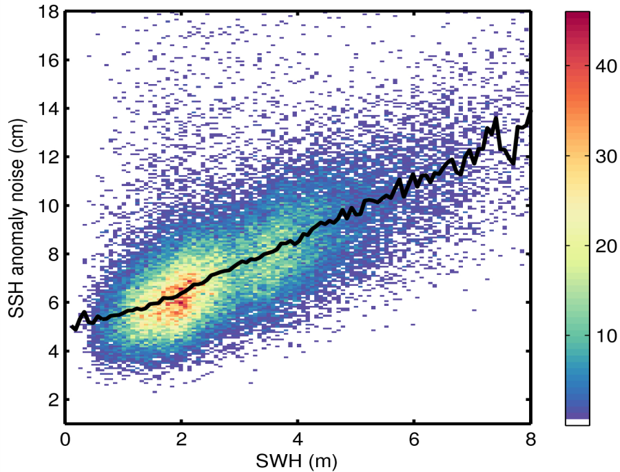
Figure 9. 2D histogram showing flag-valid SSH anomaly noise as a function of SWH for 11/07/2015. The black line denotes the median SSH anomaly as a function of SWH.
