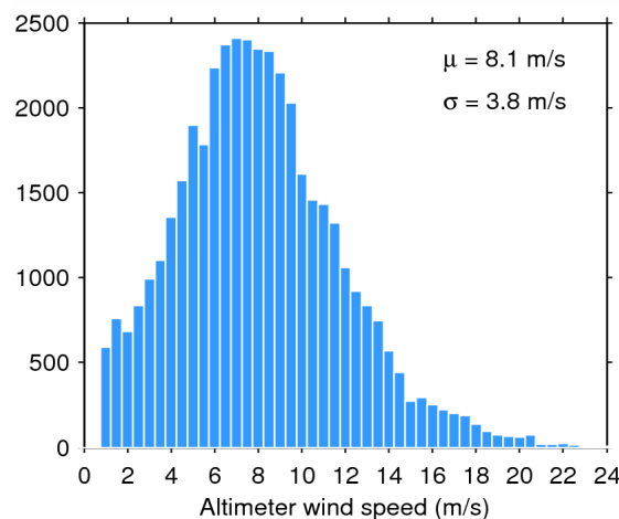
Figure 35. Histogram of science-valid wind over oceans and lakes for 11/07/2015. The mean ( \mu ) and standard deviation ( \sigma ) are also shown. Note that values larger than 24 m/s are excluded from the histogram for the sake of readability but not from the computation of \mu and \sigma .
