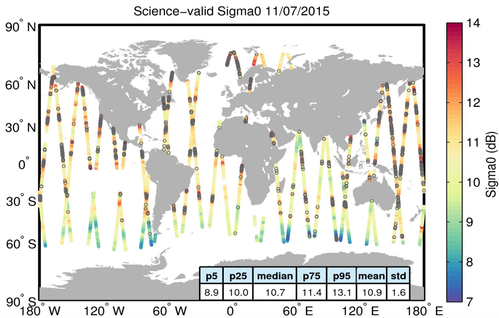
Figure 27. Geographical distribution of science-valid sigma0 data over oceans and lakes for 11/07/2015. The statistical values shown in the table refer to the sigma0 in dB and are calculated over all measurements shown in the figure. Gray circles denote records that have been rejected based on the editing criteria described in Table 4.
