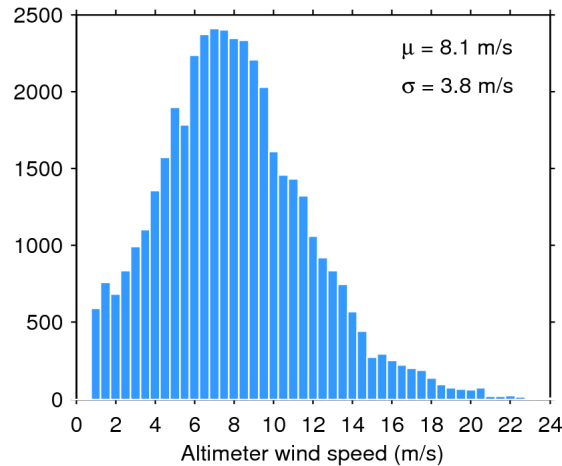
Figure 33. Histogram of flag-valid wind over oceans and lakes for 11/07/2015. The mean ( \mu ) and standard deviation ( \sigma ) are also shown. Note that values larger than 24 m/s are excluded from the histogram for the sake of readability but not from the computation of \mu and \sigma .
