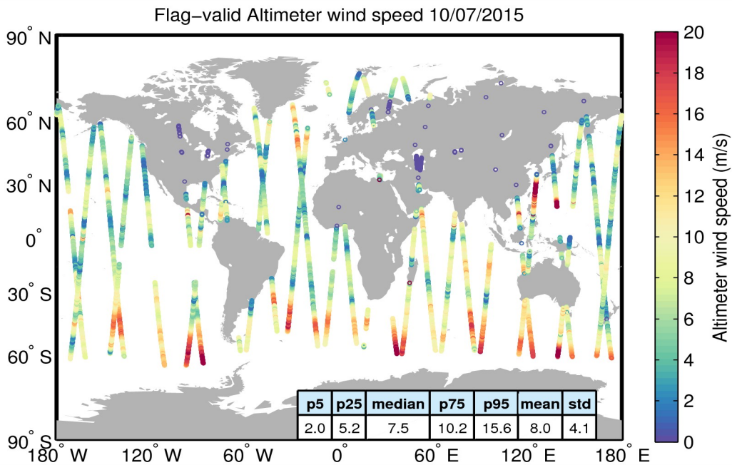
Figure 31. Geographical distribution of flag-valid wind data over oceans and lakes for 10/07/2015. The statistical values shown in the table refer to the wind in m/s and are calculated over all measurements shown in the figure.
