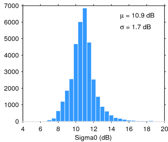
Figure 28. Histogram of science-valid sigma0 over oceans and lakes for 10/07/2015. The mean ( \mu ) and standard deviation ( \sigma ) are also shown. Note that values outside [4 20] dB are excluded from the histogram for the sake of readability but not from the computation of \mu and \sigma .
