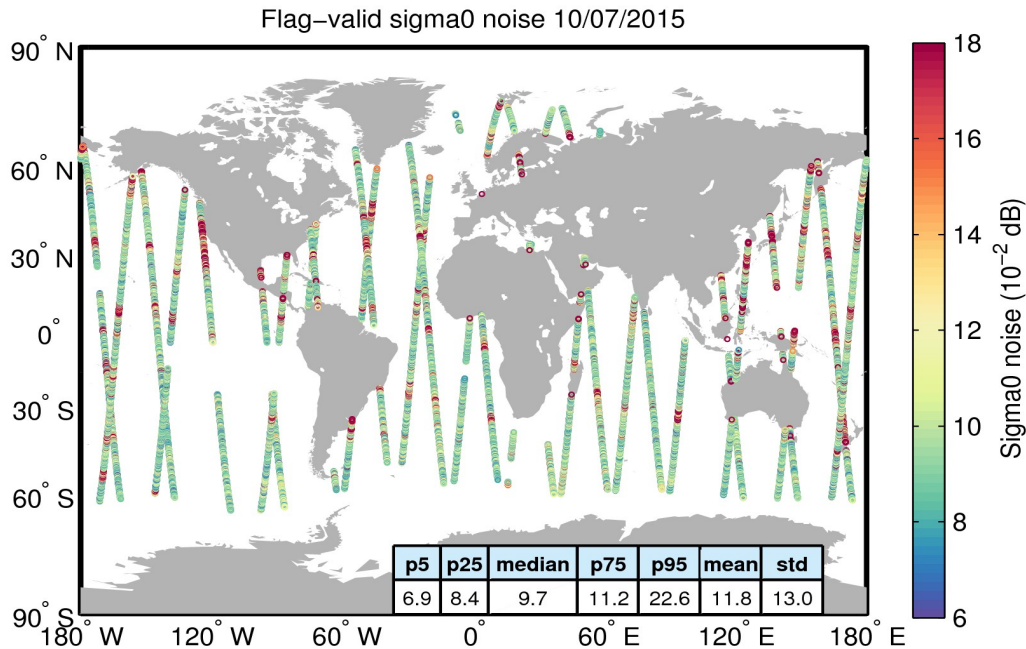
Figure 26. Geographical distribution of flag-valid 20-Hz sigma0 measurement noise over oceans and lakes for 10/07/2015. The statistical values shown in the table refer to the sigma0 noise and are calculated over all measurements shown in the figure.
