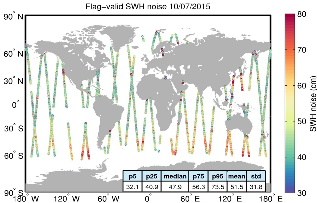
Figure 18. Geographical distribution of flag-valid 20-Hz SWH measurement noise over oceans and lakes for 10/07/2015. The statistical values shown in the figure refer to the SWH noise and are calculated over all measurements shown in the figure.
