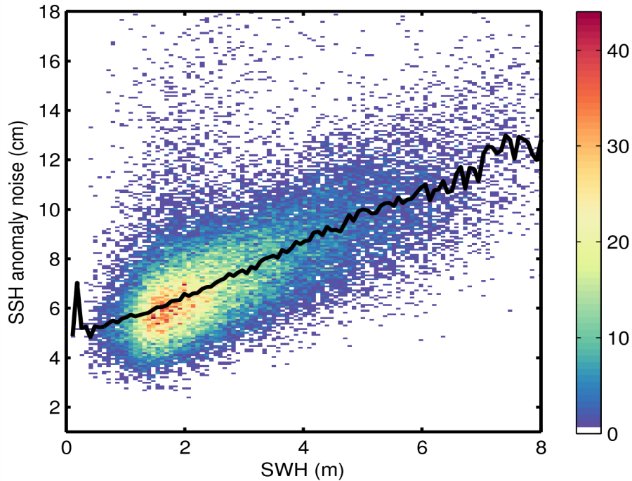
Figure 9. 2D histogram showing flag-valid SSH anomaly noise as a function of SWH for 10/07/2015. The black line denotes the median SSH anomaly as a function of SWH.
