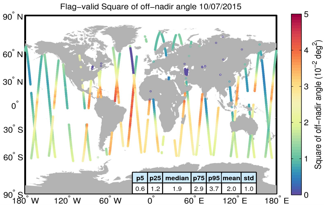
Figure 37. Geographical distribution of flag-valid mispointing data over oceans and lakes for 10/07/2015. The statistical values shown in the table refer to the mispointing in 10^{-2} \text{deg}^2 and are calculated over all measurements shown in the figure.
