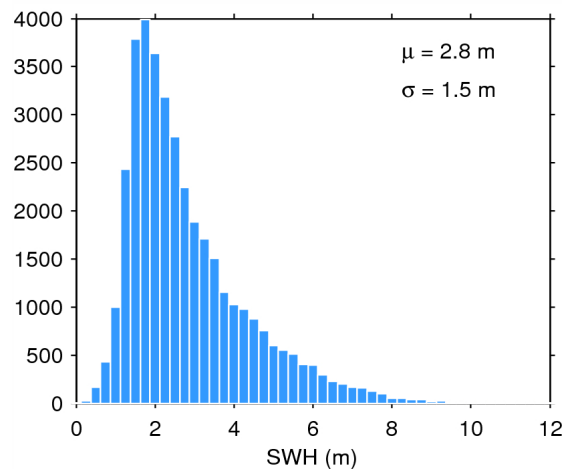
Figure 17. Histogram of flag-valid SWH over oceans and lakes for 10/07/2015. The mean ( \mu ) and standard deviation ( \sigma ) are also shown. Note that values larger than 12 m are excluded from the histogram for the sake of readability but not from the computation of \mu and \sigma .
