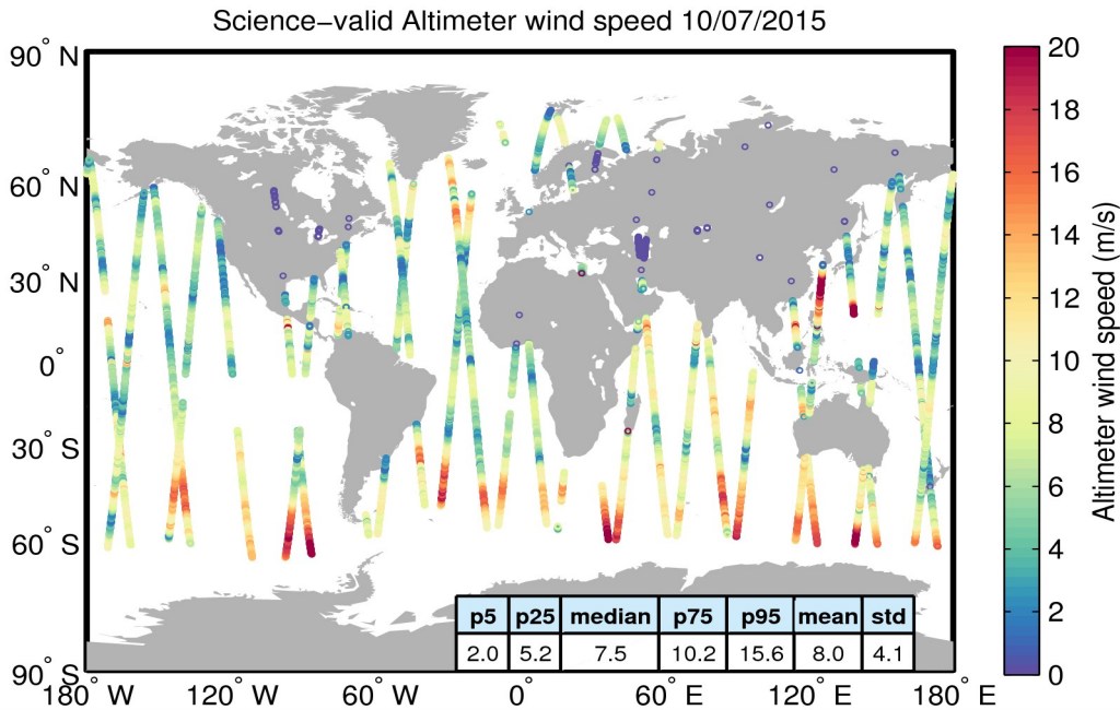
Figure 34. Geographical distribution of science-valid wind data over oceans and lakes for 10/07/2015. The statistical values shown in the table refer to the wind in m/s and are calculated over all measurements shown in the figure. Gray circles denote records that have been rejected based on the editing criteria described in Table 5.
