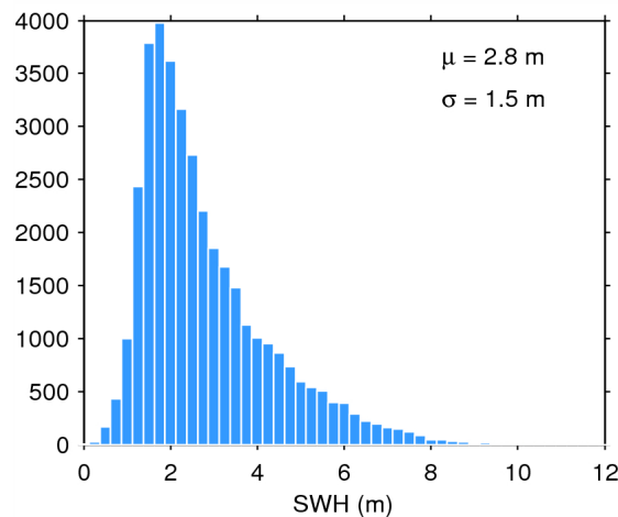
Figure 20. Histogram of science-valid SWH over oceans and lakes for 10/07/2015. The mean ( \mu ) and standard deviation ( \sigma ) are also shown. Note that values larger than 12 m are excluded from the histogram for the sake of readability but not from the computation of \mu and \sigma .
