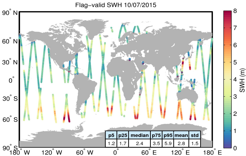
Figure 15. Geographical distribution of flag-valid SWH data over oceans and lakes for 10/07/2015. The statistical values shown in the table refer to the SWH in m and are calculated over all measurements shown in the figure.
