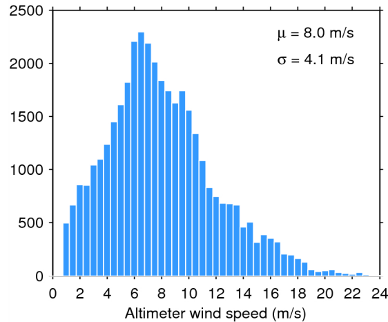
Figure 33. Histogram of flag-valid wind over oceans and lakes for 10/07/2015. The mean ( \mu ) and standard deviation ( \sigma ) are also shown. Note that values larger than 24 m/s are excluded from the histogram for the sake of readability but not from the computation of \mu and \sigma .
