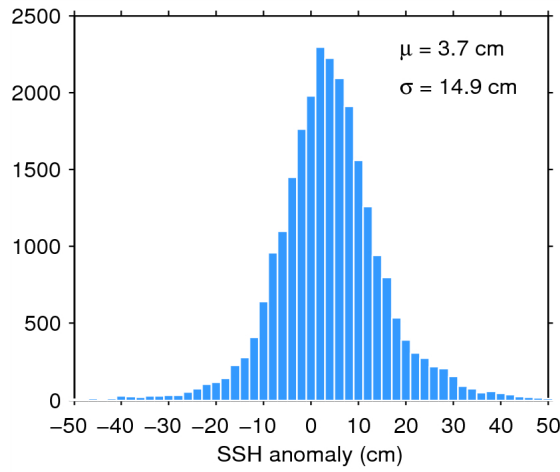
Figure 11. Histogram of science-valid SSH anomaly over oceans and lakes for 10/07/2015. The mean ( \mu ) and standard deviation ( \sigma ) are also shown. Note that values outside [-50 50] cm are excluded from the histogram for the sake of readability but not from the computation of \mu and \sigma .
