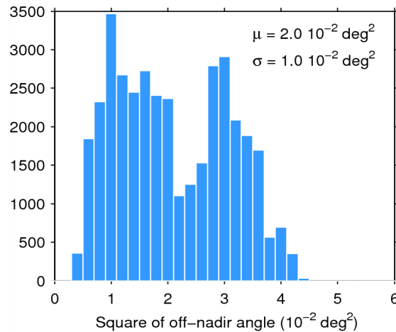
Figure 39. Histogram of flag-valid mispointing over oceans and lakes for 10/07/2015. The mean ( \mu ) and standard deviation ( \sigma ) are also shown. Note that values larger than 6 \cdot 10^{-2} \text{ deg}^2 are excluded from the histogram for the sake of readability but not from the computation of \mu and \sigma .
