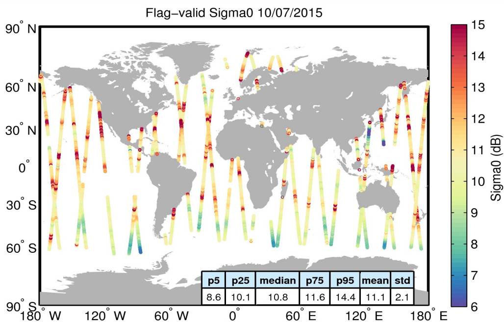
Figure 23. Geographical distribution of flag-valid sigma0 data over oceans and lakes for 10/07/2015. The statistical values shown in the table refer to the sigma0 in dB and are calculated over all measurements shown in the figure.
