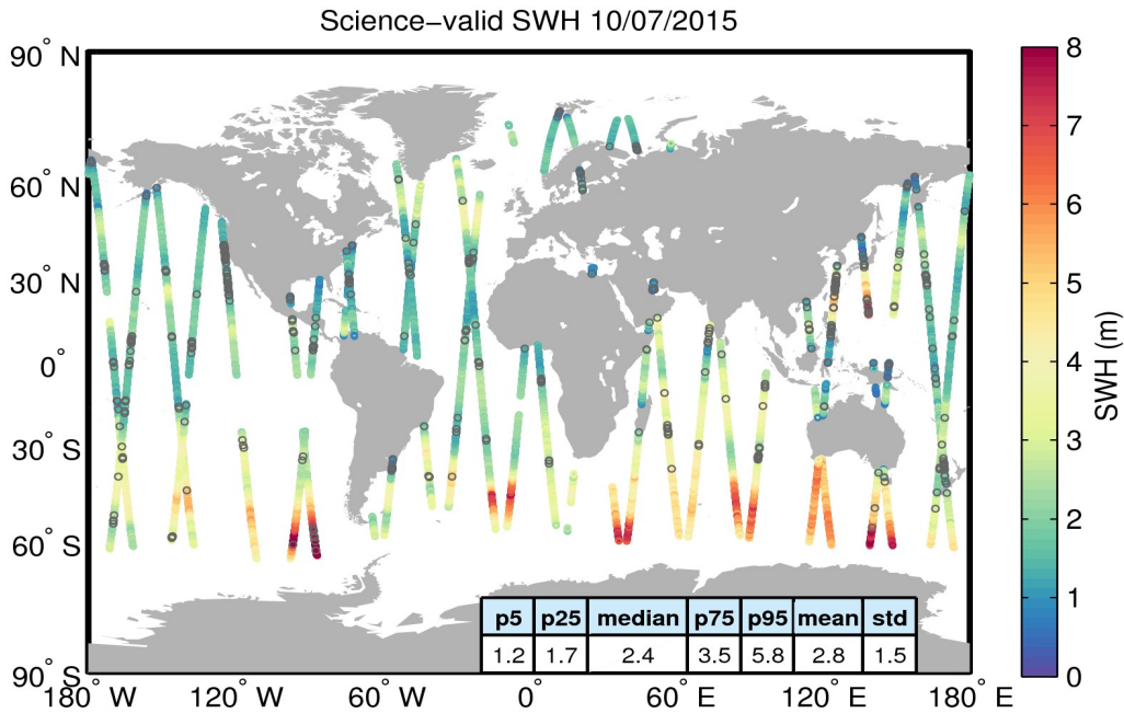
Figure 19. Geographical distribution of science-valid SWH data over oceans and lakes for 10/07/2015. The statistical values shown in the table refer to the SWH in m and are calculated over all measurements shown in the figure. Gray circles denote records that have been rejected based on the editing criteria described in Table 3.
