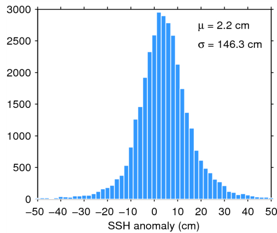
Figure 7. Histogram of flag-valid SSH anomaly over oceans and lakes for 10/07/2015. The mean ( \mu ) and standard deviation ( \sigma ) are also shown. Note that values outside [-50\ 50] cm are excluded from the histogram for the sake of readability but not from the computation of \mu and \sigma .
