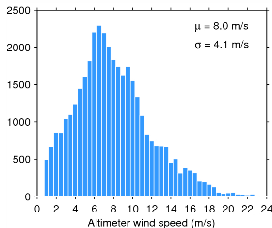
Figure 35. Histogram of science-valid wind over oceans and lakes for 10/07/2015. The mean ( \mu ) and standard deviation ( \sigma ) are also shown. Note that values larger than 24 m/s are excluded from the histogram for the sake of readability but not from the computation of \mu and \sigma .
