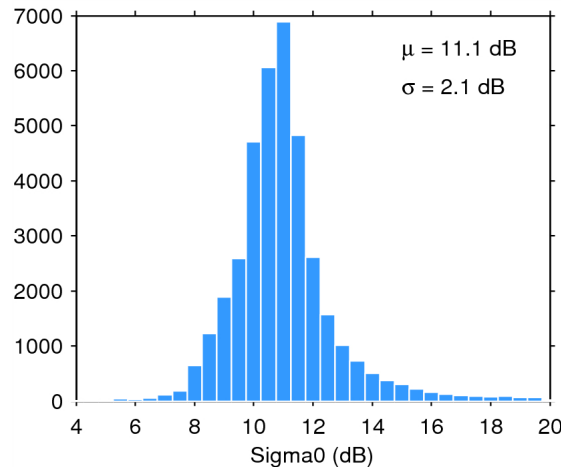
Figure 25. Histogram of flag-valid sigma0 over oceans and lakes for 10/07/2015. The mean ( \mu ) and standard deviation ( \sigma ) are also shown. Note that values outside [4 20] dB are excluded from the histogram for the sake of readability but not from the computation of \mu and \sigma .
