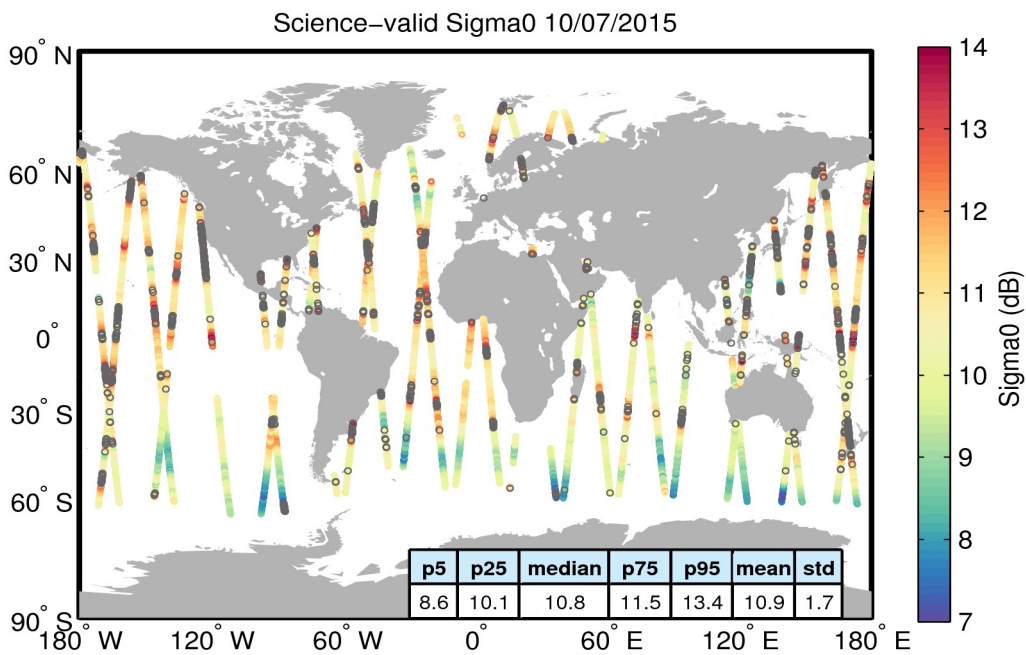
Figure 27. Geographical distribution of science-valid sigma0 data over oceans and lakes for 10/07/2015. The statistical values shown in the table refer to the sigma0 in dB and are calculated over all measurements shown in the figure. Gray circles denote records that have been rejected based on the editing criteria described in Table 4.
