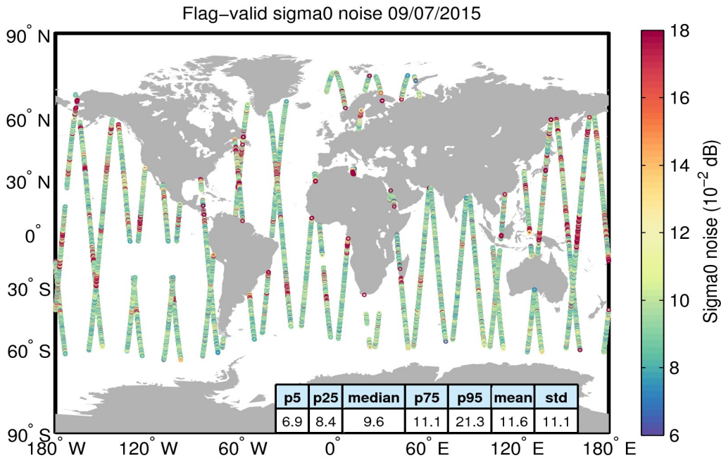
Figure 26. Geographical distribution of flag-valid 20-Hz sigma0 measurement noise over oceans and lakes for 09/07/2015. The statistical values shown in the table refer to the sigma0 noise and are calculated over all measurements shown in the figure.
