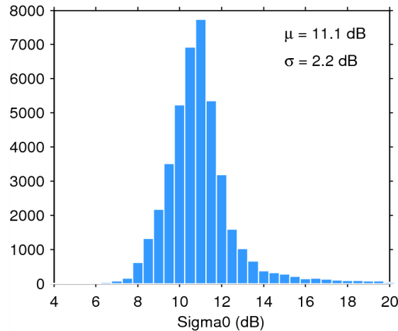
Figure 25. Histogram of flag-valid sigma0 over oceans and lakes for 09/07/2015. The mean ( \mu ) and standard deviation ( \sigma ) are also shown. Note that values outside [4 20] dB are excluded from the histogram for the sake of readability but not from the computation of \mu and \sigma .
