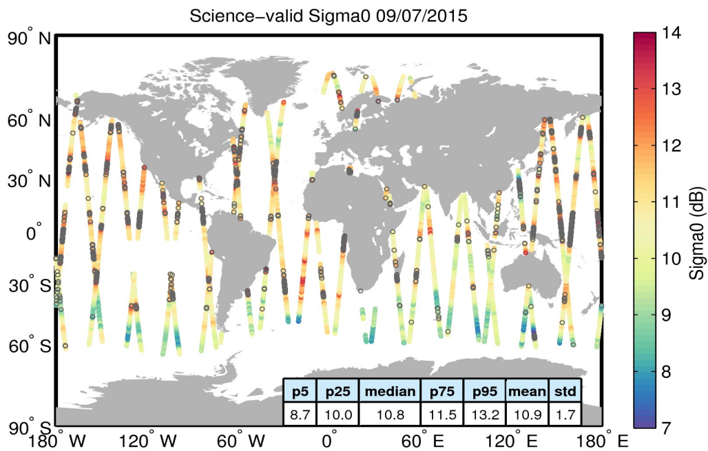
Figure 27. Geographical distribution of science-valid sigma0 data over oceans and lakes for 09/07/2015. The statistical values shown in the table refer to the sigma0 in dB and are calculated over all measurements shown in the figure. Gray circles denote records that have been rejected based on the editing criteria described in Table 4.
