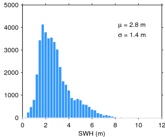
Figure 20. Histogram of science-valid SWH over oceans and lakes for 09/07/2015. The mean ( \mu ) and standard deviation ( \sigma ) are also shown. Note that values larger than 12 m are excluded from the histogram for the sake of readability but not from the computation of \mu and \sigma .
