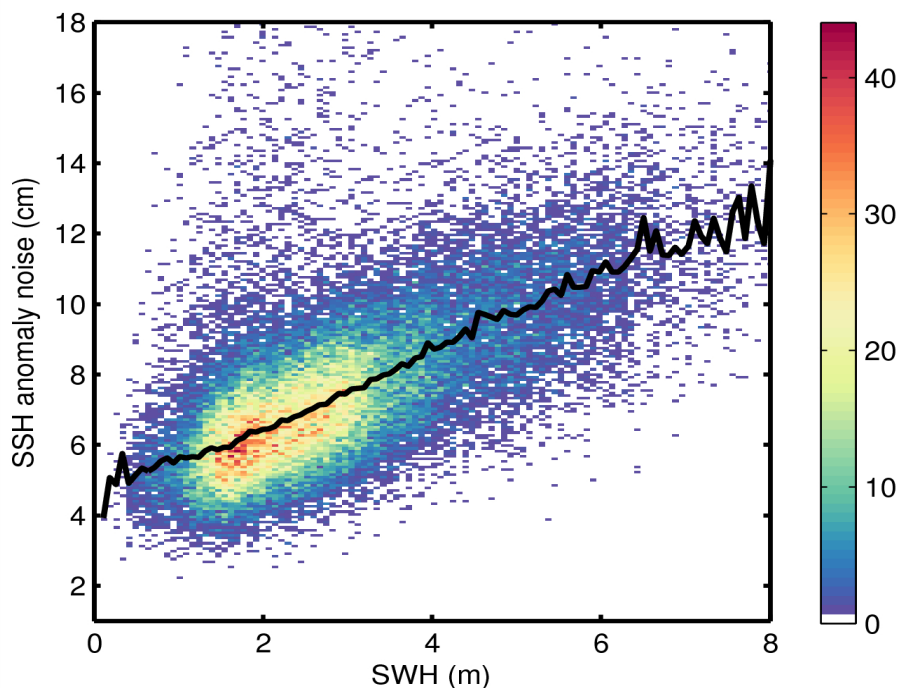
Figure 9. 2D histogram showing flag-valid SSH anomaly noise as a function of SWH for 09/07/2015. The black line denotes the median SSH anomaly as a function of SWH.
