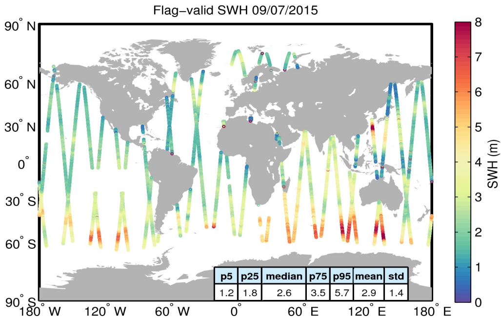
Figure 15. Geographical distribution of flag-valid SWH data over oceans and lakes for 09/07/2015. The statistical values shown in the table refer to the SWH in m and are calculated over all measurements shown in the figure.
