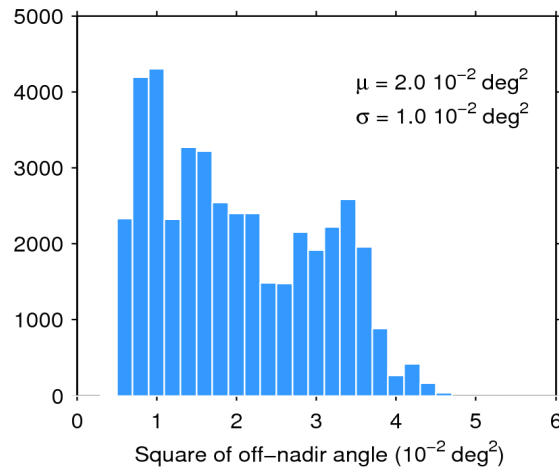
Figure 39. Histogram of flag-valid mispointing over oceans and lakes for 09/07/2015. The mean ( \mu ) and standard deviation ( \sigma ) are also shown. Note that values larger than 6 \cdot 10^{-2} \text{ deg}^2 are excluded from the histogram for the sake of readability but not from the computation of \mu and \sigma .
