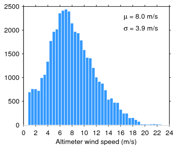
Figure 35. Histogram of science-valid wind over oceans and lakes for 09/07/2015. The mean ( \mu ) and standard deviation ( \sigma ) are also shown. Note that values larger than 24 m/s are excluded from the histogram for the sake of readability but not from the computation of \mu and \sigma .
