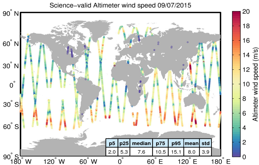
Figure 34. Geographical distribution of science-valid wind data over oceans and lakes for 09/07/2015. The statistical values shown in the table refer to the wind in m/s and are calculated over all measurements shown in the figure. Gray circles denote records that have been rejected based on the editing criteria described in Table 5.
