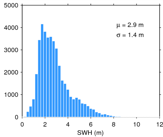
Figure 17. Histogram of flag-valid SWH over oceans and lakes for 09/07/2015. The mean ( \mu ) and standard deviation ( \sigma ) are also shown. Note that values larger than 12 m are excluded from the histogram for the sake of readability but not from the computation of \mu and \sigma .
