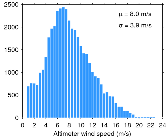
Figure 33. Histogram of flag-valid wind over oceans and lakes for 09/07/2015. The mean ( \mu ) and standard deviation ( \sigma ) are also shown. Note that values larger than 24 m/s are excluded from the histogram for the sake of readability but not from the computation of \mu and \sigma .
