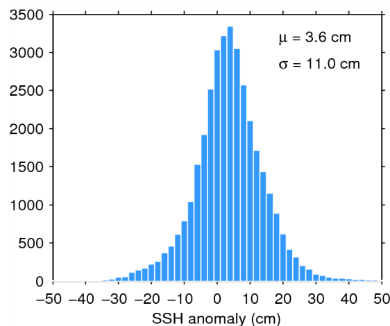
Figure 11. Histogram of science-valid SSH anomaly over oceans and lakes for 09/07/2015. The mean ( \mu ) and standard deviation ( \sigma ) are also shown. Note that values outside [-50 50] cm are excluded from the histogram for the sake of readability but not from the computation of \mu and \sigma .
