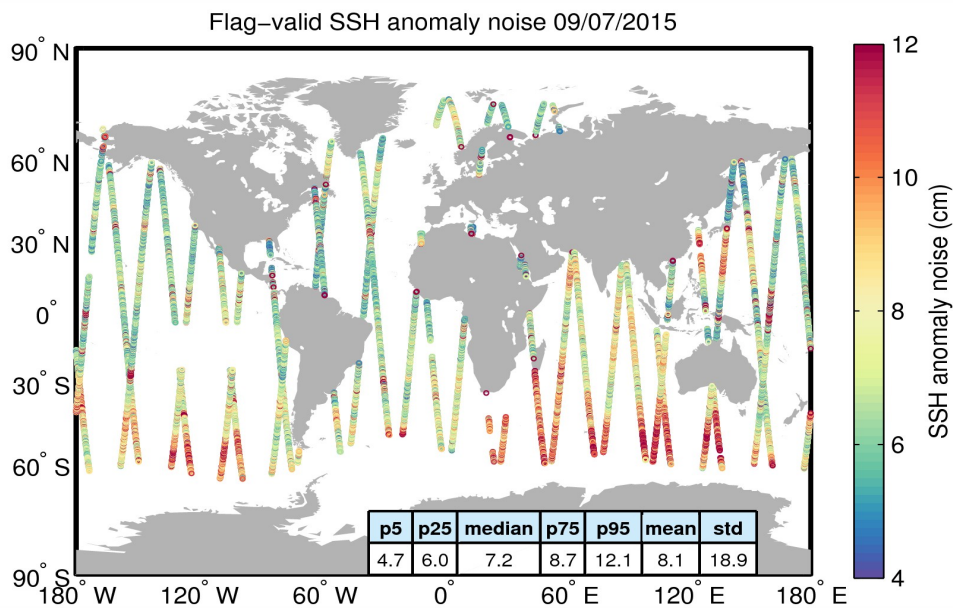
Figure 8. Geographical distribution of flag-valid 20-Hz SSH anomaly measurement noise over oceans and lakes for 09/07/2015. The statistical values shown in the table refer to the SSH anomaly noise and are calculated over all measurements shown in the figure.
