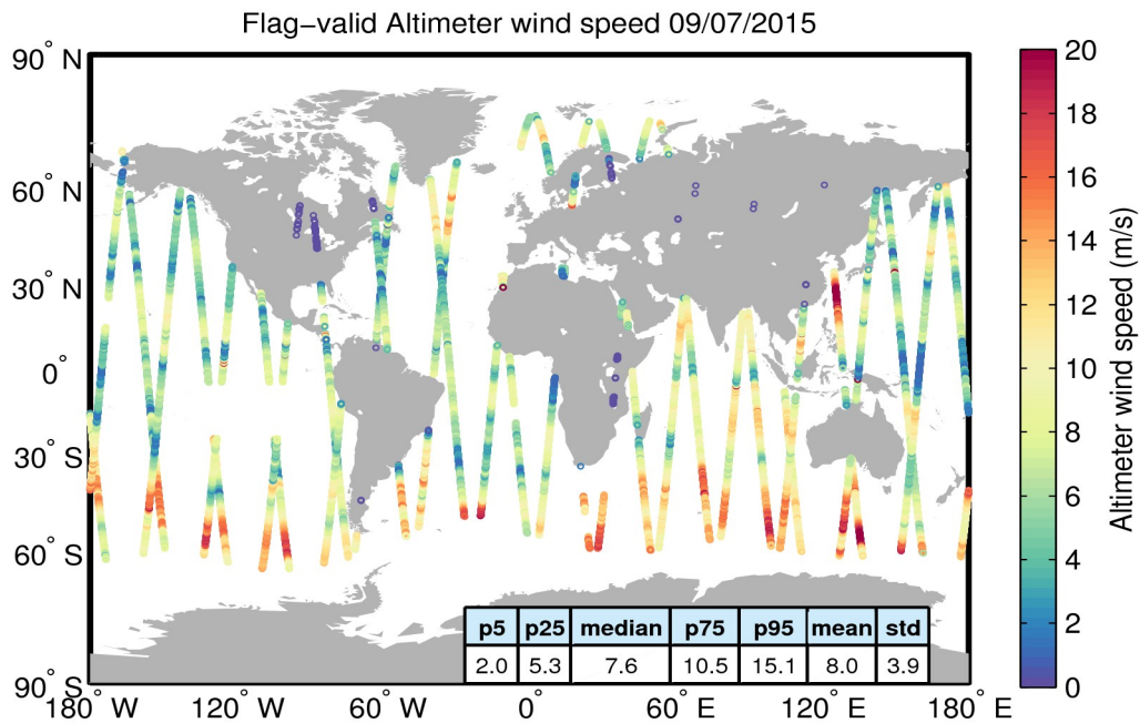
Figure 31. Geographical distribution of flag-valid wind data over oceans and lakes for 09/07/2015. The statistical values shown in the table refer to the wind in m/s and are calculated over all measurements shown in the figure.
