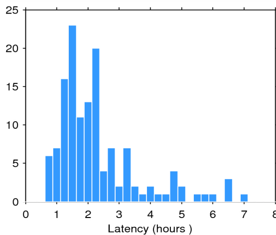
Figure 2. Histogram of the data latency for 09/07/2015. The y-axis denotes the number of files that are made available with a delay of x-hours with respect to the mean time of the records stored in the file.
