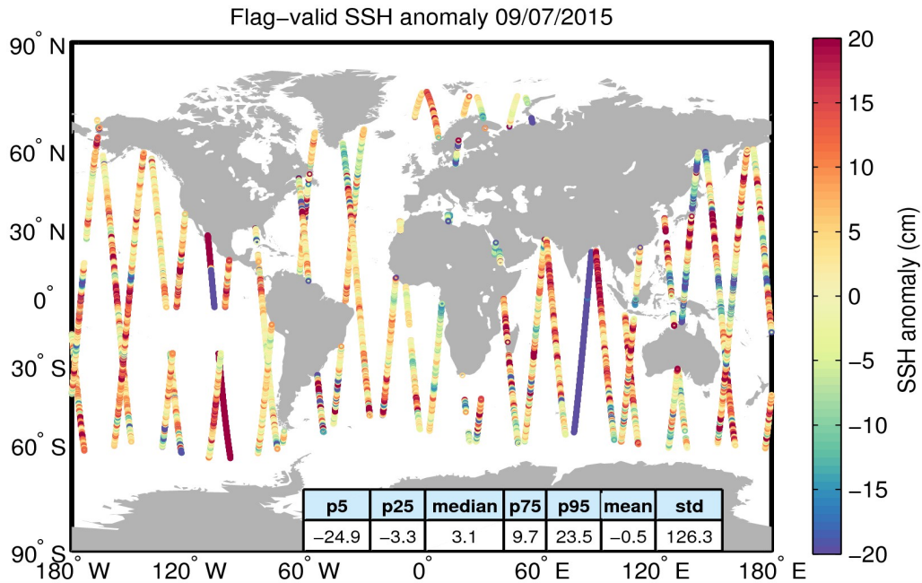
Figure 5. Geographical distribution of flag-valid 1-Hz SSH anomaly data over oceans and lakes for 09/07/2015. The statistical values shown in the table refer to the SSH anomaly in cm and are calculated over all measurements shown in the figure.
