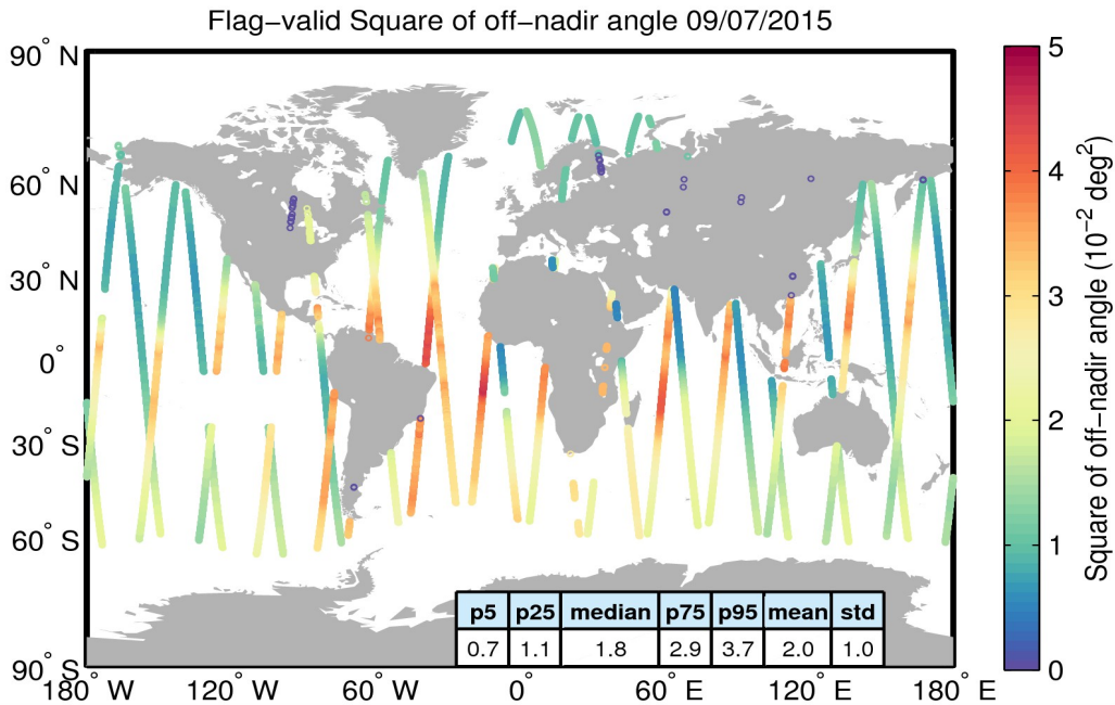
Figure 37. Geographical distribution of flag-valid mispointing data over oceans and lakes for 09/07/2015. The statistical values shown in the table refer to the mispointing in 10^{-2} \text{deg}^2 and are calculated over all measurements shown in the figure.
