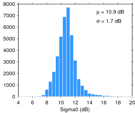
Figure 28. Histogram of science-valid sigma0 over oceans and lakes for 09/07/2015. The mean ( \mu ) and standard deviation ( \sigma ) are also shown. Note that values outside [4 20] dB are excluded from the histogram for the sake of readability but not from the computation of \mu and \sigma .
