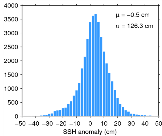
Figure 7. Histogram of flag-valid SSH anomaly over oceans and lakes for 09/07/2015. The mean ( \mu ) and standard deviation ( \sigma ) are also shown. Note that values outside [-50 50] cm are excluded from the histogram for the sake of readability but not from the computation of \mu and \sigma .
