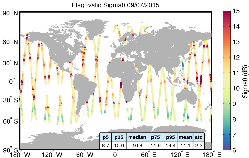
Figure 23. Geographical distribution of flag-valid sigma0 data over oceans and lakes for 09/07/2015. The statistical values shown in the table refer to the sigma0 in dB and are calculated over all measurements shown in the figure.
