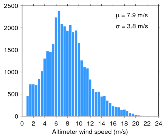
Figure 35. Histogram of science-valid wind over oceans and lakes for 08/07/2015. The mean ( \mu ) and standard deviation ( \sigma ) are also shown. Note that values larger than 24 m/s are excluded from the histogram for the sake of readability but not from the computation of \mu and \sigma .
