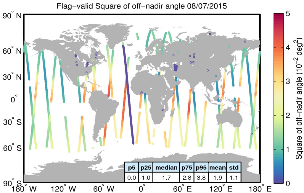
Figure 37. Geographical distribution of flag-valid mispointing data over oceans and lakes for 08/07/2015. The statistical values shown in the table refer to the mispointing in 10^{-2} deg 2 and are calculated over all measurements shown in the figure.
