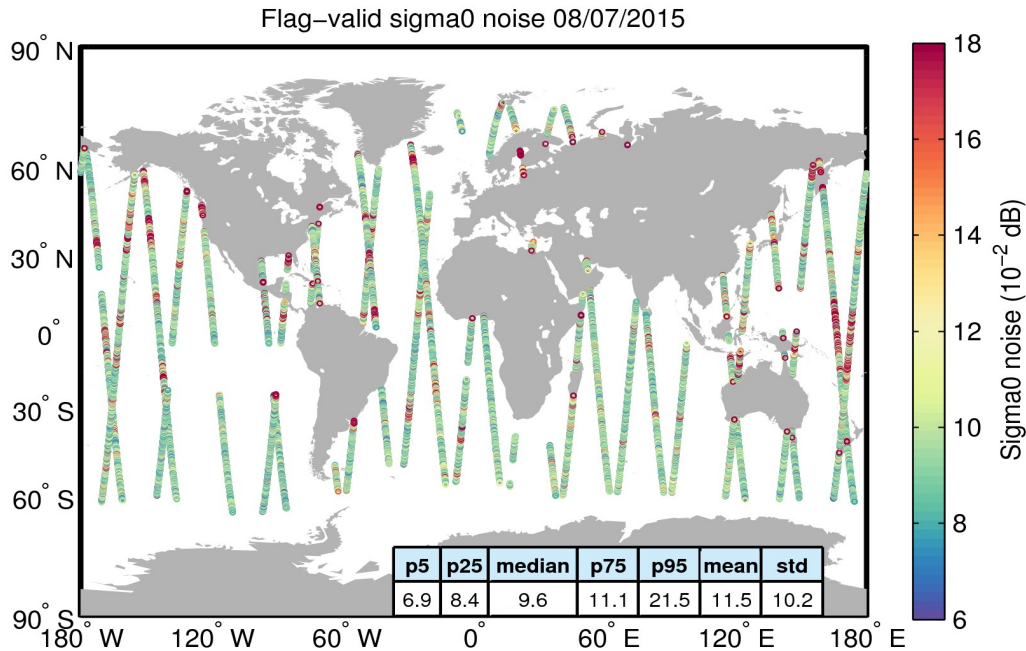
Figure 26. Geographical distribution of flag-valid 20-Hz sigma0 measurement noise over oceans and lakes for 08/07/2015. The statistical values shown in the table refer to the sigma0 noise and are calculated over all measurements shown in the figure.
