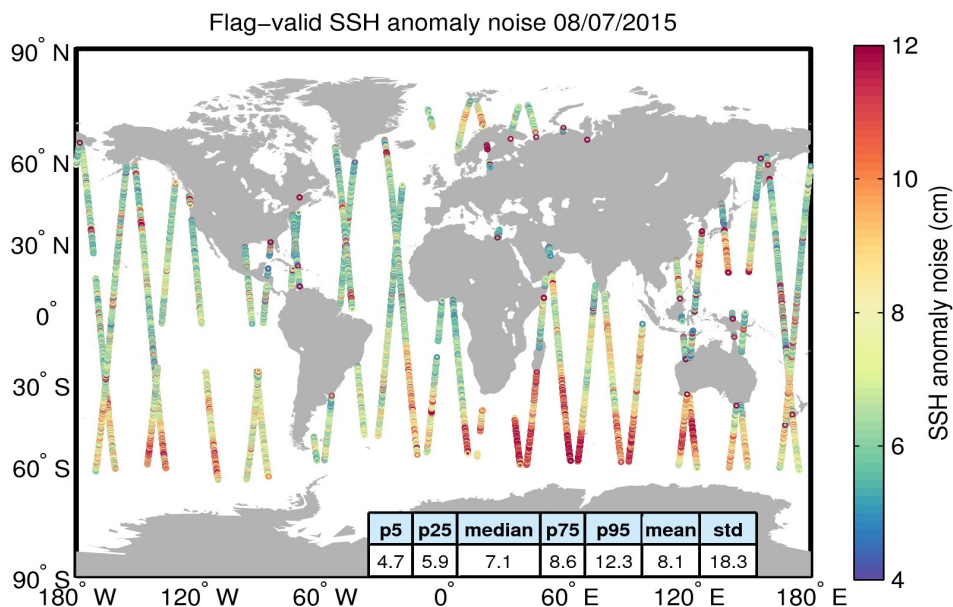
Figure 8. Geographical distribution of flag-valid 20-Hz SSH anomaly measurement noise over oceans and lakes for 08/07/2015. The statistical values shown in the table refer to the SSH anomaly noise and are calculated over all measurements shown in the figure.
