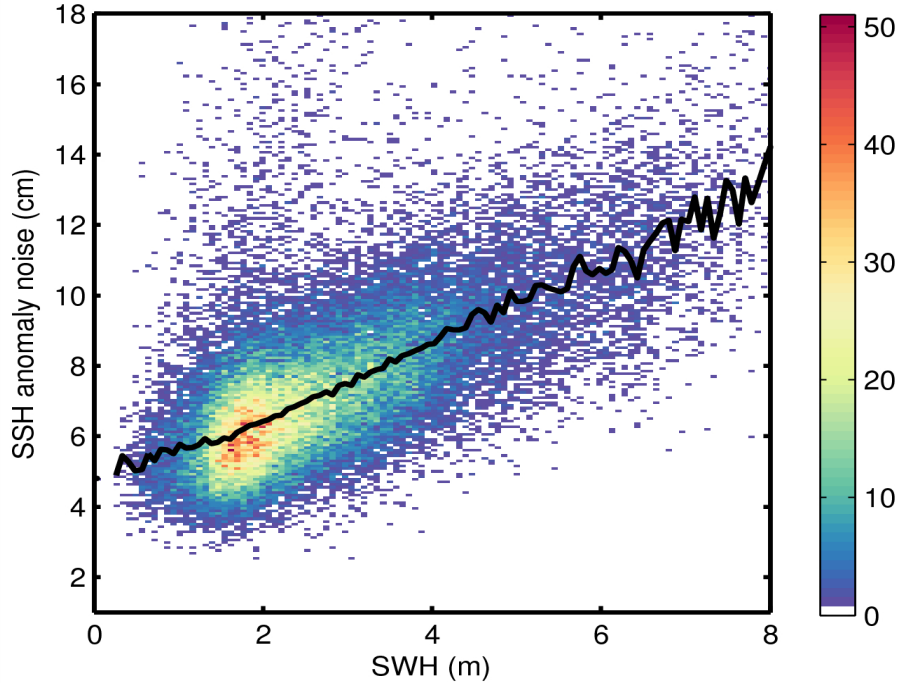
Figure 9. 2D histogram showing flag-valid SSH anomaly noise as a function of SWH for 08/07/2015. The black line denotes the median SSH anomaly as a function of SWH.
