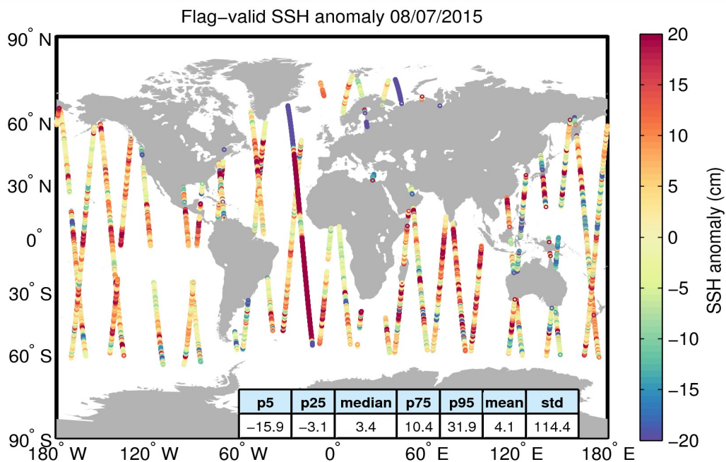
Figure 5. Geographical distribution of flag-valid 1-Hz SSH anomaly data over oceans and lakes for 08/07/2015. The statistical values shown in the table refer to the SSH anomaly in cm and are calculated over all measurements shown in the figure.
