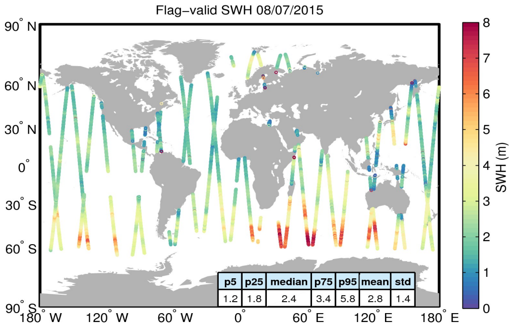
Figure 15. Geographical distribution of flag-valid SWH data over oceans and lakes for 08/07/2015. The statistical values shown in the table refer to the SWH in m and are calculated over all measurements shown in the figure.
