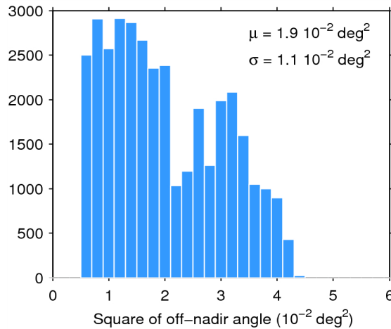
Figure 39. Histogram of flag-valid mispointing over oceans and lakes for 08/07/2015. The mean ( \mu ) and standard deviation ( \sigma ) are also shown. Note that values larger than 6 \cdot 10^{-2} \text{ deg}^2 are excluded from the histogram for the sake of readability but not from the computation of \mu and \sigma .
