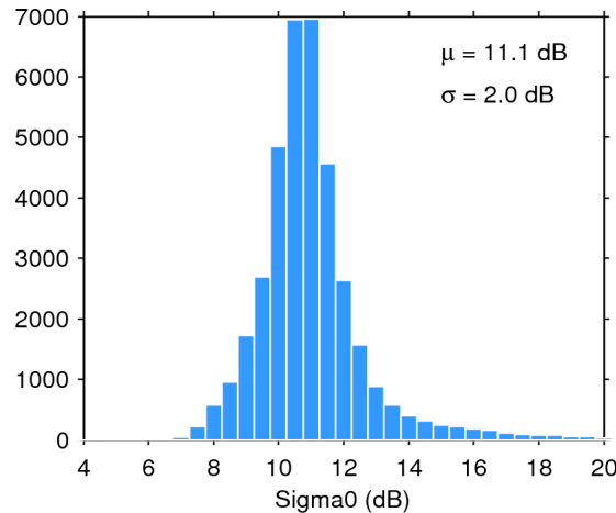
Figure 25. Histogram of flag-valid sigma0 over oceans and lakes for 08/07/2015. The mean ( \mu ) and standard deviation ( \sigma ) are also shown. Note that values outside [4 20] dB are excluded from the histogram for the sake of readability but not from the computation of \mu and \sigma .
