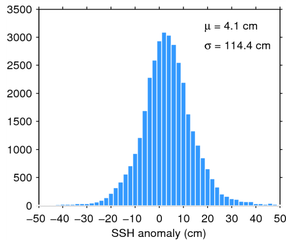
Figure 7. Histogram of flag-valid SSH anomaly over oceans and lakes for 08/07/2015. The mean ( \mu ) and standard deviation ( \sigma ) are also shown. Note that values outside [-50\ 50] cm are excluded from the histogram for the sake of readability but not from the computation of \mu and \sigma .
