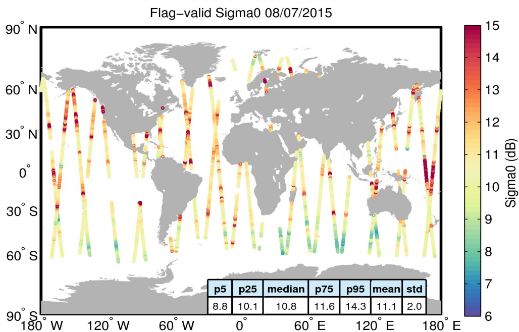
Figure 23. Geographical distribution of flag-valid sigma0 data over oceans and lakes for 08/07/2015. The statistical values shown in the table refer to the sigma0 in dB and are calculated over all measurements shown in the figure.
