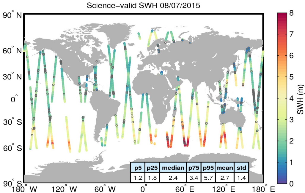
Figure 19. Geographical distribution of science-valid SWH data over oceans and lakes for 08/07/2015. The statistical values shown in the table refer to the SWH in m and are calculated over all measurements shown in the figure. Gray circles denote records that have been rejected based on the editing criteria described in Table 3.
