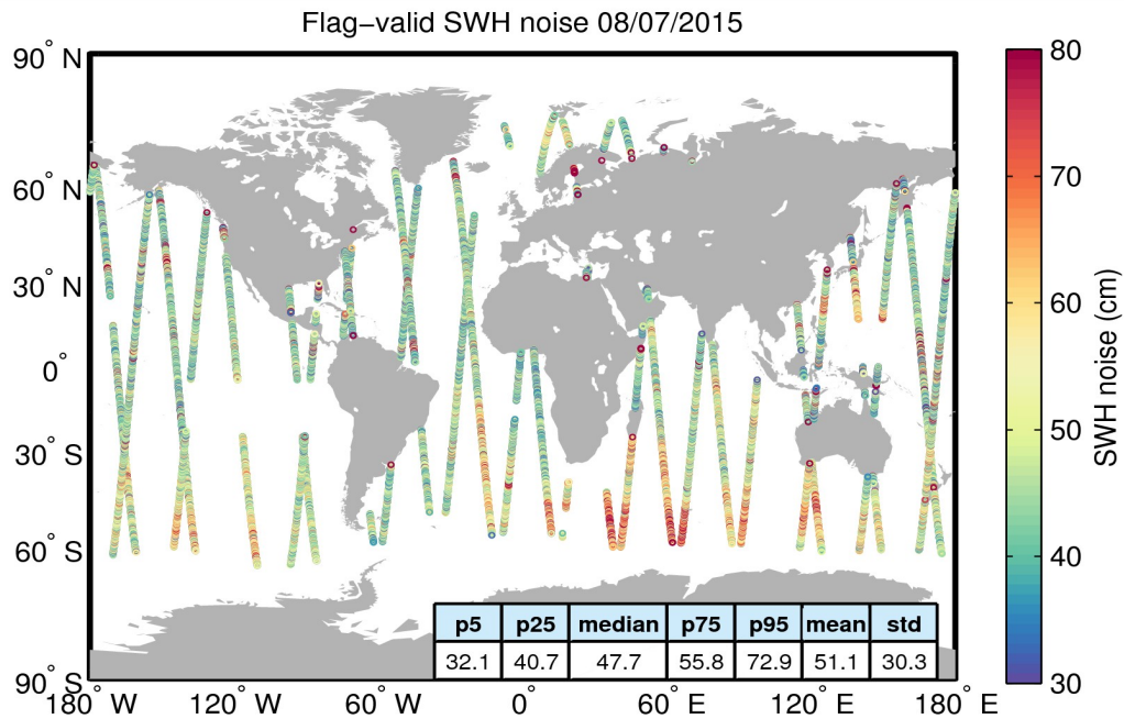
Figure 18. Geographical distribution of flag-valid 20-Hz SWH measurement noise over oceans and lakes for 08/07/2015. The statistical values shown in the figure refer to the SWH noise and are calculated over all measurements shown in the figure.
