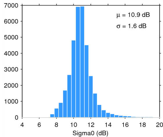
Figure 28. Histogram of science-valid sigma0 over oceans and lakes for 08/07/2015. The mean ( \mu ) and standard deviation ( \sigma ) are also shown. Note that values outside [4 20] dB are excluded from the histogram for the sake of readability but not from the computation of \mu and \sigma .
