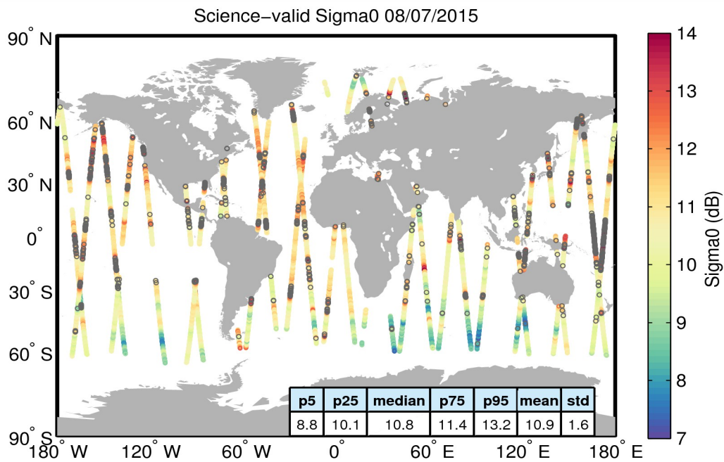
Figure 27. Geographical distribution of science-valid sigma0 data over oceans and lakes for 08/07/2015. The statistical values shown in the table refer to the sigma0 in dB and are calculated over all measurements shown in the figure. Gray circles denote records that have been rejected based on the editing criteria described in Table 4.
