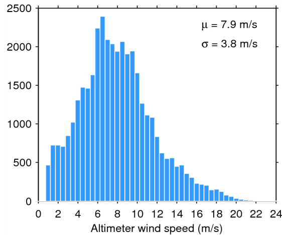
Figure 33. Histogram of flag-valid wind over oceans and lakes for 08/07/2015. The mean ( \mu ) and standard deviation ( \sigma ) are also shown. Note that values larger than 24 m/s are excluded from the histogram for the sake of readability but not from the computation of \mu and \sigma .
