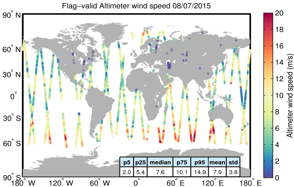
Figure 31. Geographical distribution of flag-valid wind data over oceans and lakes for 08/07/2015. The statistical values shown in the table refer to the wind in m/s and are calculated over all measurements shown in the figure.
