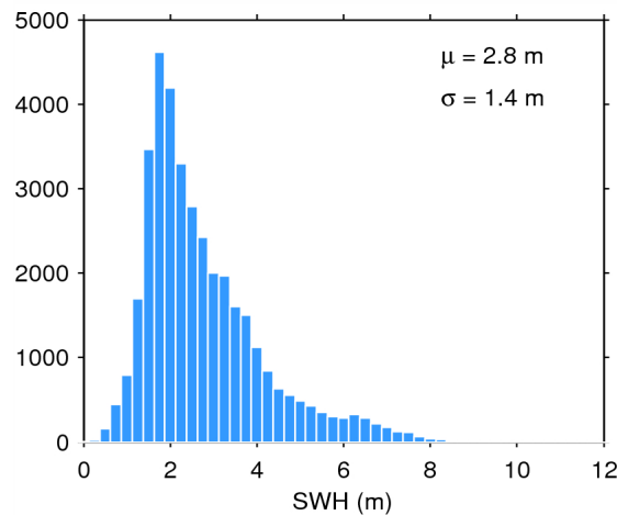
Figure 17. Histogram of flag-valid SWH over oceans and lakes for 08/07/2015. The mean ( \mu ) and standard deviation ( \sigma ) are also shown. Note that values larger than 12 m are excluded from the histogram for the sake of readability but not from the computation of \mu and \sigma .
