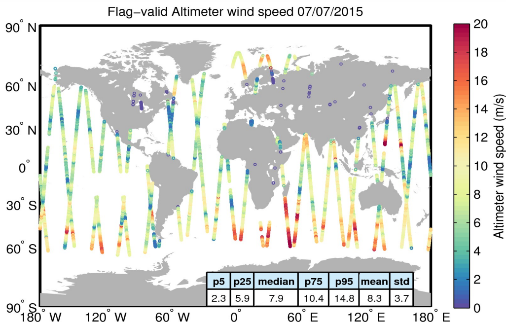
Figure 31. Geographical distribution of flag-valid wind data over oceans and lakes for 07/07/2015. The statistical values shown in the table refer to the wind in m/s and are calculated over all measurements shown in the figure.
