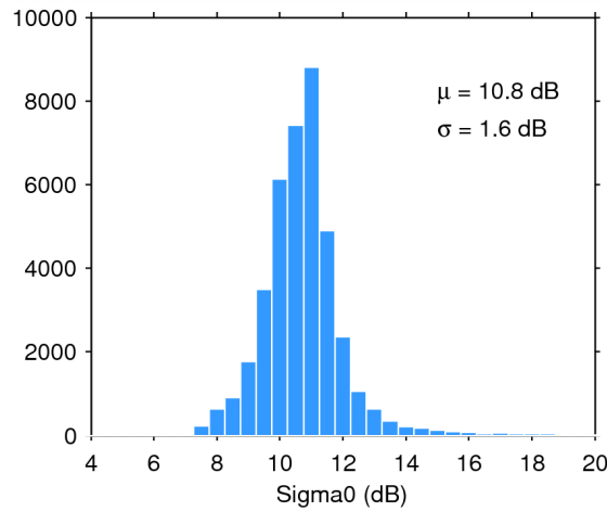
Figure 28. Histogram of science-valid sigma0 over oceans and lakes for 07/07/2015. The mean ( \mu ) and standard deviation ( \sigma ) are also shown. Note that values outside [4 20] dB are excluded from the histogram for the sake of readability but not from the computation of \mu and \sigma .
