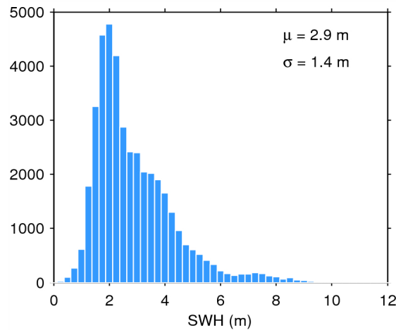
Figure 17. Histogram of flag-valid SWH over oceans and lakes for 07/07/2015. The mean ( \mu ) and standard deviation ( \sigma ) are also shown. Note that values larger than 12 m are excluded from the histogram for the sake of readability but not from the computation of \mu and \sigma .
