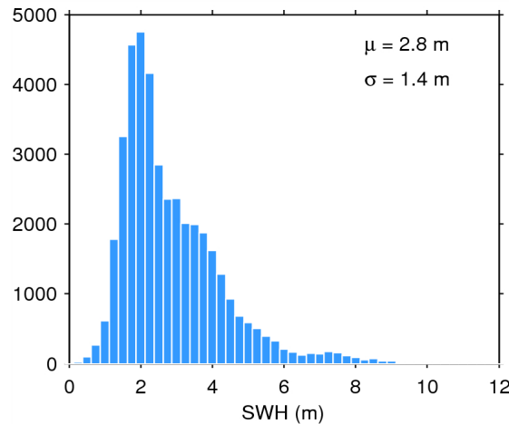
Figure 20. Histogram of science-valid SWH over oceans and lakes for 07/07/2015. The mean ( \mu ) and standard deviation ( \sigma ) are also shown. Note that values larger than 12 m are excluded from the histogram for the sake of readability but not from the computation of \mu and \sigma .
