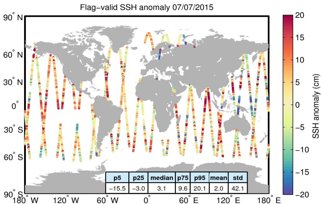
Figure 5. Geographical distribution of flag-valid 1-Hz SSH anomaly data over oceans and lakes for 07/07/2015. The statistical values shown in the table refer to the SSH anomaly in cm and are calculated over all measurements shown in the figure.
