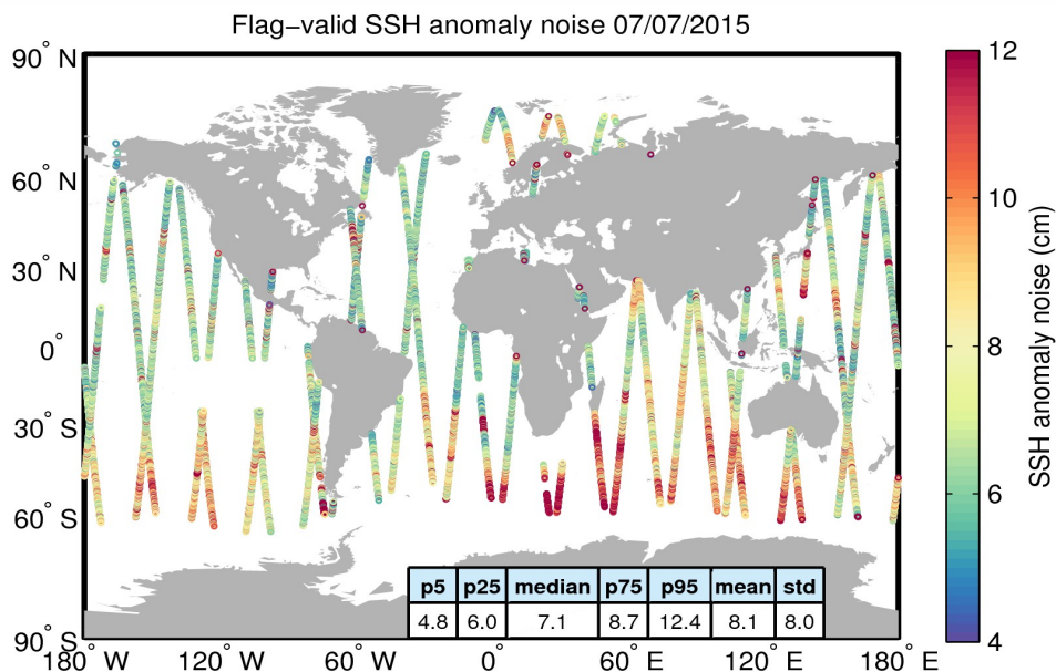
Figure 8. Geographical distribution of flag-valid 20-Hz SSH anomaly measurement noise over oceans and lakes for 07/07/2015. The statistical values shown in the table refer to the SSH anomaly noise and are calculated over all measurements shown in the figure.
