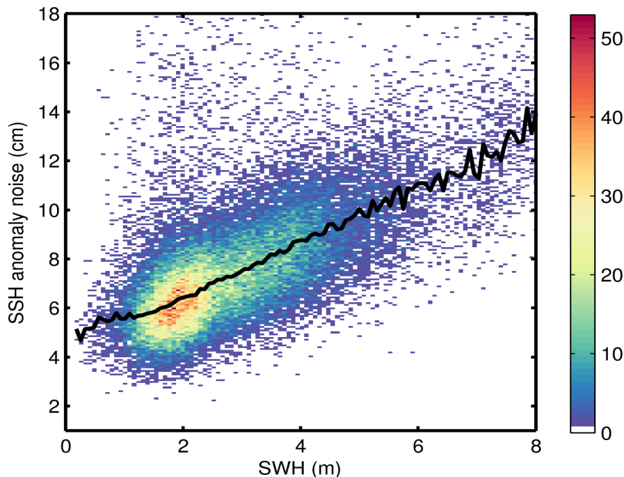
Figure 9. 2D histogram showing flag-valid SSH anomaly noise as a function of SWH for 07/07/2015. The black line denotes the median SSH anomaly as a function of SWH.
