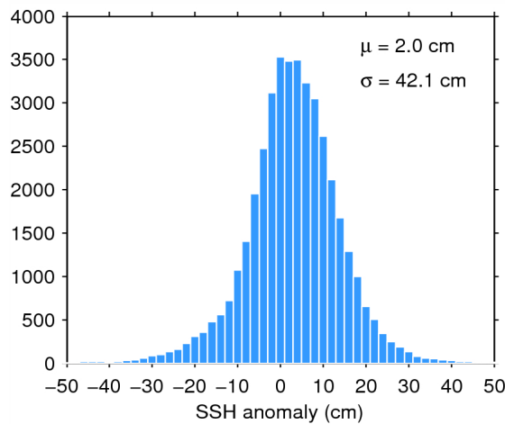
Figure 7. Histogram of flag-valid SSH anomaly over oceans and lakes for 07/07/2015. The mean ( \mu ) and standard deviation ( \sigma ) are also shown. Note that values outside [-50 50] cm are excluded from the histogram for the sake of readability but not from the computation of \mu and \sigma .
