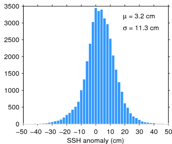
Figure 11. Histogram of science-valid SSH anomaly over oceans and lakes for 07/07/2015. The mean ( \mu ) and standard deviation ( \sigma ) are also shown. Note that values outside [-50 50] cm are excluded from the histogram for the sake of readability but not from the computation of \mu and \sigma .
