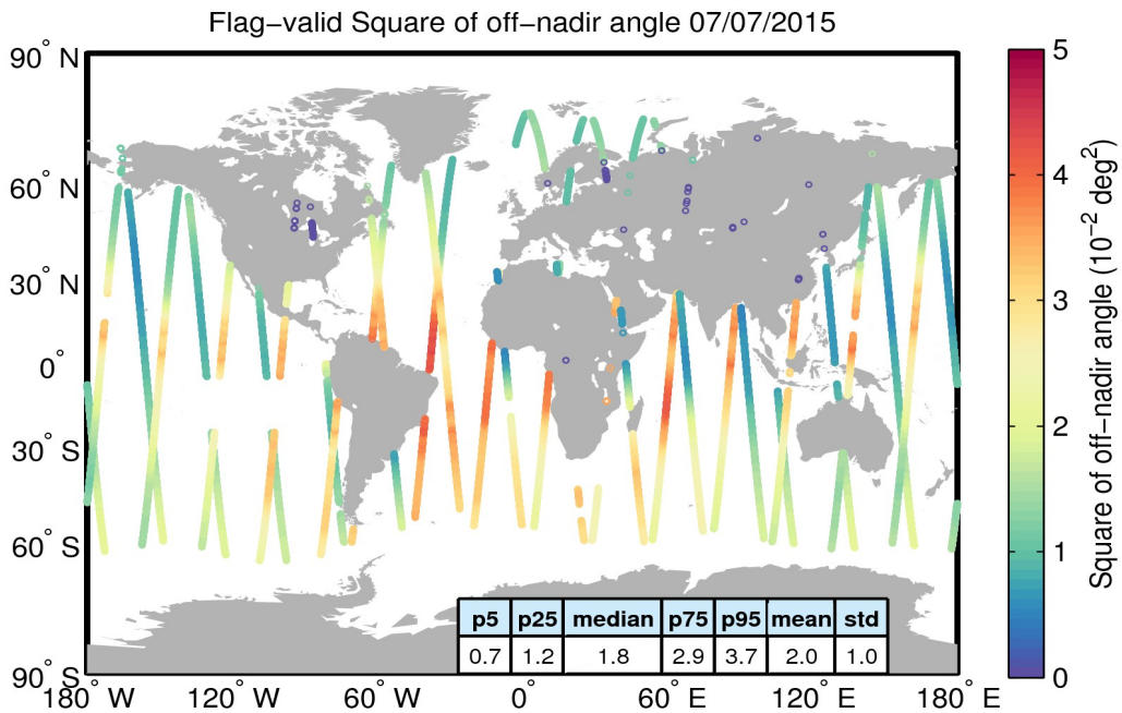
Figure 37. Geographical distribution of flag-valid mispointing data over oceans and lakes for 07/07/2015. The statistical values shown in the table refer to the mispointing in 10^{-2} \text{ deg}^2 and are calculated over all measurements shown in the figure.
