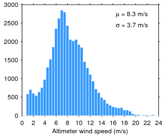
Figure 33. Histogram of flag-valid wind over oceans and lakes for 07/07/2015. The mean ( \mu ) and standard deviation ( \sigma ) are also shown. Note that values larger than 24 m/s are excluded from the histogram for the sake of readability but not from the computation of \mu and \sigma .
