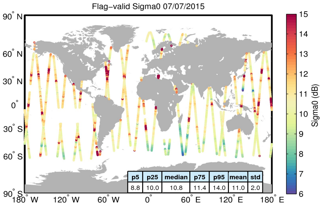
Figure 23. Geographical distribution of flag-valid sigma0 data over oceans and lakes for 07/07/2015. The statistical values shown in the table refer to the sigma0 in dB and are calculated over all measurements shown in the figure.
