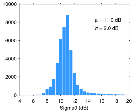
Figure 25. Histogram of flag-valid sigma0 over oceans and lakes for 07/07/2015. The mean ( \mu ) and standard deviation ( \sigma ) are also shown. Note that values outside [4 20] dB are excluded from the histogram for the sake of readability but not from the computation of \mu and \sigma .
