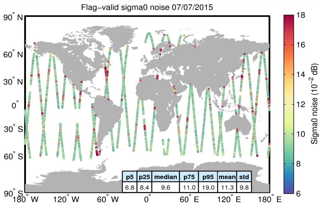
Figure 26. Geographical distribution of flag-valid 20-Hz sigma0 measurement noise over oceans and lakes for 07/07/2015. The statistical values shown in the table refer to the sigma0 noise and are calculated over all measurements shown in the figure.
