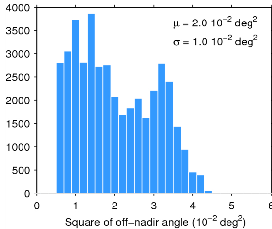
Figure 39. Histogram of flag-valid mispointing over oceans and lakes for 07/07/2015. The mean ( \mu ) and standard deviation ( \sigma ) are also shown. Note that values larger than 6 \cdot 10^{-2} \text{ deg}^2 are excluded from the histogram for the sake of readability but not from the computation of \mu and \sigma .
