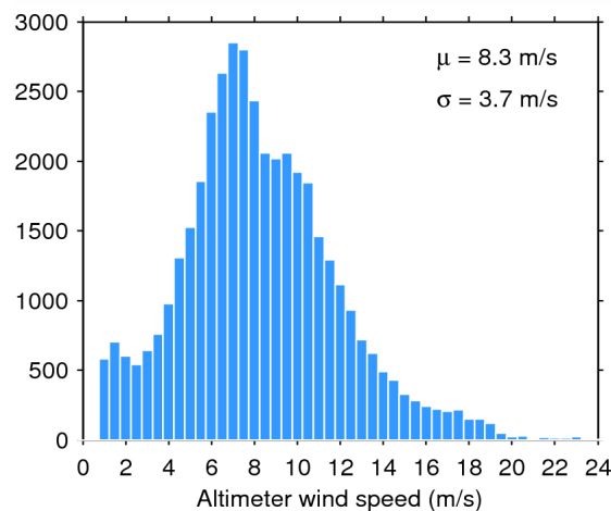
Figure 35. Histogram of science-valid wind over oceans and lakes for 07/07/2015. The mean ( \mu ) and standard deviation ( \sigma ) are also shown. Note that values larger than 24 m/s are excluded from the histogram for the sake of readability but not from the computation of \mu and \sigma .
