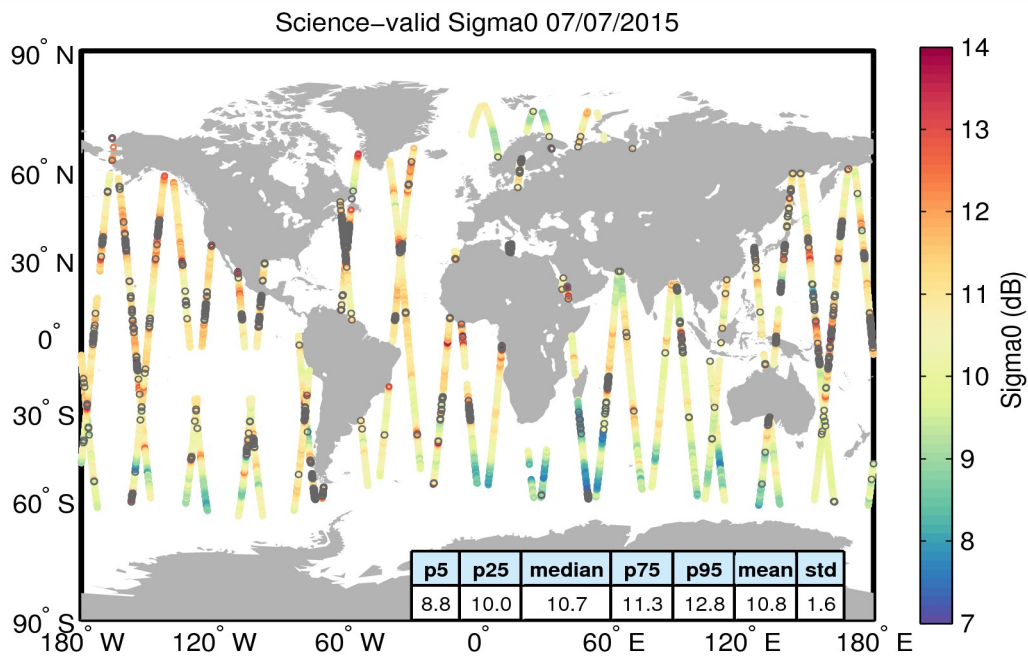
Figure 27. Geographical distribution of science-valid sigma0 data over oceans and lakes for 07/07/2015. The statistical values shown in the table refer to the sigma0 in dB and are calculated over all measurements shown in the figure. Gray circles denote records that have been rejected based on the editing criteria described in Table 4.
