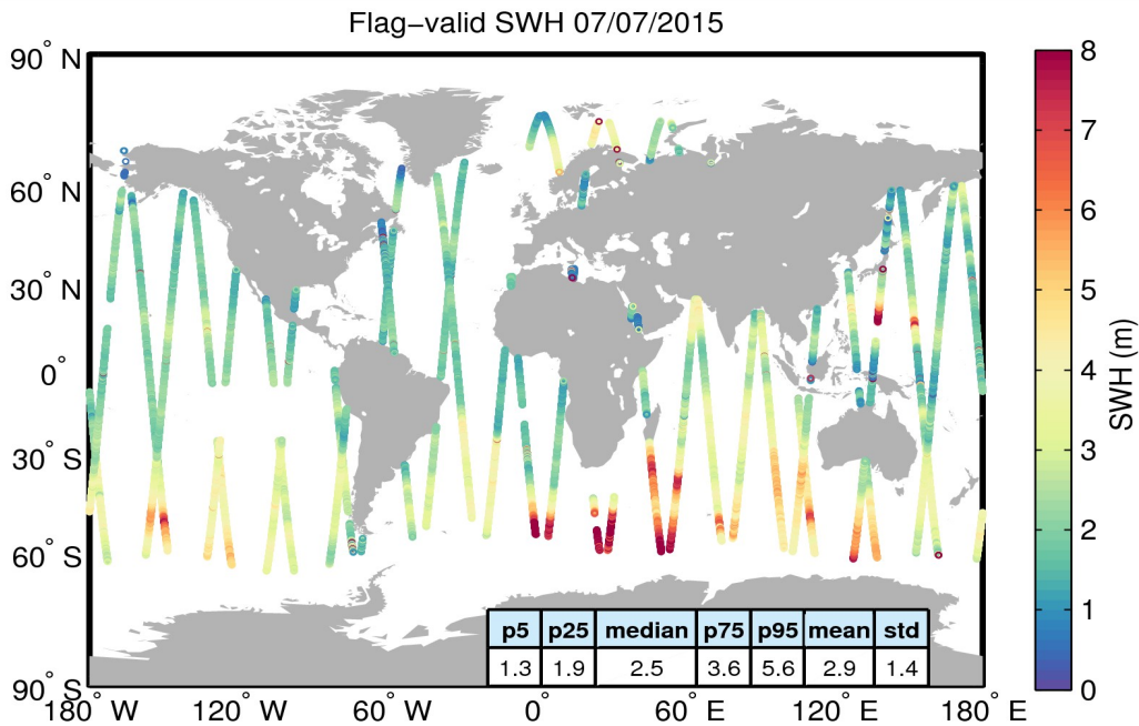
Figure 15. Geographical distribution of flag-valid SWH data over oceans and lakes for 07/07/2015. The statistical values shown in the table refer to the SWH in m and are calculated over all measurements shown in the figure.
