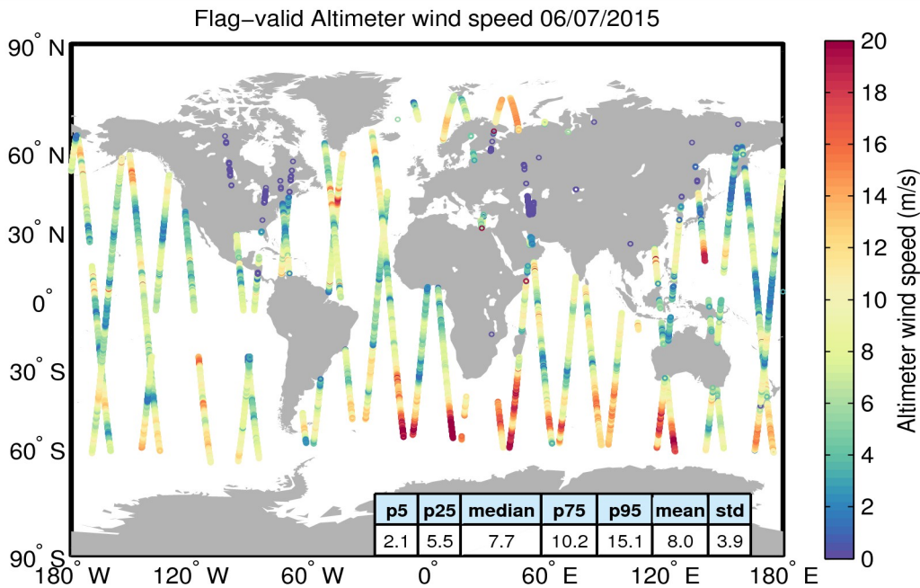
Figure 31. Geographical distribution of flag-valid wind data over oceans and lakes for 06/07/2015. The statistical values shown in the table refer to the wind in m/s and are calculated over all measurements shown in the figure.
