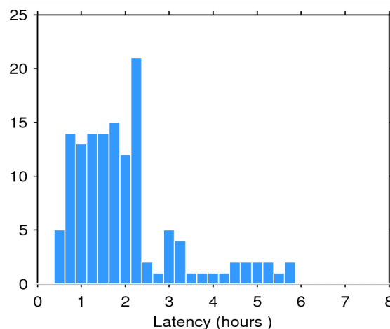
Figure 2. Histogram of the data latency for 06/07/2015. The y-axis denotes the number of files that are made available with a delay of x-hours with respect to the mean time of the records stored in the file.
