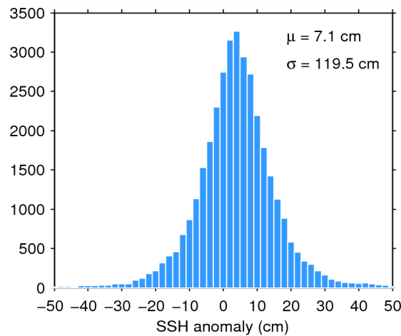
Figure 7. Histogram of flag-valid SSH anomaly over oceans and lakes for 06/07/2015. The mean ( \mu ) and standard deviation ( \sigma ) are also shown. Note that values outside [-50\ 50] cm are excluded from the histogram for the sake of readability but not from the computation of \mu and \sigma .
