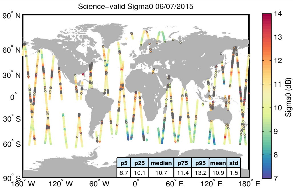
Figure 27. Geographical distribution of science-valid sigma0 data over oceans and lakes for 06/07/2015. The statistical values shown in the table refer to the sigma0 in dB and are calculated over all measurements shown in the figure. Gray circles denote records that have been rejected based on the editing criteria described in Table 4.
