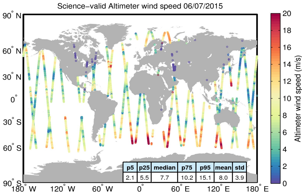
Figure 34. Geographical distribution of science-valid wind data over oceans and lakes for 06/07/2015. The statistical values shown in the table refer to the wind in m/s and are calculated over all measurements shown in the figure. Gray circles denote records that have been rejected based on the editing criteria described in Table 5.
