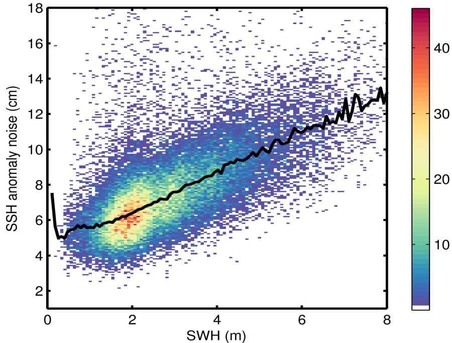
Figure 9. 2D histogram showing flag-valid SSH anomaly noise as a function of SWH for 06/07/2015. The black line denotes the median SSH anomaly as a function of SWH.
