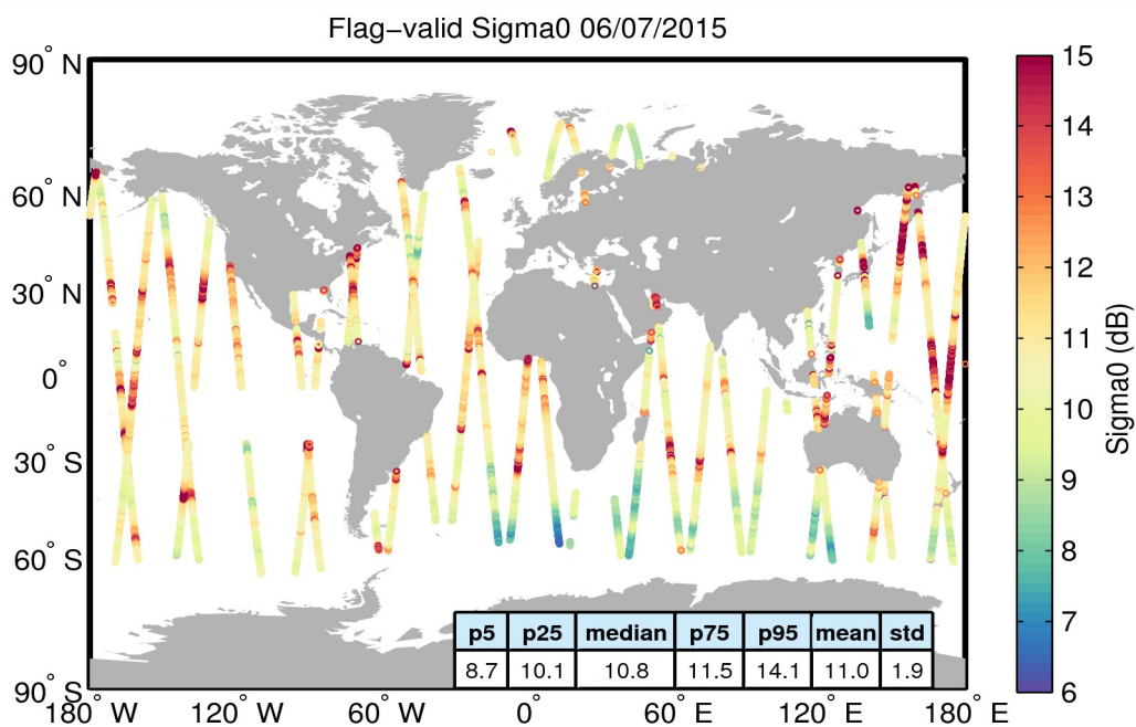
Figure 23. Geographical distribution of flag-valid sigma0 data over oceans and lakes for 06/07/2015. The statistical values shown in the table refer to the sigma0 in dB and are calculated over all measurements shown in the figure.
