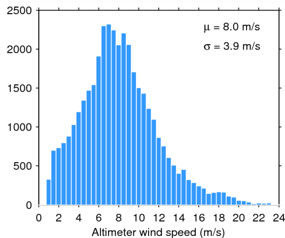
Figure 35. Histogram of science-valid wind over oceans and lakes for 06/07/2015. The mean ( \mu ) and standard deviation ( \sigma ) are also shown. Note that values larger than 24 m/s are excluded from the histogram for the sake of readability but not from the computation of \mu and \sigma .
