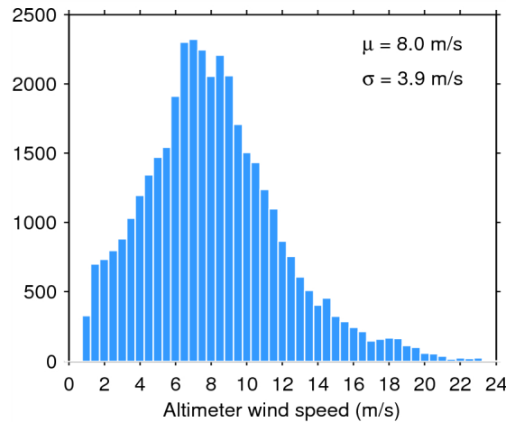
Figure 33. Histogram of flag-valid wind over oceans and lakes for 06/07/2015. The mean ( \mu ) and standard deviation ( \sigma ) are also shown. Note that values larger than 24 m/s are excluded from the histogram for the sake of readability but not from the computation of \mu and \sigma .
