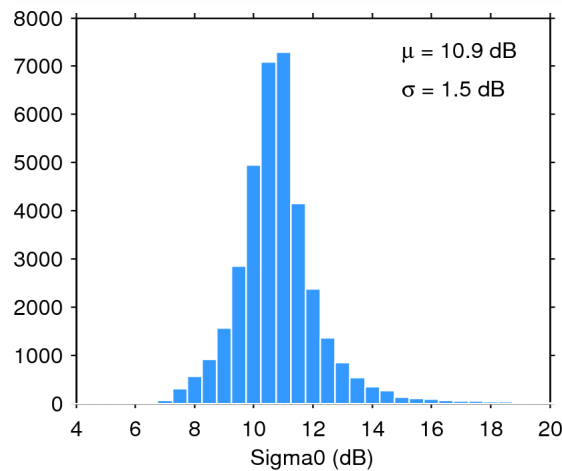
Figure 28. Histogram of science-valid sigma0 over oceans and lakes for 06/07/2015. The mean ( \mu ) and standard deviation ( \sigma ) are also shown. Note that values outside [4 20] dB are excluded from the histogram for the sake of readability but not from the computation of \mu and \sigma .
