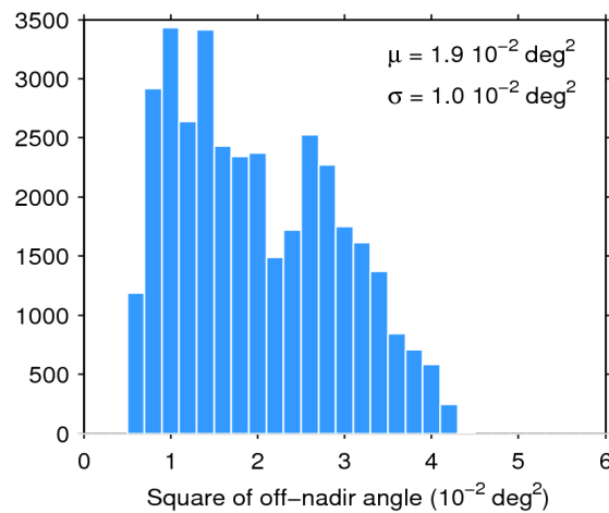
Figure 39. Histogram of flag-valid mispointing over oceans and lakes for 06/07/2015. The mean ( \mu ) and standard deviation ( \sigma ) are also shown. Note that values larger than 6 \cdot 10^{-2} \text{ deg}^2 are excluded from the histogram for the sake of readability but not from the computation of \mu and \sigma .
