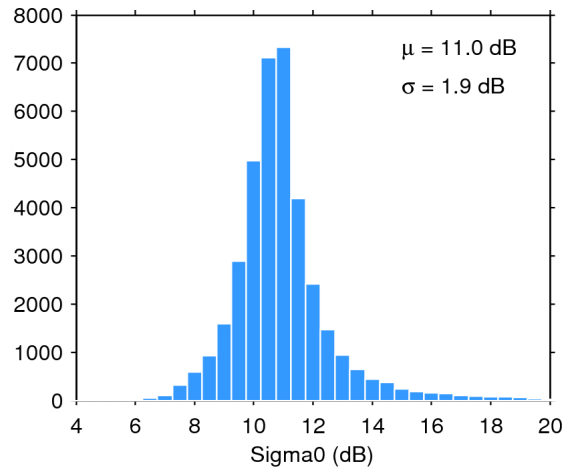
Figure 25. Histogram of flag-valid sigma0 over oceans and lakes for 06/07/2015. The mean ( \mu ) and standard deviation ( \sigma ) are also shown. Note that values outside [4 20] dB are excluded from the histogram for the sake of readability but not from the computation of \mu and \sigma .
