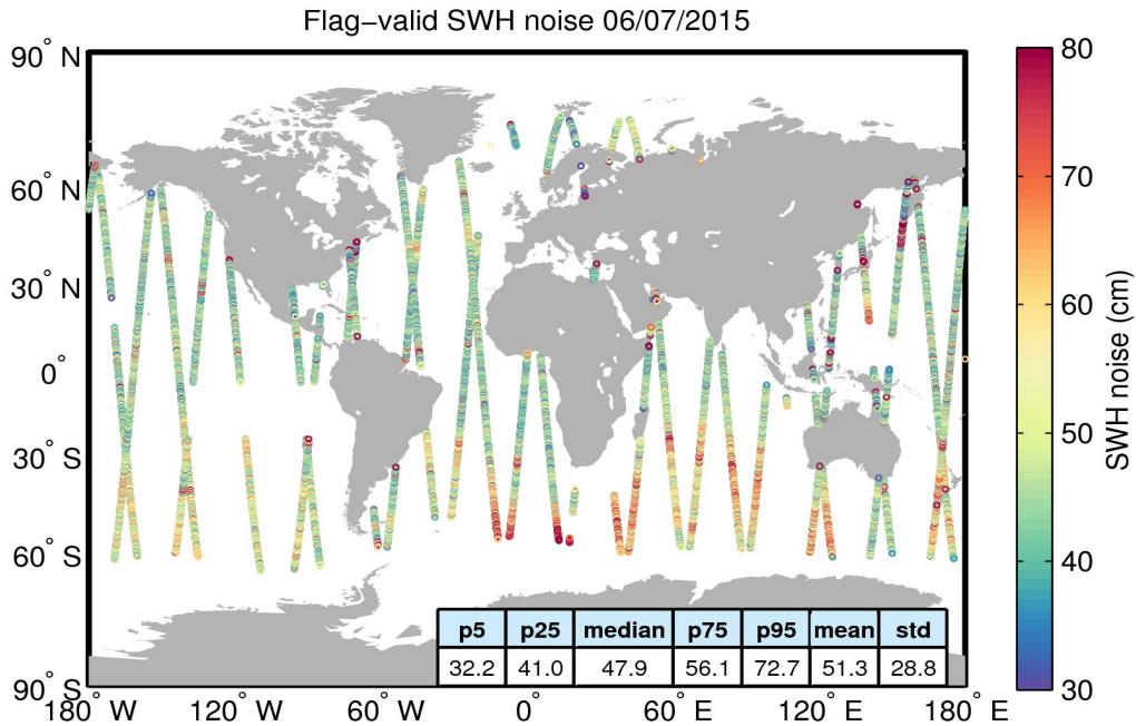
Figure 18. Geographical distribution of flag-valid 20-Hz SWH measurement noise over oceans and lakes for 06/07/2015. The statistical values shown in the figure refer to the SWH noise and are calculated over all measurements shown in the figure.
