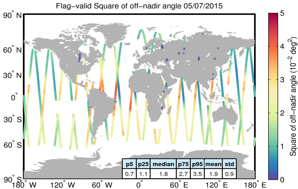
Figure 37. Geographical distribution of flag-valid mispointing data over oceans and lakes for 05/07/2015. The statistical values shown in the table refer to the mispointing in 10^{-2} \text{ deg}^2 and are calculated over all measurements shown in the figure.
