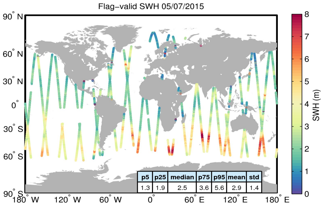
Figure 15. Geographical distribution of flag-valid SWH data over oceans and lakes for 05/07/2015. The statistical values shown in the table refer to the SWH in m and are calculated over all measurements shown in the figure.
