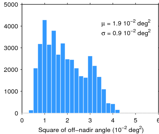
Figure 39. Histogram of flag-valid mispointing over oceans and lakes for 05/07/2015. The mean ( \mu ) and standard deviation ( \sigma ) are also shown. Note that values larger than 6 \cdot 10^{-2} \text{ deg}^2 are excluded from the histogram for the sake of readability but not from the computation of \mu and \sigma .
