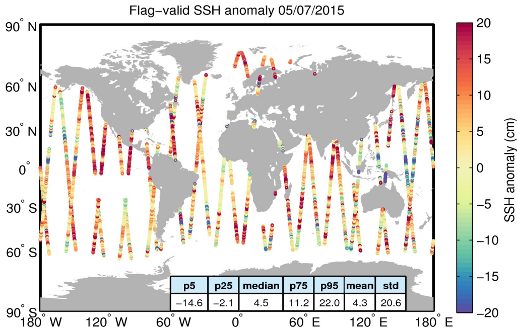
Figure 5. Geographical distribution of flag-valid 1-Hz SSH anomaly data over oceans and lakes for 05/07/2015. The statistical values shown in the table refer to the SSH anomaly in cm and are calculated over all measurements shown in the figure.
