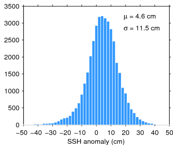
Figure 11. Histogram of science-valid SSH anomaly over oceans and lakes for 05/07/2015. The mean ( \mu ) and standard deviation ( \sigma ) are also shown. Note that values outside [-50 50] cm are excluded from the histogram for the sake of readability but not from the computation of \mu and \sigma .
