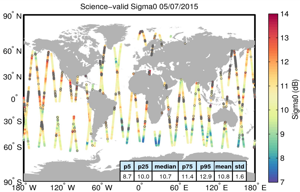
Figure 27. Geographical distribution of science-valid sigma0 data over oceans and lakes for 05/07/2015. The statistical values shown in the table refer to the sigma0 in dB and are calculated over all measurements shown in the figure. Gray circles denote records that have been rejected based on the editing criteria described in Table 4.
