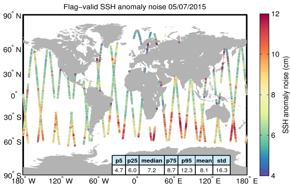
Figure 8. Geographical distribution of flag-valid 20-Hz SSH anomaly measurement noise over oceans and lakes for 05/07/2015. The statistical values shown in the table refer to the SSH anomaly noise and are calculated over all measurements shown in the figure.
