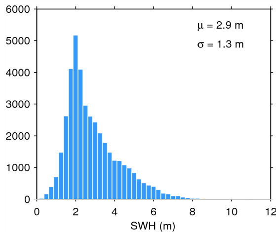
Figure 20. Histogram of science-valid SWH over oceans and lakes for 05/07/2015. The mean ( \mu ) and standard deviation ( \sigma ) are also shown. Note that values larger than 12 m are excluded from the histogram for the sake of readability but not from the computation of \mu and \sigma .
