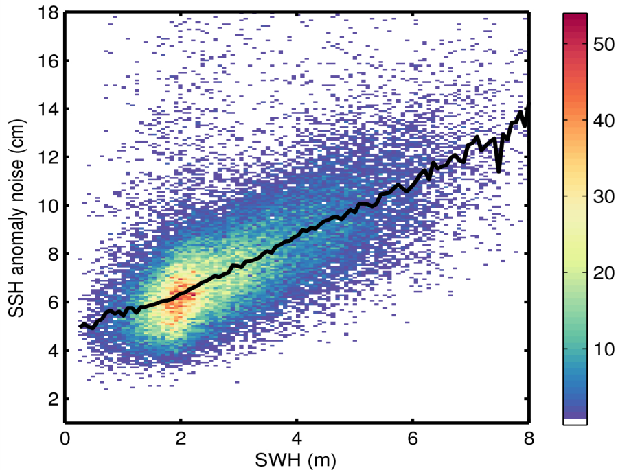
Figure 9. 2D histogram showing flag-valid SSH anomaly noise as a function of SWH for 05/07/2015. The black line denotes the median SSH anomaly as a function of SWH.
