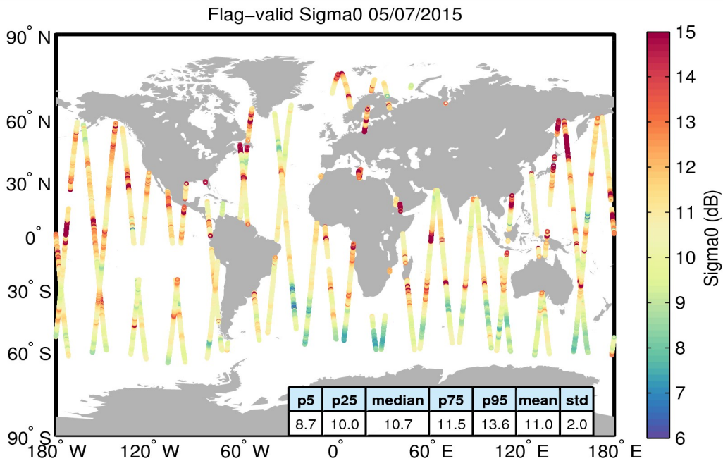
Figure 23. Geographical distribution of flag-valid sigma0 data over oceans and lakes for 05/07/2015. The statistical values shown in the table refer to the sigma0 in dB and are calculated over all measurements shown in the figure.
