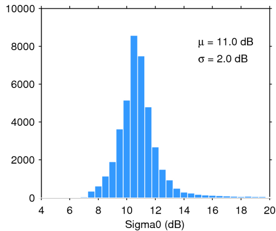
Figure 25. Histogram of flag-valid sigma0 over oceans and lakes for 05/07/2015. The mean ( \mu ) and standard deviation ( \sigma ) are also shown. Note that values outside [4 20] dB are excluded from the histogram for the sake of readability but not from the computation of \mu and \sigma .
