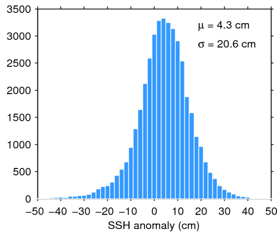
Figure 7. Histogram of flag-valid SSH anomaly over oceans and lakes for 05/07/2015. The mean ( \mu ) and standard deviation ( \sigma ) are also shown. Note that values outside [-50 50] cm are excluded from the histogram for the sake of readability but not from the computation of \mu and \sigma .
