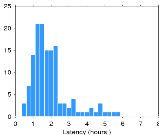
Figure 2. Histogram of the data latency for 05/07/2015. The y-axis denotes the number of files that are made available with a delay of x-hours with respect to the mean time of the records stored in the file.
