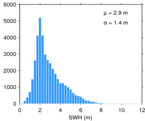
Figure 17. Histogram of flag-valid SWH over oceans and lakes for 05/07/2015. The mean ( \mu ) and standard deviation ( \sigma ) are also shown. Note that values larger than 12 m are excluded from the histogram for the sake of readability but not from the computation of \mu and \sigma .
