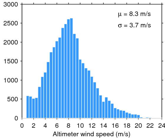
Figure 33. Histogram of flag-valid wind over oceans and lakes for 05/07/2015. The mean ( \mu ) and standard deviation ( \sigma ) are also shown. Note that values larger than 24 m/s are excluded from the histogram for the sake of readability but not from the computation of \mu and \sigma .
