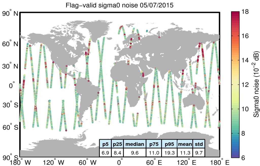
Figure 26. Geographical distribution of flag-valid 20-Hz sigma0 measurement noise over oceans and lakes for 05/07/2015. The statistical values shown in the table refer to the sigma0 noise and are calculated over all measurements shown in the figure.
