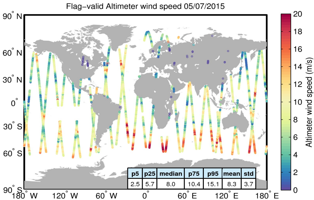
Figure 31. Geographical distribution of flag-valid wind data over oceans and lakes for 05/07/2015. The statistical values shown in the table refer to the wind in m/s and are calculated over all measurements shown in the figure.
