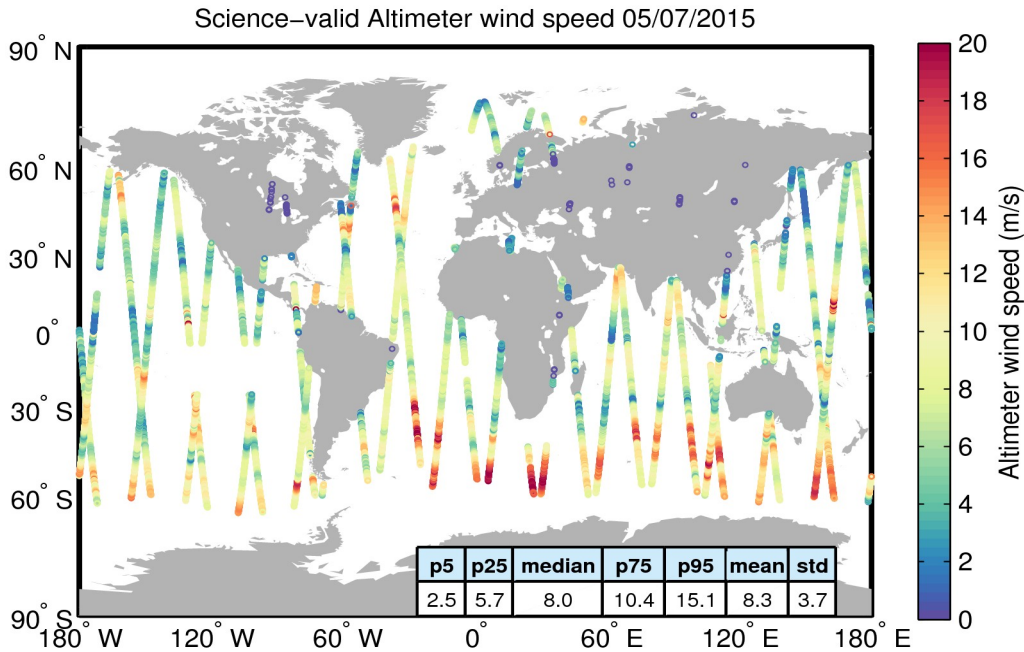
Figure 34. Geographical distribution of science-valid wind data over oceans and lakes for 05/07/2015. The statistical values shown in the table refer to the wind in m/s and are calculated over all measurements shown in the figure. Gray circles denote records that have been rejected based on the editing criteria described in Table 5.
