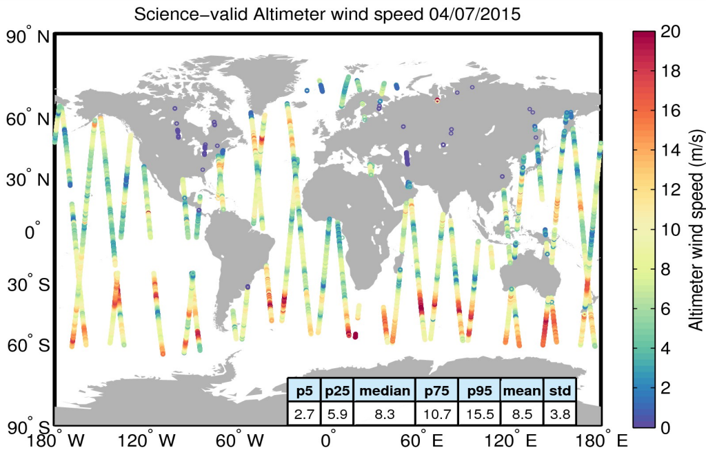
Figure 34. Geographical distribution of science-valid wind data over oceans and lakes for 04/07/2015. The statistical values shown in the table refer to the wind in m/s and are calculated over all measurements shown in the figure. Gray circles denote records that have been rejected based on the editing criteria described in Table 5.
