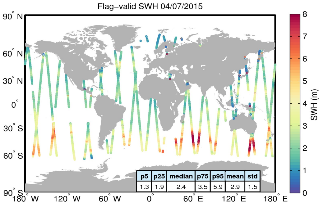
Figure 15. Geographical distribution of flag-valid SWH data over oceans and lakes for 04/07/2015. The statistical values shown in the figure refer to the SWH in m and are calculated over all measurements shown in the figure.
