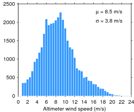
Figure 33. Histogram of flag-valid wind over oceans and lakes for 04/07/2015. The mean ( \mu ) and standard deviation ( \sigma ) are also shown. Note that values larger than 24 m/s are excluded from the histogram for the sake of readability but not from the computation of \mu and \sigma .
