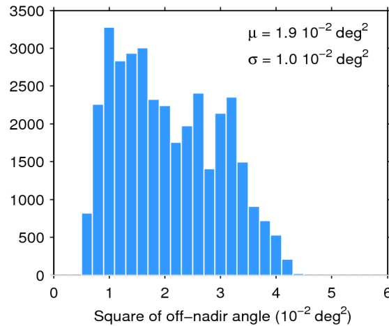
Figure 39. Histogram of flag-valid mispointing over oceans and lakes for 04/07/2015. The mean ( \mu ) and standard deviation ( \sigma ) are also shown. Note that values larger than 6 \cdot 10^{-2} \text{ deg}^2 are excluded from the histogram for the sake of readability but not from the computation of \mu and \sigma .
