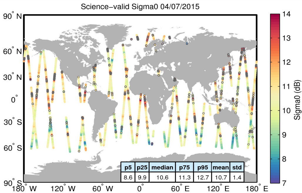
Figure 27. Geographical distribution of science-valid sigma0 data over oceans and lakes for 04/07/2015. The statistical values shown in the table refer to the sigma0 in dB and are calculated over all measurements shown in the figure. Gray circles denote records that have been rejected based on the editing criteria described in Table 4.
