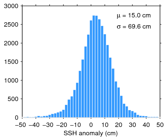
Figure 7. Histogram of flag-valid SSH anomaly over oceans and lakes for 04/07/2015. The mean ( \mu ) and standard deviation ( \sigma ) are also shown. Note that values outside [-50\ 50] cm are excluded from the histogram for the sake of readability but not from the computation of \mu and \sigma .
