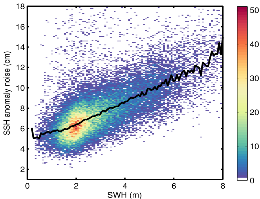
Figure 9. 2D histogram showing flag-valid SSH anomaly noise as a function of SWH for 04/07/2015. The black line denotes the median SSH anomaly as a function of SWH.
