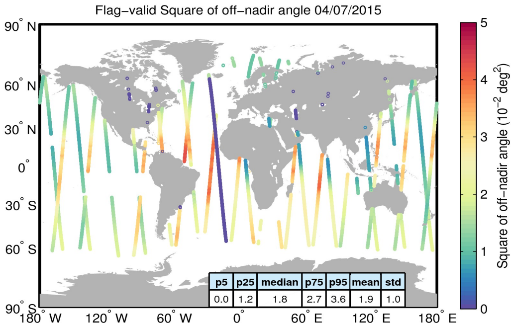
Figure 37. Geographical distribution of flag-valid mispointing data over oceans and lakes for 04/07/2015. The statistical values shown in the table refer to the mispointing in 10^{-2} \text{ deg}^2 and are calculated over all measurements shown in the figure.
