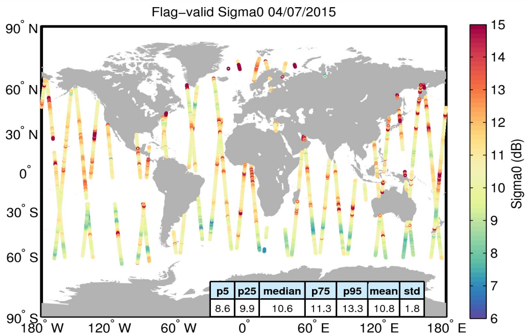
Figure 23. Geographical distribution of flag-valid sigma0 data over oceans and lakes for 04/07/2015. The statistical values shown in the table refer to the sigma0 in dB and are calculated over all measurements shown in the figure.
