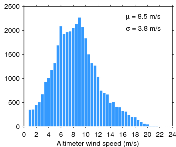
Figure 35. Histogram of science-valid wind over oceans and lakes for 04/07/2015. The mean ( \mu ) and standard deviation ( \sigma ) are also shown. Note that values larger than 24 m/s are excluded from the histogram for the sake of readability but not from the computation of \mu and \sigma .
