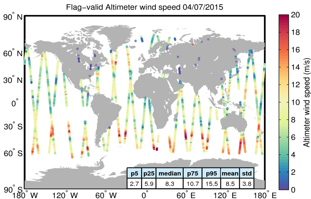
Figure 31. Geographical distribution of flag-valid wind data over oceans and lakes for 04/07/2015. The statistical values shown in the table refer to the wind in m/s and are calculated over all measurements shown in the figure.
