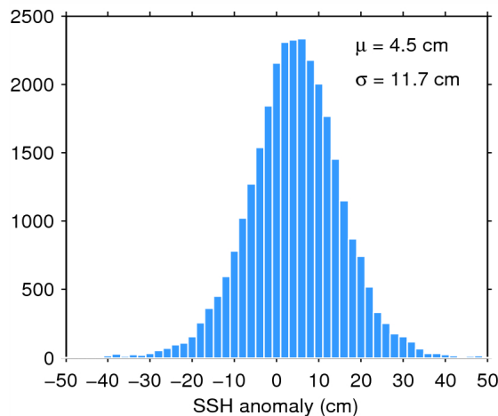
Figure 11. Histogram of science-valid SSH anomaly over oceans and lakes for 04/07/2015. The mean ( \mu ) and standard deviation ( \sigma ) are also shown. Note that values outside [-50 50] cm are excluded from the histogram for the sake of readability but not from the computation of \mu and \sigma .
