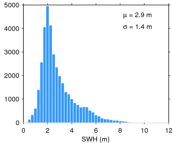
Figure 20. Histogram of science-valid SWH over oceans and lakes for 04/07/2015. The mean ( \mu ) and standard deviation ( \sigma ) are also shown. Note that values larger than 12 m are excluded from the histogram for the sake of readability but not from the computation of \mu and \sigma .
