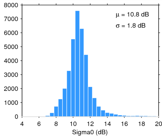
Figure 25. Histogram of flag-valid sigma0 over oceans and lakes for 04/07/2015. The mean ( \mu ) and standard deviation ( \sigma ) are also shown. Note that values outside [4 20] dB are excluded from the histogram for the sake of readability but not from the computation of \mu and \sigma .
