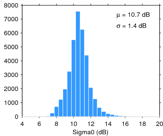
Figure 28. Histogram of science-valid sigma0 over oceans and lakes for 04/07/2015. The mean ( \mu ) and standard deviation ( \sigma ) are also shown. Note that values outside [4 20] dB are excluded from the histogram for the sake of readability but not from the computation of \mu and \sigma .
