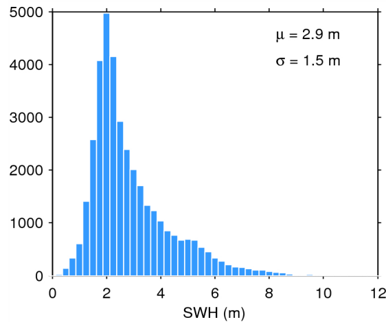
Figure 17. Histogram of flag-valid SWH over oceans and lakes for 04/07/2015. The mean ( \mu ) and standard deviation ( \sigma ) are also shown. Note that values larger than 12 m are excluded from the histogram for the sake of readability but not from the computation of \mu and \sigma .
