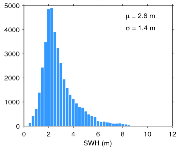
Figure 17. Histogram of flag-valid SWH over oceans and lakes for 03/07/2015. The mean ( \mu ) and standard deviation ( \sigma ) are also shown. Note that values larger than 12 m are excluded from the histogram for the sake of readability but not from the computation of \mu and \sigma .
