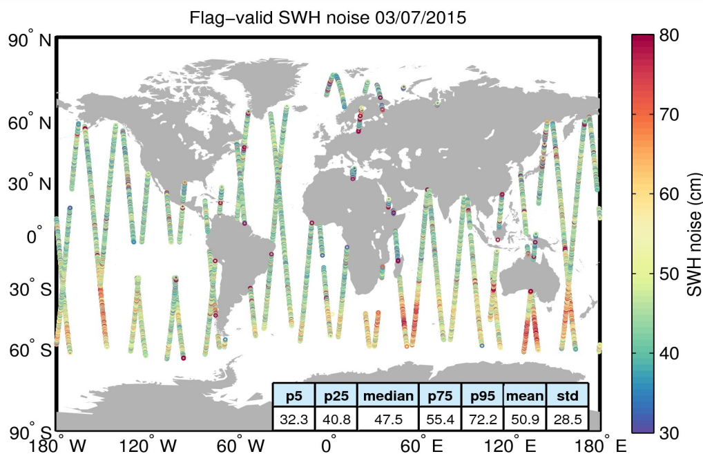
Figure 18. Geographical distribution of flag-valid 20-Hz SWH measurement noise over oceans and lakes for 03/07/2015. The statistical values shown in the figure refer to the SWH noise and are calculated over all measurements shown in the figure.
