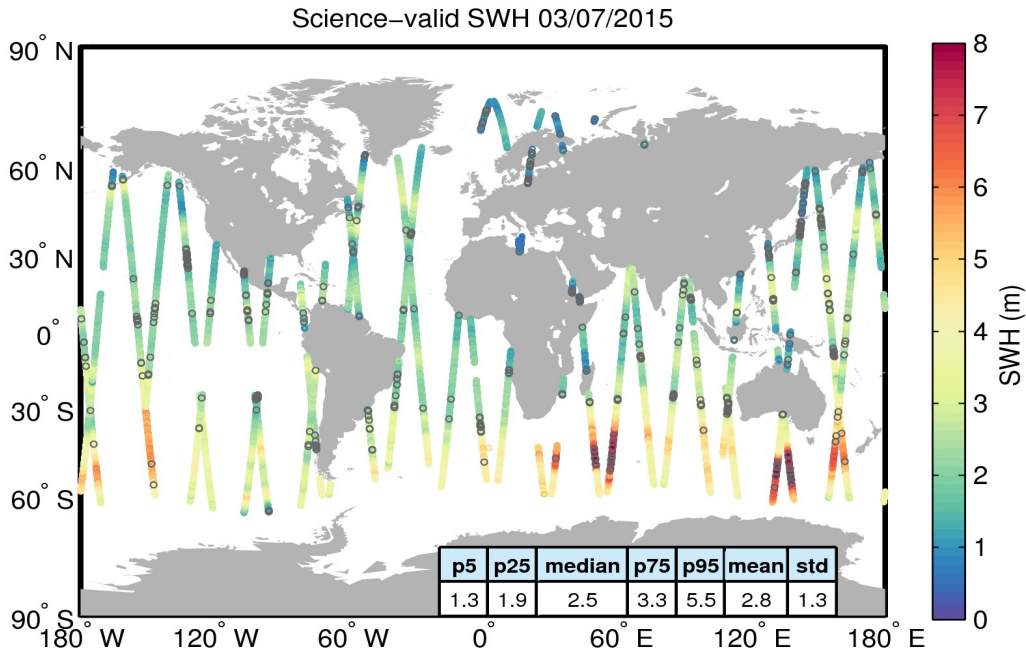
Figure 19. Geographical distribution of science-valid SWH data over oceans and lakes for 03/07/2015. The statistical values shown in the table refer to the SWH in m and are calculated over all measurements shown in the figure. Gray circles denote records that have been rejected based on the editing criteria described in Table 3.
