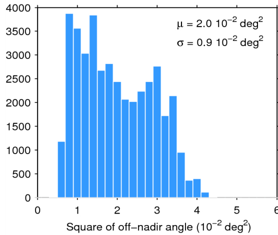
Figure 39. Histogram of flag-valid mispointing over oceans and lakes for 03/07/2015. The mean ( \mu ) and standard deviation ( \sigma ) are also shown. Note that values larger than 6 \cdot 10^{-2} \text{ deg}^2 are excluded from the histogram for the sake of readability but not from the computation of \mu and \sigma .
