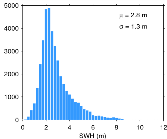
Figure 20. Histogram of science-valid SWH over oceans and lakes for 03/07/2015. The mean ( \mu ) and standard deviation ( \sigma ) are also shown. Note that values larger than 12 m are excluded from the histogram for the sake of readability but not from the computation of \mu and \sigma .
