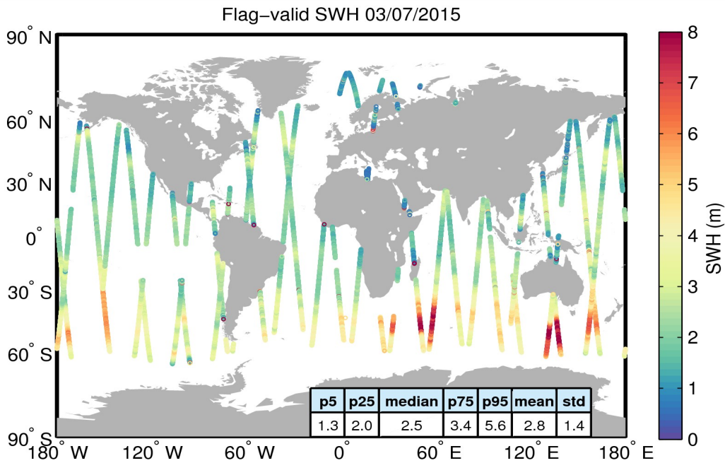
Figure 15. Geographical distribution of flag-valid SWH data over oceans and lakes for 03/07/2015. The statistical values shown in the table refer to the SWH in m and are calculated over all measurements shown in the figure.
