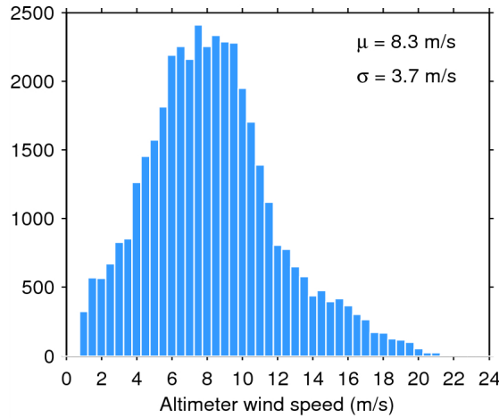
Figure 33. Histogram of flag-valid wind over oceans and lakes for 03/07/2015. The mean ( \mu ) and standard deviation ( \sigma ) are also shown. Note that values larger than 24 m/s are excluded from the histogram for the sake of readability but not from the computation of \mu and \sigma .
