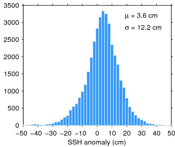
Figure 11. Histogram of science-valid SSH anomaly over oceans and lakes for 03/07/2015. The mean ( \mu ) and standard deviation ( \sigma ) are also shown. Note that values outside [-50 50] cm are excluded from the histogram for the sake of readability but not from the computation of \mu and \sigma .
