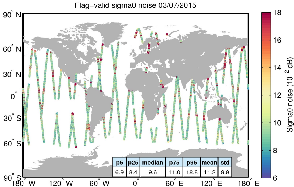
Figure 26. Geographical distribution of flag-valid 20-Hz sigma0 measurement noise over oceans and lakes for 03/07/2015. The statistical values shown in the table refer to the sigma0 noise and are calculated over all measurements shown in the figure.
