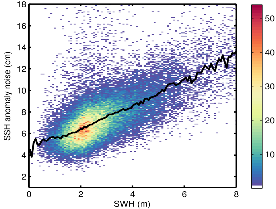
Figure 9. 2D histogram showing flag-valid SSH anomaly noise as a function of SWH for 03/07/2015. The black line denotes the median SSH anomaly as a function of SWH.
