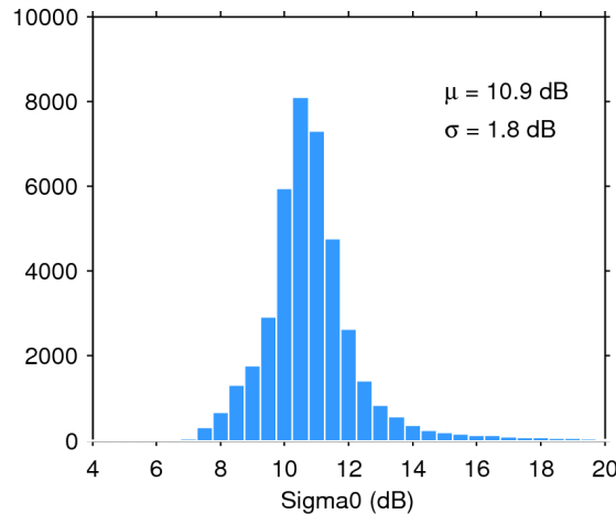
Figure 25. Histogram of flag-valid sigma0 over oceans and lakes for 03/07/2015. The mean ( \mu ) and standard deviation ( \sigma ) are also shown. Note that values outside [4 20] dB are excluded from the histogram for the sake of readability but not from the computation of \mu and \sigma .
