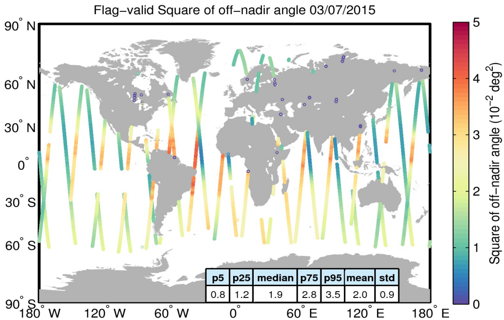
Figure 37. Geographical distribution of flag-valid mispointing data over oceans and lakes for 03/07/2015. The statistical values shown in the table refer to the mispointing in 10^{-2} \text{ deg}^2 and are calculated over all measurements shown in the figure.
