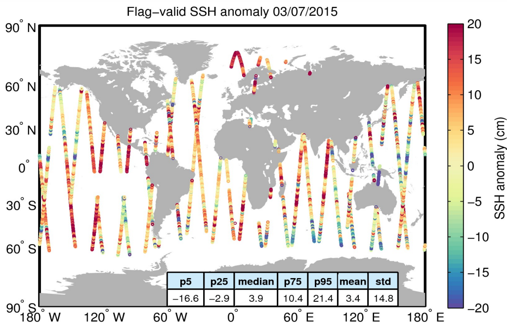
Figure 5. Geographical distribution of flag-valid 1-Hz SSH anomaly data over oceans and lakes for 03/07/2015. The statistical values shown in the table refer to the SSH anomaly in cm and are calculated over all measurements shown in the figure.
