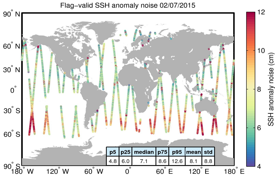
Figure 8. Geographical distribution of flag-valid 20-Hz SSH anomaly measurement noise over oceans and lakes for 02/07/2015. The statistical values shown in the table refer to the SSH anomaly noise and are calculated over all measurements shown in the figure.
