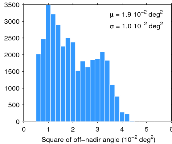
Figure 39. Histogram of flag-valid mispointing over oceans and lakes for 02/07/2015. The mean ( \mu ) and standard deviation ( \sigma ) are also shown. Note that values larger than 6 \cdot 10^{-2} \text{ deg}^2 are excluded from the histogram for the sake of readability but not from the computation of \mu and \sigma .
