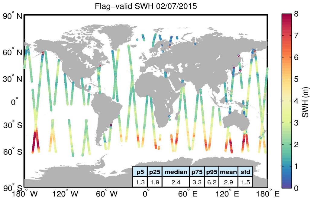
Figure 15. Geographical distribution of flag-valid SWH data over oceans and lakes for 02/07/2015. The statistical values shown in the table refer to the SWH in m and are calculated over all measurements shown in the figure.
