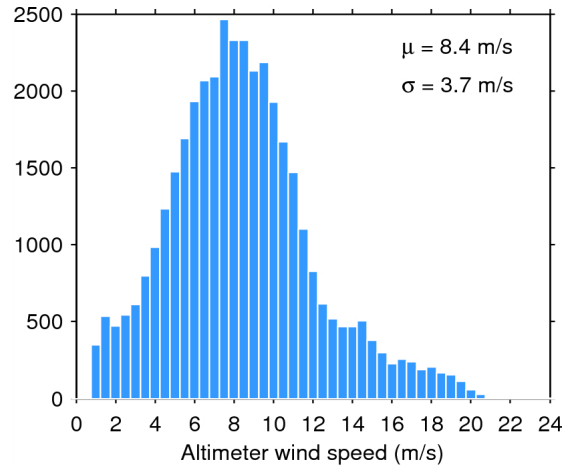
Figure 33. Histogram of flag-valid wind over oceans and lakes for 02/07/2015. The mean ( \mu ) and standard deviation ( \sigma ) are also shown. Note that values larger than 24 m/s are excluded from the histogram for the sake of readability but not from the computation of \mu and \sigma .
