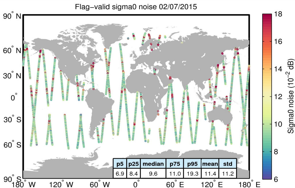
Figure 26. Geographical distribution of flag-valid 20-Hz sigma0 measurement noise over oceans and lakes for 02/07/2015. The statistical values shown in the table refer to the sigma0 noise and are calculated over all measurements shown in the figure.
