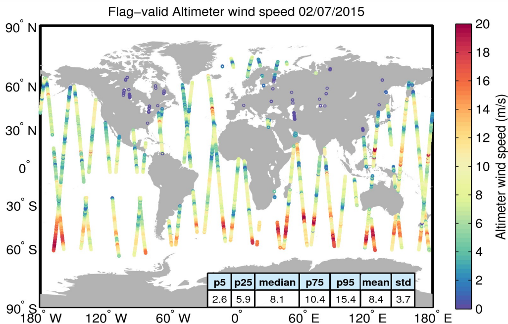
Figure 31. Geographical distribution of flag-valid wind data over oceans and lakes for 02/07/2015. The statistical values shown in the table refer to the wind in m/s and are calculated over all measurements shown in the figure.
