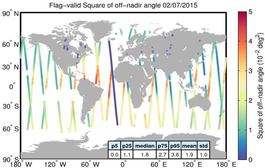
Figure 37. Geographical distribution of flag-valid mispointing data over oceans and lakes for 02/07/2015. The statistical values shown in the table refer to the mispointing in 10^{-2} deg 2 and are calculated over all measurements shown in the figure.
