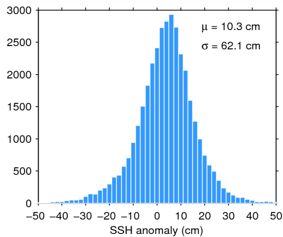
Figure 7. Histogram of flag-valid SSH anomaly over oceans and lakes for 02/07/2015. The mean ( \mu ) and standard deviation ( \sigma ) are also shown. Note that values outside [-50 50] cm are excluded from the histogram for the sake of readability but not from the computation of \mu and \sigma .
