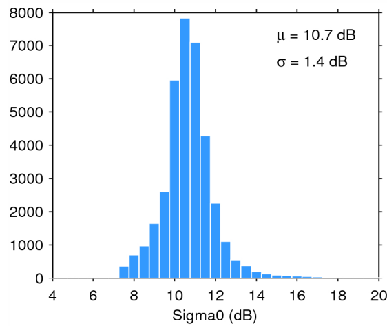
Figure 28. Histogram of science-valid sigma0 over oceans and lakes for 02/07/2015. The mean ( \mu ) and standard deviation ( \sigma ) are also shown. Note that values outside [4 20] dB are excluded from the histogram for the sake of readability but not from the computation of \mu and \sigma .
