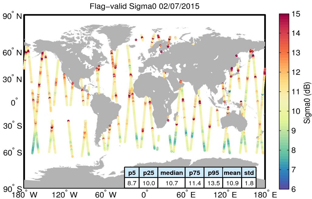
Figure 23. Geographical distribution of flag-valid sigma0 data over oceans and lakes for 02/07/2015. The statistical values shown in the table refer to the sigma0 in dB and are calculated over all measurements shown in the figure.
