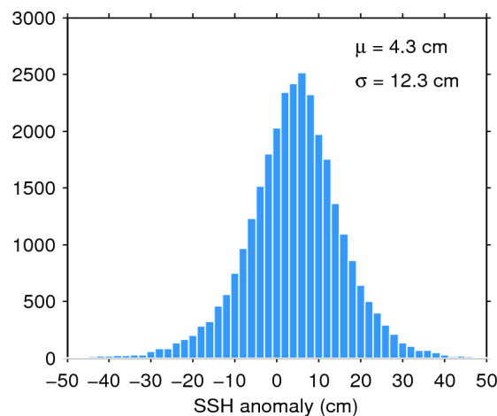
Figure 11. Histogram of science-valid SSH anomaly over oceans and lakes for 02/07/2015. The mean ( \mu ) and standard deviation ( \sigma ) are also shown. Note that values outside [-50 50] cm are excluded from the histogram for the sake of readability but not from the computation of \mu and \sigma .
