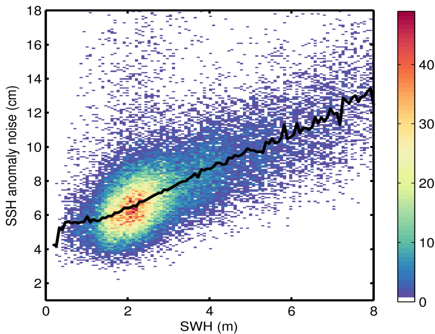
Figure 9. 2D histogram showing flag-valid SSH anomaly noise as a function of SWH for 02/07/2015. The black line denotes the median SSH anomaly as a function of SWH.
