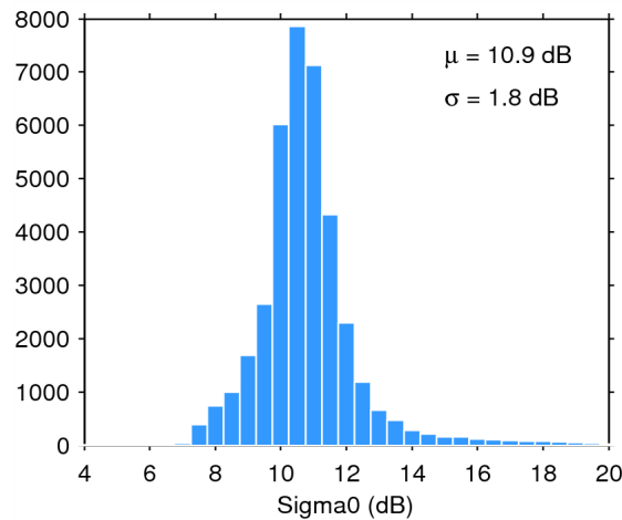
Figure 25. Histogram of flag-valid sigma0 over oceans and lakes for 02/07/2015. The mean ( \mu ) and standard deviation ( \sigma ) are also shown. Note that values outside [4 20] dB are excluded from the histogram for the sake of readability but not from the computation of \mu and \sigma .
