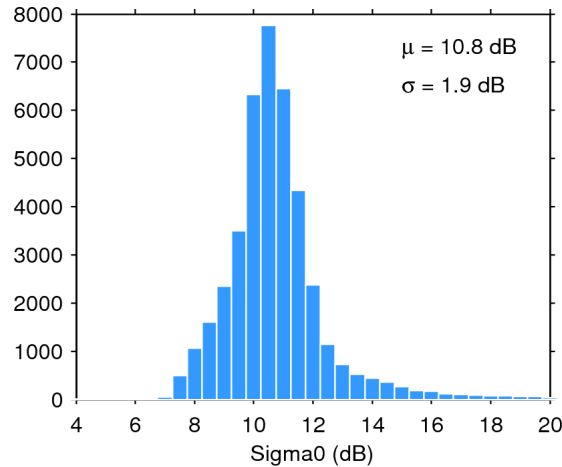
Figure 25. Histogram of flag-valid sigma0 over oceans and lakes for 01/07/2015. The mean ( \mu ) and standard deviation ( \sigma ) are also shown. Note that values outside [4 20] dB are excluded from the histogram for the sake of readability but not from the computation of \mu and \sigma .
