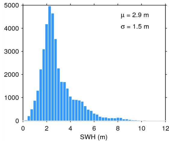
Figure 17. Histogram of flag-valid SWH over oceans and lakes for 01/07/2015. The mean ( \mu ) and standard deviation ( \sigma ) are also shown. Note that values larger than 12 m are excluded from the histogram for the sake of readability but not from the computation of \mu and \sigma .
