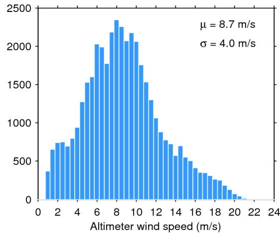
Figure 33. Histogram of flag-valid wind over oceans and lakes for 01/07/2015. The mean ( \mu ) and standard deviation ( \sigma ) are also shown. Note that values larger than 24 m/s are excluded from the histogram for the sake of readability but not from the computation of \mu and \sigma .
