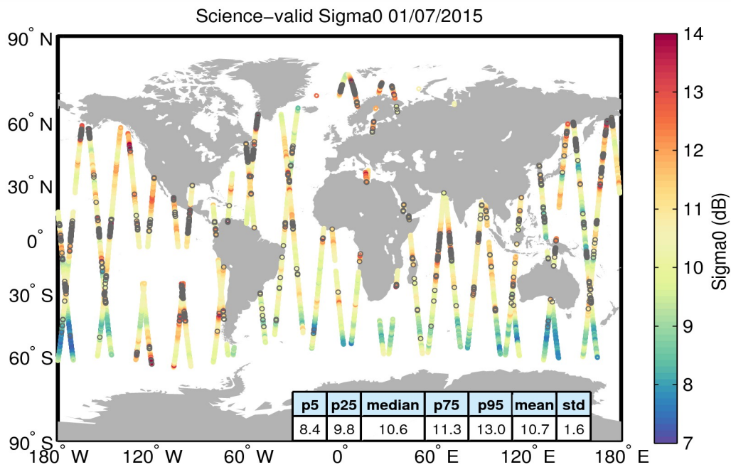
Figure 27. Geographical distribution of science-valid sigma0 data over oceans and lakes for 01/07/2015. The statistical values shown in the table refer to the sigma0 in dB and are calculated over all measurements shown in the figure. Gray circles denote records that have been rejected based on the editing criteria described in Table 4.
