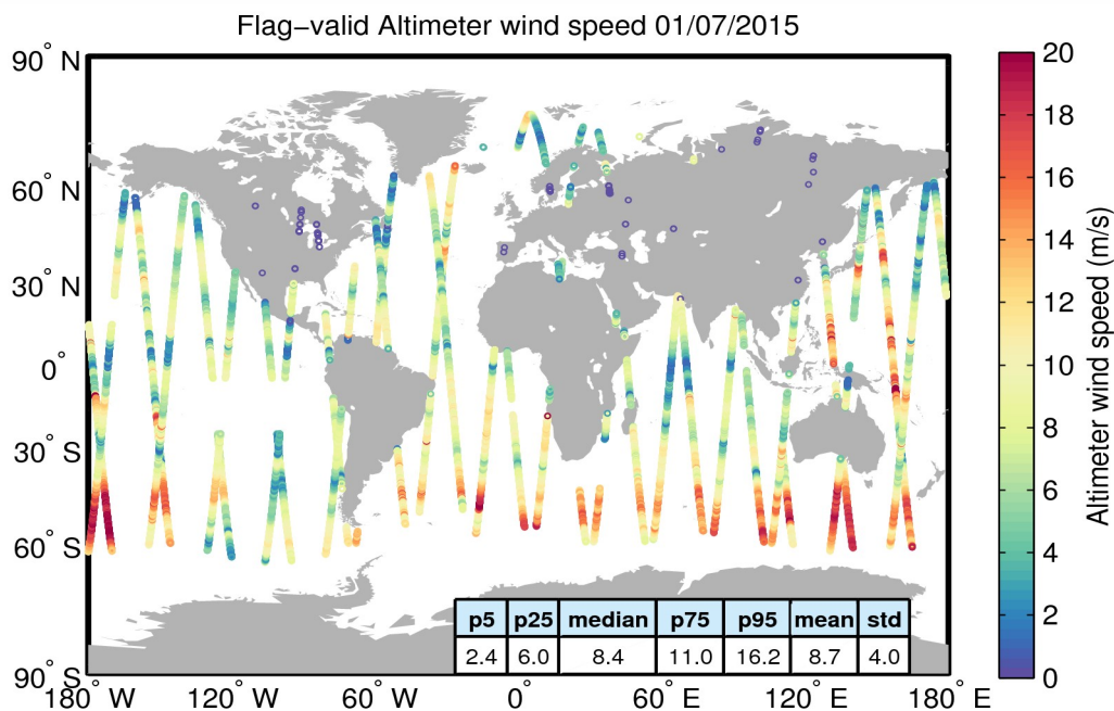
Figure 31. Geographical distribution of flag-valid wind data over oceans and lakes for 01/07/2015. The statistical values shown in the table refer to the wind in m/s and are calculated over all measurements shown in the figure.
