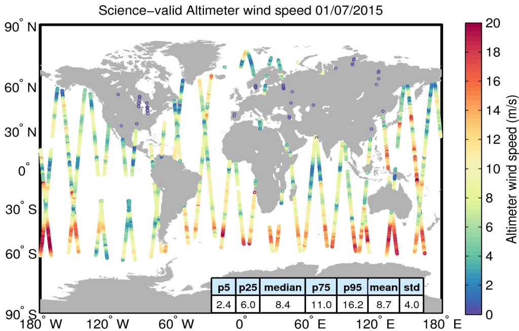
Figure 34. Geographical distribution of science-valid wind data over oceans and lakes for 01/07/2015. The statistical values shown in the table refer to the wind in m/s and are calculated over all measurements shown in the figure. Gray circles denote records that have been rejected based on the editing criteria described in Table 5.
