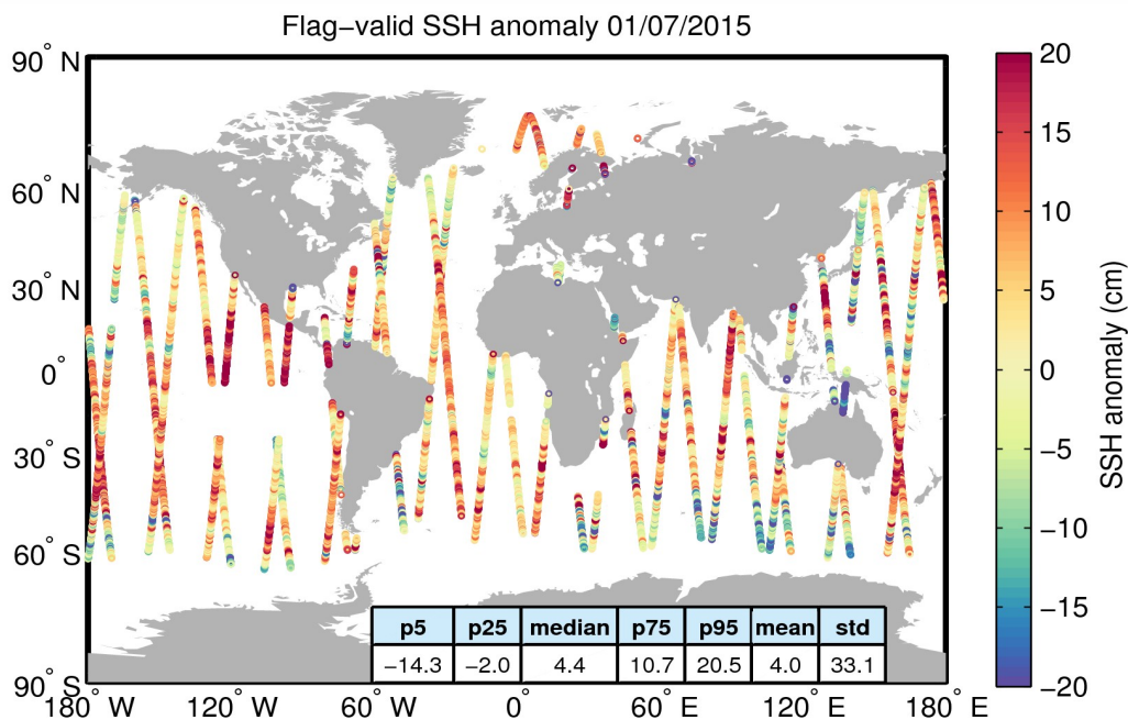
Figure 5. Geographical distribution of flag-valid 1-Hz SSH anomaly data over oceans and lakes for 01/07/2015. The statistical values shown in the table refer to the SSH anomaly in cm and are calculated over all measurements shown in the figure.
