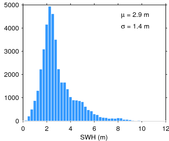
Figure 20. Histogram of science-valid SWH over oceans and lakes for 01/07/2015. The mean ( \mu ) and standard deviation ( \sigma ) are also shown. Note that values larger than 12 m are excluded from the histogram for the sake of readability but not from the computation of \mu and \sigma .
