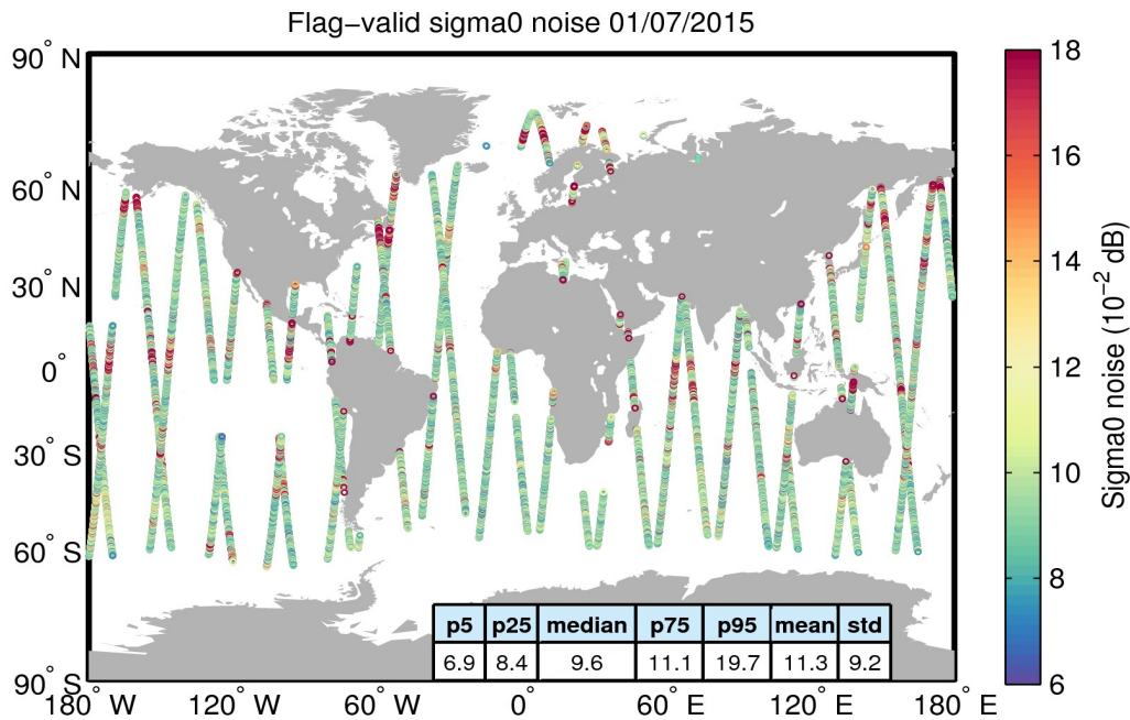
Figure 26. Geographical distribution of flag-valid 20-Hz sigma0 measurement noise over oceans and lakes for 01/07/2015. The statistical values shown in the table refer to the sigma0 noise and are calculated over all measurements shown in the figure.
