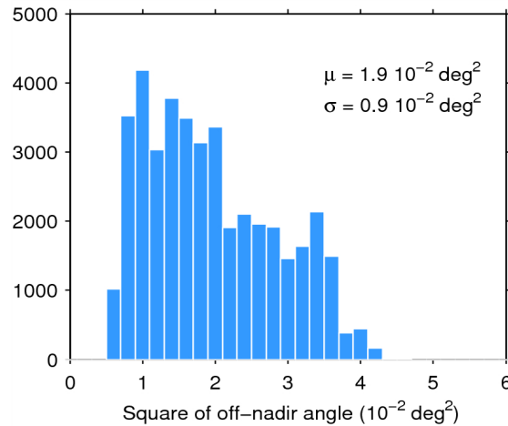
Figure 39. Histogram of flag-valid mispointing over oceans and lakes for 01/07/2015. The mean ( \mu ) and standard deviation ( \sigma ) are also shown. Note that values larger than 6 \cdot 10^{-2} \text{ deg}^2 are excluded from the histogram for the sake of readability but not from the computation of \mu and \sigma .
