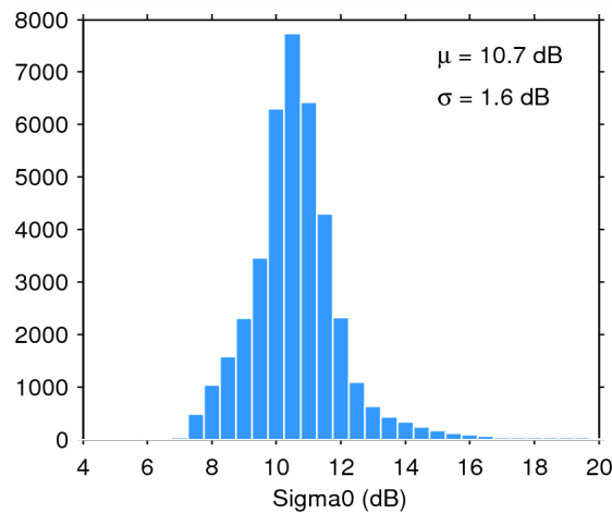
Figure 28. Histogram of science-valid sigma0 over oceans and lakes for 01/07/2015. The mean ( \mu ) and standard deviation ( \sigma ) are also shown. Note that values outside [4 20] dB are excluded from the histogram for the sake of readability but not from the computation of \mu and \sigma .
