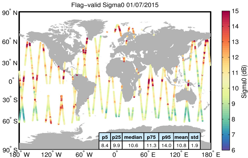
Figure 23. Geographical distribution of flag-valid sigma0 data over oceans and lakes for 01/07/2015. The statistical values shown in the table refer to the sigma0 in dB and are calculated over all measurements shown in the figure.
