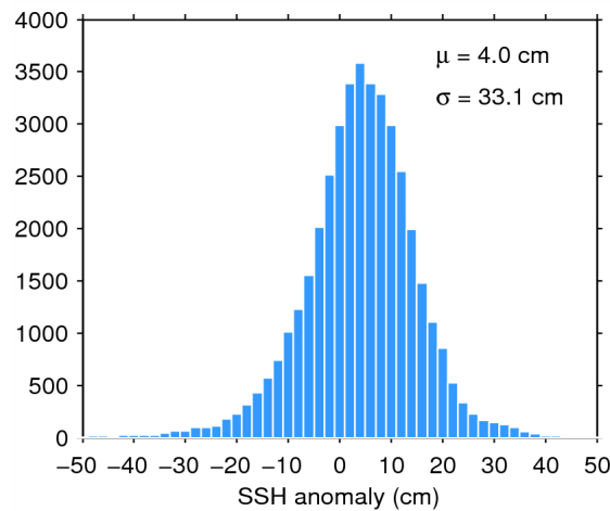
Figure 7. Histogram of flag-valid SSH anomaly over oceans and lakes for 01/07/2015. The mean ( \mu ) and standard deviation ( \sigma ) are also shown. Note that values outside [-50\ 50] cm are excluded from the histogram for the sake of readability but not from the computation of \mu and \sigma .
