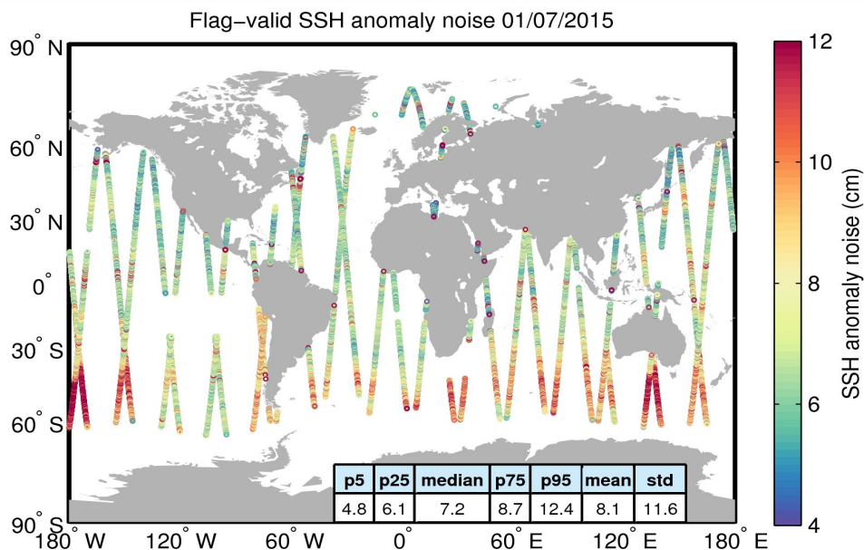
Figure 8. Geographical distribution of flag-valid 20-Hz SSH anomaly measurement noise over oceans and lakes for 01/07/2015. The statistical values shown in the table refer to the SSH anomaly noise and are calculated over all measurements shown in the figure.
