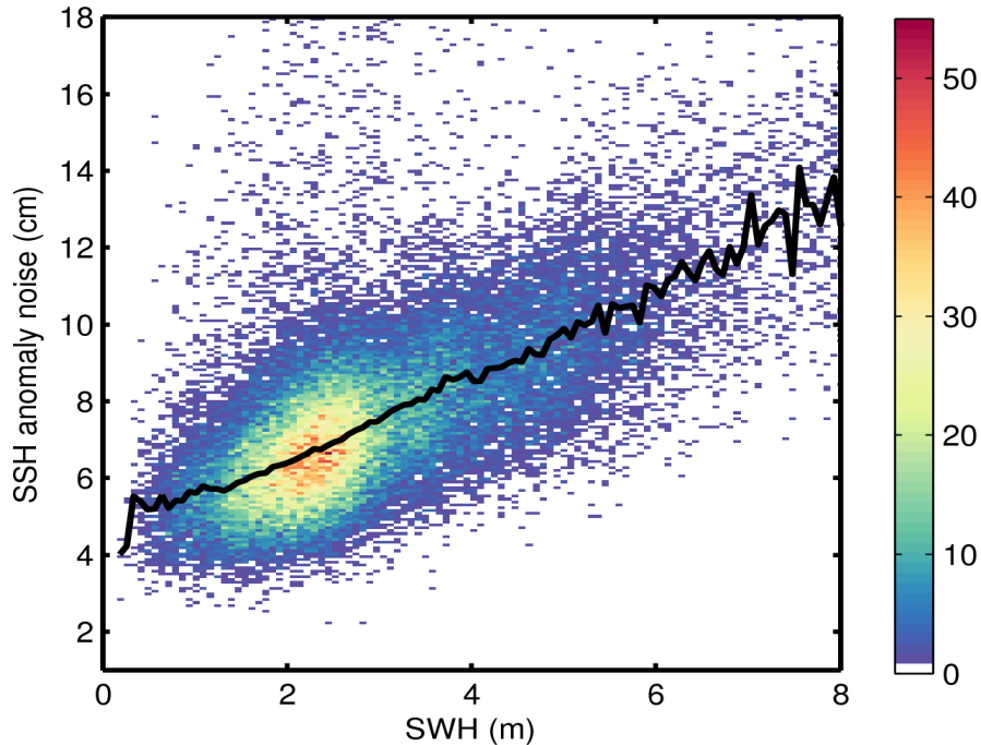
Figure 9. 2D histogram showing flag-valid SSH anomaly noise as a function of SWH for 01/07/2015. The black line denotes the median SSH anomaly as a function of SWH.
