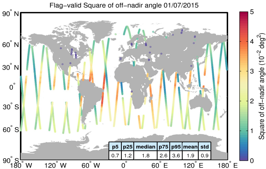
Figure 37. Geographical distribution of flag-valid mispointing data over oceans and lakes for 01/07/2015. The statistical values shown in the table refer to the mispointing in 10^{-2} \text{deg}^2 and are calculated over all measurements shown in the figure.
