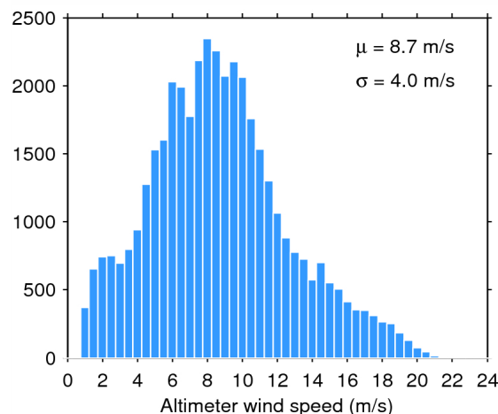
Figure 35. Histogram of science-valid wind over oceans and lakes for 01/07/2015. The mean ( \mu ) and standard deviation ( \sigma ) are also shown. Note that values larger than 24 m/s are excluded from the histogram for the sake of readability but not from the computation of \mu and \sigma .
