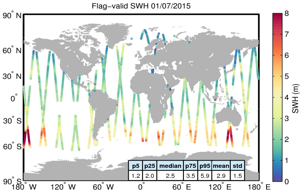
Figure 15. Geographical distribution of flag-valid SWH data over oceans and lakes for 01/07/2015. The statistical values shown in the figure refer to the SWH in m and are calculated over all measurements shown in the figure.
