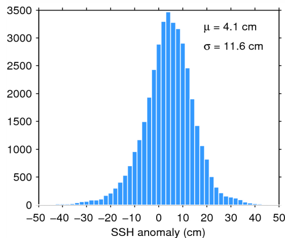
Figure 11. Histogram of science-valid SSH anomaly over oceans and lakes for 01/07/2015. The mean ( \mu ) and standard deviation ( \sigma ) are also shown. Note that values outside [-50 50] cm are excluded from the histogram for the sake of readability but not from the computation of \mu and \sigma .
