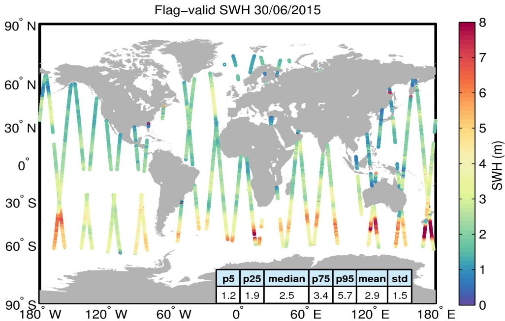
Figure 15. Geographical distribution of flag-valid SWH data over oceans and lakes for 30/06/2015. The statistical values shown in the table refer to the SWH in m and are calculated over all measurements shown in the figure.
