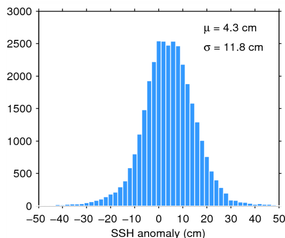
Figure 11. Histogram of science-valid SSH anomaly over oceans and lakes for 30/06/2015. The mean ( \mu ) and standard deviation ( \sigma ) are also shown. Note that values outside [-50 50] cm are excluded from the histogram for the sake of readability but not from the computation of \mu and \sigma .
