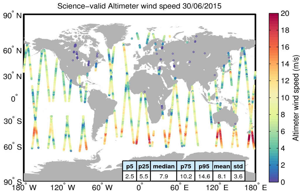
Figure 34. Geographical distribution of science-valid wind data over oceans and lakes for 30/06/2015. The statistical values shown in the table refer to the wind in m/s and are calculated over all measurements shown in the figure. Gray circles denote records that have been rejected based on the editing criteria described in Table 5.
