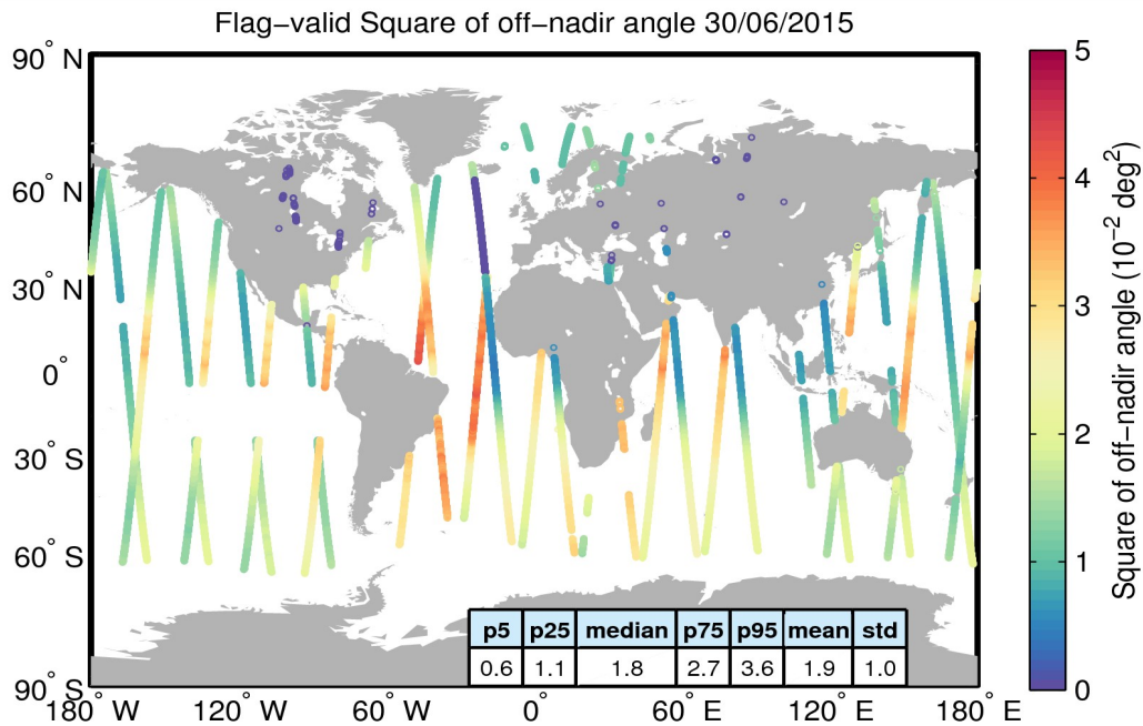
Figure 37. Geographical distribution of flag-valid mispointing data over oceans and lakes for 30/06/2015. The statistical values shown in the table refer to the mispointing in 10^{-2} deg 2 and are calculated over all measurements shown in the figure.
