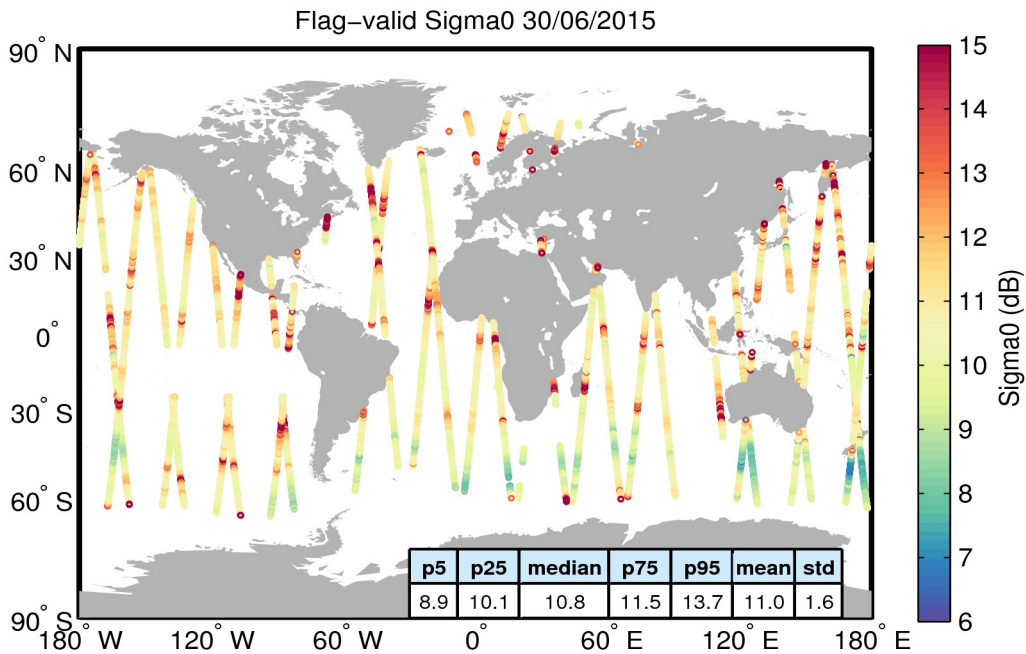
Figure 23. Geographical distribution of flag-valid sigma0 data over oceans and lakes for 30/06/2015. The statistical values shown in the table refer to the sigma0 in dB and are calculated over all measurements shown in the figure.
