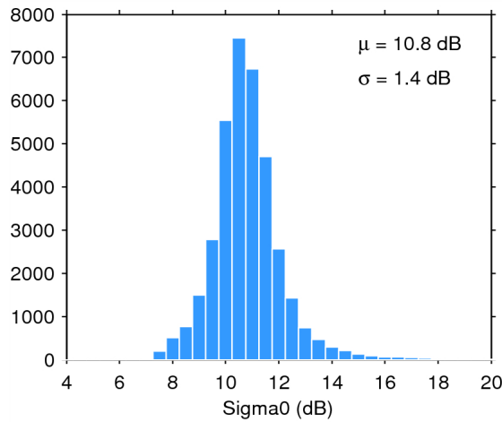
Figure 28. Histogram of science-valid sigma0 over oceans and lakes for 30/06/2015. The mean ( \mu ) and standard deviation ( \sigma ) are also shown. Note that values outside [4 20] dB are excluded from the histogram for the sake of readability but not from the computation of \mu and \sigma .
