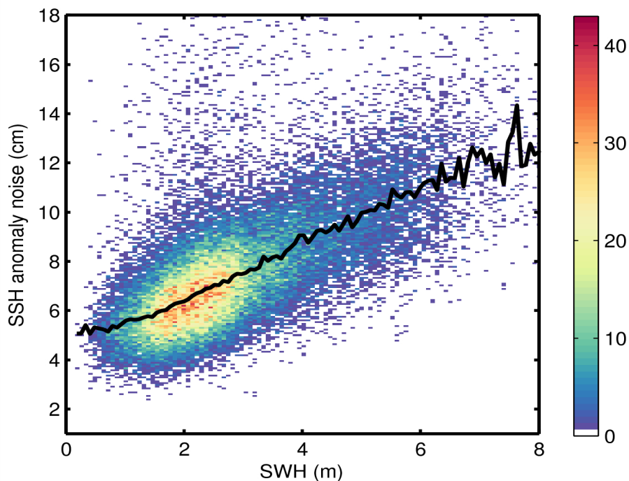
Figure 9. 2D histogram showing flag-valid SSH anomaly noise as a function of SWH for 30/06/2015. The black line denotes the median SSH anomaly as a function of SWH.
