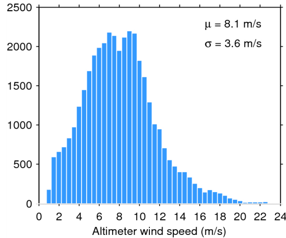
Figure 33. Histogram of flag-valid wind over oceans and lakes for 30/06/2015. The mean ( \mu ) and standard deviation ( \sigma ) are also shown. Note that values larger than 24 m/s are excluded from the histogram for the sake of readability but not from the computation of \mu and \sigma .
