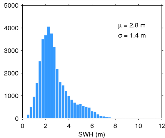
Figure 20. Histogram of science-valid SWH over oceans and lakes for 30/06/2015. The mean ( \mu ) and standard deviation ( \sigma ) are also shown. Note that values larger than 12 m are excluded from the histogram for the sake of readability but not from the computation of \mu and \sigma .
