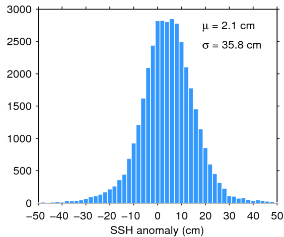
Figure 7. Histogram of flag-valid SSH anomaly over oceans and lakes for 30/06/2015. The mean ( \mu ) and standard deviation ( \sigma ) are also shown. Note that values outside [-50 50] cm are excluded from the histogram for the sake of readability but not from the computation of \mu and \sigma .
