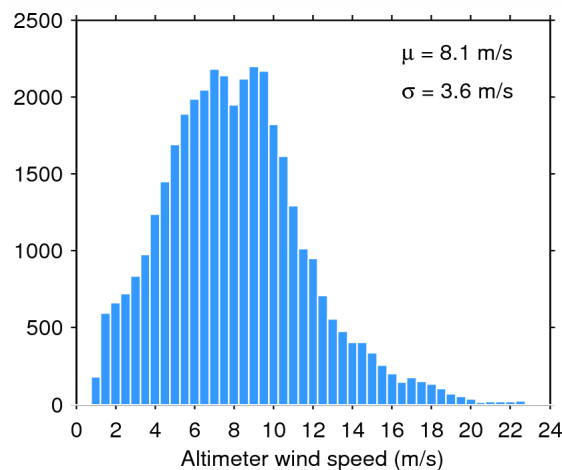
Figure 35. Histogram of science-valid wind over oceans and lakes for 30/06/2015. The mean ( \mu ) and standard deviation ( \sigma ) are also shown. Note that values larger than 24 m/s are excluded from the histogram for the sake of readability but not from the computation of \mu and \sigma .
