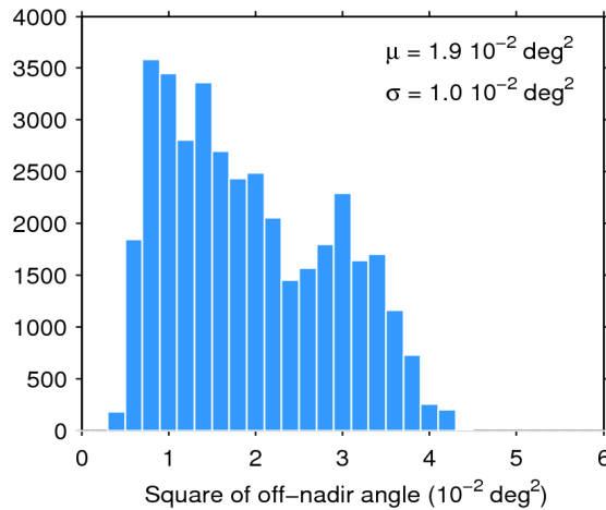
Figure 39. Histogram of flag-valid mispointing over oceans and lakes for 30/06/2015. The mean ( \mu ) and standard deviation ( \sigma ) are also shown. Note that values larger than 6 \cdot 10^{-2} \text{ deg}^2 are excluded from the histogram for the sake of readability but not from the computation of \mu and \sigma .
