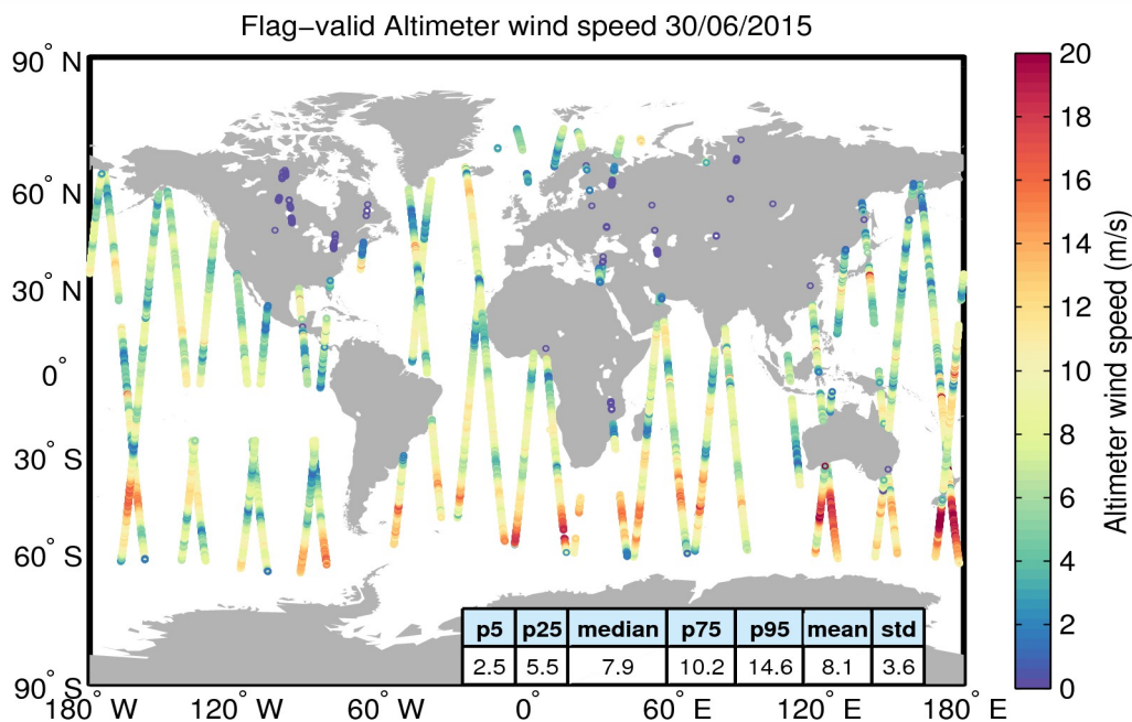
Figure 31. Geographical distribution of flag-valid wind data over oceans and lakes for 30/06/2015. The statistical values shown in the table refer to the wind in m/s and are calculated over all measurements shown in the figure.
