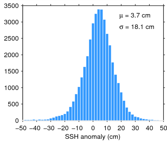
Figure 7. Histogram of flag-valid SSH anomaly over oceans and lakes for 29/06/2015. The mean ( \mu ) and standard deviation ( \sigma ) are also shown. Note that values outside [-50\ 50] cm are excluded from the histogram for the sake of readability but not from the computation of \mu and \sigma .
