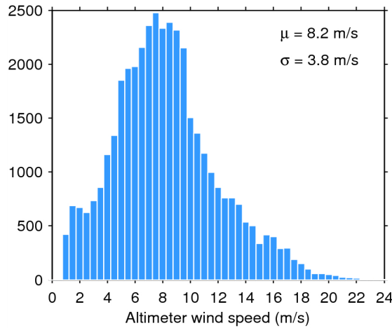
Figure 33. Histogram of flag-valid wind over oceans and lakes for 29/06/2015. The mean ( \mu ) and standard deviation ( \sigma ) are also shown. Note that values larger than 24 m/s are excluded from the histogram for the sake of readability but not from the computation of \mu and \sigma .
