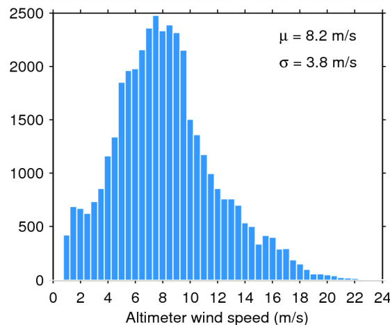
Figure 35. Histogram of science-valid wind over oceans and lakes for 29/06/2015. The mean ( \mu ) and standard deviation ( \sigma ) are also shown. Note that values larger than 24 m/s are excluded from the histogram for the sake of readability but not from the computation of \mu and \sigma .
