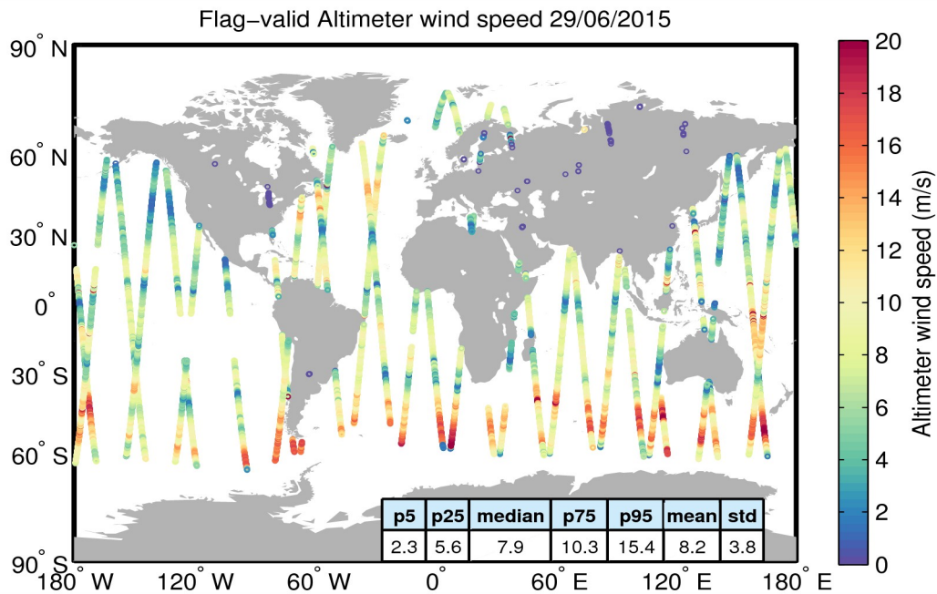
Figure 31. Geographical distribution of flag-valid wind data over oceans and lakes for 29/06/2015. The statistical values shown in the table refer to the wind in m/s and are calculated over all measurements shown in the figure.
