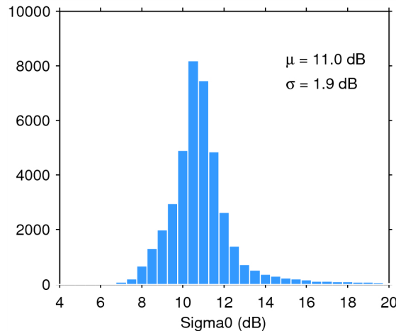
Figure 25. Histogram of flag-valid sigma0 over oceans and lakes for 29/06/2015. The mean ( \mu ) and standard deviation ( \sigma ) are also shown. Note that values outside [4 20] dB are excluded from the histogram for the sake of readability but not from the computation of \mu and \sigma .
