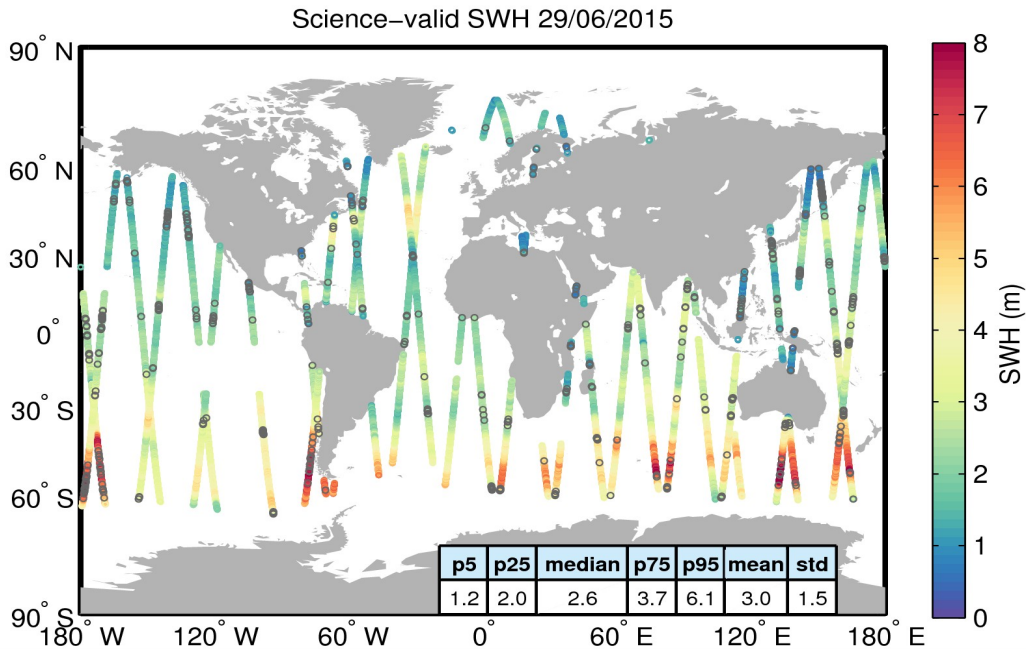
Figure 19. Geographical distribution of science-valid SWH data over oceans and lakes for 29/06/2015. The statistical values shown in the table refer to the SWH in m and are calculated over all measurements shown in the figure. Gray circles denote records that have been rejected based on the editing criteria described in Table 3.
