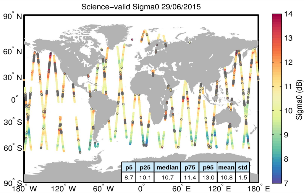
Figure 27. Geographical distribution of science-valid sigma0 data over oceans and lakes for 29/06/2015. The statistical values shown in the table refer to the sigma0 in dB and are calculated over all measurements shown in the figure. Gray circles denote records that have been rejected based on the editing criteria described in Table 4.
