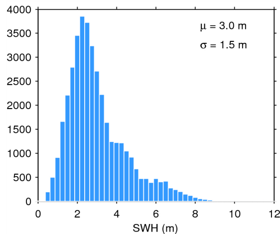
Figure 20. Histogram of science-valid SWH over oceans and lakes for 29/06/2015. The mean ( \mu ) and standard deviation ( \sigma ) are also shown. Note that values larger than 12 m are excluded from the histogram for the sake of readability but not from the computation of \mu and \sigma .
