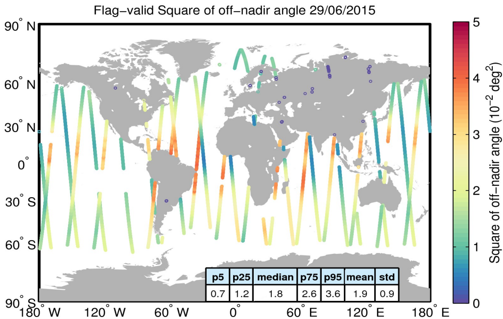
Figure 37. Geographical distribution of flag-valid mispointing data over oceans and lakes for 29/06/2015. The statistical values shown in the table refer to the mispointing in 10^{-2} \text{ deg}^2 and are calculated over all measurements shown in the figure.
