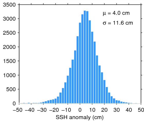
Figure 11. Histogram of science-valid SSH anomaly over oceans and lakes for 29/06/2015. The mean ( \mu ) and standard deviation ( \sigma ) are also shown. Note that values outside [-50 50] cm are excluded from the histogram for the sake of readability but not from the computation of \mu and \sigma .
