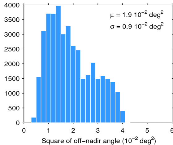
Figure 39. Histogram of flag-valid mispointing over oceans and lakes for 29/06/2015. The mean ( \mu ) and standard deviation ( \sigma ) are also shown. Note that values larger than 6 \cdot 10^{-2} \text{ deg}^2 are excluded from the histogram for the sake of readability but not from the computation of \mu and \sigma .
