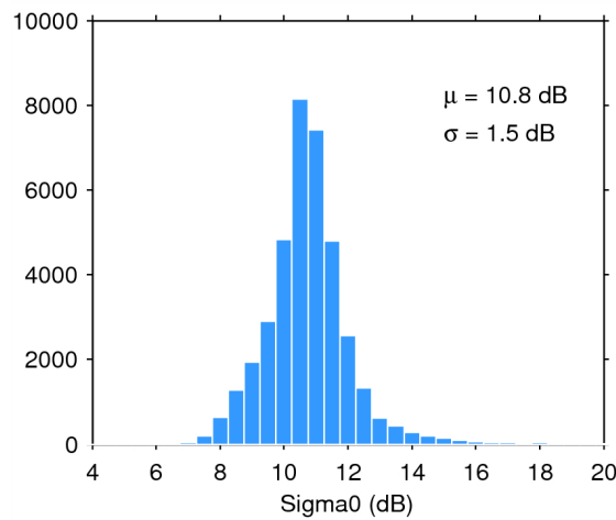
Figure 28. Histogram of science-valid sigma0 over oceans and lakes for 29/06/2015. The mean ( \mu ) and standard deviation ( \sigma ) are also shown. Note that values outside [4 20] dB are excluded from the histogram for the sake of readability but not from the computation of \mu and \sigma .
