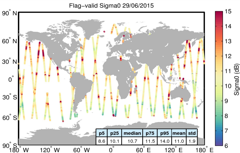
Figure 23. Geographical distribution of flag-valid sigma0 data over oceans and lakes for 29/06/2015. The statistical values shown in the table refer to the sigma0 in dB and are calculated over all measurements shown in the figure.
