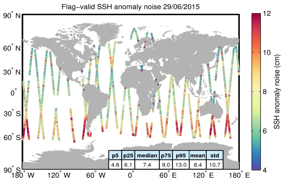
Figure 8. Geographical distribution of flag-valid 20-Hz SSH anomaly measurement noise over oceans and lakes for 29/06/2015. The statistical values shown in the table refer to the SSH anomaly noise and are calculated over all measurements shown in the figure.
