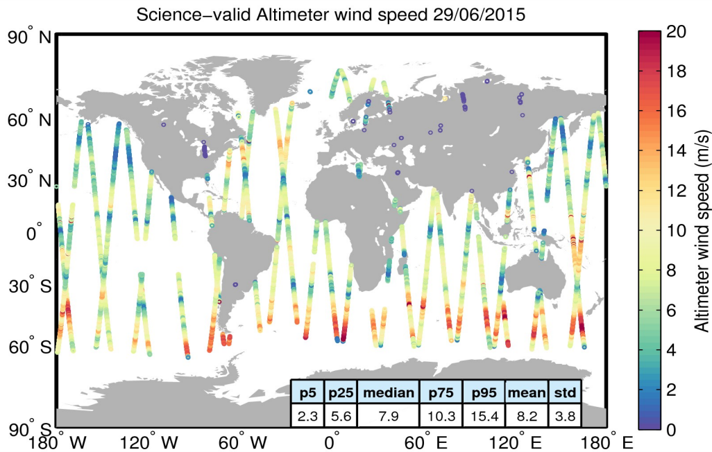
Figure 34. Geographical distribution of science-valid wind data over oceans and lakes for 29/06/2015. The statistical values shown in the table refer to the wind in m/s and are calculated over all measurements shown in the figure. Gray circles denote records that have been rejected based on the editing criteria described in Table 5.
