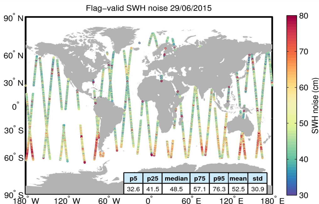
Figure 18. Geographical distribution of flag-valid 20-Hz SWH measurement noise over oceans and lakes for 29/06/2015. The statistical values shown in the figure refer to the SWH noise and are calculated over all measurements shown in the figure.
