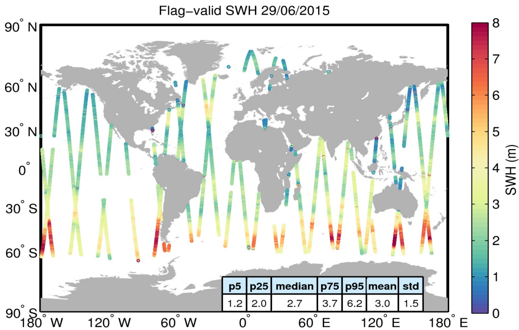
Figure 15. Geographical distribution of flag-valid SWH data over oceans and lakes for 29/06/2015. The statistical values shown in the table refer to the SWH in m and are calculated over all measurements shown in the figure.
