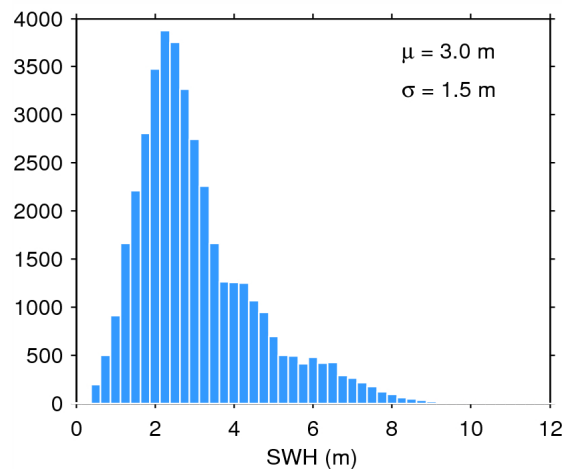
Figure 17. Histogram of flag-valid SWH over oceans and lakes for 29/06/2015. The mean ( \mu ) and standard deviation ( \sigma ) are also shown. Note that values larger than 12 m are excluded from the histogram for the sake of readability but not from the computation of \mu and \sigma .
