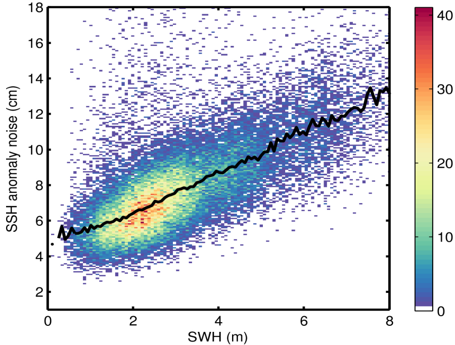
Figure 9. 2D histogram showing flag-valid SSH anomaly noise as a function of SWH for 29/06/2015. The black line denotes the median SSH anomaly as a function of SWH.
