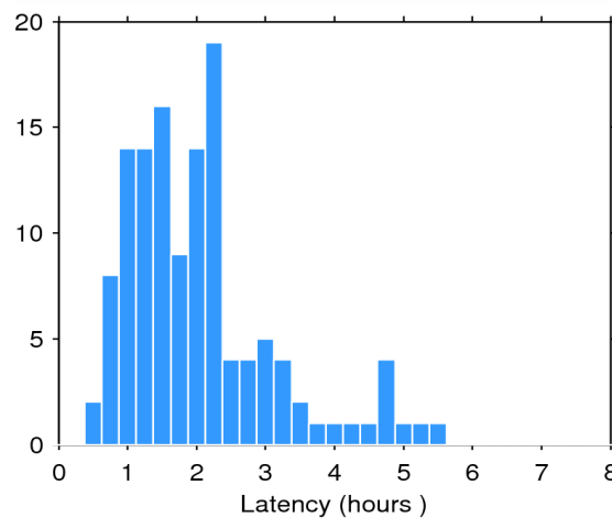
Figure 2. Histogram of the data latency for 29/06/2015. The y-axis denotes the number of files that are made available with a delay of x-hours with respect to the mean time of the records stored in the file.
