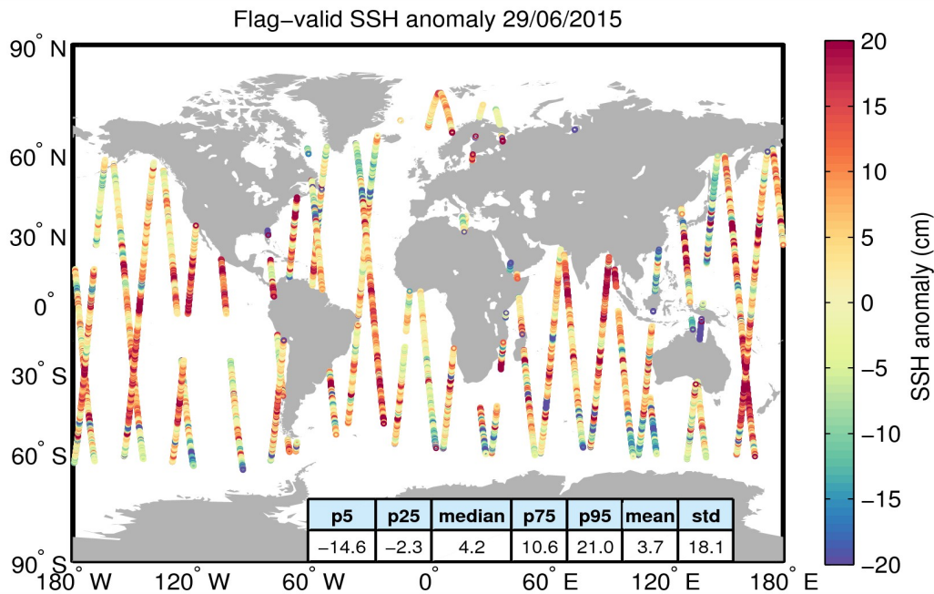
Figure 5. Geographical distribution of flag-valid 1-Hz SSH anomaly data over oceans and lakes for 29/06/2015. The statistical values shown in the table refer to the SSH anomaly in cm and are calculated over all measurements shown in the figure.
