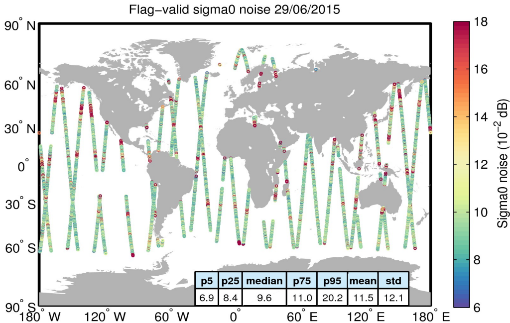
Figure 26. Geographical distribution of flag-valid 20-Hz sigma0 measurement noise over oceans and lakes for 29/06/2015. The statistical values shown in the table refer to the sigma0 noise and are calculated over all measurements shown in the figure.
