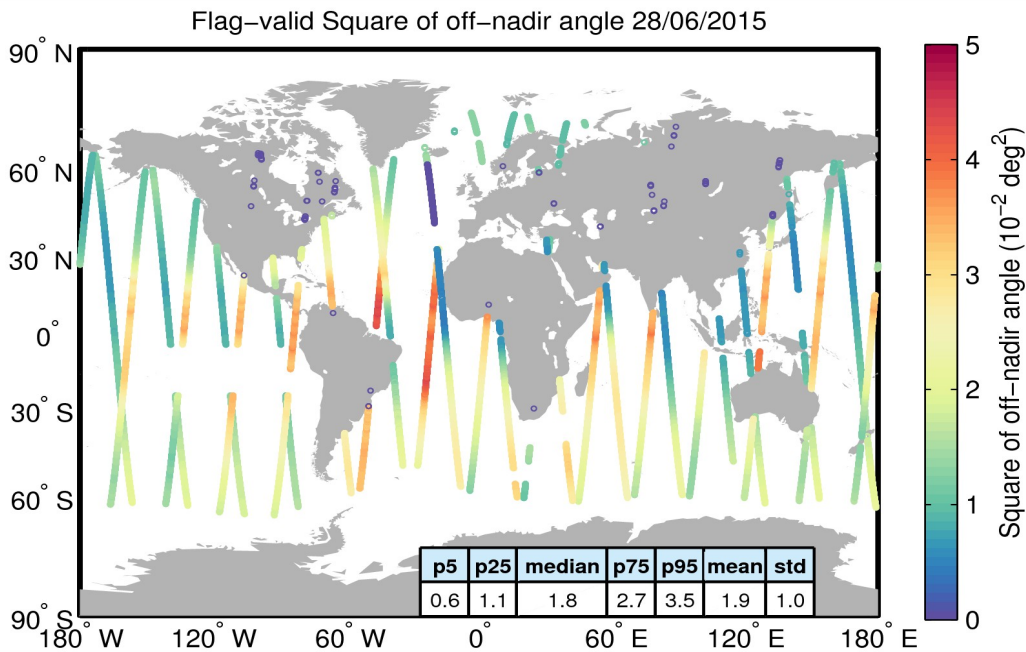
Figure 37. Geographical distribution of flag-valid mispointing data over oceans and lakes for 28/06/2015. The statistical values shown in the table refer to the mispointing in 10^{-2} \text{ deg}^2 and are calculated over all measurements shown in the figure.
