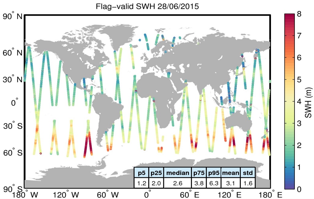
Figure 15. Geographical distribution of flag-valid SWH data over oceans and lakes for 28/06/2015. The statistical values shown in the table refer to the SWH in m and are calculated over all measurements shown in the figure.
