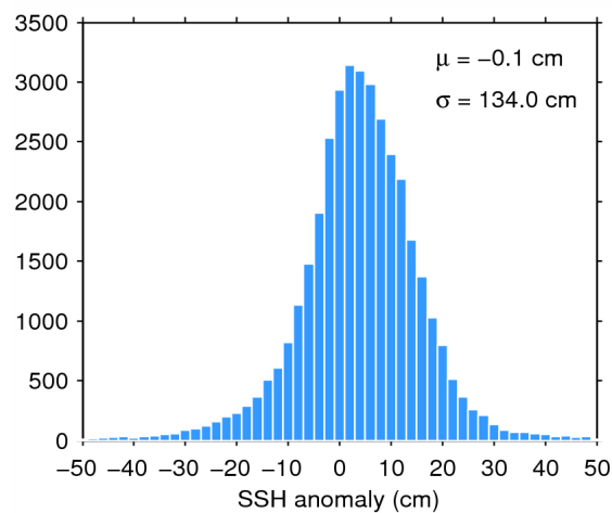
Figure 7. Histogram of flag-valid SSH anomaly over oceans and lakes for 28/06/2015. The mean ( \mu ) and standard deviation ( \sigma ) are also shown. Note that values outside [-50\ 50] cm are excluded from the histogram for the sake of readability but not from the computation of \mu and \sigma .
