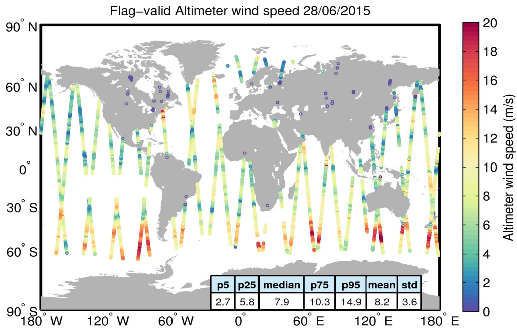
Figure 31. Geographical distribution of flag-valid wind data over oceans and lakes for 28/06/2015. The statistical values shown in the table refer to the wind in m/s and are calculated over all measurements shown in the figure.
