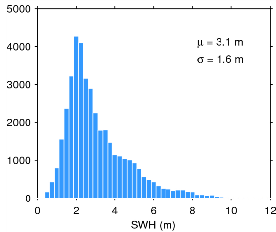
Figure 17. Histogram of flag-valid SWH over oceans and lakes for 28/06/2015. The mean ( \mu ) and standard deviation ( \sigma ) are also shown. Note that values larger than 12 m are excluded from the histogram for the sake of readability but not from the computation of \mu and \sigma .
