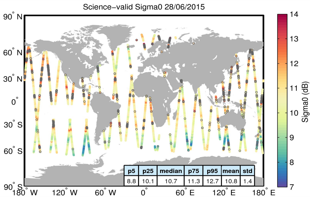
Figure 27. Geographical distribution of science-valid sigma0 data over oceans and lakes for 28/06/2015. The statistical values shown in the table refer to the sigma0 in dB and are calculated over all measurements shown in the figure. Gray circles denote records that have been rejected based on the editing criteria described in Table 4.
