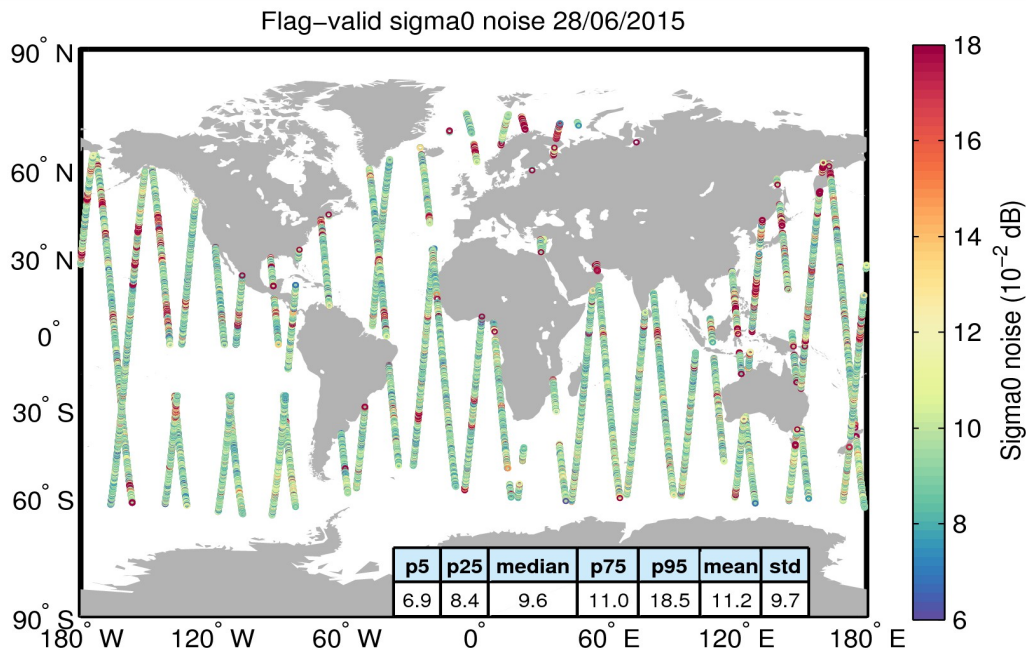
Figure 26. Geographical distribution of flag-valid 20-Hz sigma0 measurement noise over oceans and lakes for 28/06/2015. The statistical values shown in the table refer to the sigma0 noise and are calculated over all measurements shown in the figure.
