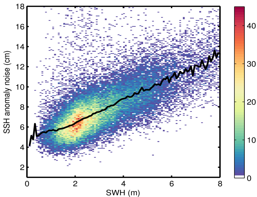
Figure 9. 2D histogram showing flag-valid SSH anomaly noise as a function of SWH for 28/06/2015. The black line denotes the median SSH anomaly as a function of SWH.
