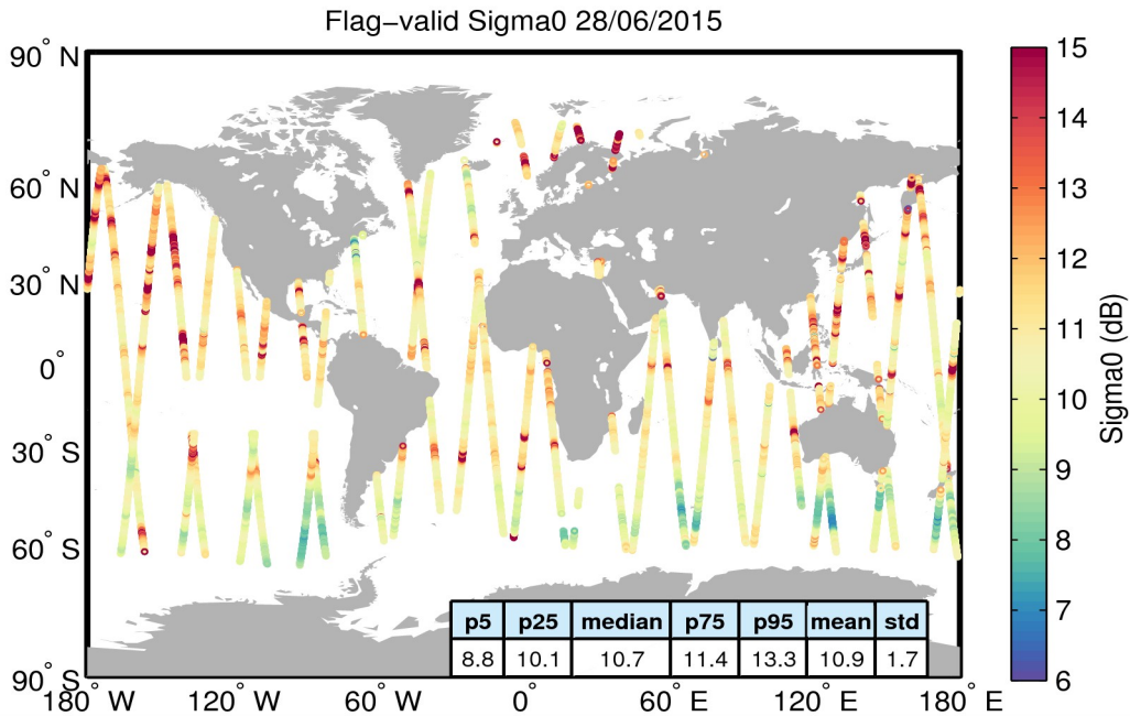
Figure 23. Geographical distribution of flag-valid sigma0 data over oceans and lakes for 28/06/2015. The statistical values shown in the table refer to the sigma0 in dB and are calculated over all measurements shown in the figure.
