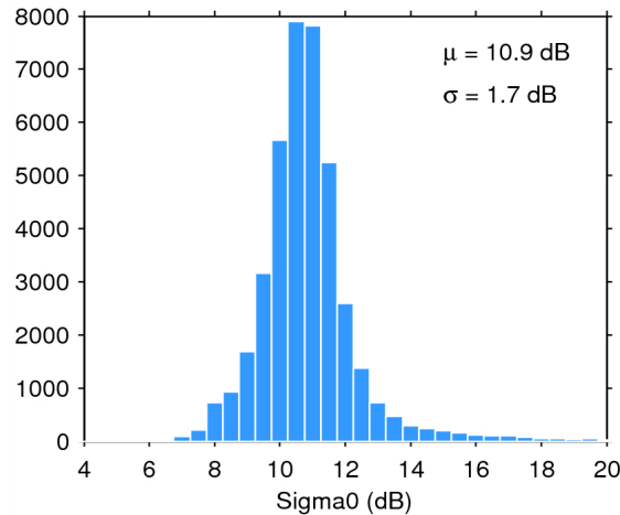
Figure 25. Histogram of flag-valid sigma0 over oceans and lakes for 28/06/2015. The mean ( \mu ) and standard deviation ( \sigma ) are also shown. Note that values outside [4 20] dB are excluded from the histogram for the sake of readability but not from the computation of \mu and \sigma .
