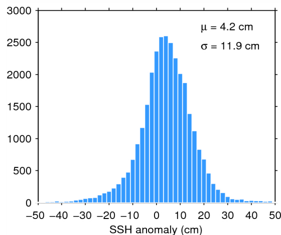
Figure 11. Histogram of science-valid SSH anomaly over oceans and lakes for 28/06/2015. The mean ( \mu ) and standard deviation ( \sigma ) are also shown. Note that values outside [-50 50] cm are excluded from the histogram for the sake of readability but not from the computation of \mu and \sigma .
