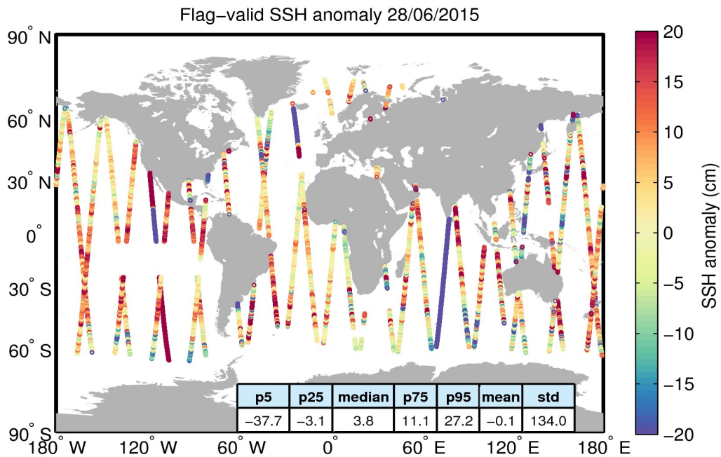
Figure 5. Geographical distribution of flag-valid 1-Hz SSH anomaly data over oceans and lakes for 28/06/2015. The statistical values shown in the table refer to the SSH anomaly in cm and are calculated over all measurements shown in the figure.
