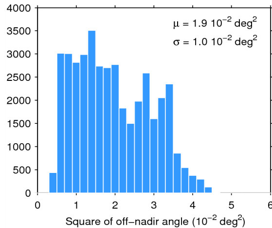
Figure 39. Histogram of flag-valid mispointing over oceans and lakes for 28/06/2015. The mean ( \mu ) and standard deviation ( \sigma ) are also shown. Note that values larger than 6 \cdot 10^{-2} \text{ deg}^2 are excluded from the histogram for the sake of readability but not from the computation of \mu and \sigma .
