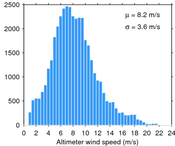
Figure 33. Histogram of flag-valid wind over oceans and lakes for 28/06/2015. The mean ( \mu ) and standard deviation ( \sigma ) are also shown. Note that values larger than 24 m/s are excluded from the histogram for the sake of readability but not from the computation of \mu and \sigma .
