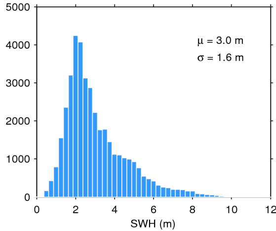
Figure 20. Histogram of science-valid SWH over oceans and lakes for 28/06/2015. The mean ( \mu ) and standard deviation ( \sigma ) are also shown. Note that values larger than 12 m are excluded from the histogram for the sake of readability but not from the computation of \mu and \sigma .
