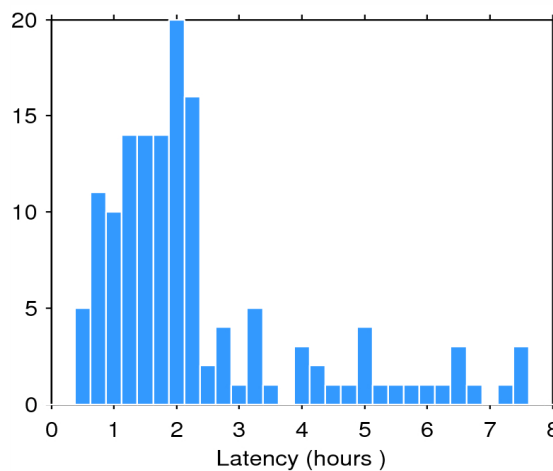
Figure 2. Histogram of the data latency for 28/06/2015. The y-axis denotes the number of files that are made available with a delay of x-hours with respect to the mean time of the records stored in the file.
