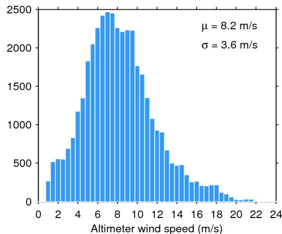
Figure 35. Histogram of science-valid wind over oceans and lakes for 28/06/2015. The mean ( \mu ) and standard deviation ( \sigma ) are also shown. Note that values larger than 24 m/s are excluded from the histogram for the sake of readability but not from the computation of \mu and \sigma .
