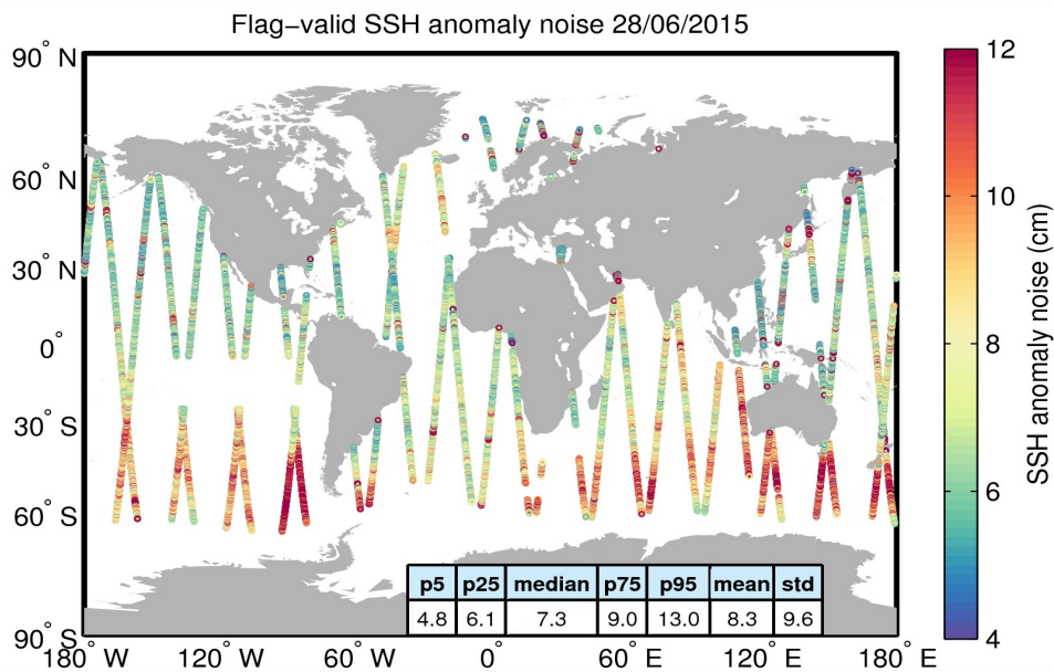
Figure 8. Geographical distribution of flag-valid 20-Hz SSH anomaly measurement noise over oceans and lakes for 28/06/2015. The statistical values shown in the table refer to the SSH anomaly noise and are calculated over all measurements shown in the figure.
