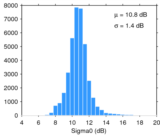
Figure 28. Histogram of science-valid sigma0 over oceans and lakes for 28/06/2015. The mean ( \mu ) and standard deviation ( \sigma ) are also shown. Note that values outside [4 20] dB are excluded from the histogram for the sake of readability but not from the computation of \mu and \sigma .
