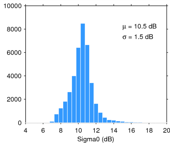
Figure 28. Histogram of science-valid sigma0 over oceans and lakes for 27/06/2015. The mean ( \mu ) and standard deviation ( \sigma ) are also shown. Note that values outside [4 20] dB are excluded from the histogram for the sake of readability but not from the computation of \mu and \sigma .
