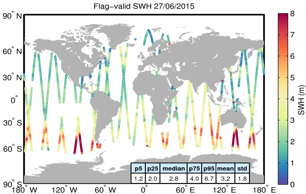
Figure 15. Geographical distribution of flag-valid SWH data over oceans and lakes for 27/06/2015. The statistical values shown in the table refer to the SWH in m and are calculated over all measurements shown in the figure.
