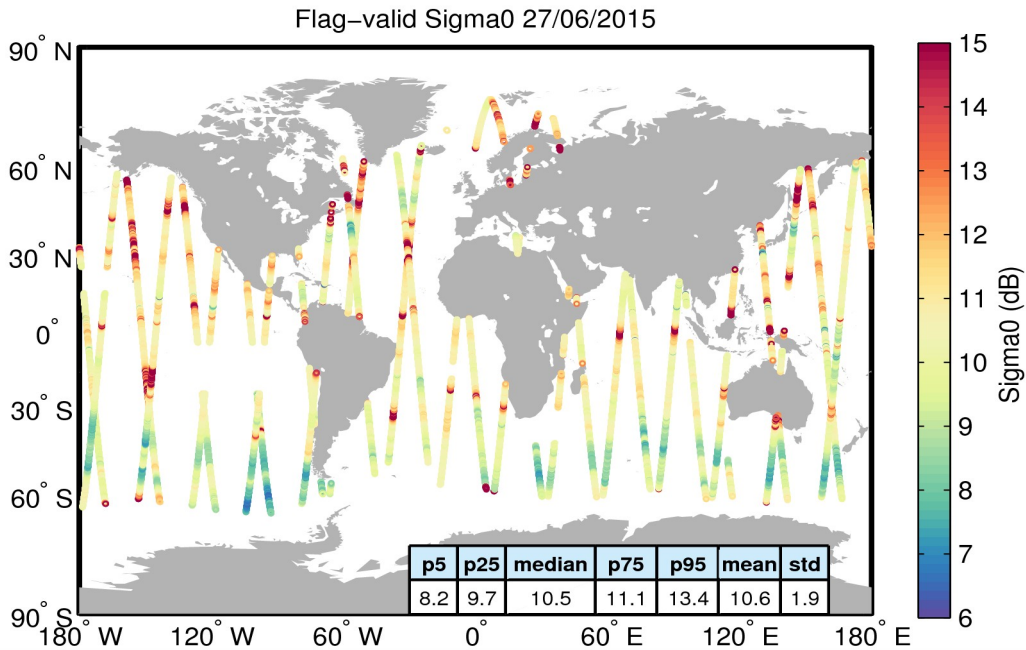
Figure 23. Geographical distribution of flag-valid sigma0 data over oceans and lakes for 27/06/2015. The statistical values shown in the table refer to the sigma0 in dB and are calculated over all measurements shown in the figure.
