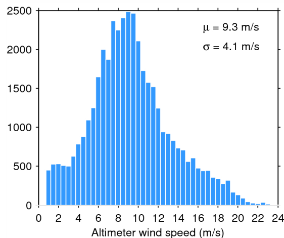
Figure 35. Histogram of science-valid wind over oceans and lakes for 27/06/2015. The mean ( \mu ) and standard deviation ( \sigma ) are also shown. Note that values larger than 24 m/s are excluded from the histogram for the sake of readability but not from the computation of \mu and \sigma .
