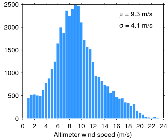
Figure 33. Histogram of flag-valid wind over oceans and lakes for 27/06/2015. The mean ( \mu ) and standard deviation ( \sigma ) are also shown. Note that values larger than 24 m/s are excluded from the histogram for the sake of readability but not from the computation of \mu and \sigma .
