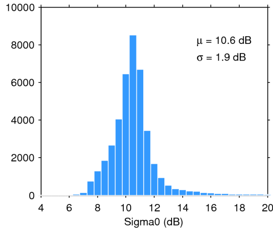
Figure 25. Histogram of flag-valid sigma0 over oceans and lakes for 27/06/2015. The mean ( \mu ) and standard deviation ( \sigma ) are also shown. Note that values outside [4 20] dB are excluded from the histogram for the sake of readability but not from the computation of \mu and \sigma .
