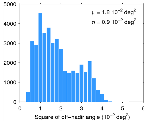
Figure 39. Histogram of flag-valid mispointing over oceans and lakes for 27/06/2015. The mean ( \mu ) and standard deviation ( \sigma ) are also shown. Note that values larger than 6 \cdot 10^{-2} \text{ deg}^2 are excluded from the histogram for the sake of readability but not from the computation of \mu and \sigma .
