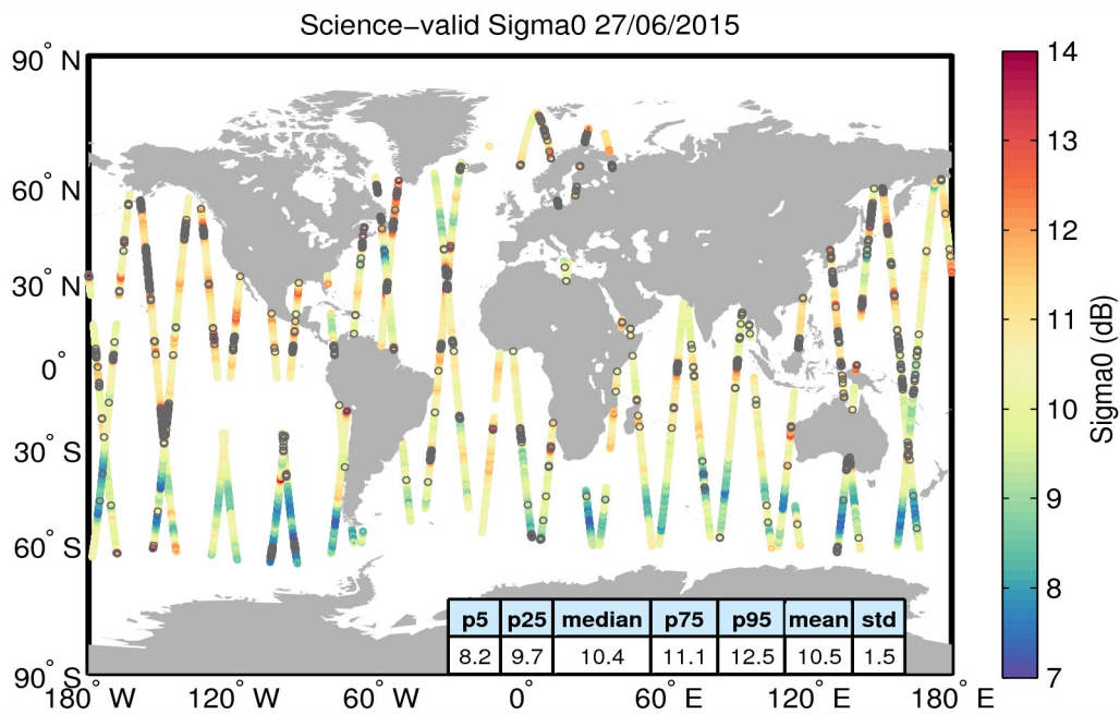
Figure 27. Geographical distribution of science-valid sigma0 data over oceans and lakes for 27/06/2015. The statistical values shown in the table refer to the sigma0 in dB and are calculated over all measurements shown in the figure. Gray circles denote records that have been rejected based on the editing criteria described in Table 4.
