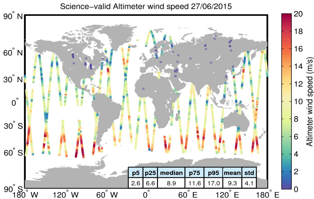
Figure 34. Geographical distribution of science-valid wind data over oceans and lakes for 27/06/2015. The statistical values shown in the table refer to the wind in m/s and are calculated over all measurements shown in the figure. Gray circles denote records that have been rejected based on the editing criteria described in Table 5.
