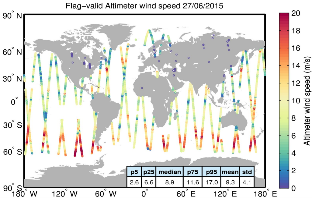
Figure 31. Geographical distribution of flag-valid wind data over oceans and lakes for 27/06/2015. The statistical values shown in the table refer to the wind in m/s and are calculated over all measurements shown in the figure.
