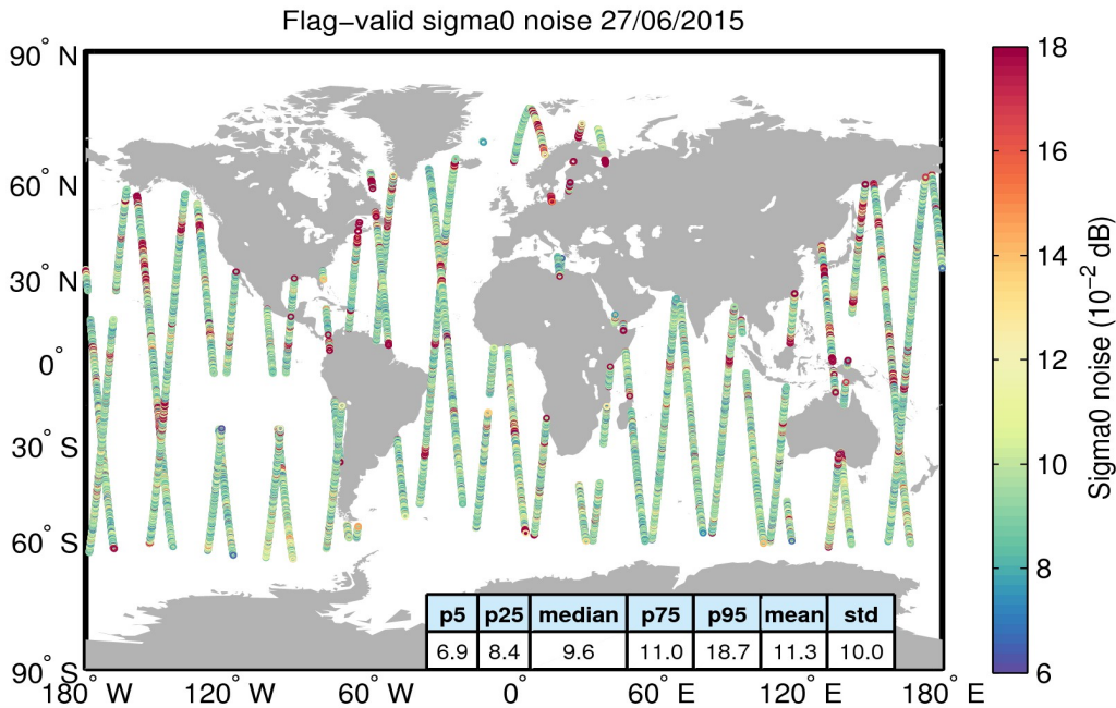
Figure 26. Geographical distribution of flag-valid 20-Hz sigma0 measurement noise over oceans and lakes for 27/06/2015. The statistical values shown in the table refer to the sigma0 noise and are calculated over all measurements shown in the figure.
