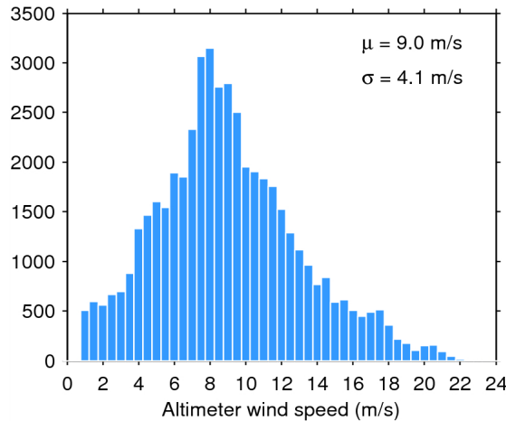
Figure 33. Histogram of flag-valid wind over oceans and lakes for 25/06/2015. The mean ( \mu ) and standard deviation ( \sigma ) are also shown. Note that values larger than 24 m/s are excluded from the histogram for the sake of readability but not from the computation of \mu and \sigma .
