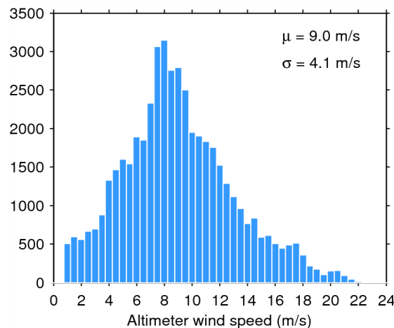
Figure 35. Histogram of science-valid wind over oceans and lakes for 25/06/2015. The mean ( \mu ) and standard deviation ( \sigma ) are also shown. Note that values larger than 24 m/s are excluded from the histogram for the sake of readability but not from the computation of \mu and \sigma .
