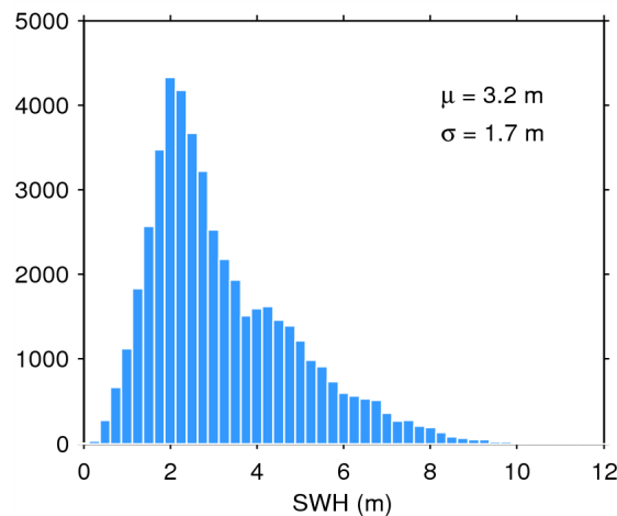
Figure 20. Histogram of science-valid SWH over oceans and lakes for 25/06/2015. The mean ( \mu ) and standard deviation ( \sigma ) are also shown. Note that values larger than 12 m are excluded from the histogram for the sake of readability but not from the computation of \mu and \sigma .
