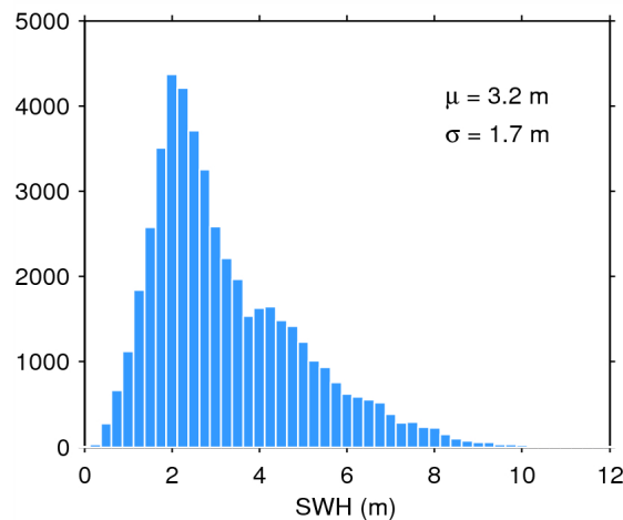
Figure 17. Histogram of flag-valid SWH over oceans and lakes for 25/06/2015. The mean ( \mu ) and standard deviation ( \sigma ) are also shown. Note that values larger than 12 m are excluded from the histogram for the sake of readability but not from the computation of \mu and \sigma .
