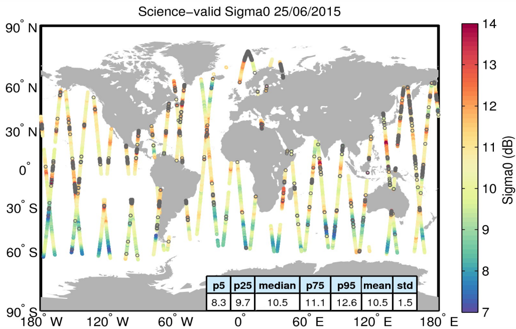
Figure 27. Geographical distribution of science-valid sigma0 data over oceans and lakes for 25/06/2015. The statistical values shown in the table refer to the sigma0 in dB and are calculated over all measurements shown in the figure. Gray circles denote records that have been rejected based on the editing criteria described in Table 4.
