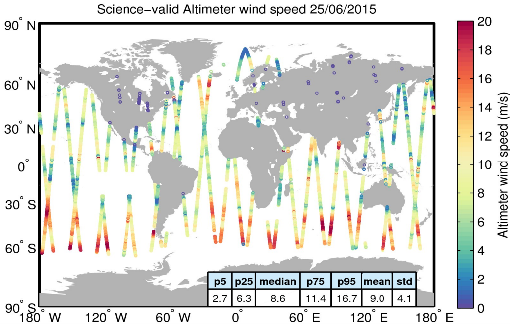
Figure 34. Geographical distribution of science-valid wind data over oceans and lakes for 25/06/2015. The statistical values shown in the table refer to the wind in m/s and are calculated over all measurements shown in the figure. Gray circles denote records that have been rejected based on the editing criteria described in Table 5.
