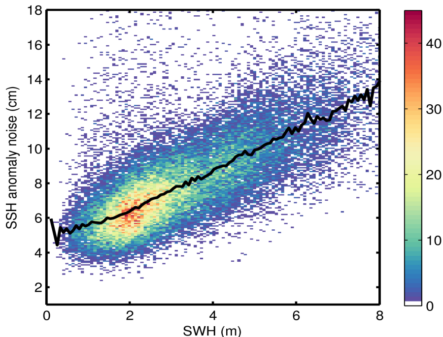
Figure 9. 2D histogram showing flag-valid SSH anomaly noise as a function of SWH for 25/06/2015. The black line denotes the median SSH anomaly as a function of SWH.
