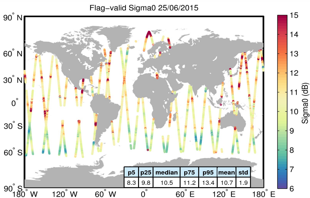
Figure 23. Geographical distribution of flag-valid sigma0 data over oceans and lakes for 25/06/2015. The statistical values shown in the table refer to the sigma0 in dB and are calculated over all measurements shown in the figure.
