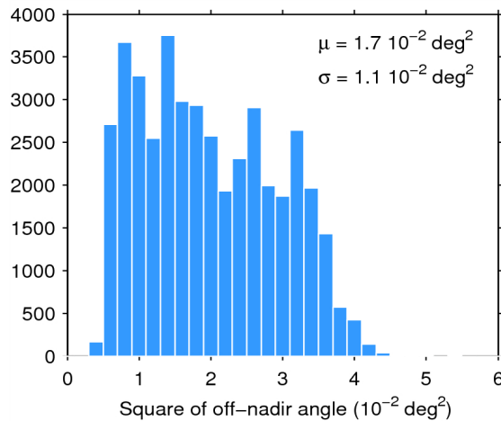
Figure 39. Histogram of flag-valid mispointing over oceans and lakes for 25/06/2015. The mean ( \mu ) and standard deviation ( \sigma ) are also shown. Note that values larger than 6 \cdot 10^{-2} \text{ deg}^2 are excluded from the histogram for the sake of readability but not from the computation of \mu and \sigma .
