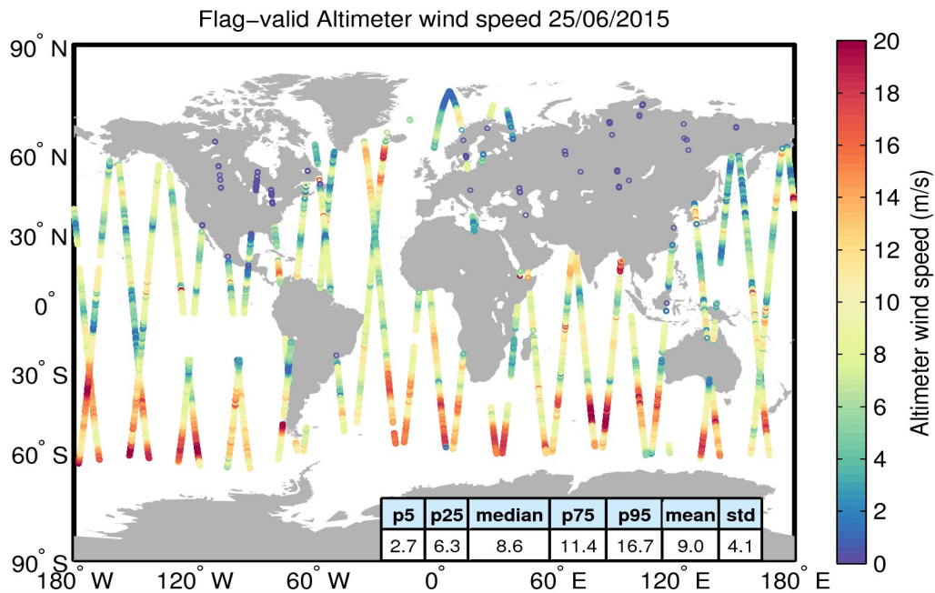
Figure 31. Geographical distribution of flag-valid wind data over oceans and lakes for 25/06/2015. The statistical values shown in the table refer to the wind in m/s and are calculated over all measurements shown in the figure.
