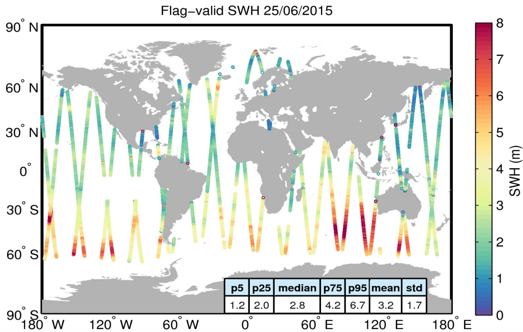
Figure 15. Geographical distribution of flag-valid SWH data over oceans and lakes for 25/06/2015. The statistical values shown in the table refer to the SWH in m and are calculated over all measurements shown in the figure.
