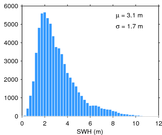
Figure 17. Histogram of flag-valid SWH over oceans and lakes for 24/06/2015. The mean ( \mu ) and standard deviation ( \sigma ) are also shown. Note that values larger than 12 m are excluded from the histogram for the sake of readability but not from the computation of \mu and \sigma .
