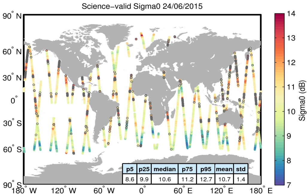
Figure 27. Geographical distribution of science-valid sigma0 data over oceans and lakes for 24/06/2015. The statistical values shown in the table refer to the sigma0 in dB and are calculated over all measurements shown in the figure. Gray circles denote records that have been rejected based on the editing criteria described in Table 4.
