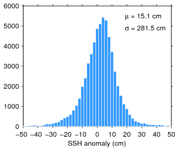
Figure 7. Histogram of flag-valid SSH anomaly over oceans and lakes for 24/06/2015. The mean ( \mu ) and standard deviation ( \sigma ) are also shown. Note that values outside [-50\ 50] cm are excluded from the histogram for the sake of readability but not from the computation of \mu and \sigma .
