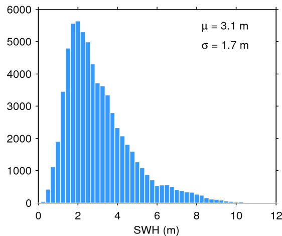
Figure 20. Histogram of science-valid SWH over oceans and lakes for 24/06/2015. The mean ( \mu ) and standard deviation ( \sigma ) are also shown. Note that values larger than 12 m are excluded from the histogram for the sake of readability but not from the computation of \mu and \sigma .
