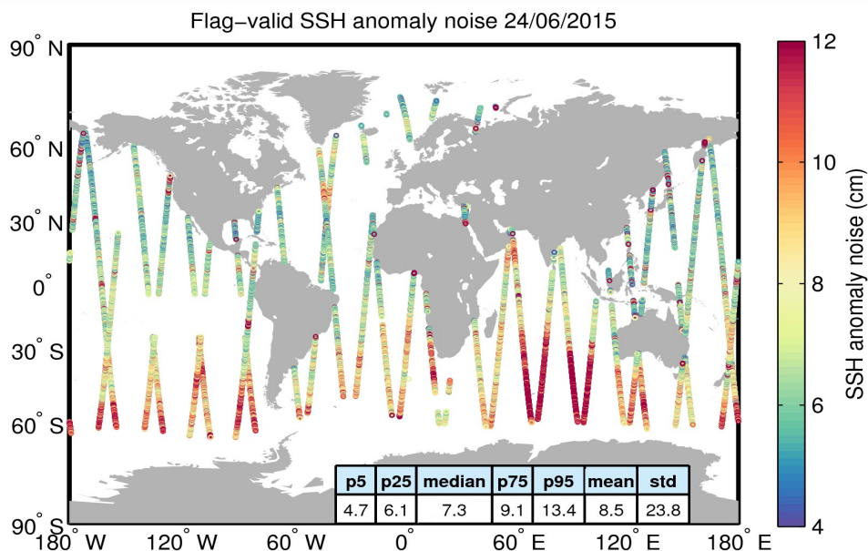
Figure 8. Geographical distribution of flag-valid 20-Hz SSH anomaly measurement noise over oceans and lakes for 24/06/2015. The statistical values shown in the table refer to the SSH anomaly noise and are calculated over all measurements shown in the figure.
