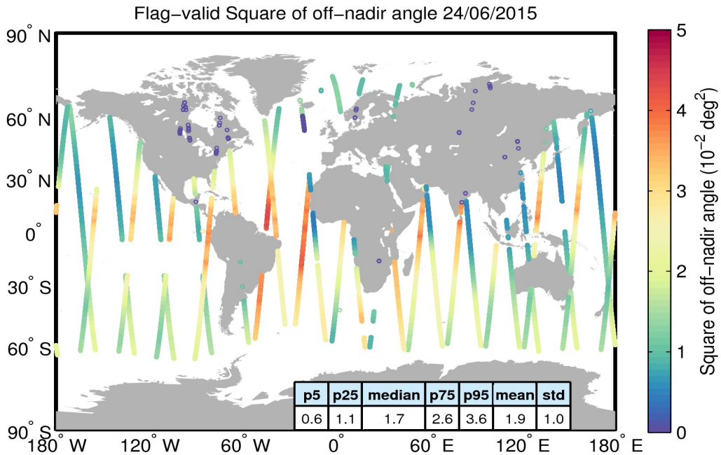
Figure 37. Geographical distribution of flag-valid mispointing data over oceans and lakes for 24/06/2015. The statistical values shown in the table refer to the mispointing in 10^{-2} \text{ deg}^2 and are calculated over all measurements shown in the figure.
