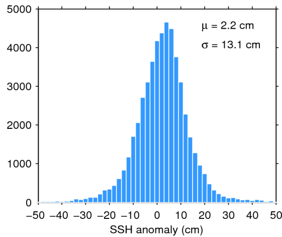
Figure 11. Histogram of science-valid SSH anomaly over oceans and lakes for 24/06/2015. The mean ( \mu ) and standard deviation ( \sigma ) are also shown. Note that values outside [-50 50] cm are excluded from the histogram for the sake of readability but not from the computation of \mu and \sigma .
