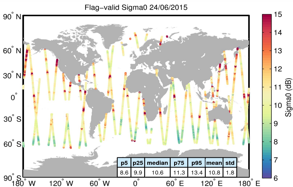
Figure 23. Geographical distribution of flag-valid sigma0 data over oceans and lakes for 24/06/2015. The statistical values shown in the table refer to the sigma0 in dB and are calculated over all measurements shown in the figure.
