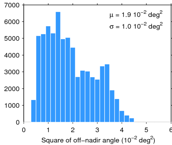
Figure 39. Histogram of flag-valid mispointing over oceans and lakes for 24/06/2015. The mean ( \mu ) and standard deviation ( \sigma ) are also shown. Note that values larger than 6 \cdot 10^{-2} \text{ deg}^2 are excluded from the histogram for the sake of readability but not from the computation of \mu and \sigma .
