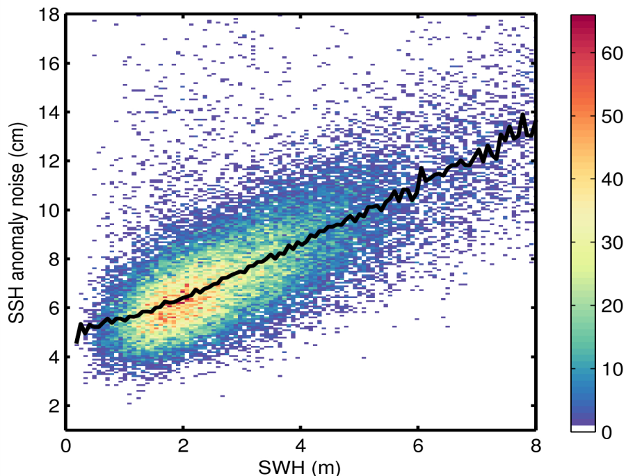
Figure 9. 2D histogram showing flag-valid SSH anomaly noise as a function of SWH for 24/06/2015. The black line denotes the median SSH anomaly as a function of SWH.
