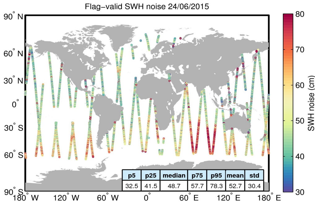
Figure 18. Geographical distribution of flag-valid 20-Hz SWH measurement noise over oceans and lakes for 24/06/2015. The statistical values shown in the figure refer to the SWH noise and are calculated over all measurements shown in the figure.
