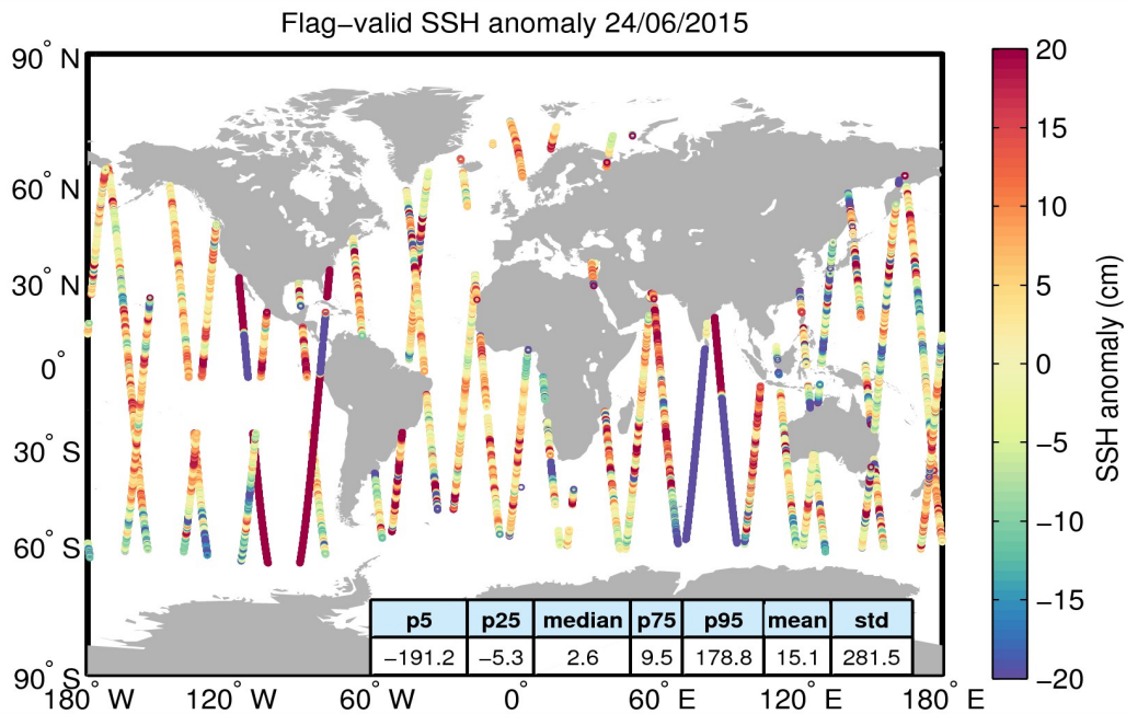
Figure 5. Geographical distribution of flag-valid 1-Hz SSH anomaly data over oceans and lakes for 24/06/2015. The statistical values shown in the table refer to the SSH anomaly in cm and are calculated over all measurements shown in the figure.
