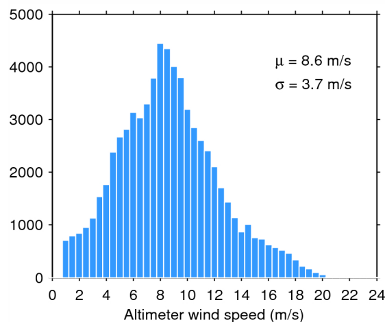
Figure 35. Histogram of science-valid wind over oceans and lakes for 24/06/2015. The mean ( \mu ) and standard deviation ( \sigma ) are also shown. Note that values larger than 24 m/s are excluded from the histogram for the sake of readability but not from the computation of \mu and \sigma .
