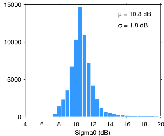
Figure 25. Histogram of flag-valid sigma0 over oceans and lakes for 24/06/2015. The mean ( \mu ) and standard deviation ( \sigma ) are also shown. Note that values outside [4 20] dB are excluded from the histogram for the sake of readability but not from the computation of \mu and \sigma .
