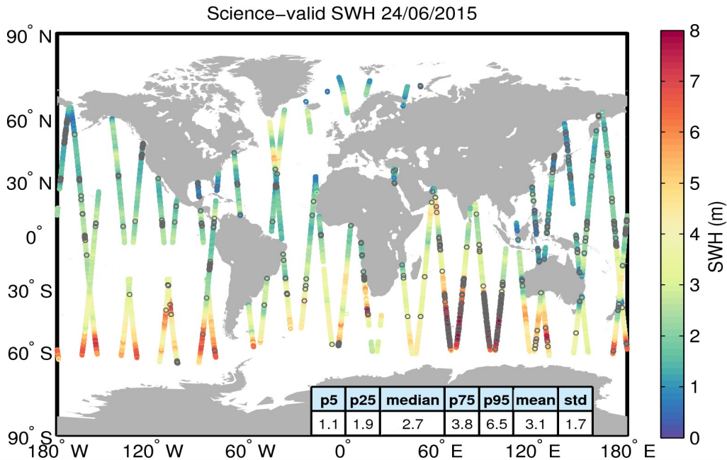
Figure 19. Geographical distribution of science-valid SWH data over oceans and lakes for 24/06/2015. The statistical values shown in the table refer to the SWH in m and are calculated over all measurements shown in the figure. Gray circles denote records that have been rejected based on the editing criteria described in Table 3.
