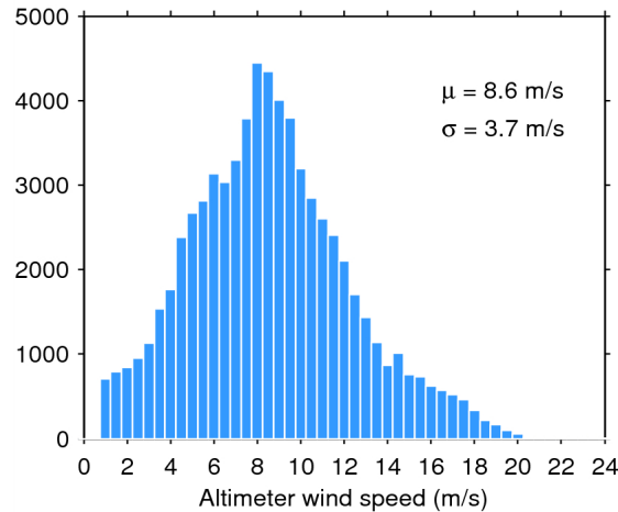
Figure 33. Histogram of flag-valid wind over oceans and lakes for 24/06/2015. The mean ( \mu ) and standard deviation ( \sigma ) are also shown. Note that values larger than 24 m/s are excluded from the histogram for the sake of readability but not from the computation of \mu and \sigma .
