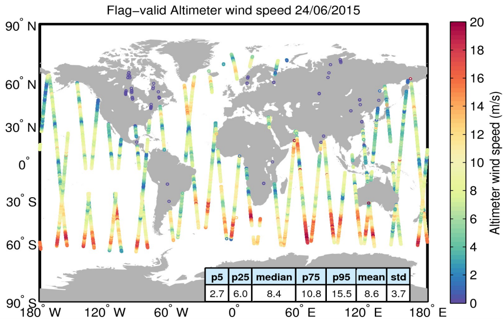
Figure 31. Geographical distribution of flag-valid wind data over oceans and lakes for 24/06/2015. The statistical values shown in the table refer to the wind in m/s and are calculated over all measurements shown in the figure.
