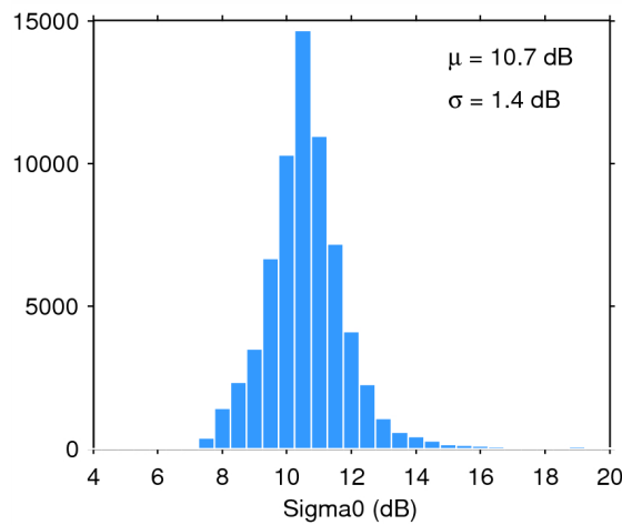
Figure 28. Histogram of science-valid sigma0 over oceans and lakes for 24/06/2015. The mean ( \mu ) and standard deviation ( \sigma ) are also shown. Note that values outside [4 20] dB are excluded from the histogram for the sake of readability but not from the computation of \mu and \sigma .
