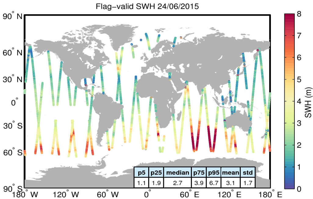
Figure 15. Geographical distribution of flag-valid SWH data over oceans and lakes for 24/06/2015. The statistical values shown in the table refer to the SWH in m and are calculated over all measurements shown in the figure.
