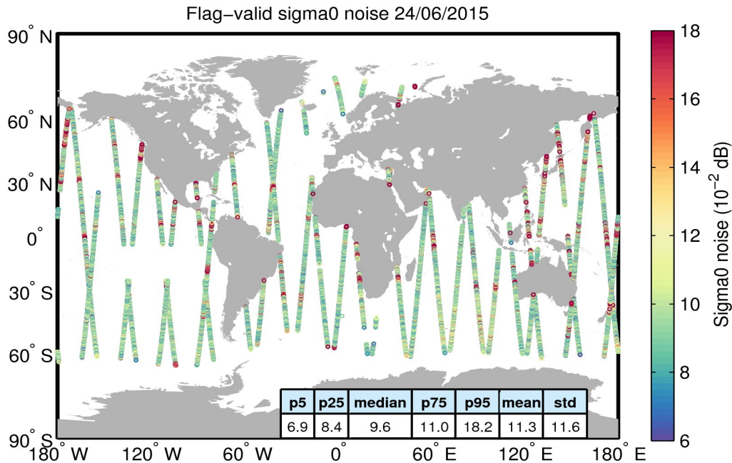
Figure 26. Geographical distribution of flag-valid 20-Hz sigma0 measurement noise over oceans and lakes for 24/06/2015. The statistical values shown in the table refer to the sigma0 noise and are calculated over all measurements shown in the figure.
