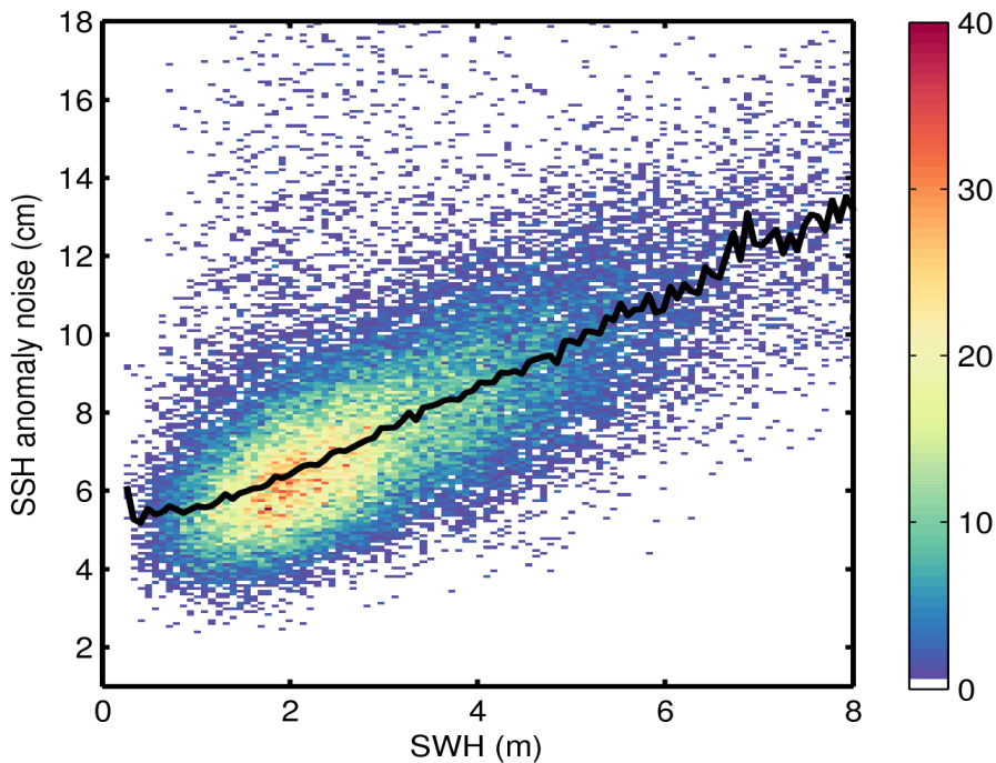
Figure 9. 2D histogram showing flag-valid SSH anomaly noise as a function of SWH for 23/06/2015. The black line denotes the median SSH anomaly as a function of SWH.
