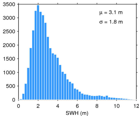
Figure 20. Histogram of science-valid SWH over oceans and lakes for 23/06/2015. The mean ( \mu ) and standard deviation ( \sigma ) are also shown. Note that values larger than 12 m are excluded from the histogram for the sake of readability but not from the computation of \mu and \sigma .
