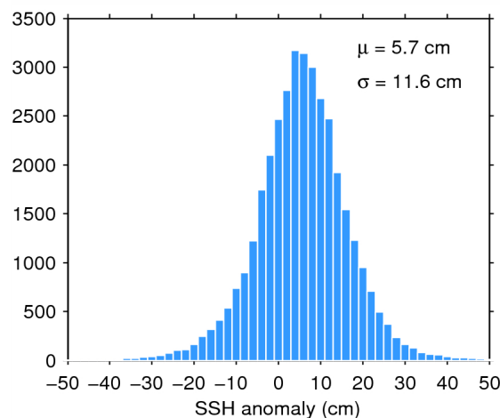
Figure 11. Histogram of science-valid SSH anomaly over oceans and lakes for 23/06/2015. The mean ( \mu ) and standard deviation ( \sigma ) are also shown. Note that values outside [-50 50] cm are excluded from the histogram for the sake of readability but not from the computation of \mu and \sigma .
