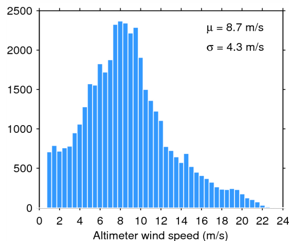
Figure 35. Histogram of science-valid wind over oceans and lakes for 23/06/2015. The mean ( \mu ) and standard deviation ( \sigma ) are also shown. Note that values larger than 24 m/s are excluded from the histogram for the sake of readability but not from the computation of \mu and \sigma .
