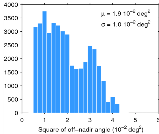
Figure 39. Histogram of flag-valid mispointing over oceans and lakes for 23/06/2015. The mean ( \mu ) and standard deviation ( \sigma ) are also shown. Note that values larger than 6 \cdot 10^{-2} \text{ deg}^2 are excluded from the histogram for the sake of readability but not from the computation of \mu and \sigma .
