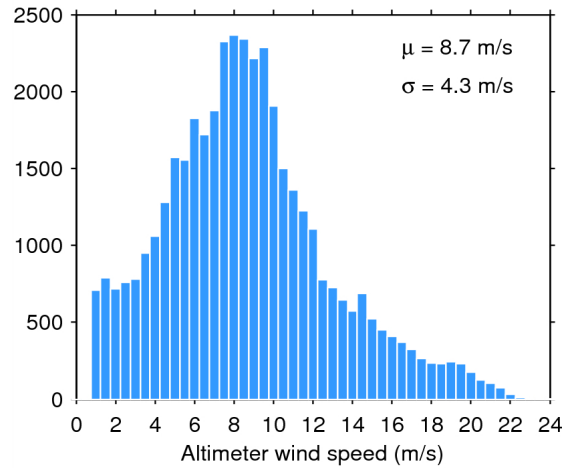
Figure 33. Histogram of flag-valid wind over oceans and lakes for 23/06/2015. The mean ( \mu ) and standard deviation ( \sigma ) are also shown. Note that values larger than 24 m/s are excluded from the histogram for the sake of readability but not from the computation of \mu and \sigma .
