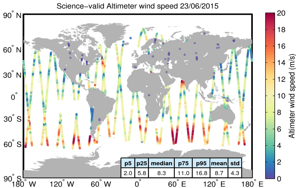
Figure 34. Geographical distribution of science-valid wind data over oceans and lakes for 23/06/2015. The statistical values shown in the table refer to the wind in m/s and are calculated over all measurements shown in the figure. Gray circles denote records that have been rejected based on the editing criteria described in Table 5.
