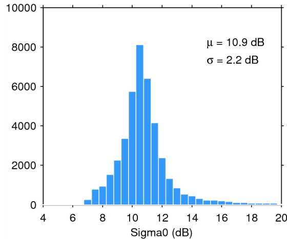
Figure 25. Histogram of flag-valid sigma0 over oceans and lakes for 23/06/2015. The mean ( \mu ) and standard deviation ( \sigma ) are also shown. Note that values outside [4 20] dB are excluded from the histogram for the sake of readability but not from the computation of \mu and \sigma .
