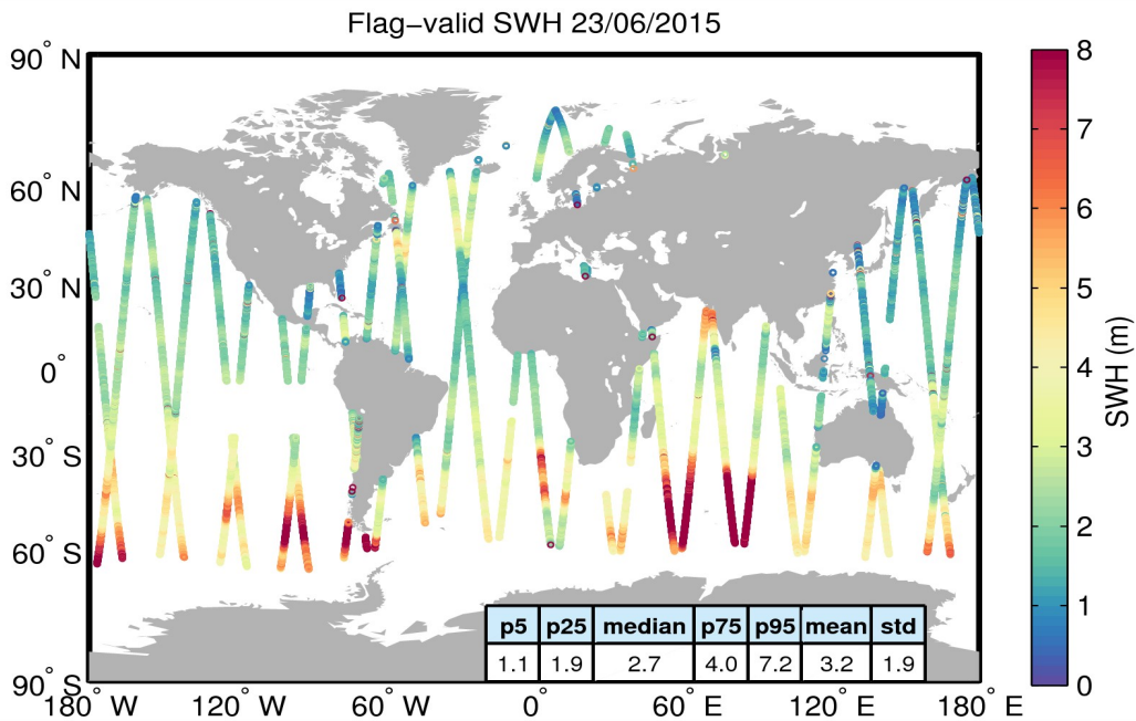
Figure 15. Geographical distribution of flag-valid SWH data over oceans and lakes for 23/06/2015. The statistical values shown in the table refer to the SWH in m and are calculated over all measurements shown in the figure.
