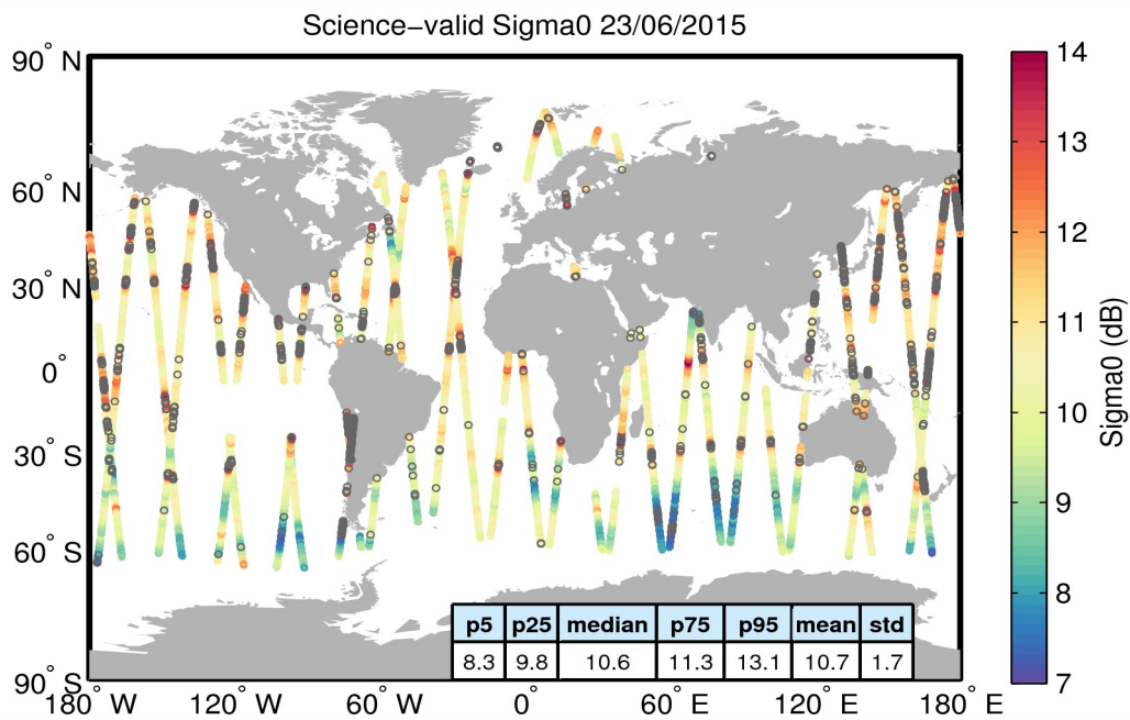
Figure 27. Geographical distribution of science-valid sigma0 data over oceans and lakes for 23/06/2015. The statistical values shown in the table refer to the sigma0 in dB and are calculated over all measurements shown in the figure. Gray circles denote records that have been rejected based on the editing criteria described in Table 4.
