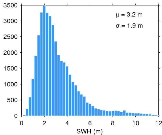
Figure 17. Histogram of flag-valid SWH over oceans and lakes for 23/06/2015. The mean ( \mu ) and standard deviation ( \sigma ) are also shown. Note that values larger than 12 m are excluded from the histogram for the sake of readability but not from the computation of \mu and \sigma .
