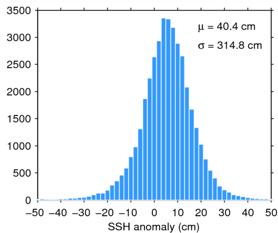
Figure 7. Histogram of flag-valid SSH anomaly over oceans and lakes for 23/06/2015. The mean ( \mu ) and standard deviation ( \sigma ) are also shown. Note that values outside [-50 50] cm are excluded from the histogram for the sake of readability but not from the computation of \mu and \sigma .
