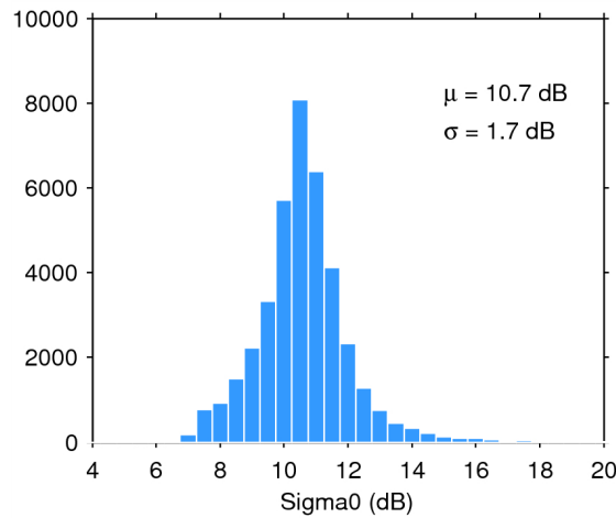
Figure 28. Histogram of science-valid sigma0 over oceans and lakes for 23/06/2015. The mean ( \mu ) and standard deviation ( \sigma ) are also shown. Note that values outside [4 20] dB are excluded from the histogram for the sake of readability but not from the computation of \mu and \sigma .
