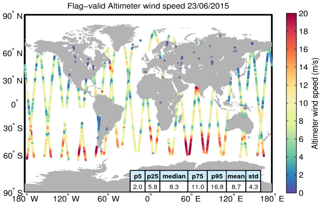
Figure 31. Geographical distribution of flag-valid wind data over oceans and lakes for 23/06/2015. The statistical values shown in the table refer to the wind in m/s and are calculated over all measurements shown in the figure.
