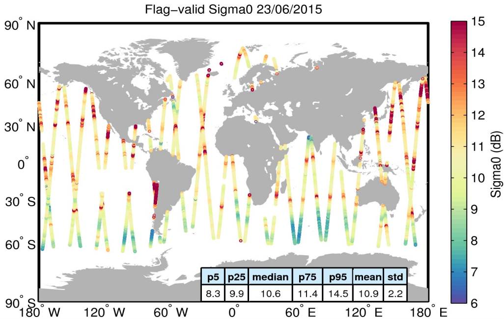
Figure 23. Geographical distribution of flag-valid sigma0 data over oceans and lakes for 23/06/2015. The statistical values shown in the table refer to the sigma0 in dB and are calculated over all measurements shown in the figure.
