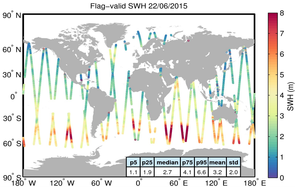
Figure 15. Geographical distribution of flag-valid SWH data over oceans and lakes for 22/06/2015. The statistical values shown in the table refer to the SWH in m and are calculated over all measurements shown in the figure.
