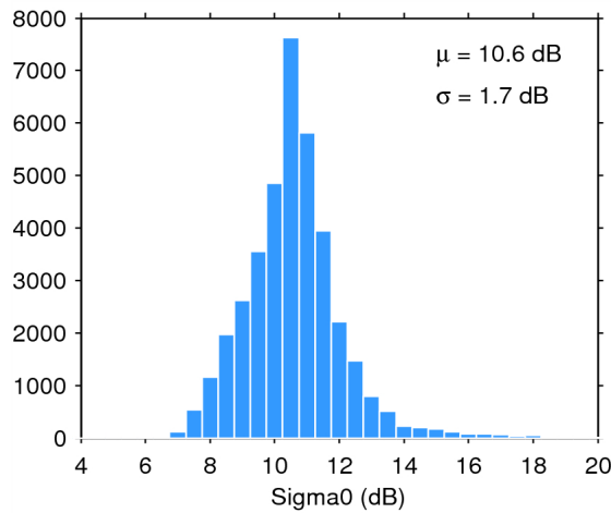
Figure 28. Histogram of science-valid sigma0 over oceans and lakes for 22/06/2015. The mean ( \mu ) and standard deviation ( \sigma ) are also shown. Note that values outside [4 20] dB are excluded from the histogram for the sake of readability but not from the computation of \mu and \sigma .
