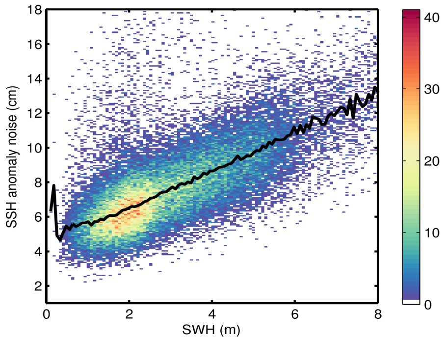
Figure 9. 2D histogram showing flag-valid SSH anomaly noise as a function of SWH for 22/06/2015. The black line denotes the median SSH anomaly as a function of SWH.
