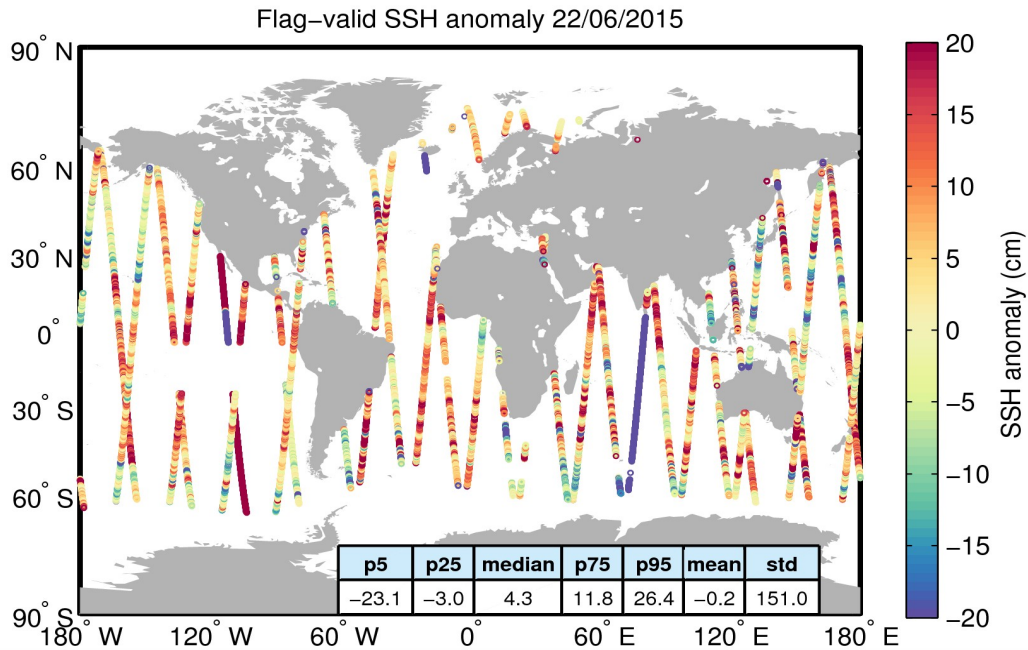
Figure 5. Geographical distribution of flag-valid 1-Hz SSH anomaly data over oceans and lakes for 22/06/2015. The statistical values shown in the table refer to the SSH anomaly in cm and are calculated over all measurements shown in the figure.
