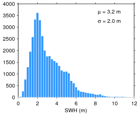
Figure 17. Histogram of flag-valid SWH over oceans and lakes for 22/06/2015. The mean ( \mu ) and standard deviation ( \sigma ) are also shown. Note that values larger than 12 m are excluded from the histogram for the sake of readability but not from the computation of \mu and \sigma .
