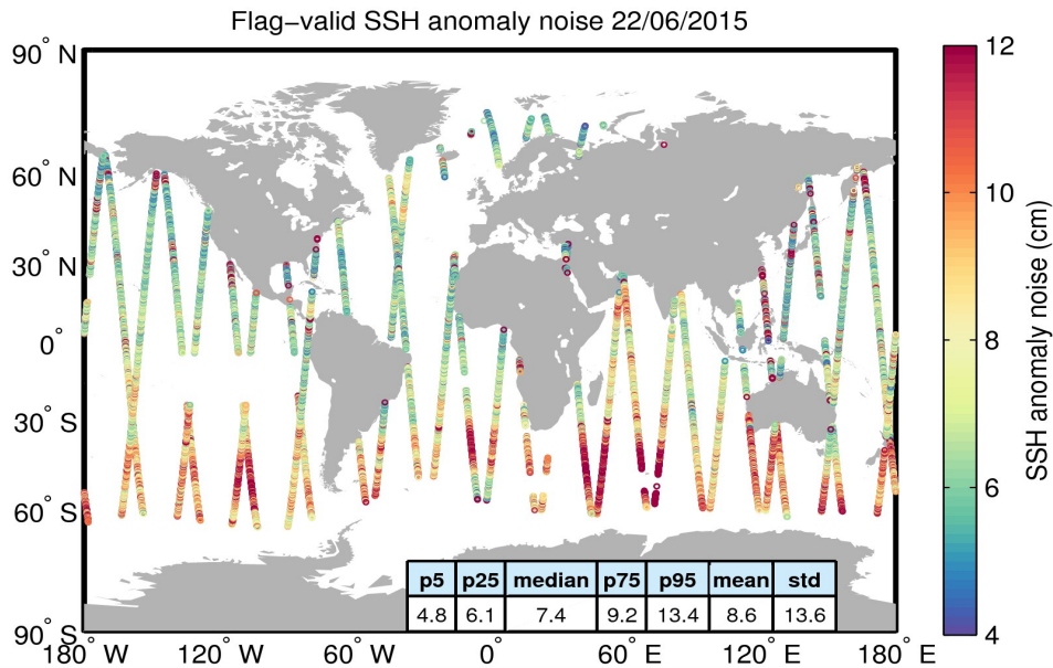
Figure 8. Geographical distribution of flag-valid 20-Hz SSH anomaly measurement noise over oceans and lakes for 22/06/2015. The statistical values shown in the table refer to the SSH anomaly noise and are calculated over all measurements shown in the figure.
