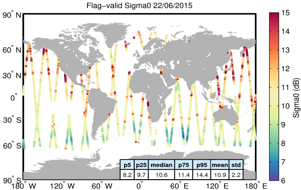
Figure 23. Geographical distribution of flag-valid sigma0 data over oceans and lakes for 22/06/2015. The statistical values shown in the table refer to the sigma0 in dB and are calculated over all measurements shown in the figure.
