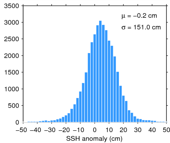
Figure 7. Histogram of flag-valid SSH anomaly over oceans and lakes for 22/06/2015. The mean ( \mu ) and standard deviation ( \sigma ) are also shown. Note that values outside [-50 50] cm are excluded from the histogram for the sake of readability but not from the computation of \mu and \sigma .
