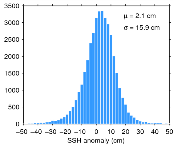
Figure 7. Histogram of flag-valid SSH anomaly over oceans and lakes for 21/06/2015. The mean ( \mu ) and standard deviation ( \sigma ) are also shown. Note that values outside [-50\ 50] cm are excluded from the histogram for the sake of readability but not from the computation of \mu and \sigma .
