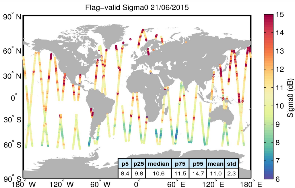
Figure 23. Geographical distribution of flag-valid sigma0 data over oceans and lakes for 21/06/2015. The statistical values shown in the table refer to the sigma0 in dB and are calculated over all measurements shown in the figure.
