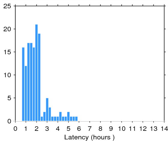
Figure 2. Histogram of the data latency for 21/06/2015. The y-axis denotes the number of files that are made available with a delay of x-hours with respect to the mean time of the records stored in the file.
