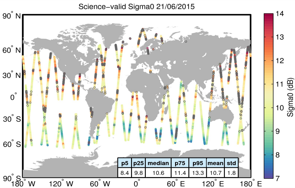
Figure 27. Geographical distribution of science-valid sigma0 data over oceans and lakes for 21/06/2015. The statistical values shown in the table refer to the sigma0 in dB and are calculated over all measurements shown in the figure. Gray circles denote records that have been rejected based on the editing criteria described in Table 4.
