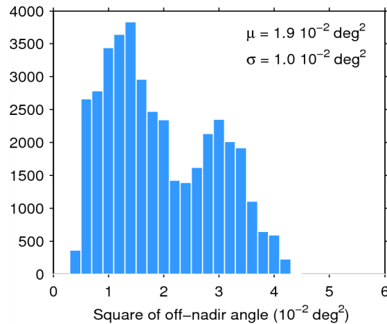
Figure 39. Histogram of flag-valid mispointing over oceans and lakes for 21/06/2015. The mean ( \mu ) and standard deviation ( \sigma ) are also shown. Note that values larger than 6 \cdot 10^{-2} \text{ deg}^2 are excluded from the histogram for the sake of readability but not from the computation of \mu and \sigma .
