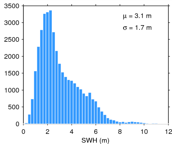
Figure 17. Histogram of flag-valid SWH over oceans and lakes for 21/06/2015. The mean ( \mu ) and standard deviation ( \sigma ) are also shown. Note that values larger than 12 m are excluded from the histogram for the sake of readability but not from the computation of \mu and \sigma .
