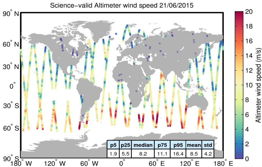
Figure 34. Geographical distribution of science-valid wind data over oceans and lakes for 21/06/2015. The statistical values shown in the table refer to the wind in m/s and are calculated over all measurements shown in the figure. Gray circles denote records that have been rejected based on the editing criteria described in Table 5.
