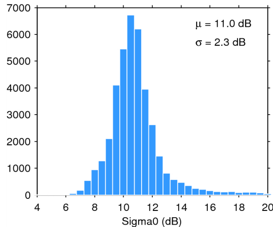
Figure 25. Histogram of flag-valid sigma0 over oceans and lakes for 21/06/2015. The mean ( \mu ) and standard deviation ( \sigma ) are also shown. Note that values outside [4 20] dB are excluded from the histogram for the sake of readability but not from the computation of \mu and \sigma .
