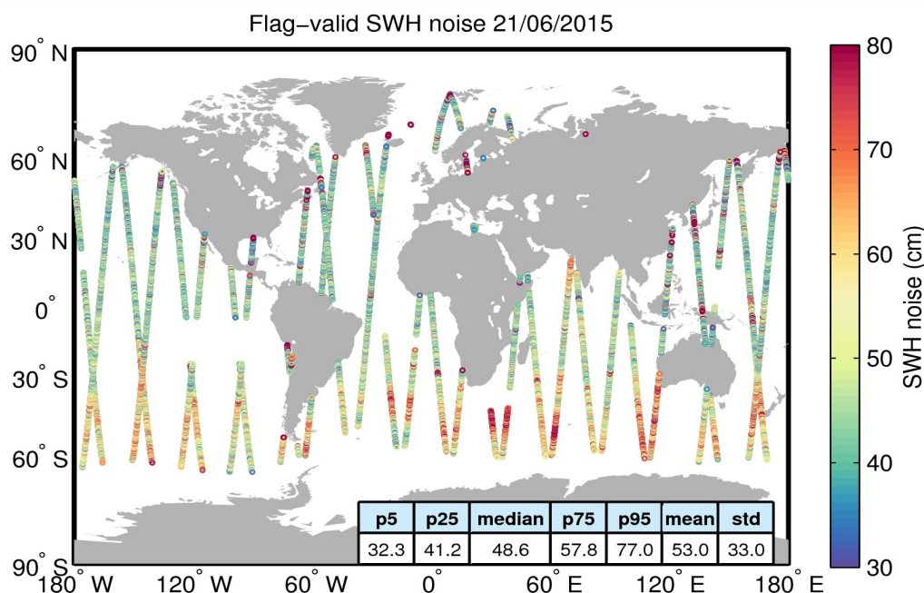
Figure 18. Geographical distribution of flag-valid 20-Hz SWH measurement noise over oceans and lakes for 21/06/2015. The statistical values shown in the figure refer to the SWH noise and are calculated over all measurements shown in the figure.
