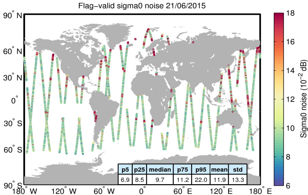
Figure 26. Geographical distribution of flag-valid 20-Hz sigma0 measurement noise over oceans and lakes for 21/06/2015. The statistical values shown in the table refer to the sigma0 noise and are calculated over all measurements shown in the figure.
