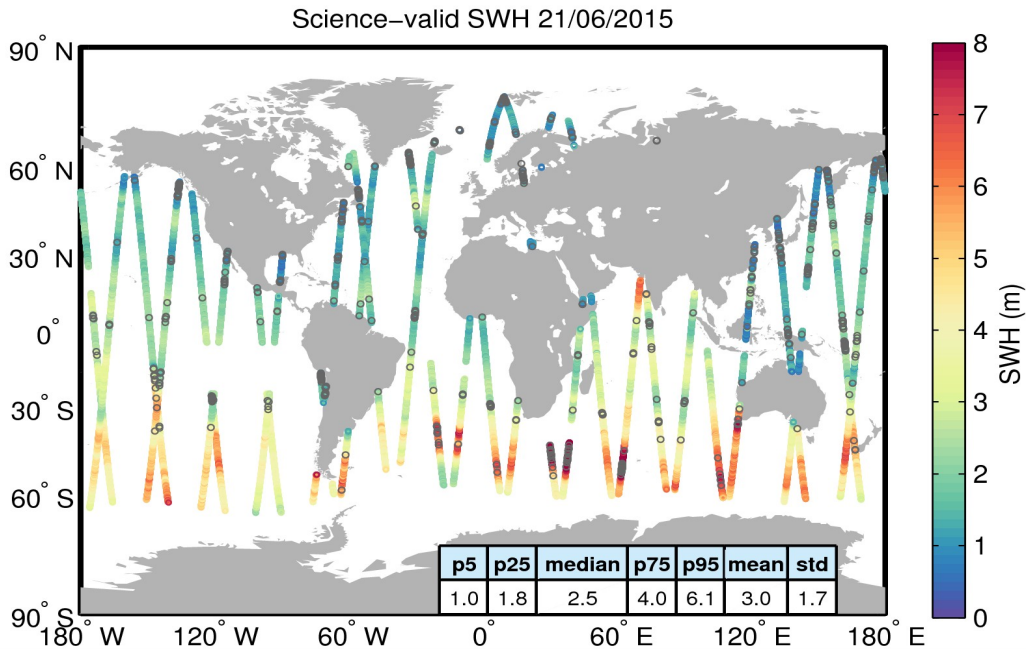
Figure 19. Geographical distribution of science-valid SWH data over oceans and lakes for 21/06/2015. The statistical values shown in the table refer to the SWH in m and are calculated over all measurements shown in the figure. Gray circles denote records that have been rejected based on the editing criteria described in Table 3.
