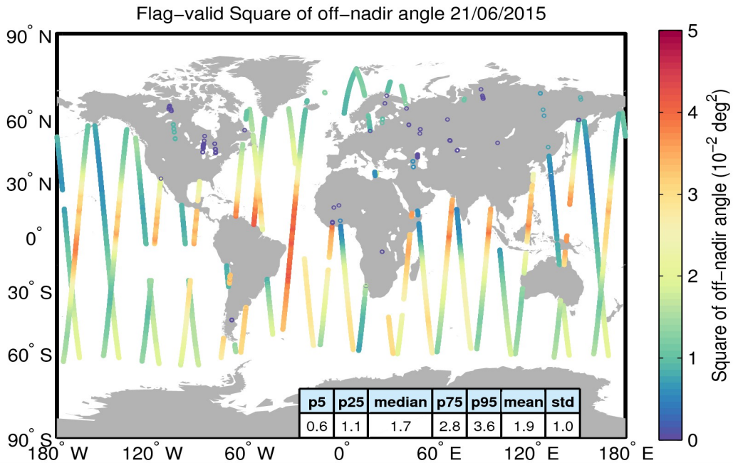
Figure 37. Geographical distribution of flag-valid mispointing data over oceans and lakes for 21/06/2015. The statistical values shown in the table refer to the mispointing in 10^{-2} \text{ deg}^2 and are calculated over all measurements shown in the figure.
