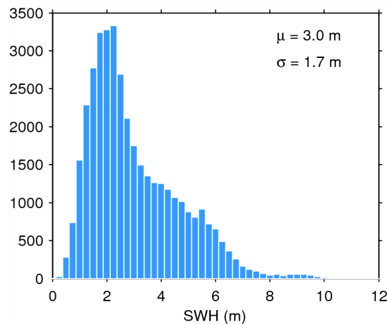
Figure 20. Histogram of science-valid SWH over oceans and lakes for 21/06/2015. The mean ( \mu ) and standard deviation ( \sigma ) are also shown. Note that values larger than 12 m are excluded from the histogram for the sake of readability but not from the computation of \mu and \sigma .
