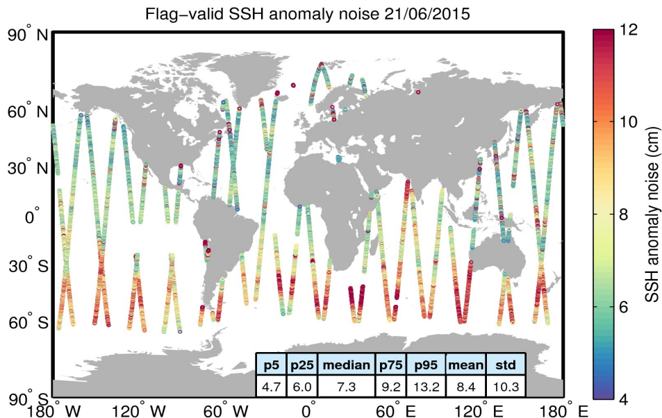
Figure 8. Geographical distribution of flag-valid 20-Hz SSH anomaly measurement noise over oceans and lakes for 21/06/2015. The statistical values shown in the table refer to the SSH anomaly noise and are calculated over all measurements shown in the figure.
