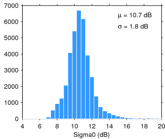
Figure 28. Histogram of science-valid sigma0 over oceans and lakes for 21/06/2015. The mean ( \mu ) and standard deviation ( \sigma ) are also shown. Note that values outside [4 20] dB are excluded from the histogram for the sake of readability but not from the computation of \mu and \sigma .
