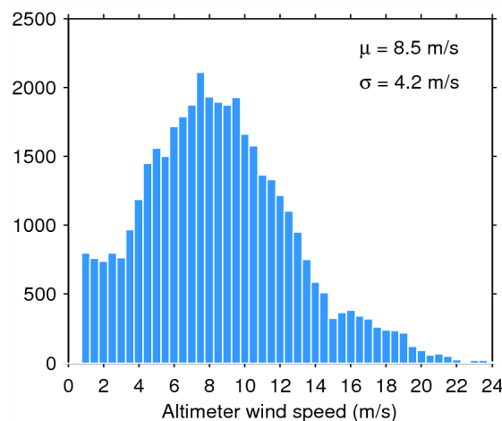
Figure 35. Histogram of science-valid wind over oceans and lakes for 21/06/2015. The mean ( \mu ) and standard deviation ( \sigma ) are also shown. Note that values larger than 24 m/s are excluded from the histogram for the sake of readability but not from the computation of \mu and \sigma .
