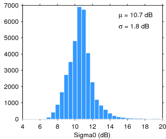
Figure 28. Histogram of science-valid sigma0 over oceans and lakes for 20/06/2015. The mean ( \mu ) and standard deviation ( \sigma ) are also shown. Note that values outside [4 20] dB are excluded from the histogram for the sake of readability but not from the computation of \mu and \sigma .
