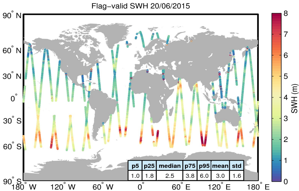
Figure 15. Geographical distribution of flag-valid SWH data over oceans and lakes for 20/06/2015. The statistical values shown in the table refer to the SWH in m and are calculated over all measurements shown in the figure.
