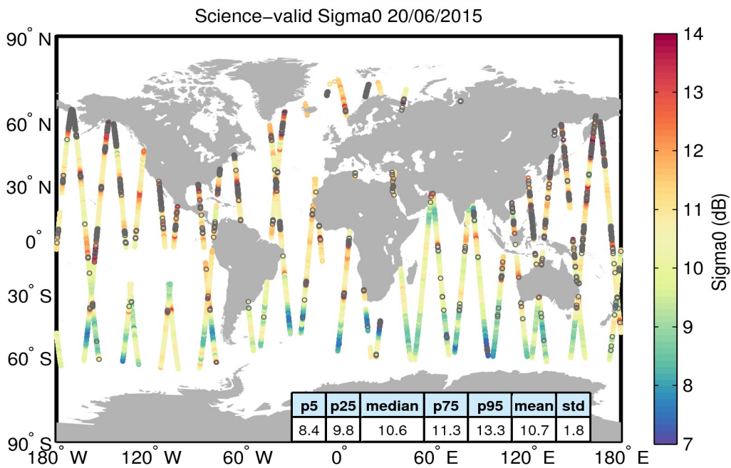
Figure 27. Geographical distribution of science-valid sigma0 data over oceans and lakes for 20/06/2015. The statistical values shown in the table refer to the sigma0 in dB and are calculated over all measurements shown in the figure. Gray circles denote records that have been rejected based on the editing criteria described in Table 4.
