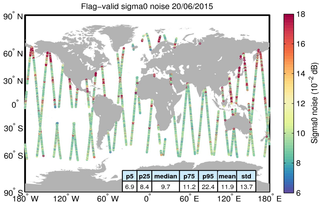
Figure 26. Geographical distribution of flag-valid 20-Hz sigma0 measurement noise over oceans and lakes for 20/06/2015. The statistical values shown in the table refer to the sigma0 noise and are calculated over all measurements shown in the figure.
