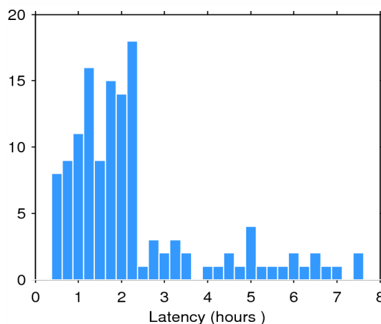
Figure 2. Histogram of the data latency for 20/06/2015. The y-axis denotes the number of files that are made available with a delay of x-hours with respect to the mean time of the records stored in the file.
