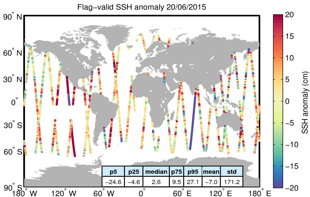
Figure 5. Geographical distribution of flag-valid 1-Hz SSH anomaly data over oceans and lakes for 20/06/2015. The statistical values shown in the table refer to the SSH anomaly in cm and are calculated over all measurements shown in the figure.
