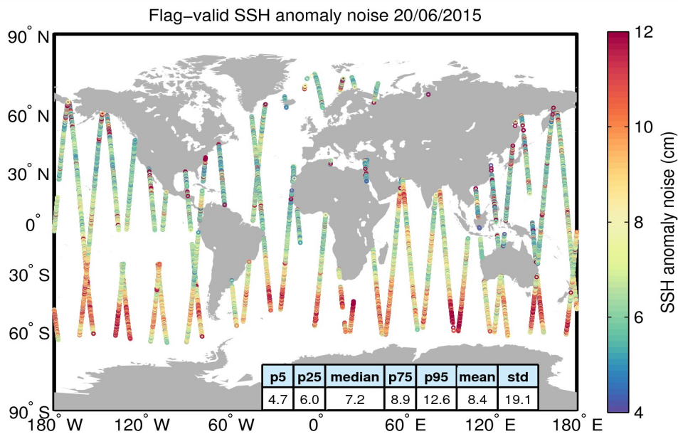
Figure 8. Geographical distribution of flag-valid 20-Hz SSH anomaly measurement noise over oceans and lakes for 20/06/2015. The statistical values shown in the table refer to the SSH anomaly noise and are calculated over all measurements shown in the figure.
