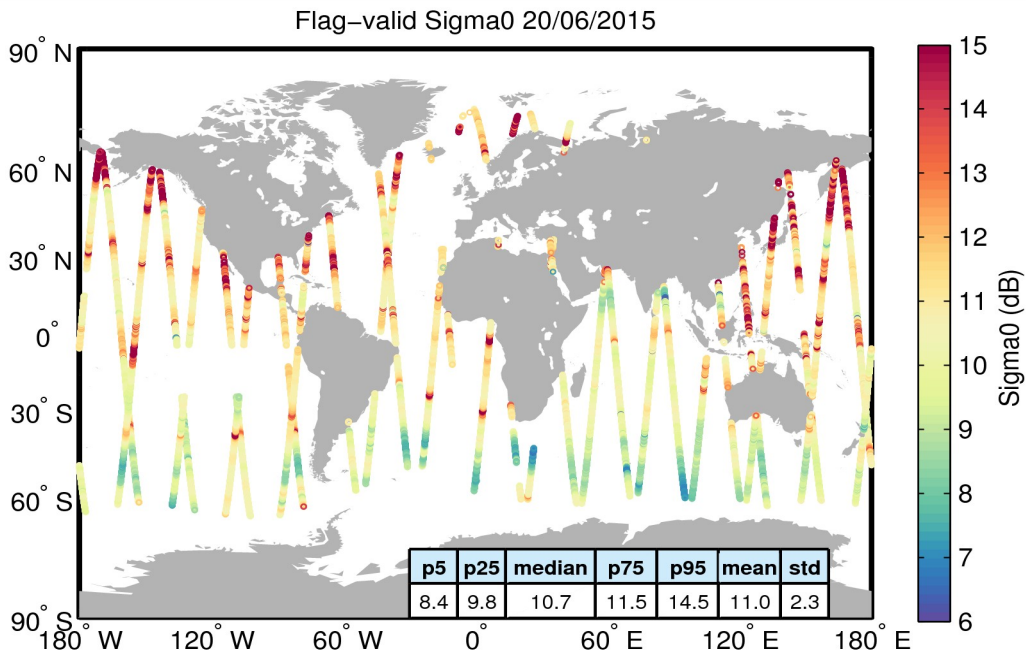
Figure 23. Geographical distribution of flag-valid sigma0 data over oceans and lakes for 20/06/2015. The statistical values shown in the table refer to the sigma0 in dB and are calculated over all measurements shown in the figure.
