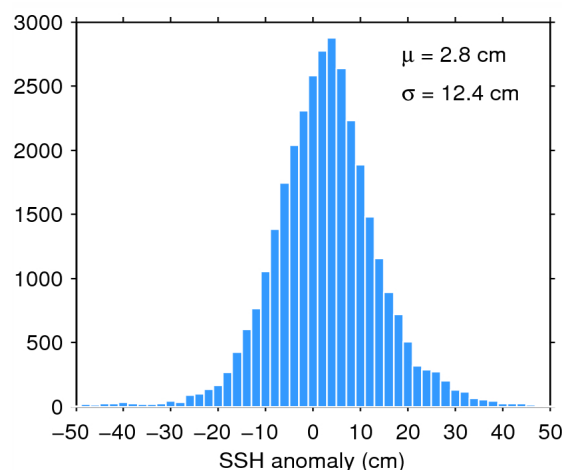
Figure 11. Histogram of science-valid SSH anomaly over oceans and lakes for 20/06/2015. The mean ( \mu ) and standard deviation ( \sigma ) are also shown. Note that values outside [-50 50] cm are excluded from the histogram for the sake of readability but not from the computation of \mu and \sigma .
