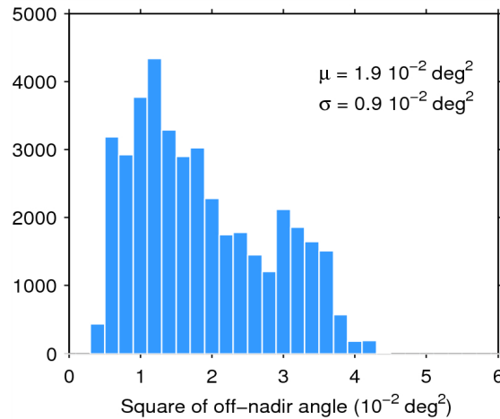
Figure 39. Histogram of flag-valid mispointing over oceans and lakes for 20/06/2015. The mean ( \mu ) and standard deviation ( \sigma ) are also shown. Note that values larger than 6 \cdot 10^{-2} \text{ deg}^2 are excluded from the histogram for the sake of readability but not from the computation of \mu and \sigma .
