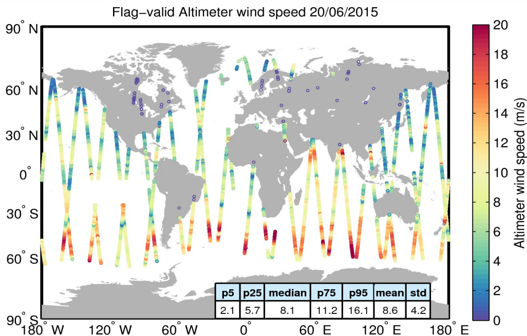
Figure 31. Geographical distribution of flag-valid wind data over oceans and lakes for 20/06/2015. The statistical values shown in the table refer to the wind in m/s and are calculated over all measurements shown in the figure.
