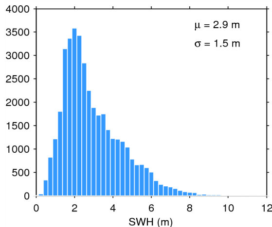
Figure 20. Histogram of science-valid SWH over oceans and lakes for 20/06/2015. The mean ( \mu ) and standard deviation ( \sigma ) are also shown. Note that values larger than 12 m are excluded from the histogram for the sake of readability but not from the computation of \mu and \sigma .
