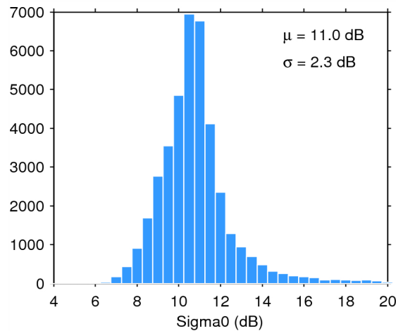
Figure 25. Histogram of flag-valid sigma0 over oceans and lakes for 20/06/2015. The mean ( \mu ) and standard deviation ( \sigma ) are also shown. Note that values outside [4 20] dB are excluded from the histogram for the sake of readability but not from the computation of \mu and \sigma .
