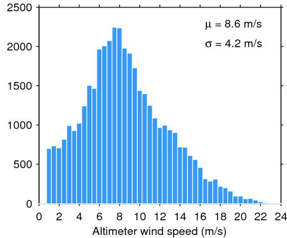
Figure 33. Histogram of flag-valid wind over oceans and lakes for 20/06/2015. The mean ( \mu ) and standard deviation ( \sigma ) are also shown. Note that values larger than 24 m/s are excluded from the histogram for the sake of readability but not from the computation of \mu and \sigma .
