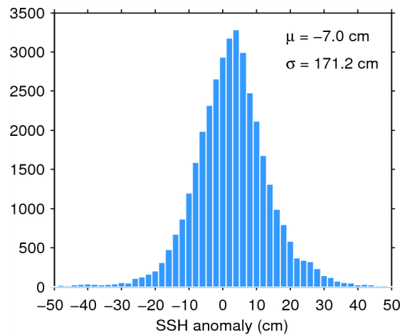
Figure 7. Histogram of flag-valid SSH anomaly over oceans and lakes for 20/06/2015. The mean ( \mu ) and standard deviation ( \sigma ) are also shown. Note that values outside [-50 50] cm are excluded from the histogram for the sake of readability but not from the computation of \mu and \sigma .
