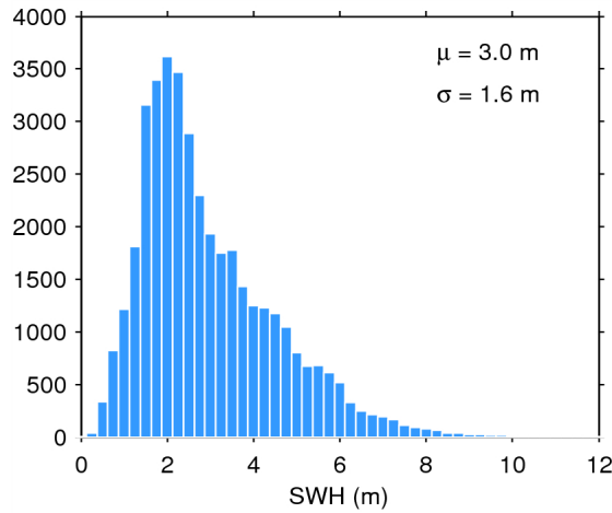
Figure 17. Histogram of flag-valid SWH over oceans and lakes for 20/06/2015. The mean ( \mu ) and standard deviation ( \sigma ) are also shown. Note that values larger than 12 m are excluded from the histogram for the sake of readability but not from the computation of \mu and \sigma .
