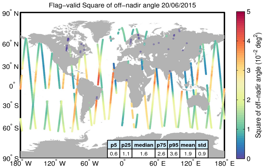
Figure 37. Geographical distribution of flag-valid mispointing data over oceans and lakes for 20/06/2015. The statistical values shown in the table refer to the mispointing in 10^{-2} \text{deg}^2 and are calculated over all measurements shown in the figure.
