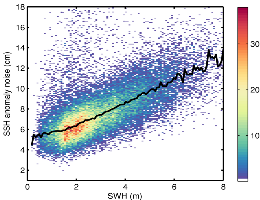
Figure 9. 2D histogram showing flag-valid SSH anomaly noise as a function of SWH for 20/06/2015. The black line denotes the median SSH anomaly as a function of SWH.
