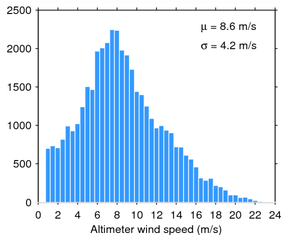
Figure 35. Histogram of science-valid wind over oceans and lakes for 20/06/2015. The mean ( \mu ) and standard deviation ( \sigma ) are also shown. Note that values larger than 24 m/s are excluded from the histogram for the sake of readability but not from the computation of \mu and \sigma .
