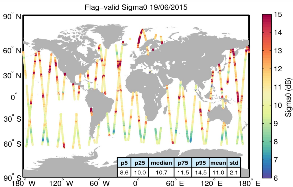
Figure 23. Geographical distribution of flag-valid sigma0 data over oceans and lakes for 19/06/2015. The statistical values shown in the table refer to the sigma0 in dB and are calculated over all measurements shown in the figure.
