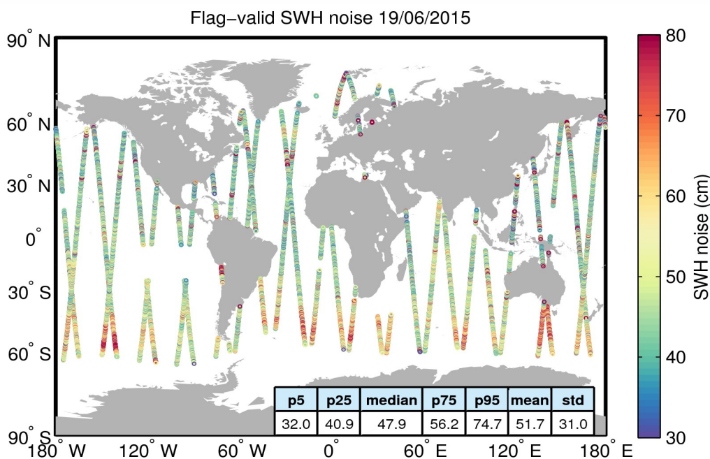
Figure 18. Geographical distribution of flag-valid 20-Hz SWH measurement noise over oceans and lakes for 19/06/2015. The statistical values shown in the figure refer to the SWH noise and are calculated over all measurements shown in the figure.
