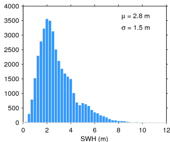
Figure 20. Histogram of science-valid SWH over oceans and lakes for 19/06/2015. The mean ( \mu ) and standard deviation ( \sigma ) are also shown. Note that values larger than 12 m are excluded from the histogram for the sake of readability but not from the computation of \mu and \sigma .
