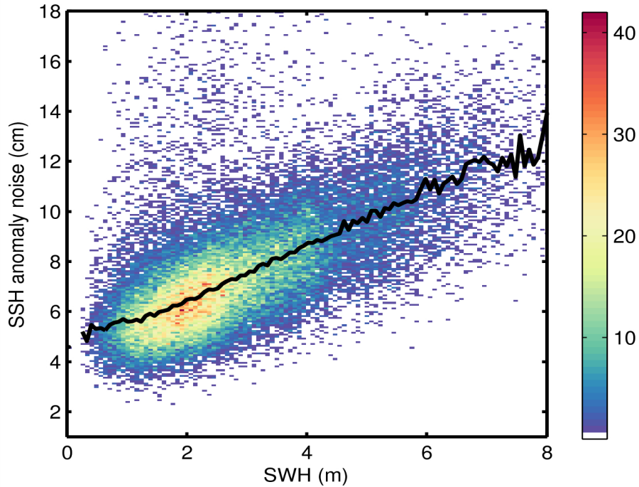
Figure 9. 2D histogram showing flag-valid SSH anomaly noise as a function of SWH for 19/06/2015. The black line denotes the median SSH anomaly as a function of SWH.
