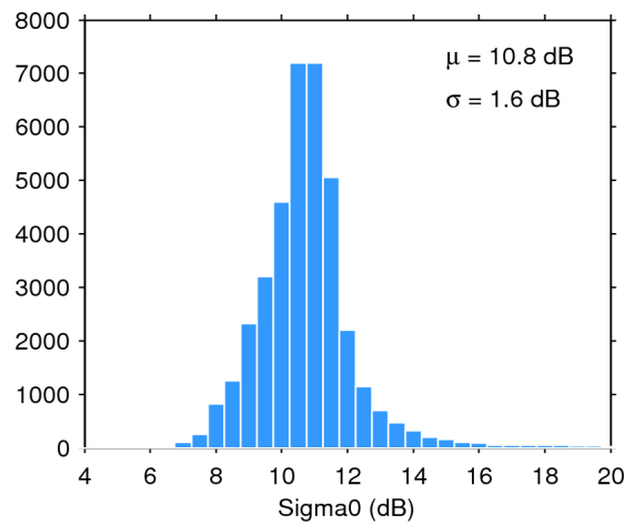
Figure 28. Histogram of science-valid sigma0 over oceans and lakes for 19/06/2015. The mean ( \mu ) and standard deviation ( \sigma ) are also shown. Note that values outside [4 20] dB are excluded from the histogram for the sake of readability but not from the computation of \mu and \sigma .
