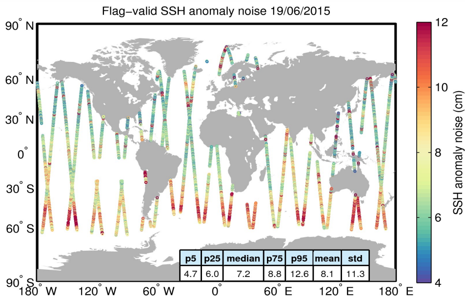
Figure 8. Geographical distribution of flag-valid 20-Hz SSH anomaly measurement noise over oceans and lakes for 19/06/2015. The statistical values shown in the table refer to the SSH anomaly noise and are calculated over all measurements shown in the figure.
