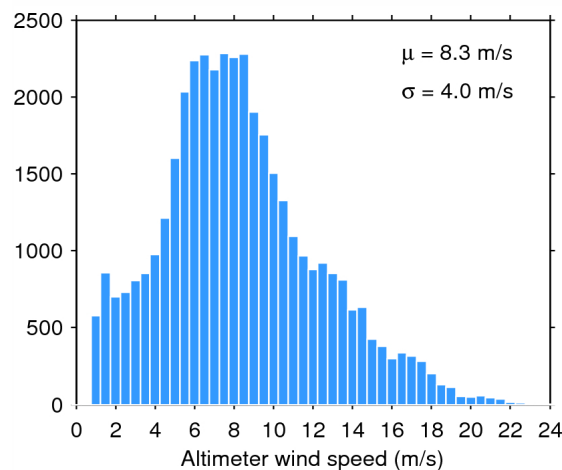
Figure 35. Histogram of science-valid wind over oceans and lakes for 19/06/2015. The mean ( \mu ) and standard deviation ( \sigma ) are also shown. Note that values larger than 24 m/s are excluded from the histogram for the sake of readability but not from the computation of \mu and \sigma .
