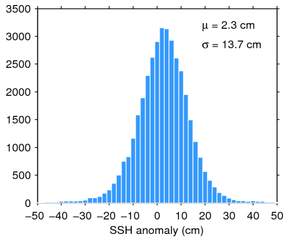
Figure 11. Histogram of science-valid SSH anomaly over oceans and lakes for 19/06/2015. The mean ( \mu ) and standard deviation ( \sigma ) are also shown. Note that values outside [-50 50] cm are excluded from the histogram for the sake of readability but not from the computation of \mu and \sigma .
