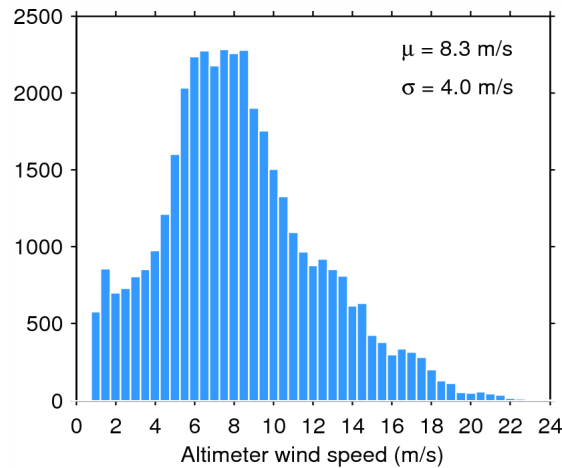
Figure 33. Histogram of flag-valid wind over oceans and lakes for 19/06/2015. The mean ( \mu ) and standard deviation ( \sigma ) are also shown. Note that values larger than 24 m/s are excluded from the histogram for the sake of readability but not from the computation of \mu and \sigma .
