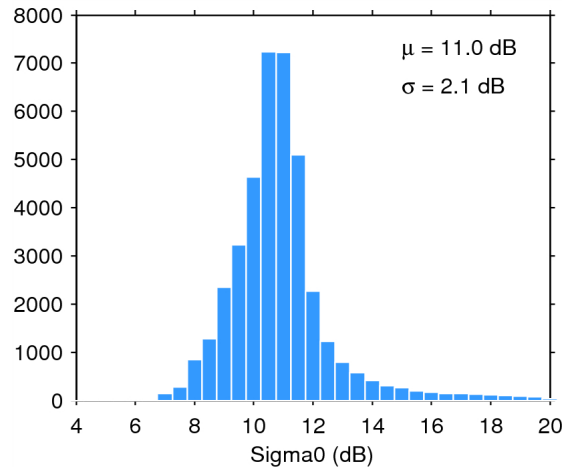
Figure 25. Histogram of flag-valid sigma0 over oceans and lakes for 19/06/2015. The mean ( \mu ) and standard deviation ( \sigma ) are also shown. Note that values outside [4 20] dB are excluded from the histogram for the sake of readability but not from the computation of \mu and \sigma .
