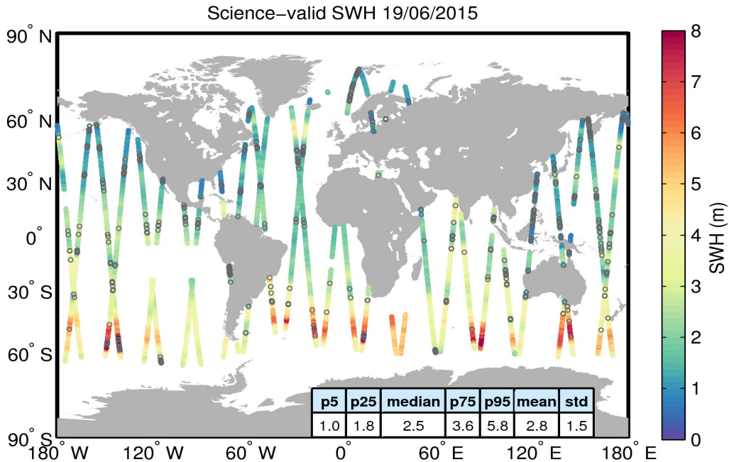
Figure 19. Geographical distribution of science-valid SWH data over oceans and lakes for 19/06/2015. The statistical values shown in the table refer to the SWH in m and are calculated over all measurements shown in the figure. Gray circles denote records that have been rejected based on the editing criteria described in Table 3.
