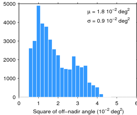
Figure 39. Histogram of flag-valid mispointing over oceans and lakes for 19/06/2015. The mean ( \mu ) and standard deviation ( \sigma ) are also shown. Note that values larger than 6 \cdot 10^{-2} \text{ deg}^2 are excluded from the histogram for the sake of readability but not from the computation of \mu and \sigma .
