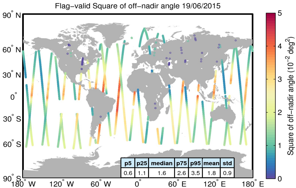
Figure 37. Geographical distribution of flag-valid mispointing data over oceans and lakes for 19/06/2015. The statistical values shown in the table refer to the mispointing in 10^{-2} \text{ deg}^2 and are calculated over all measurements shown in the figure.
