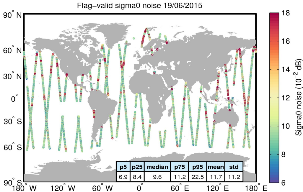
Figure 26. Geographical distribution of flag-valid 20-Hz sigma0 measurement noise over oceans and lakes for 19/06/2015. The statistical values shown in the table refer to the sigma0 noise and are calculated over all measurements shown in the figure.
