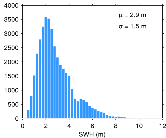
Figure 17. Histogram of flag-valid SWH over oceans and lakes for 19/06/2015. The mean ( \mu ) and standard deviation ( \sigma ) are also shown. Note that values larger than 12 m are excluded from the histogram for the sake of readability but not from the computation of \mu and \sigma .
