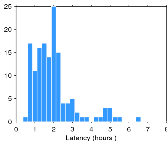
Figure 2. Histogram of the data latency for 19/06/2015. The y-axis denotes the number of files that are made available with a delay of x-hours with respect to the mean time of the records stored in the file.
