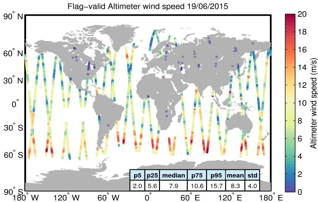
Figure 31. Geographical distribution of flag-valid wind data over oceans and lakes for 19/06/2015. The statistical values shown in the table refer to the wind in m/s and are calculated over all measurements shown in the figure.
