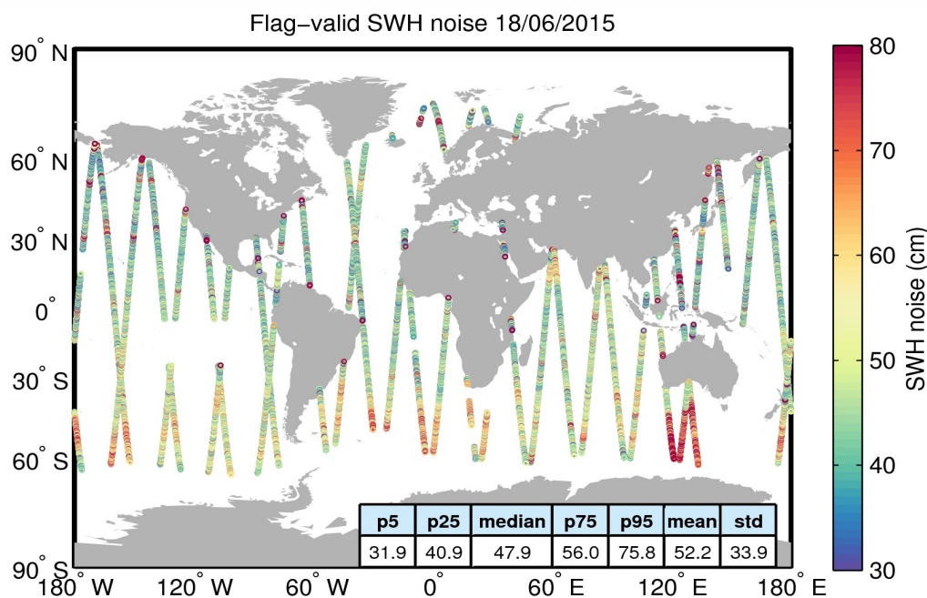
Figure 18. Geographical distribution of flag-valid 20-Hz SWH measurement noise over oceans and lakes for 18/06/2015. The statistical values shown in the figure refer to the SWH noise and are calculated over all measurements shown in the figure.
