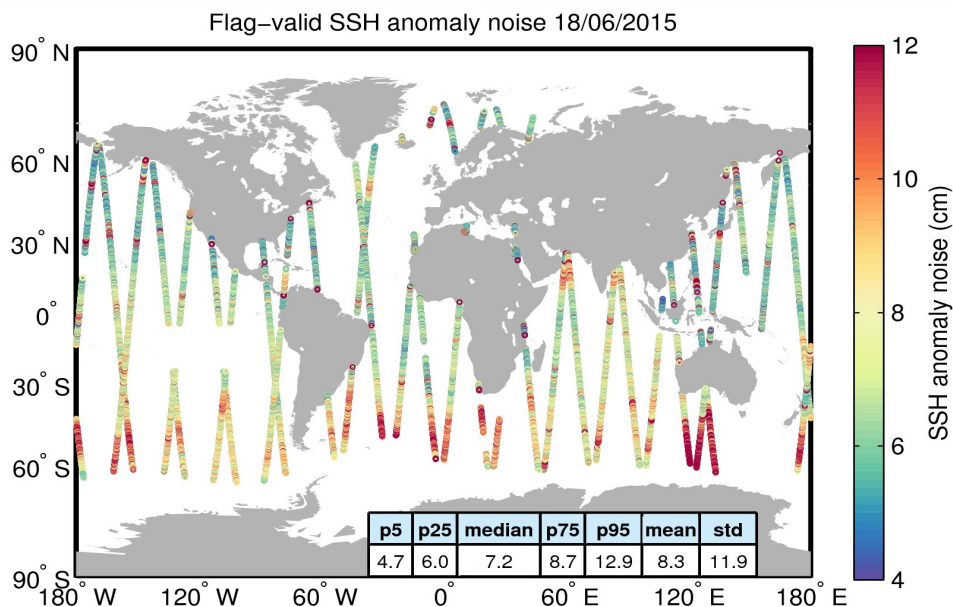
Figure 8. Geographical distribution of flag-valid 20-Hz SSH anomaly measurement noise over oceans and lakes for 18/06/2015. The statistical values shown in the table refer to the SSH anomaly noise and are calculated over all measurements shown in the figure.
