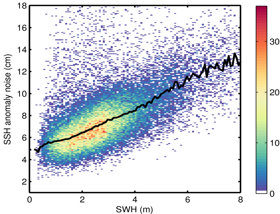
Figure 9. 2D histogram showing flag-valid SSH anomaly noise as a function of SWH for 18/06/2015. The black line denotes the median SSH anomaly as a function of SWH.
