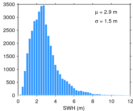
Figure 17. Histogram of flag-valid SWH over oceans and lakes for 18/06/2015. The mean ( \mu ) and standard deviation ( \sigma ) are also shown. Note that values larger than 12 m are excluded from the histogram for the sake of readability but not from the computation of \mu and \sigma .
