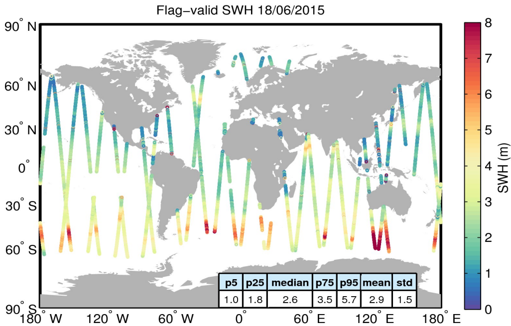
Figure 15. Geographical distribution of flag-valid SWH data over oceans and lakes for 18/06/2015. The statistical values shown in the table refer to the SWH in m and are calculated over all measurements shown in the figure.
