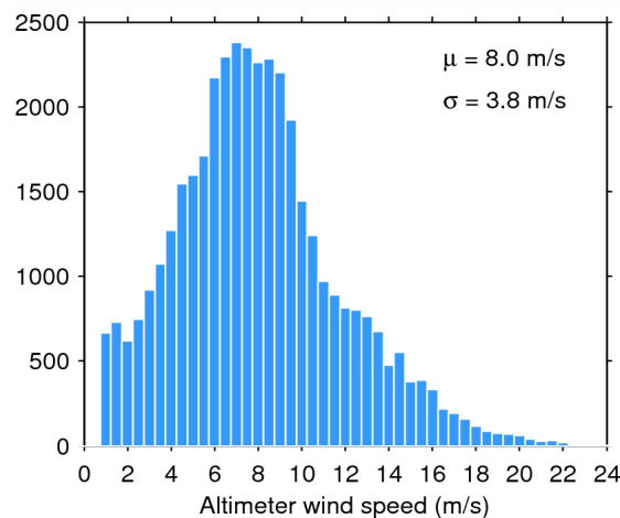
Figure 35. Histogram of science-valid wind over oceans and lakes for 18/06/2015. The mean ( \mu ) and standard deviation ( \sigma ) are also shown. Note that values larger than 24 m/s are excluded from the histogram for the sake of readability but not from the computation of \mu and \sigma .
