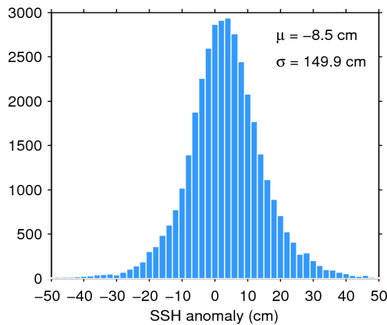
Figure 7. Histogram of flag-valid SSH anomaly over oceans and lakes for 18/06/2015. The mean ( \mu ) and standard deviation ( \sigma ) are also shown. Note that values outside [-50\ 50] cm are excluded from the histogram for the sake of readability but not from the computation of \mu and \sigma .
