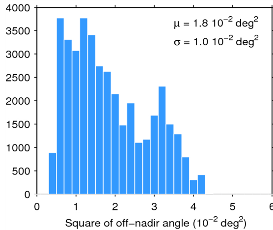
Figure 39. Histogram of flag-valid mispointing over oceans and lakes for 18/06/2015. The mean ( \mu ) and standard deviation ( \sigma ) are also shown. Note that values larger than 6 \cdot 10^{-2} \text{ deg}^2 are excluded from the histogram for the sake of readability but not from the computation of \mu and \sigma .
