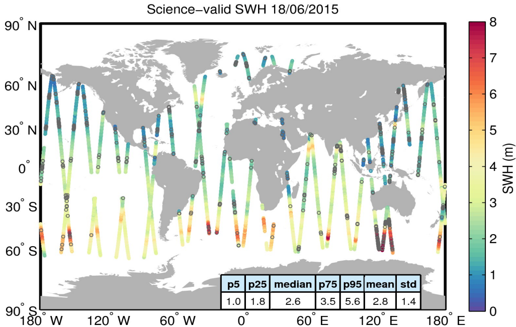
Figure 19. Geographical distribution of science-valid SWH data over oceans and lakes for 18/06/2015. The statistical values shown in the table refer to the SWH in m and are calculated over all measurements shown in the figure. Gray circles denote records that have been rejected based on the editing criteria described in Table 3.
