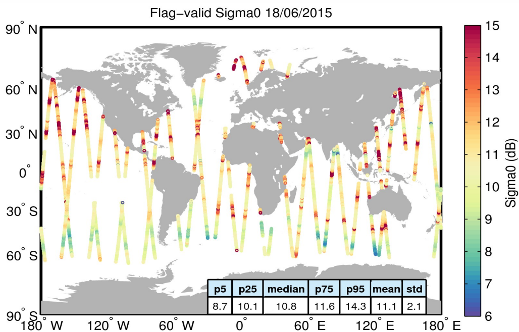
Figure 23. Geographical distribution of flag-valid sigma0 data over oceans and lakes for 18/06/2015. The statistical values shown in the table refer to the sigma0 in dB and are calculated over all measurements shown in the figure.
