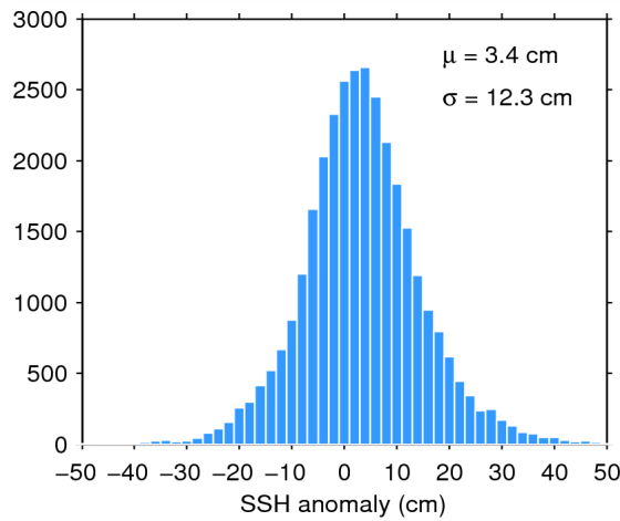
Figure 11. Histogram of science-valid SSH anomaly over oceans and lakes for 18/06/2015. The mean ( \mu ) and standard deviation ( \sigma ) are also shown. Note that values outside [-50 50] cm are excluded from the histogram for the sake of readability but not from the computation of \mu and \sigma .
