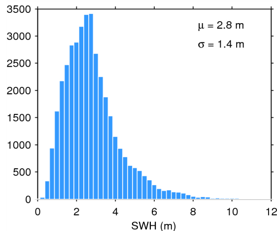
Figure 20. Histogram of science-valid SWH over oceans and lakes for 18/06/2015. The mean ( \mu ) and standard deviation ( \sigma ) are also shown. Note that values larger than 12 m are excluded from the histogram for the sake of readability but not from the computation of \mu and \sigma .
