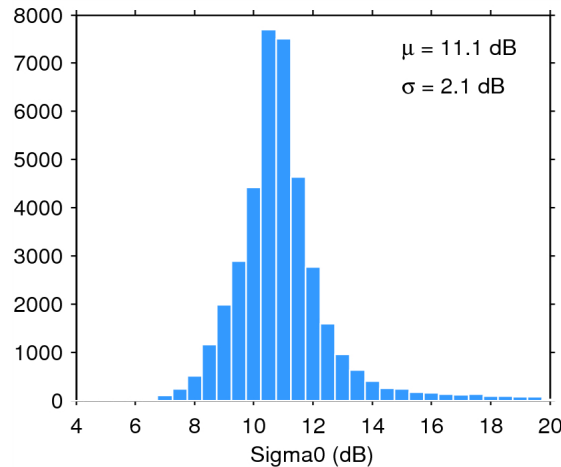
Figure 25. Histogram of flag-valid sigma0 over oceans and lakes for 18/06/2015. The mean ( \mu ) and standard deviation ( \sigma ) are also shown. Note that values outside [4 20] dB are excluded from the histogram for the sake of readability but not from the computation of \mu and \sigma .
