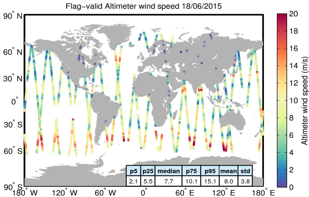
Figure 31. Geographical distribution of flag-valid wind data over oceans and lakes for 18/06/2015. The statistical values shown in the table refer to the wind in m/s and are calculated over all measurements shown in the figure.
