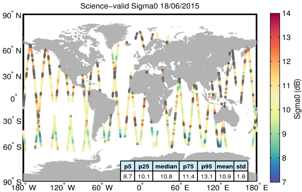
Figure 27. Geographical distribution of science-valid sigma0 data over oceans and lakes for 18/06/2015. The statistical values shown in the table refer to the sigma0 in dB and are calculated over all measurements shown in the figure. Gray circles denote records that have been rejected based on the editing criteria described in Table 4.
