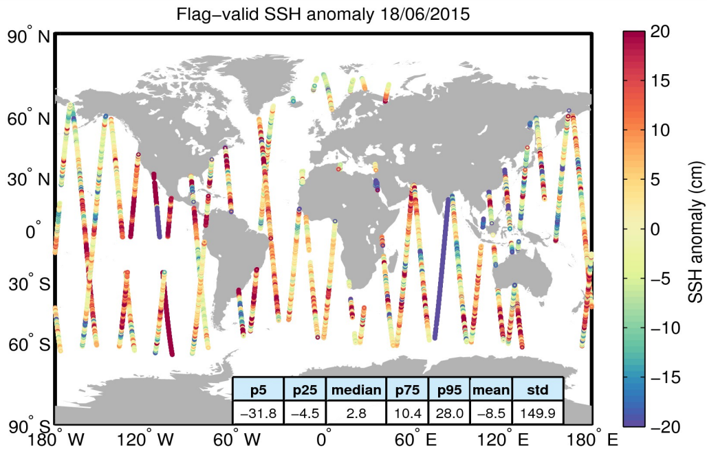
Figure 5. Geographical distribution of flag-valid 1-Hz SSH anomaly data over oceans and lakes for 18/06/2015. The statistical values shown in the table refer to the SSH anomaly in cm and are calculated over all measurements shown in the figure.
