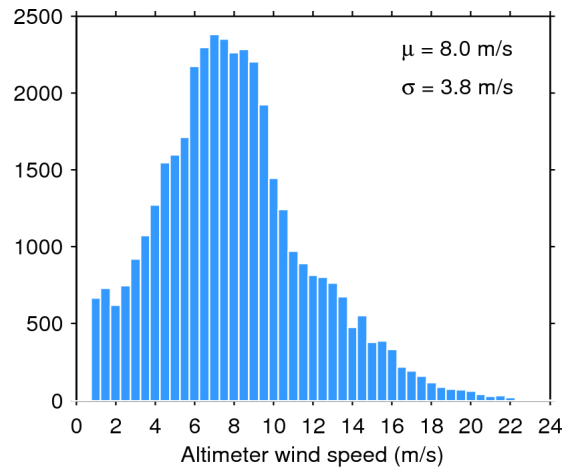
Figure 33. Histogram of flag-valid wind over oceans and lakes for 18/06/2015. The mean ( \mu ) and standard deviation ( \sigma ) are also shown. Note that values larger than 24 m/s are excluded from the histogram for the sake of readability but not from the computation of \mu and \sigma .
