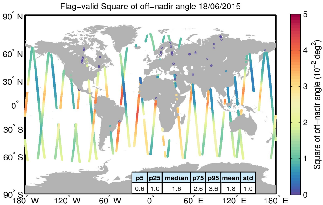
Figure 37. Geographical distribution of flag-valid mispointing data over oceans and lakes for 18/06/2015. The statistical values shown in the table refer to the mispointing in 10^{-2} \text{deg}^2 and are calculated over all measurements shown in the figure.
