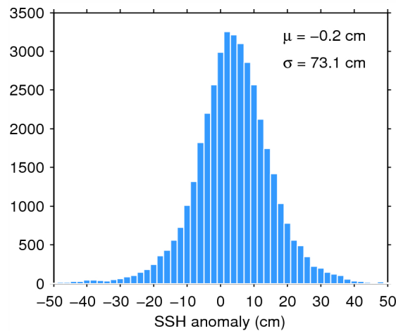
Figure 7. Histogram of flag-valid SSH anomaly over oceans and lakes for 17/06/2015. The mean ( \mu ) and standard deviation ( \sigma ) are also shown. Note that values outside [-50 50] cm are excluded from the histogram for the sake of readability but not from the computation of \mu and \sigma .
