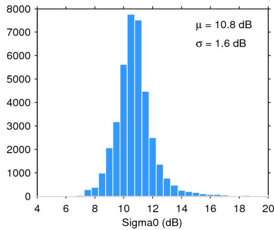
Figure 28. Histogram of science-valid sigma0 over oceans and lakes for 17/06/2015. The mean ( \mu ) and standard deviation ( \sigma ) are also shown. Note that values outside [4 20] dB are excluded from the histogram for the sake of readability but not from the computation of \mu and \sigma .
