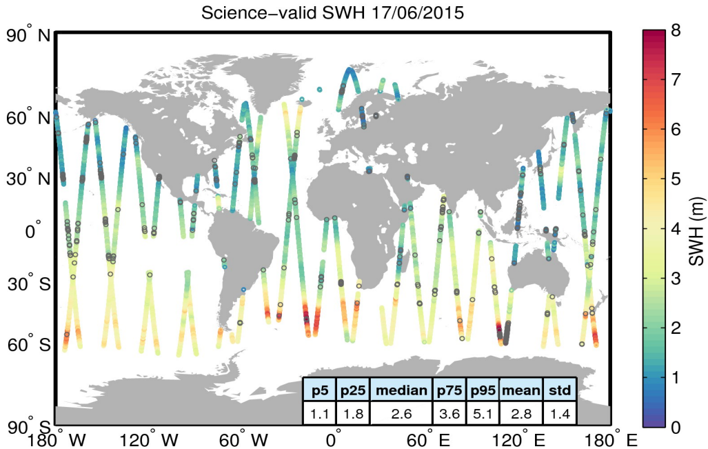
Figure 19. Geographical distribution of science-valid SWH data over oceans and lakes for 17/06/2015. The statistical values shown in the table refer to the SWH in m and are calculated over all measurements shown in the figure. Gray circles denote records that have been rejected based on the editing criteria described in Table 3.
