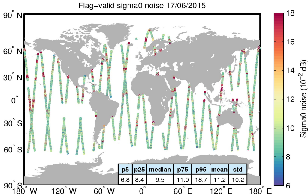
Figure 26. Geographical distribution of flag-valid 20-Hz sigma0 measurement noise over oceans and lakes for 17/06/2015. The statistical values shown in the table refer to the sigma0 noise and are calculated over all measurements shown in the figure.
