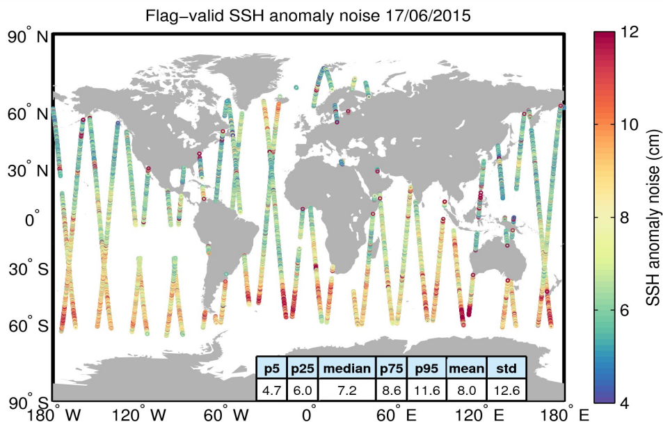
Figure 8. Geographical distribution of flag-valid 20-Hz SSH anomaly measurement noise over oceans and lakes for 17/06/2015. The statistical values shown in the table refer to the SSH anomaly noise and are calculated over all measurements shown in the figure.
