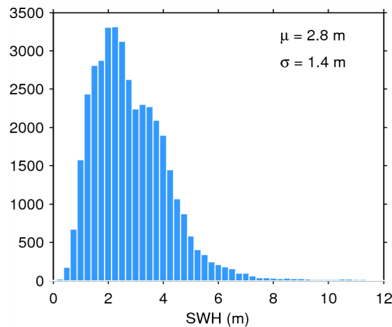
Figure 17. Histogram of flag-valid SWH over oceans and lakes for 17/06/2015. The mean ( \mu ) and standard deviation ( \sigma ) are also shown. Note that values larger than 12 m are excluded from the histogram for the sake of readability but not from the computation of \mu and \sigma .
