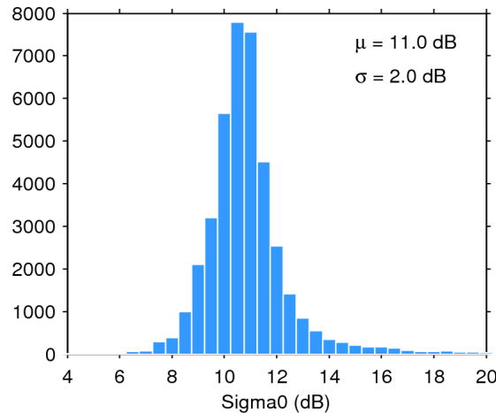
Figure 25. Histogram of flag-valid sigma0 over oceans and lakes for 17/06/2015. The mean ( \mu ) and standard deviation ( \sigma ) are also shown. Note that values outside [4 20] dB are excluded from the histogram for the sake of readability but not from the computation of \mu and \sigma .
