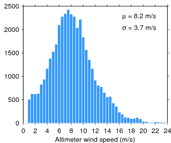
Figure 35. Histogram of science-valid wind over oceans and lakes for 17/06/2015. The mean ( \mu ) and standard deviation ( \sigma ) are also shown. Note that values larger than 24 m/s are excluded from the histogram for the sake of readability but not from the computation of \mu and \sigma .
