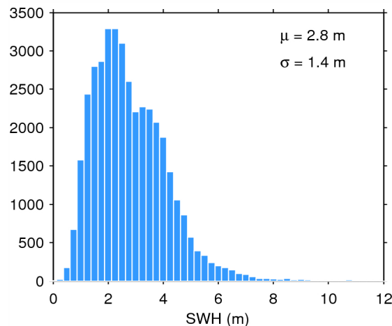
Figure 20. Histogram of science-valid SWH over oceans and lakes for 17/06/2015. The mean ( \mu ) and standard deviation ( \sigma ) are also shown. Note that values larger than 12 m are excluded from the histogram for the sake of readability but not from the computation of \mu and \sigma .
