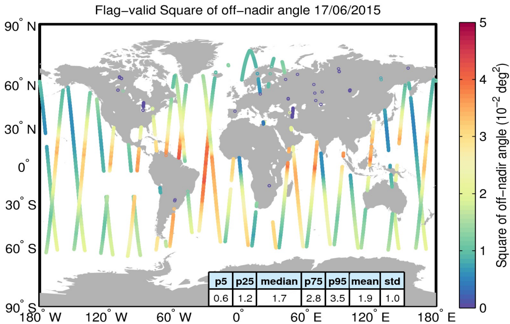
Figure 37. Geographical distribution of flag-valid mispointing data over oceans and lakes for 17/06/2015. The statistical values shown in the table refer to the mispointing in 10^{-2} deg 2 and are calculated over all measurements shown in the figure.
