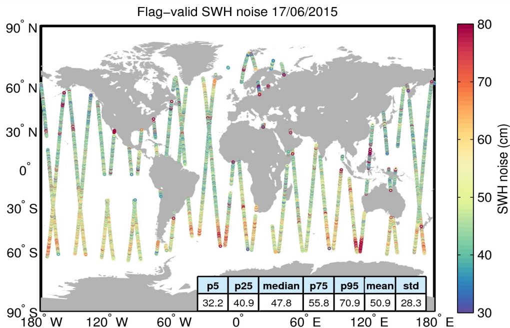
Figure 18. Geographical distribution of flag-valid 20-Hz SWH measurement noise over oceans and lakes for 17/06/2015. The statistical values shown in the figure refer to the SWH noise and are calculated over all measurements shown in the figure.
