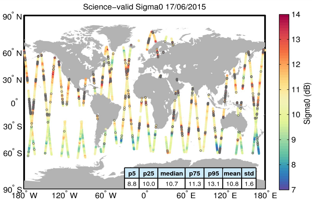
Figure 27. Geographical distribution of science-valid sigma0 data over oceans and lakes for 17/06/2015. The statistical values shown in the table refer to the sigma0 in dB and are calculated over all measurements shown in the figure. Gray circles denote records that have been rejected based on the editing criteria described in Table 4.
