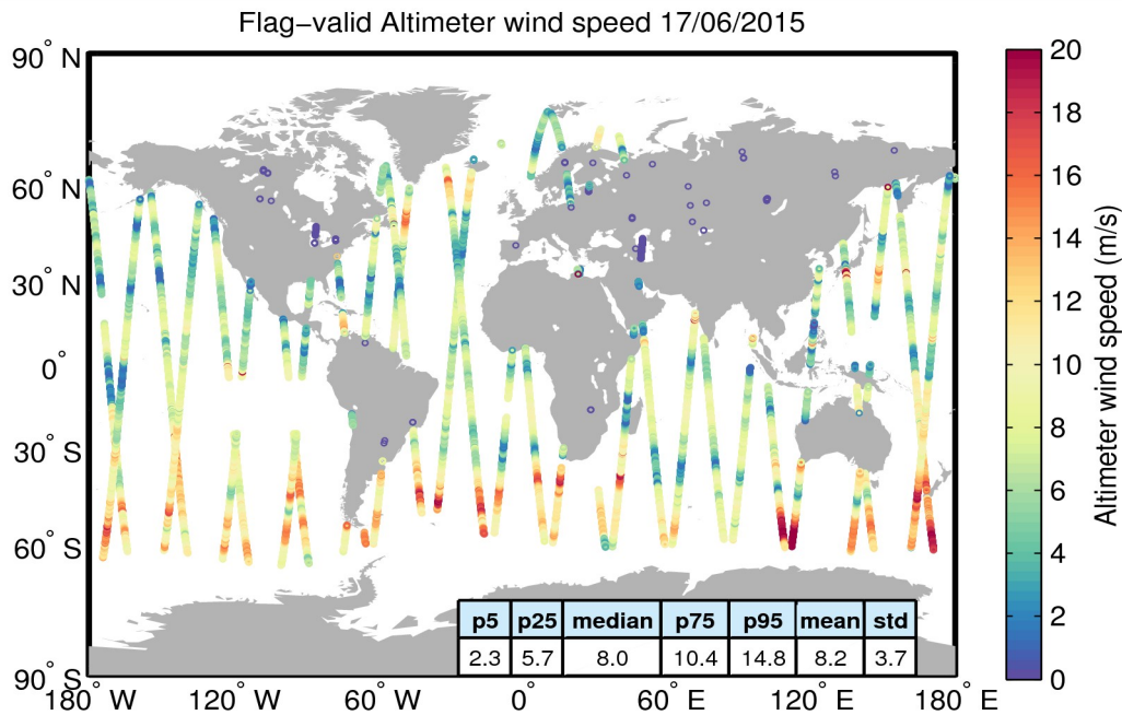
Figure 31. Geographical distribution of flag-valid wind data over oceans and lakes for 17/06/2015. The statistical values shown in the table refer to the wind in m/s and are calculated over all measurements shown in the figure.
