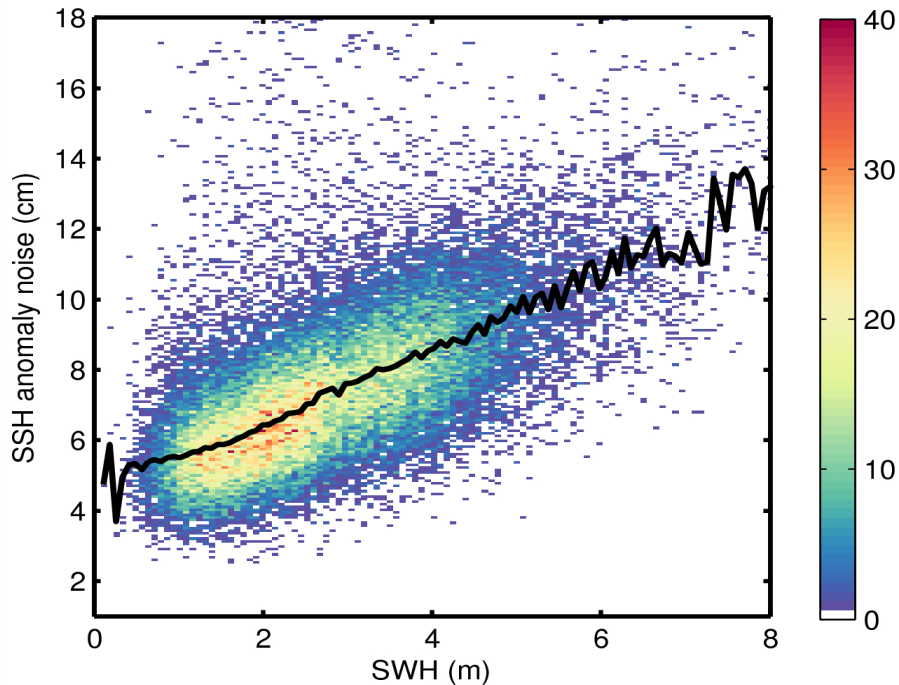
Figure 9. 2D histogram showing flag-valid SSH anomaly noise as a function of SWH for 17/06/2015. The black line denotes the median SSH anomaly as a function of SWH.
