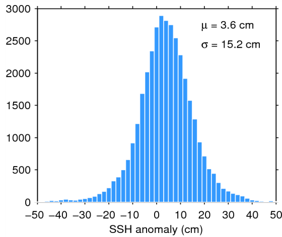
Figure 11. Histogram of science-valid SSH anomaly over oceans and lakes for 17/06/2015. The mean ( \mu ) and standard deviation ( \sigma ) are also shown. Note that values outside [-50 50] cm are excluded from the histogram for the sake of readability but not from the computation of \mu and \sigma .
