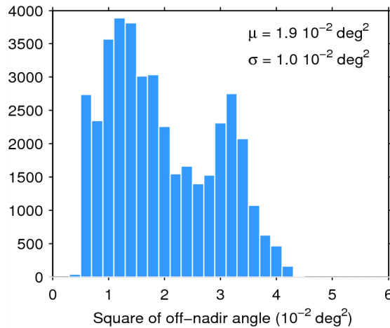
Figure 39. Histogram of flag-valid mispointing over oceans and lakes for 17/06/2015. The mean ( \mu ) and standard deviation ( \sigma ) are also shown. Note that values larger than 6 \cdot 10^{-2} \text{ deg}^2 are excluded from the histogram for the sake of readability but not from the computation of \mu and \sigma .
