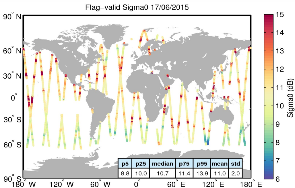
Figure 23. Geographical distribution of flag-valid sigma0 data over oceans and lakes for 17/06/2015. The statistical values shown in the table refer to the sigma0 in dB and are calculated over all measurements shown in the figure.
