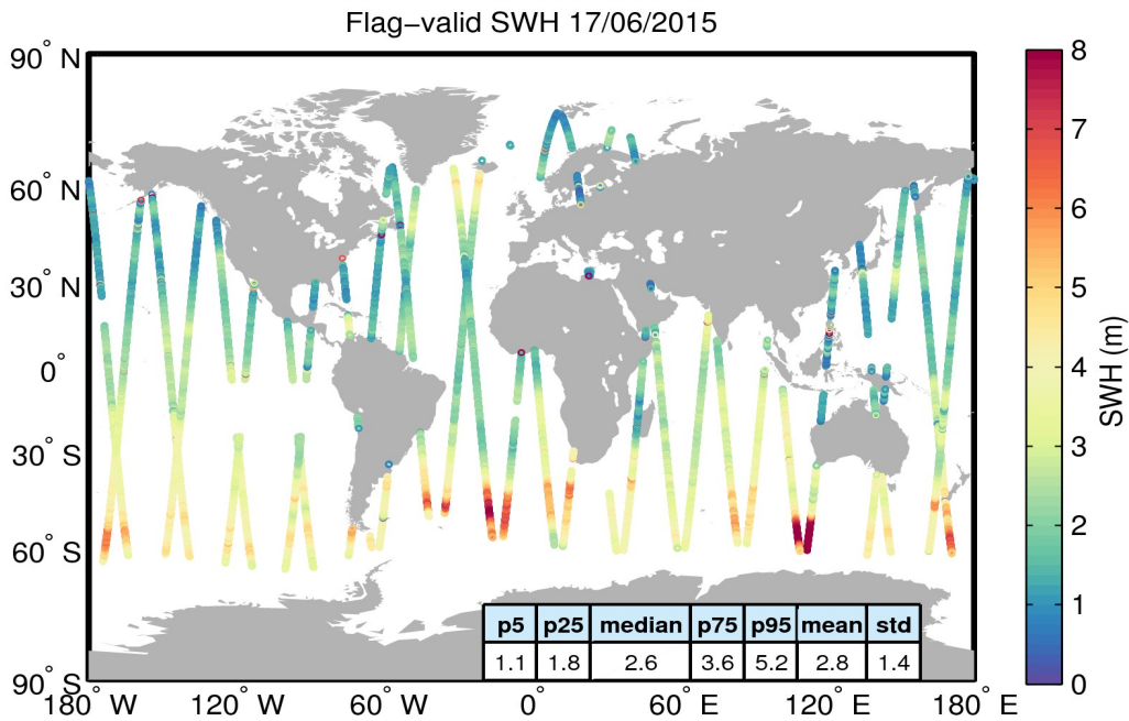
Figure 15. Geographical distribution of flag-valid SWH data over oceans and lakes for 17/06/2015. The statistical values shown in the table refer to the SWH in m and are calculated over all measurements shown in the figure.
