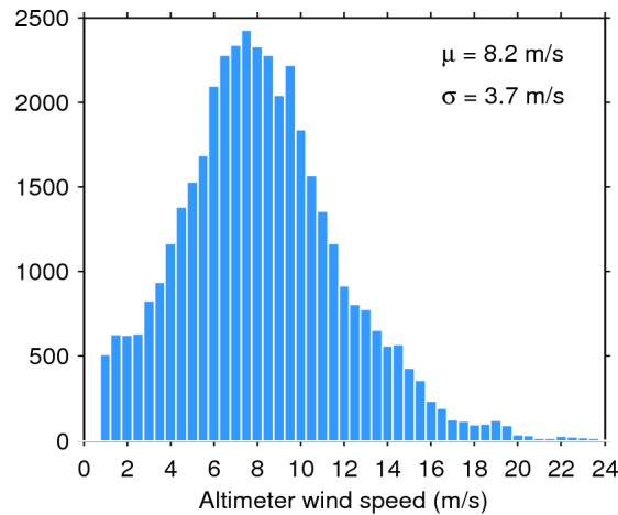
Figure 33. Histogram of flag-valid wind over oceans and lakes for 17/06/2015. The mean ( \mu ) and standard deviation ( \sigma ) are also shown. Note that values larger than 24 m/s are excluded from the histogram for the sake of readability but not from the computation of \mu and \sigma .
