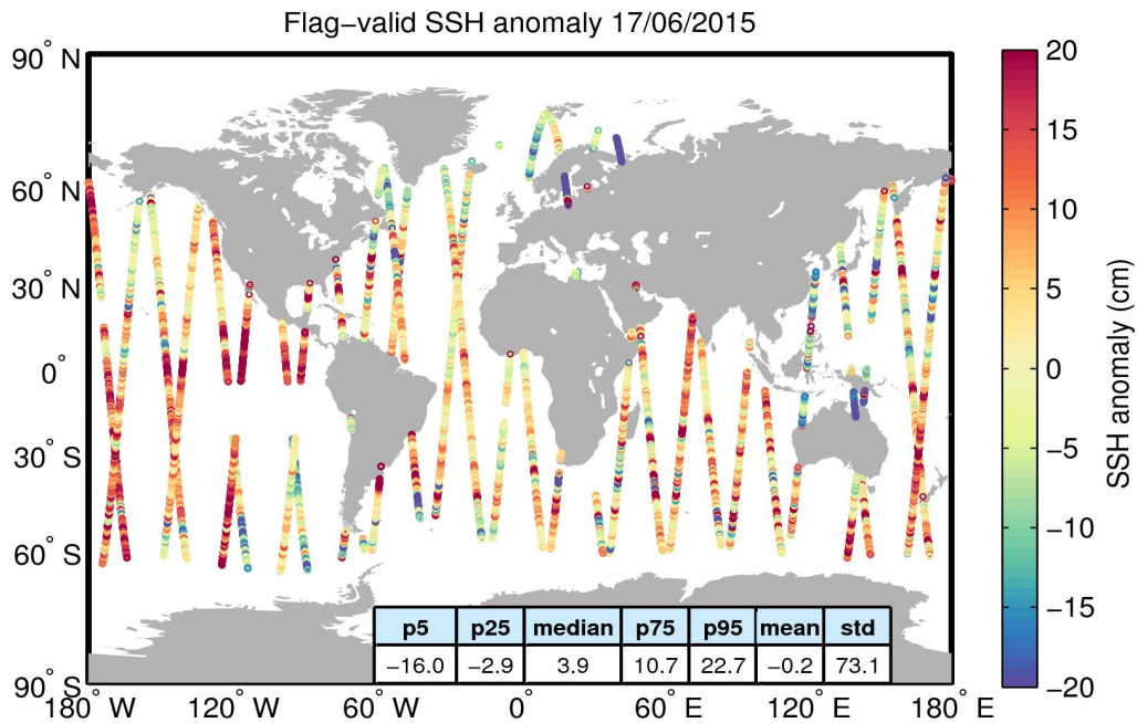
Figure 5. Geographical distribution of flag-valid 1-Hz SSH anomaly data over oceans and lakes for 17/06/2015. The statistical values shown in the table refer to the SSH anomaly in cm and are calculated over all measurements shown in the figure.
