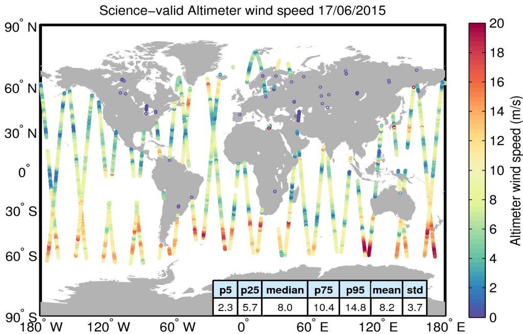
Figure 34. Geographical distribution of science-valid wind data over oceans and lakes for 17/06/2015. The statistical values shown in the table refer to the wind in m/s and are calculated over all measurements shown in the figure. Gray circles denote records that have been rejected based on the editing criteria described in Table 5.
