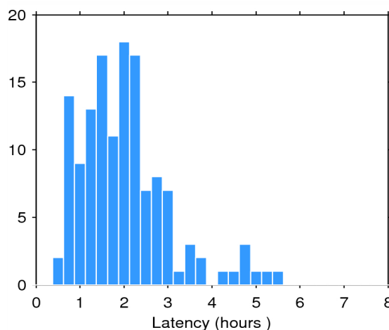
Figure 2. Histogram of the data latency for 17/06/2015. The y-axis denotes the number of files that are made available with a delay of x-hours with respect to the mean time of the records stored in the file.
