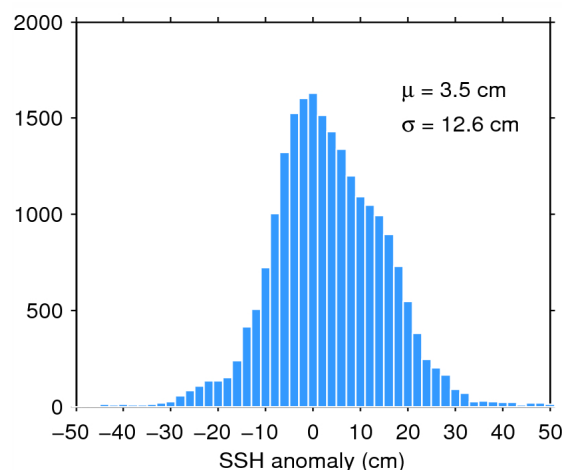
Figure 11. Histogram of science-valid SSH anomaly over oceans and lakes for 16/06/2015. The mean ( \mu ) and standard deviation ( \sigma ) are also shown. Note that values outside [-50 \text{ } 50] cm are excluded from the histogram for the sake of readability but not from the computation of \mu and \sigma .
