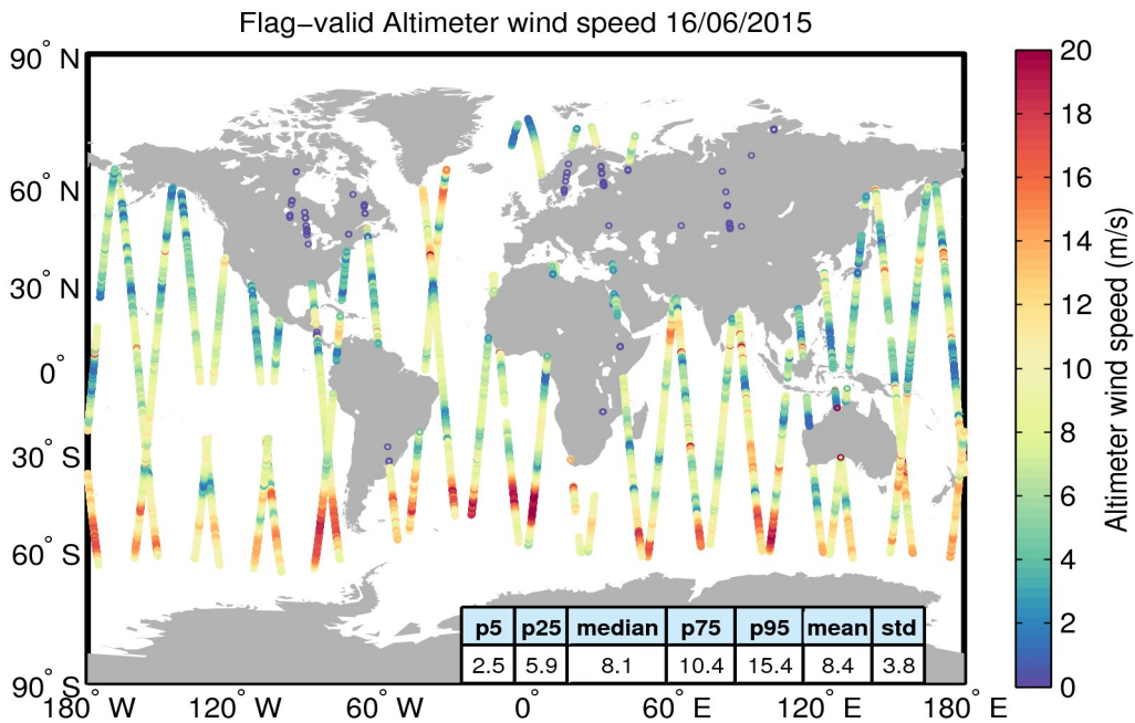
Figure 31. Geographical distribution of flag-valid wind data over oceans and lakes for 16/06/2015. The statistical values shown in the table refer to the wind in m/s and are calculated over all measurements shown in the figure.
