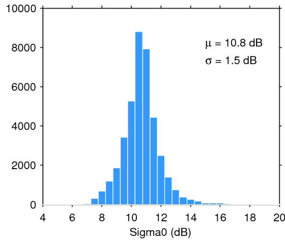
Figure 28. Histogram of science-valid sigma0 over oceans and lakes for 16/06/2015. The mean ( \mu ) and standard deviation ( \sigma ) are also shown. Note that values outside [4 20] dB are excluded from the histogram for the sake of readability but not from the computation of \mu and \sigma .
