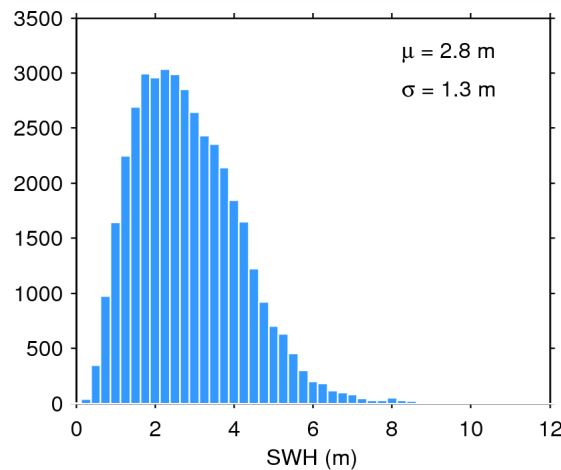
Figure 20. Histogram of science-valid SWH over oceans and lakes for 16/06/2015. The mean ( \mu ) and standard deviation ( \sigma ) are also shown. Note that values larger than 12 m are excluded from the histogram for the sake of readability but not from the computation of \mu and \sigma .
