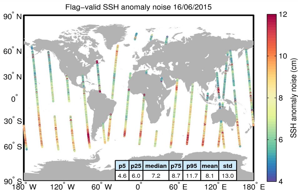
Figure 8. Geographical distribution of flag-valid 20-Hz SSH anomaly measurement noise over oceans and lakes for 16/06/2015. The statistical values shown in the table refer to the SSH anomaly noise and are calculated over all measurements shown in the figure.
