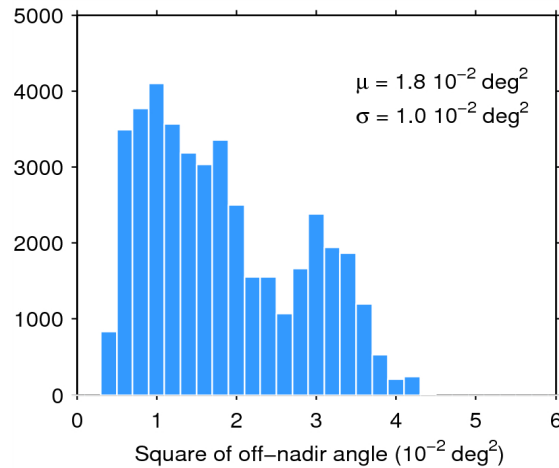
Figure 39. Histogram of flag-valid mispointing over oceans and lakes for 16/06/2015. The mean ( \mu ) and standard deviation ( \sigma ) are also shown. Note that values larger than 6 \cdot 10^{-2} \text{ deg}^2 are excluded from the histogram for the sake of readability but not from the computation of \mu and \sigma .
