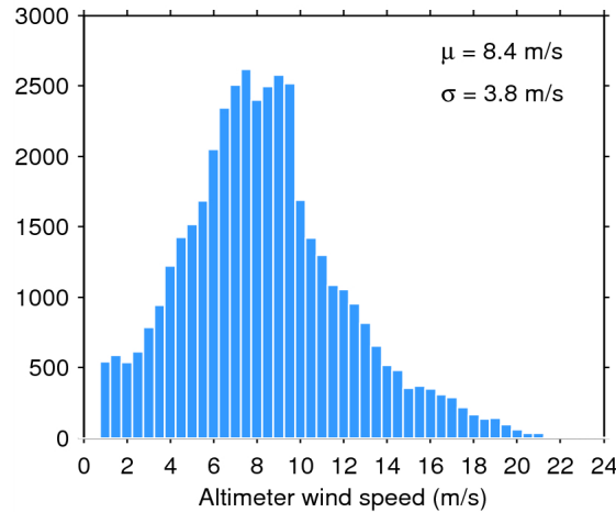
Figure 33. Histogram of flag-valid wind over oceans and lakes for 16/06/2015. The mean ( \mu ) and standard deviation ( \sigma ) are also shown. Note that values larger than 24 m/s are excluded from the histogram for the sake of readability but not from the computation of \mu and \sigma .
