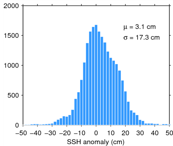
Figure 7. Histogram of flag-valid SSH anomaly over oceans and lakes for 16/06/2015. The mean ( \mu ) and standard deviation ( \sigma ) are also shown. Note that values outside [-50\ 50] cm are excluded from the histogram for the sake of readability but not from the computation of \mu and \sigma .
