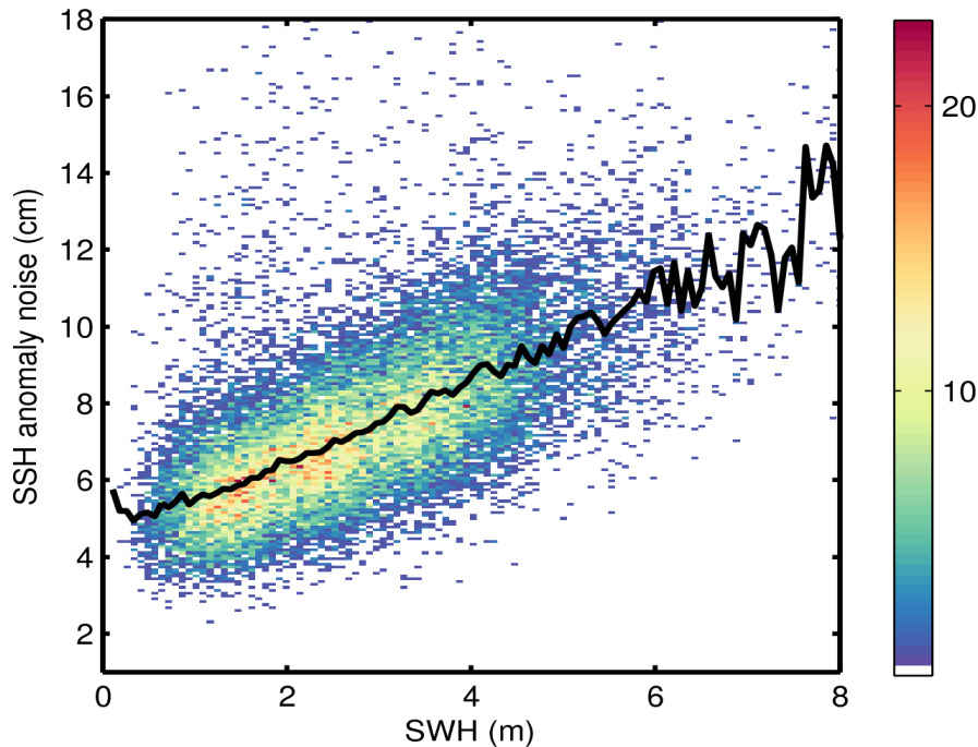
Figure 9. 2D histogram showing flag-valid SSH anomaly noise as a function of SWH for 16/06/2015. The black line denotes the median SSH anomaly as a function of SWH.
