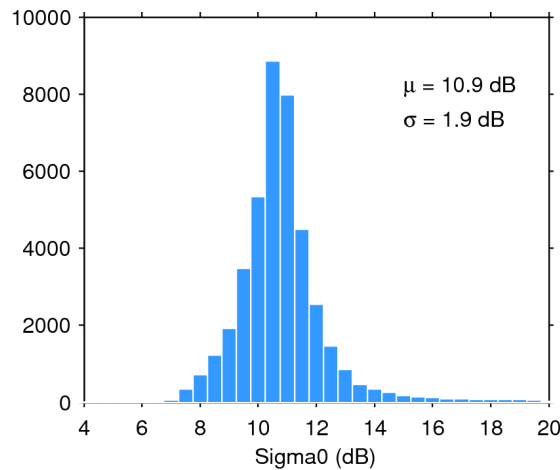
Figure 25. Histogram of flag-valid sigma0 over oceans and lakes for 16/06/2015. The mean ( \mu ) and standard deviation ( \sigma ) are also shown. Note that values outside [4 20] dB are excluded from the histogram for the sake of readability but not from the computation of \mu and \sigma .
