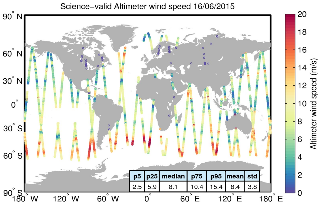
Figure 34. Geographical distribution of science-valid wind data over oceans and lakes for 16/06/2015. The statistical values shown in the table refer to the wind in m/s and are calculated over all measurements shown in the figure. Gray circles denote records that have been rejected based on the editing criteria described in Table 5.
