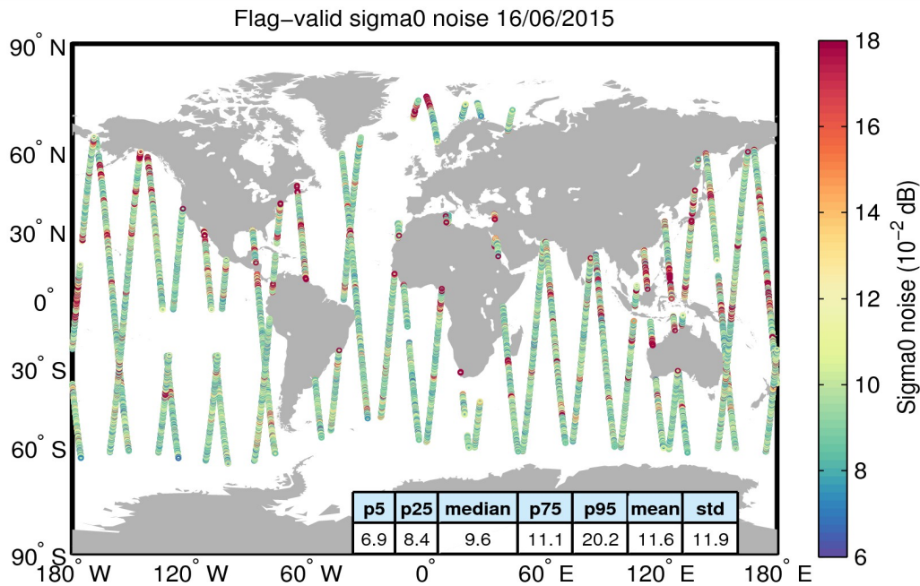
Figure 26. Geographical distribution of flag-valid 20-Hz sigma0 measurement noise over oceans and lakes for 16/06/2015. The statistical values shown in the table refer to the sigma0 noise and are calculated over all measurements shown in the figure.
