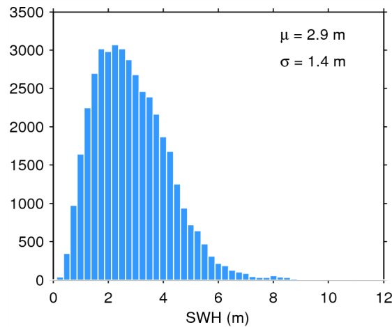
Figure 17. Histogram of flag-valid SWH over oceans and lakes for 16/06/2015. The mean ( \mu ) and standard deviation ( \sigma ) are also shown. Note that values larger than 12 m are excluded from the histogram for the sake of readability but not from the computation of \mu and \sigma .
