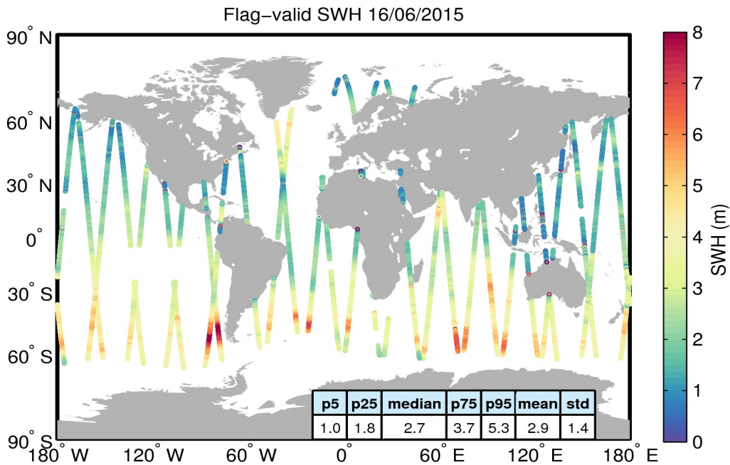
Figure 15. Geographical distribution of flag-valid SWH data over oceans and lakes for 16/06/2015. The statistical values shown in the table refer to the SWH in m and are calculated over all measurements shown in the figure.
