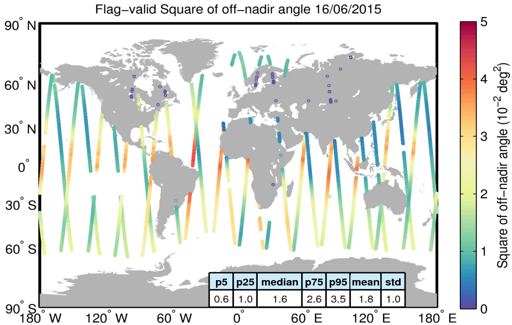
Figure 37. Geographical distribution of flag-valid mispointing data over oceans and lakes for 16/06/2015. The statistical values shown in the table refer to the mispointing in 10^{-2} \text{deg}^2 and are calculated over all measurements shown in the figure.
