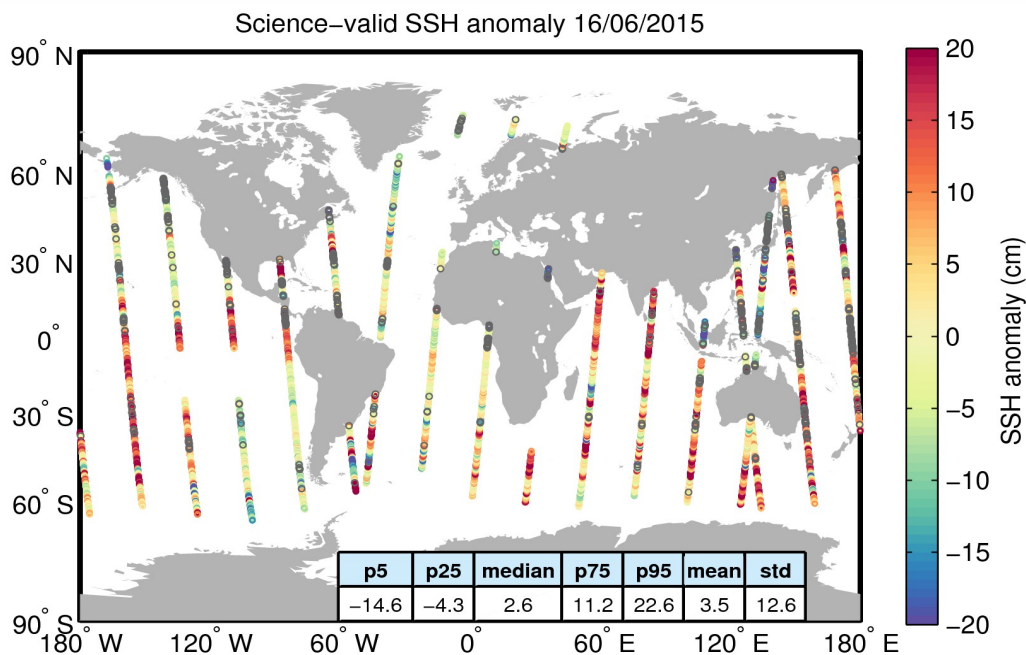
Figure 10. Geographical distribution of science-valid SSH anomaly data over oceans and lakes for 16/06/2015. The statistical values shown in the table refer to the SSH anomaly in cm and are calculated over all measurements shown in the figure. Gray circles denote records that have been rejected based on the editing criteria described in Table 2.
