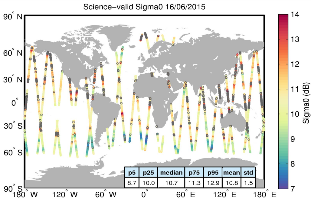
Figure 27. Geographical distribution of science-valid sigma0 data over oceans and lakes for 16/06/2015. The statistical values shown in the table refer to the sigma0 in dB and are calculated over all measurements shown in the figure. Gray circles denote records that have been rejected based on the editing criteria described in Table 4.
