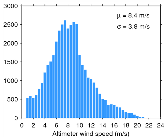
Figure 35. Histogram of science-valid wind over oceans and lakes for 16/06/2015. The mean ( \mu ) and standard deviation ( \sigma ) are also shown. Note that values larger than 24 m/s are excluded from the histogram for the sake of readability but not from the computation of \mu and \sigma .
