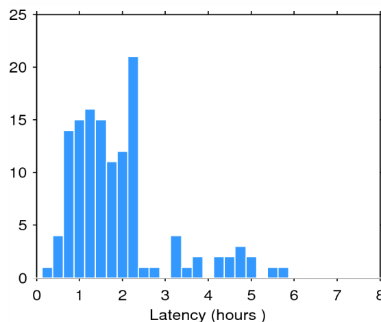
Figure 2. Histogram of the data latency for 16/06/2015. The y-axis denotes the number of files that are made available with a delay of x-hours with respect to the mean time of the records stored in the file.
