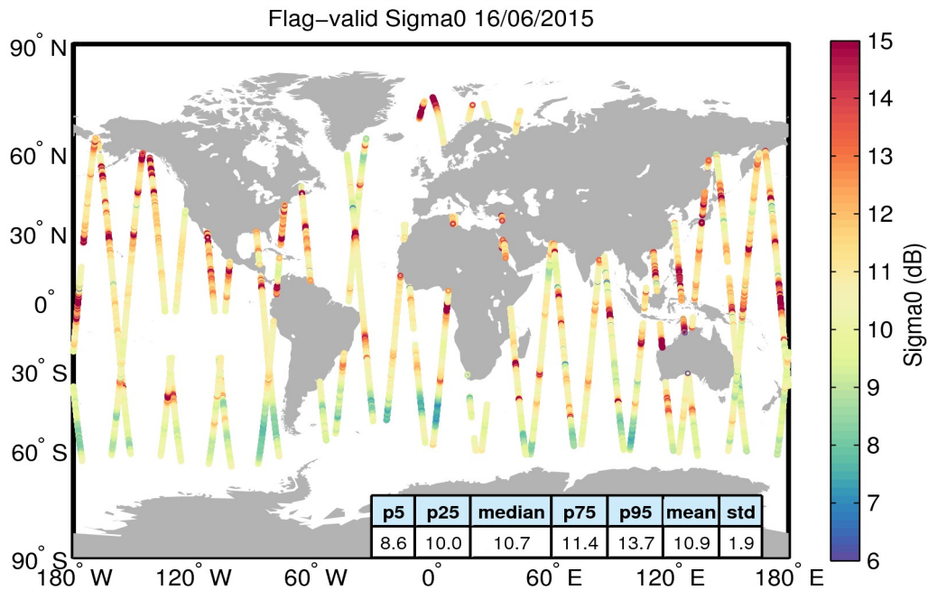
Figure 23. Geographical distribution of flag-valid sigma0 data over oceans and lakes for 16/06/2015. The statistical values shown in the table refer to the sigma0 in dB and are calculated over all measurements shown in the figure.
