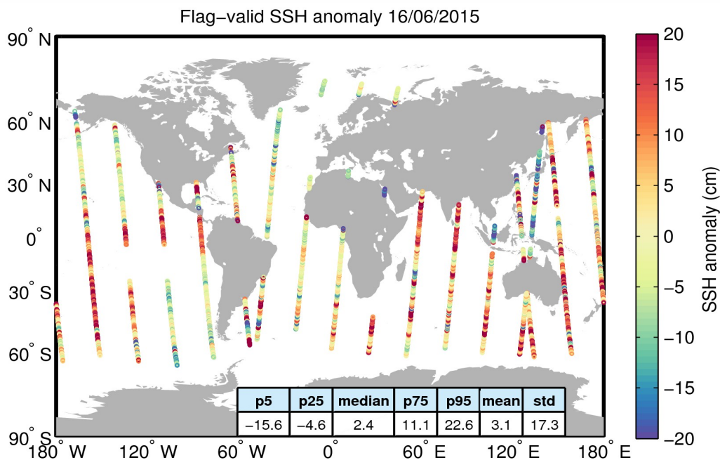
Figure 5. Geographical distribution of flag-valid 1-Hz SSH anomaly data over oceans and lakes for 16/06/2015. The statistical values shown in the table refer to the SSH anomaly in cm and are calculated over all measurements shown in the figure.
