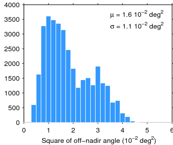
Figure 39. Histogram of flag-valid mispointing over oceans and lakes for 15/06/2015. The mean ( \mu ) and standard deviation ( \sigma ) are also shown. Note that values larger than 6 \cdot 10^{-2} \text{ deg}^2 are excluded from the histogram for the sake of readability but not from the computation of \mu and \sigma .
