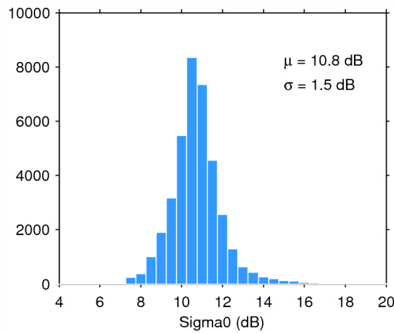
Figure 28. Histogram of science-valid sigma0 over oceans and lakes for 15/06/2015. The mean ( \mu ) and standard deviation ( \sigma ) are also shown. Note that values outside [4 20] dB are excluded from the histogram for the sake of readability but not from the computation of \mu and \sigma .
