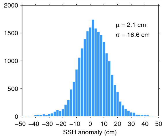
Figure 7. Histogram of flag-valid SSH anomaly over oceans and lakes for 15/06/2015. The mean ( \mu ) and standard deviation ( \sigma ) are also shown. Note that values outside [-50\ 50] cm are excluded from the histogram for the sake of readability but not from the computation of \mu and \sigma .
