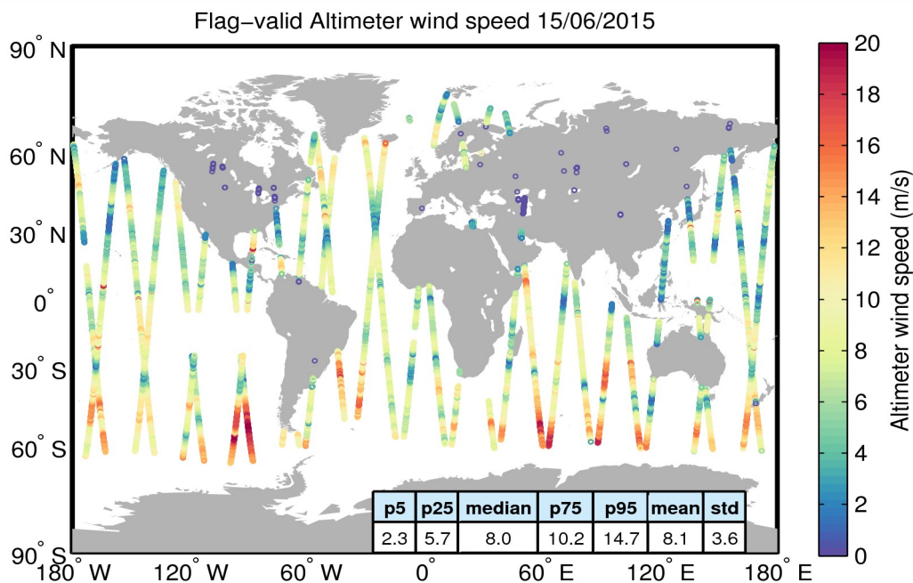
Figure 31. Geographical distribution of flag-valid wind data over oceans and lakes for 15/06/2015. The statistical values shown in the table refer to the wind in m/s and are calculated over all measurements shown in the figure.
