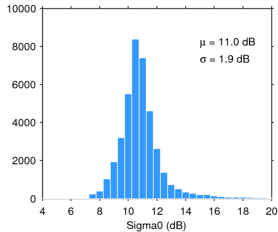
Figure 25. Histogram of flag-valid sigma0 over oceans and lakes for 15/06/2015. The mean ( \mu ) and standard deviation ( \sigma ) are also shown. Note that values outside [4 20] dB are excluded from the histogram for the sake of readability but not from the computation of \mu and \sigma .
