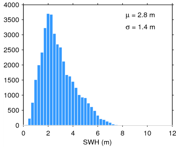
Figure 17. Histogram of flag-valid SWH over oceans and lakes for 15/06/2015. The mean ( \mu ) and standard deviation ( \sigma ) are also shown. Note that values larger than 12 m are excluded from the histogram for the sake of readability but not from the computation of \mu and \sigma .
