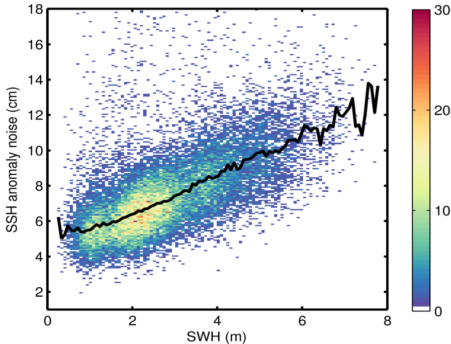
Figure 9. 2D histogram showing flag-valid SSH anomaly noise as a function of SWH for 15/06/2015. The black line denotes the median SSH anomaly as a function of SWH.
