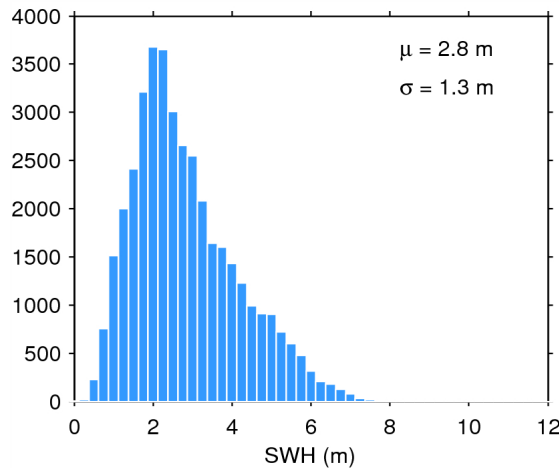
Figure 20. Histogram of science-valid SWH over oceans and lakes for 15/06/2015. The mean ( \mu ) and standard deviation ( \sigma ) are also shown. Note that values larger than 12 m are excluded from the histogram for the sake of readability but not from the computation of \mu and \sigma .
