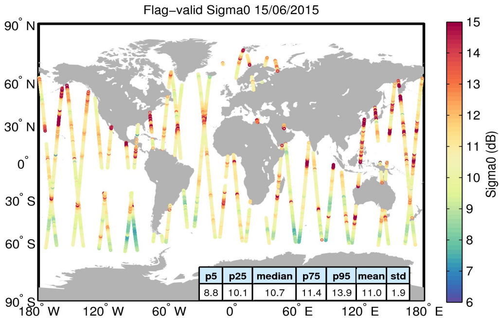
Figure 23. Geographical distribution of flag-valid sigma0 data over oceans and lakes for 15/06/2015. The statistical values shown in the table refer to the sigma0 in dB and are calculated over all measurements shown in the figure.
