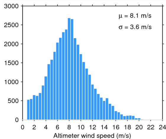
Figure 35. Histogram of science-valid wind over oceans and lakes for 15/06/2015. The mean ( \mu ) and standard deviation ( \sigma ) are also shown. Note that values larger than 24 m/s are excluded from the histogram for the sake of readability but not from the computation of \mu and \sigma .
