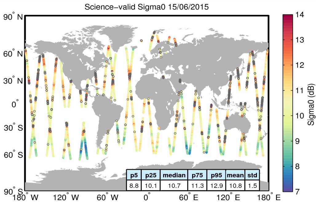
Figure 27. Geographical distribution of science-valid sigma0 data over oceans and lakes for 15/06/2015. The statistical values shown in the table refer to the sigma0 in dB and are calculated over all measurements shown in the figure. Gray circles denote records that have been rejected based on the editing criteria described in Table 4.
