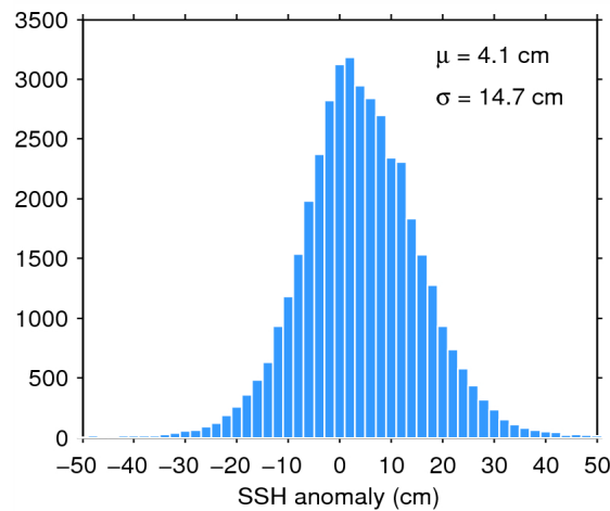
Figure 7. Histogram of flag-valid SSH anomaly over oceans and lakes for 14/06/2015. The mean ( \mu ) and standard deviation ( \sigma ) are also shown. Note that values outside [-50\ 50] cm are excluded from the histogram for the sake of readability but not from the computation of \mu and \sigma .
