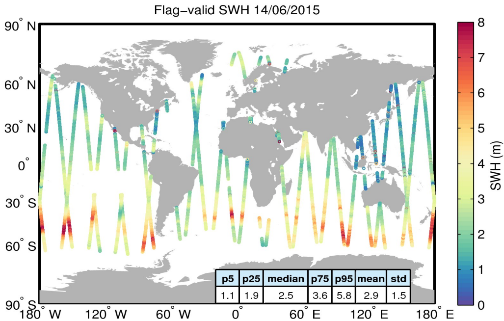
Figure 15. Geographical distribution of flag-valid SWH data over oceans and lakes for 14/06/2015. The statistical values shown in the table refer to the SWH in m and are calculated over all measurements shown in the figure.
