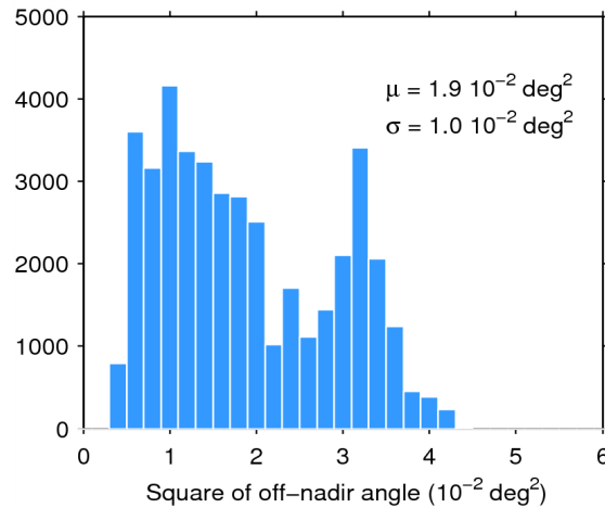
Figure 39. Histogram of flag-valid mispointing over oceans and lakes for 14/06/2015. The mean ( \mu ) and standard deviation ( \sigma ) are also shown. Note that values larger than 6 \cdot 10^{-2} \text{ deg}^2 are excluded from the histogram for the sake of readability but not from the computation of \mu and \sigma .
