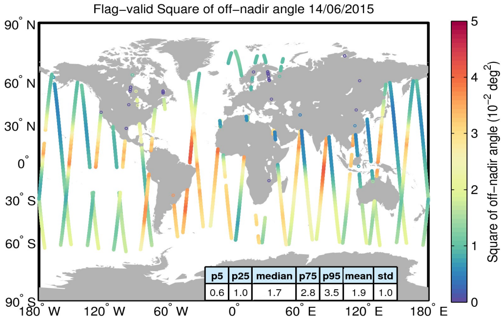
Figure 37. Geographical distribution of flag-valid mispointing data over oceans and lakes for 14/06/2015. The statistical values shown in the table refer to the mispointing in 10^{-2} \text{deg}^2 and are calculated over all measurements shown in the figure.
