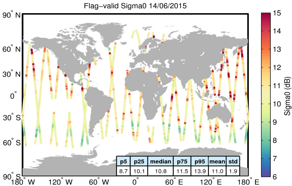
Figure 23. Geographical distribution of flag-valid sigma0 data over oceans and lakes for 14/06/2015. The statistical values shown in the table refer to the sigma0 in dB and are calculated over all measurements shown in the figure.
