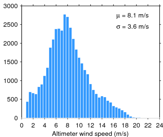
Figure 35. Histogram of science-valid wind over oceans and lakes for 14/06/2015. The mean ( \mu ) and standard deviation ( \sigma ) are also shown. Note that values larger than 24 m/s are excluded from the histogram for the sake of readability but not from the computation of \mu and \sigma .
