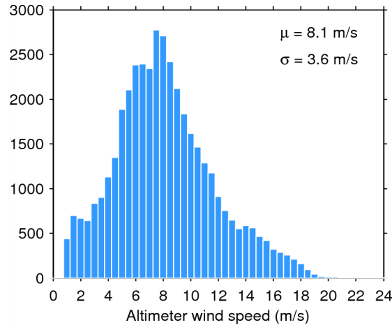
Figure 33. Histogram of flag-valid wind over oceans and lakes for 14/06/2015. The mean ( \mu ) and standard deviation ( \sigma ) are also shown. Note that values larger than 24 m/s are excluded from the histogram for the sake of readability but not from the computation of \mu and \sigma .
