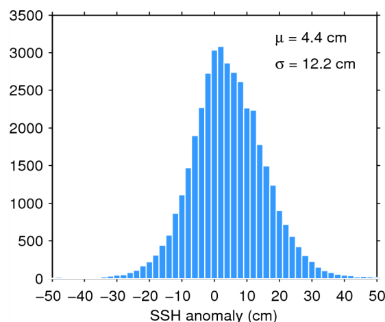
Figure 11. Histogram of science-valid SSH anomaly over oceans and lakes for 14/06/2015. The mean ( \mu ) and standard deviation ( \sigma ) are also shown. Note that values outside [-50 50] cm are excluded from the histogram for the sake of readability but not from the computation of \mu and \sigma .
