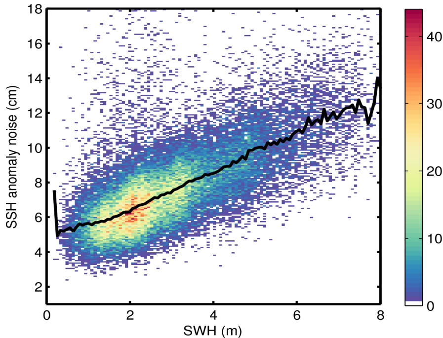
Figure 9. 2D histogram showing flag-valid SSH anomaly noise as a function of SWH for 14/06/2015. The black line denotes the median SSH anomaly as a function of SWH.
