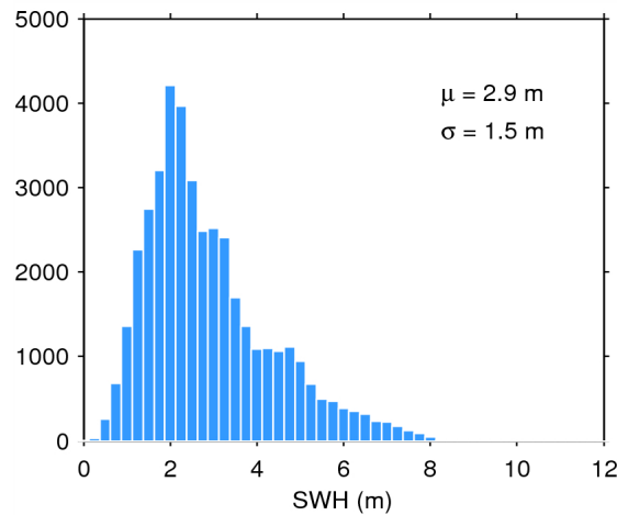
Figure 17. Histogram of flag-valid SWH over oceans and lakes for 14/06/2015. The mean ( \mu ) and standard deviation ( \sigma ) are also shown. Note that values larger than 12 m are excluded from the histogram for the sake of readability but not from the computation of \mu and \sigma .
