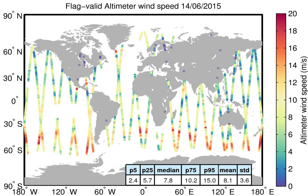
Figure 31. Geographical distribution of flag-valid wind data over oceans and lakes for 14/06/2015. The statistical values shown in the table refer to the wind in m/s and are calculated over all measurements shown in the figure.
