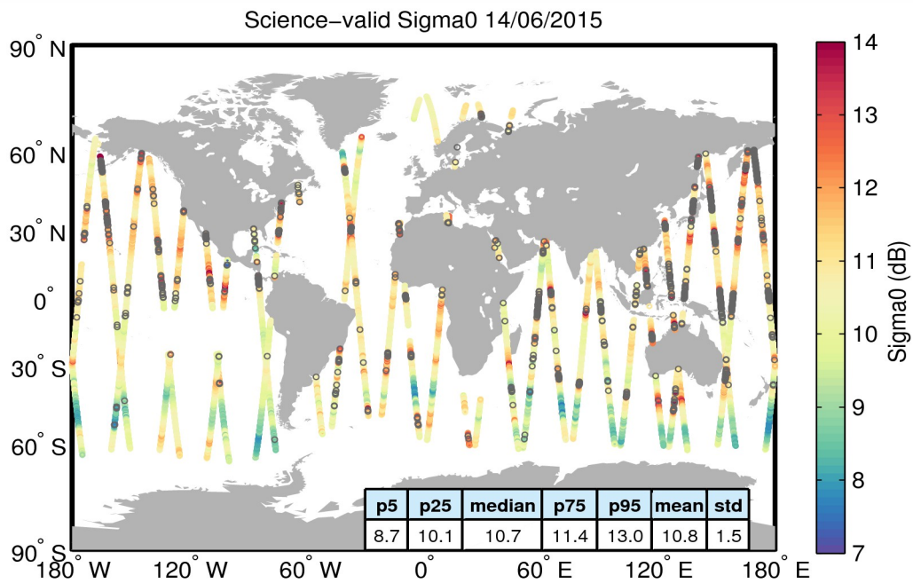
Figure 27. Geographical distribution of science-valid sigma0 data over oceans and lakes for 14/06/2015. The statistical values shown in the table refer to the sigma0 in dB and are calculated over all measurements shown in the figure. Gray circles denote records that have been rejected based on the editing criteria described in Table 4.
