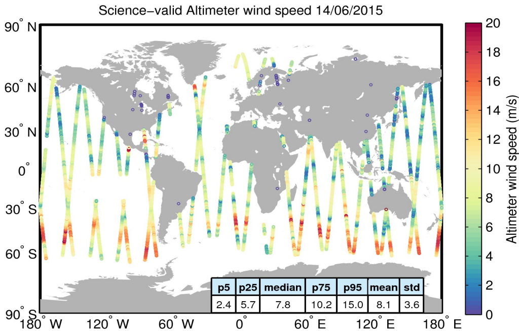
Figure 34. Geographical distribution of science-valid wind data over oceans and lakes for 14/06/2015. The statistical values shown in the table refer to the wind in m/s and are calculated over all measurements shown in the figure. Gray circles denote records that have been rejected based on the editing criteria described in Table 5.
