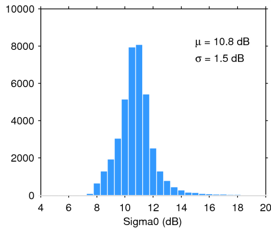
Figure 28. Histogram of science-valid sigma0 over oceans and lakes for 14/06/2015. The mean ( \mu ) and standard deviation ( \sigma ) are also shown. Note that values outside [4 20] dB are excluded from the histogram for the sake of readability but not from the computation of \mu and \sigma .
