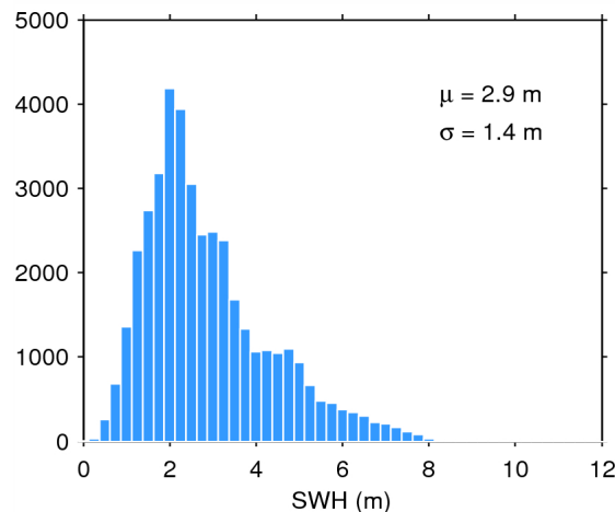
Figure 20. Histogram of science-valid SWH over oceans and lakes for 14/06/2015. The mean ( \mu ) and standard deviation ( \sigma ) are also shown. Note that values larger than 12 m are excluded from the histogram for the sake of readability but not from the computation of \mu and \sigma .
