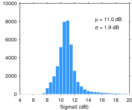
Figure 25. Histogram of flag-valid sigma0 over oceans and lakes for 14/06/2015. The mean ( \mu ) and standard deviation ( \sigma ) are also shown. Note that values outside [4 20] dB are excluded from the histogram for the sake of readability but not from the computation of \mu and \sigma .
