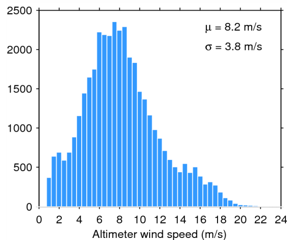
Figure 35. Histogram of science-valid wind over oceans and lakes for 13/06/2015. The mean ( \mu ) and standard deviation ( \sigma ) are also shown. Note that values larger than 24 m/s are excluded from the histogram for the sake of readability but not from the computation of \mu and \sigma .
