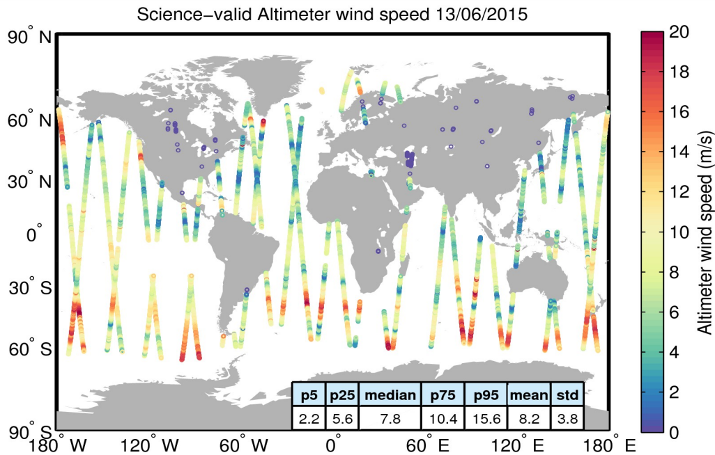
Figure 34. Geographical distribution of science-valid wind data over oceans and lakes for 13/06/2015. The statistical values shown in the table refer to the wind in m/s and are calculated over all measurements shown in the figure. Gray circles denote records that have been rejected based on the editing criteria described in Table 5.
