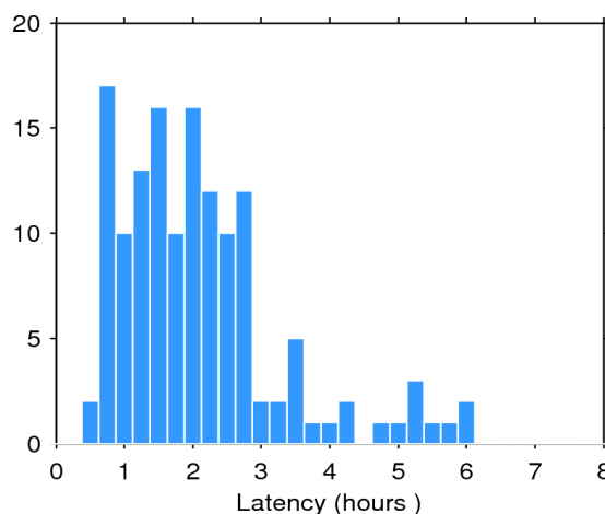
Figure 2. Histogram of the data latency for 13/06/2015. The y-axis denotes the number of files that are made available with a delay of x-hours with respect to the mean time of the records stored in the file.
