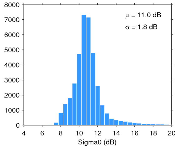
Figure 25. Histogram of flag-valid sigma0 over oceans and lakes for 13/06/2015. The mean ( \mu ) and standard deviation ( \sigma ) are also shown. Note that values outside [4 20] dB are excluded from the histogram for the sake of readability but not from the computation of \mu and \sigma .
