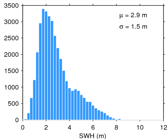
Figure 20. Histogram of science-valid SWH over oceans and lakes for 13/06/2015. The mean ( \mu ) and standard deviation ( \sigma ) are also shown. Note that values larger than 12 m are excluded from the histogram for the sake of readability but not from the computation of \mu and \sigma .
