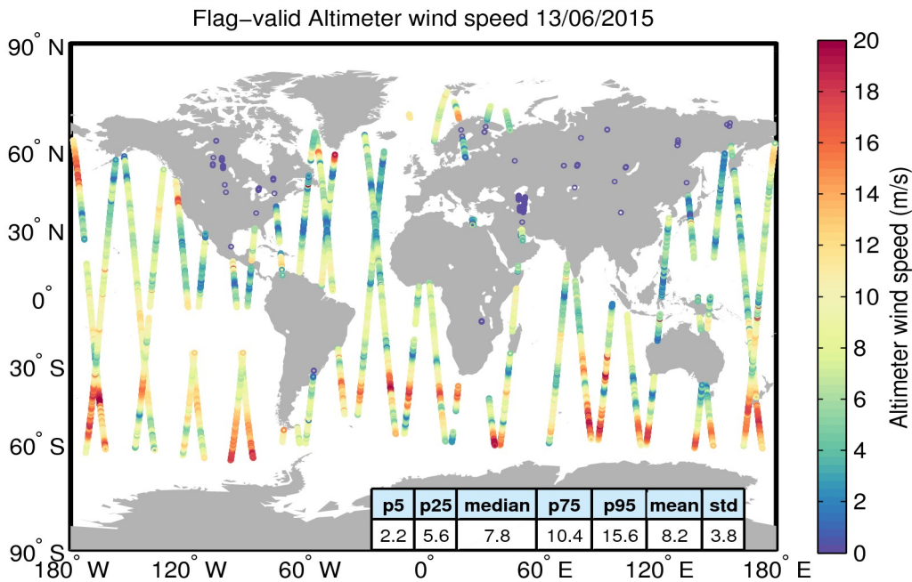
Figure 31. Geographical distribution of flag-valid wind data over oceans and lakes for 13/06/2015. The statistical values shown in the table refer to the wind in m/s and are calculated over all measurements shown in the figure.
