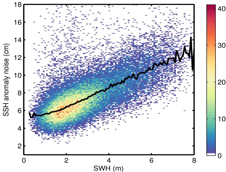
Figure 9. 2D histogram showing flag-valid SSH anomaly noise as a function of SWH for 13/06/2015. The black line denotes the median SSH anomaly as a function of SWH.
