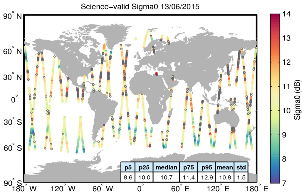
Figure 27. Geographical distribution of science-valid sigma0 data over oceans and lakes for 13/06/2015. The statistical values shown in the table refer to the sigma0 in dB and are calculated over all measurements shown in the figure. Gray circles denote records that have been rejected based on the editing criteria described in Table 4.
