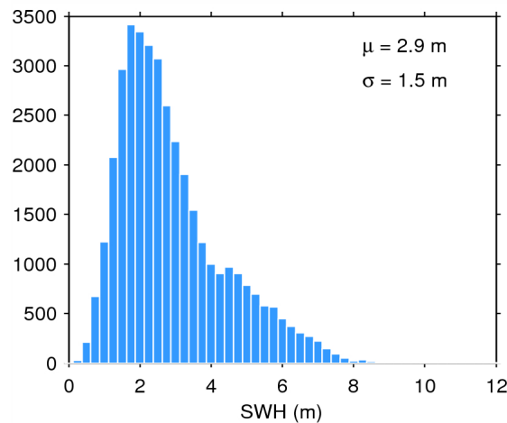
Figure 17. Histogram of flag-valid SWH over oceans and lakes for 13/06/2015. The mean ( \mu ) and standard deviation ( \sigma ) are also shown. Note that values larger than 12 m are excluded from the histogram for the sake of readability but not from the computation of \mu and \sigma .
