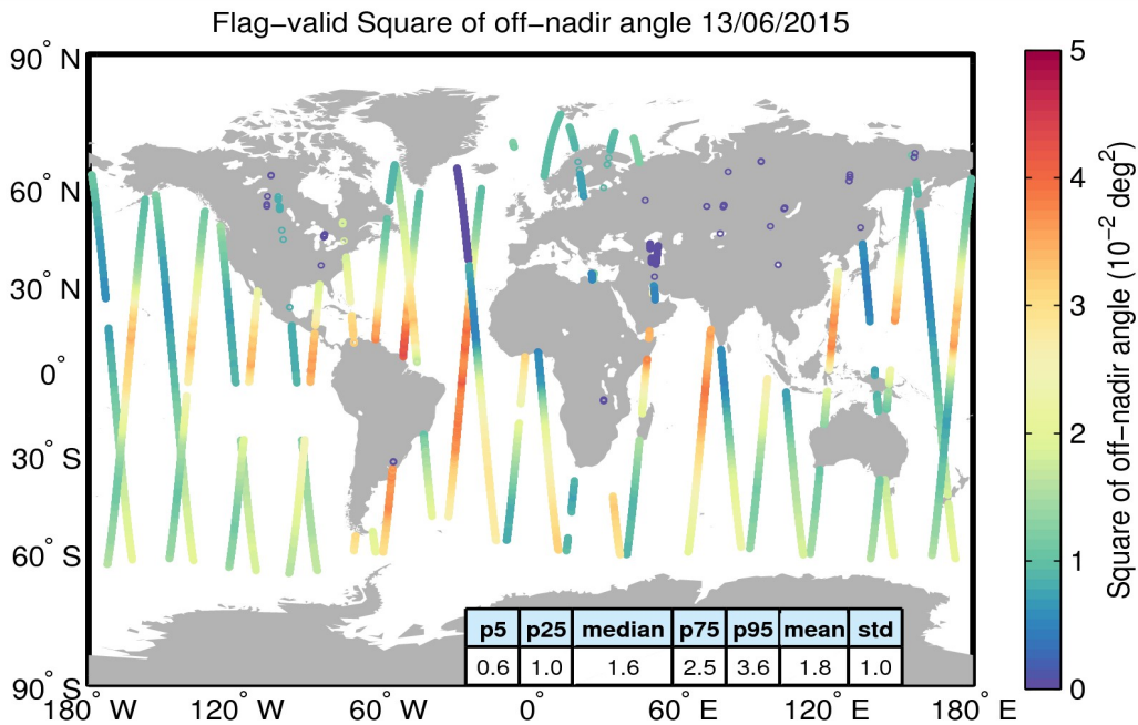
Figure 37. Geographical distribution of flag-valid mispointing data over oceans and lakes for 13/06/2015. The statistical values shown in the table refer to the mispointing in 10^{-2} \text{deg}^2 and are calculated over all measurements shown in the figure.
