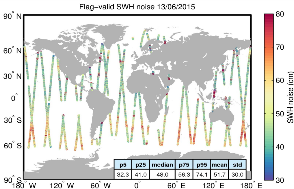
Figure 18. Geographical distribution of flag-valid 20-Hz SWH measurement noise over oceans and lakes for 13/06/2015. The statistical values shown in the figure refer to the SWH noise and are calculated over all measurements shown in the figure.
