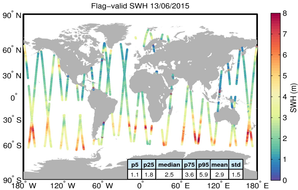
Figure 15. Geographical distribution of flag-valid SWH data over oceans and lakes for 13/06/2015. The statistical values shown in the table refer to the SWH in m and are calculated over all measurements shown in the figure.
