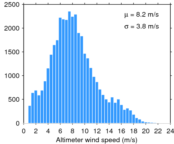
Figure 33. Histogram of flag-valid wind over oceans and lakes for 13/06/2015. The mean ( \mu ) and standard deviation ( \sigma ) are also shown. Note that values larger than 24 m/s are excluded from the histogram for the sake of readability but not from the computation of \mu and \sigma .
