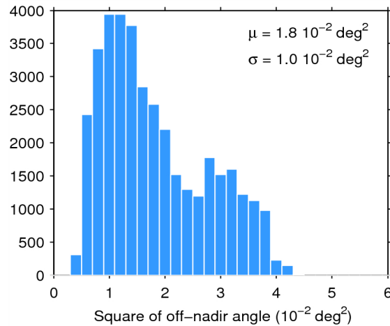
Figure 39. Histogram of flag-valid mispointing over oceans and lakes for 13/06/2015. The mean ( \mu ) and standard deviation ( \sigma ) are also shown. Note that values larger than 6 \cdot 10^{-2} \text{ deg}^2 are excluded from the histogram for the sake of readability but not from the computation of \mu and \sigma .
