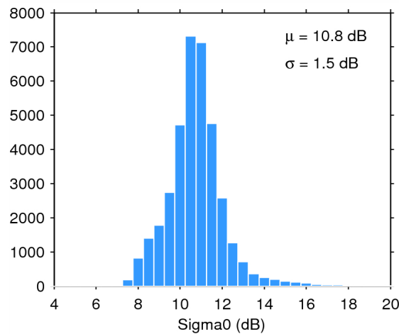
Figure 28. Histogram of science-valid sigma0 over oceans and lakes for 13/06/2015. The mean ( \mu ) and standard deviation ( \sigma ) are also shown. Note that values outside [4 20] dB are excluded from the histogram for the sake of readability but not from the computation of \mu and \sigma .
