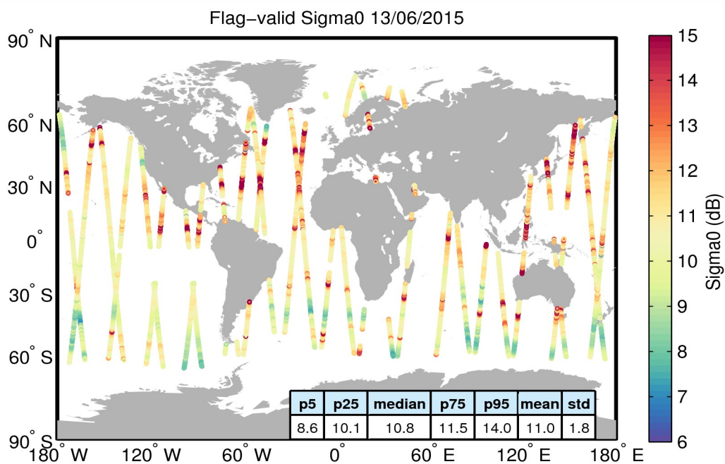
Figure 23. Geographical distribution of flag-valid sigma0 data over oceans and lakes for 13/06/2015. The statistical values shown in the table refer to the sigma0 in dB and are calculated over all measurements shown in the figure.
