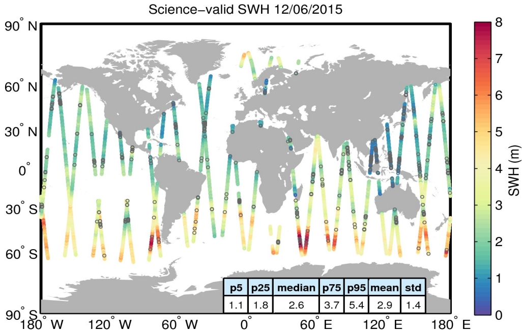
Figure 19. Geographical distribution of science-valid SWH data over oceans and lakes for 12/06/2015. The statistical values shown in the table refer to the SWH in m and are calculated over all measurements shown in the figure. Gray circles denote records that have been rejected based on the editing criteria described in Table 3.
