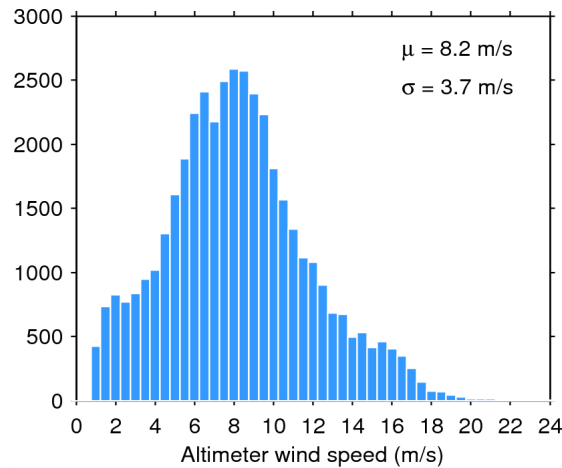
Figure 33. Histogram of flag-valid wind over oceans and lakes for 12/06/2015. The mean ( \mu ) and standard deviation ( \sigma ) are also shown. Note that values larger than 24 m/s are excluded from the histogram for the sake of readability but not from the computation of \mu and \sigma .
