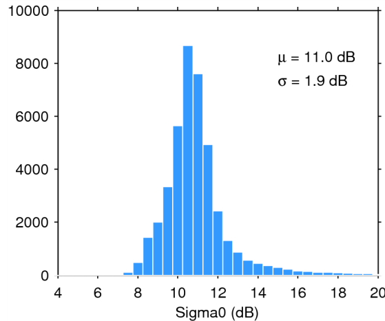
Figure 25. Histogram of flag-valid sigma0 over oceans and lakes for 12/06/2015. The mean ( \mu ) and standard deviation ( \sigma ) are also shown. Note that values outside [4 20] dB are excluded from the histogram for the sake of readability but not from the computation of \mu and \sigma .
