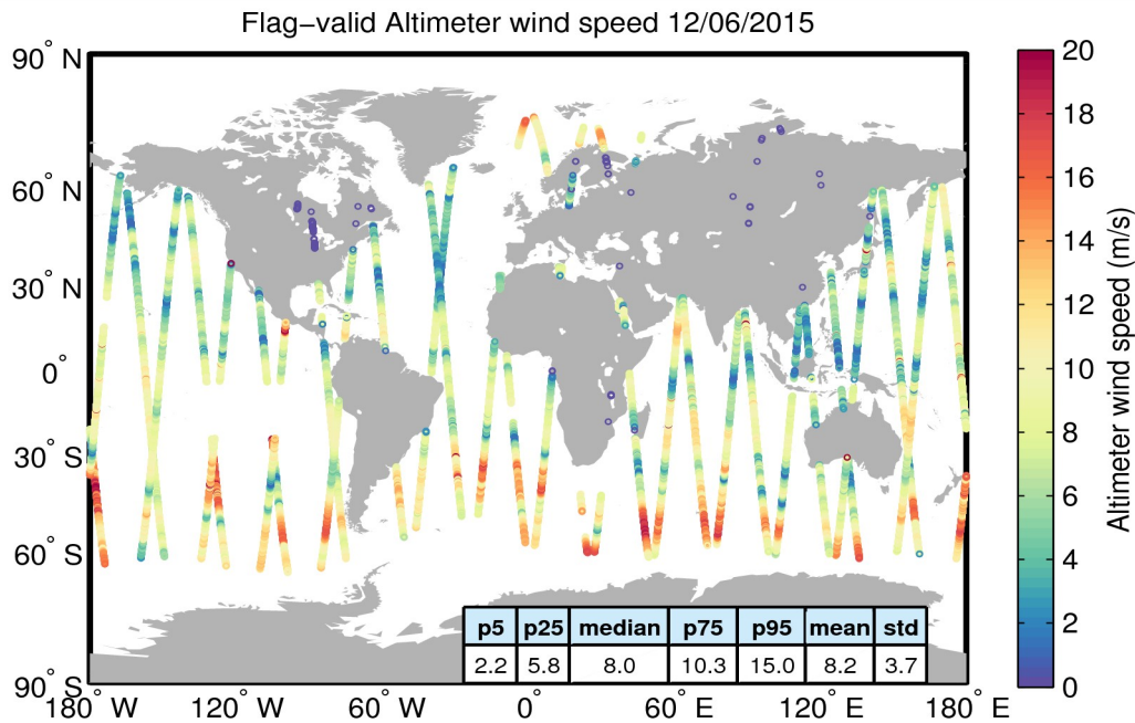
Figure 31. Geographical distribution of flag-valid wind data over oceans and lakes for 12/06/2015. The statistical values shown in the table refer to the wind in m/s and are calculated over all measurements shown in the figure.
