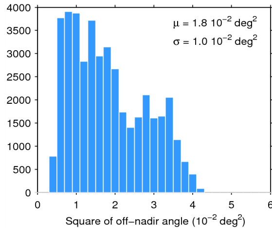
Figure 39. Histogram of flag-valid mispointing over oceans and lakes for 12/06/2015. The mean ( \mu ) and standard deviation ( \sigma ) are also shown. Note that values larger than 6 \cdot 10^{-2} \text{ deg}^2 are excluded from the histogram for the sake of readability but not from the computation of \mu and \sigma .
