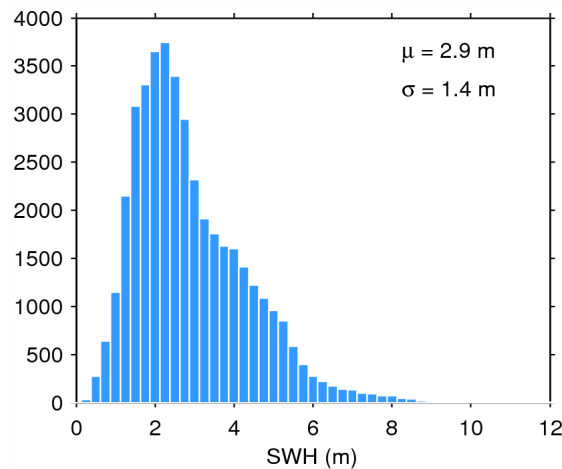
Figure 17. Histogram of flag-valid SWH over oceans and lakes for 12/06/2015. The mean ( \mu ) and standard deviation ( \sigma ) are also shown. Note that values larger than 12 m are excluded from the histogram for the sake of readability but not from the computation of \mu and \sigma .
