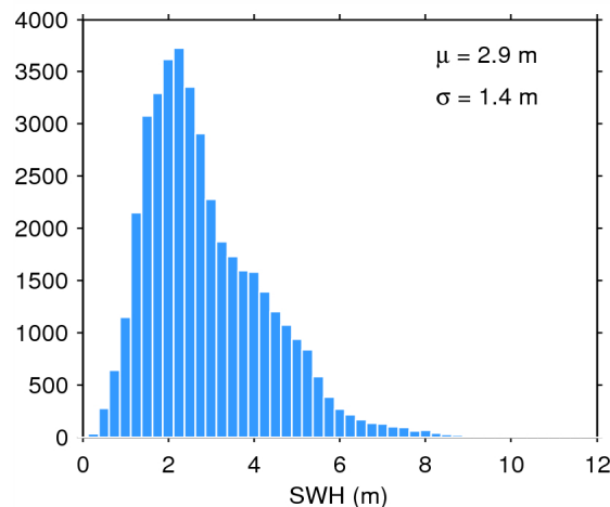
Figure 20. Histogram of science-valid SWH over oceans and lakes for 12/06/2015. The mean ( \mu ) and standard deviation ( \sigma ) are also shown. Note that values larger than 12 m are excluded from the histogram for the sake of readability but not from the computation of \mu and \sigma .
