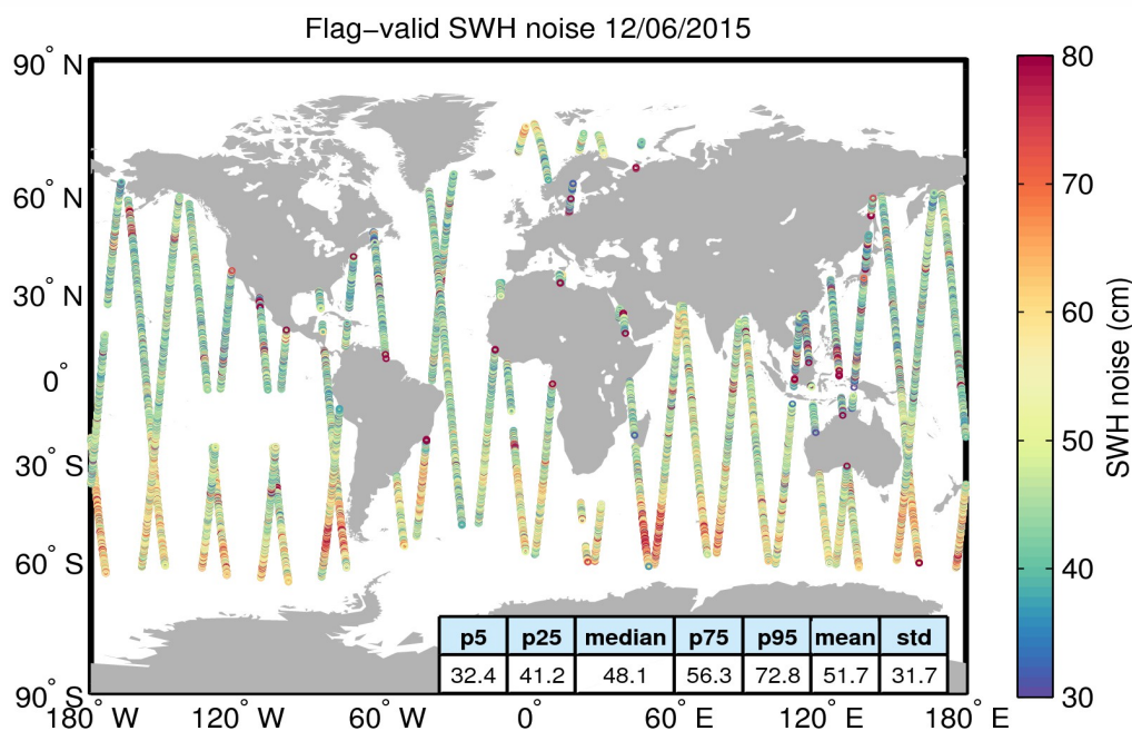
Figure 18. Geographical distribution of flag-valid 20-Hz SWH measurement noise over oceans and lakes for 12/06/2015. The statistical values shown in the figure refer to the SWH noise and are calculated over all measurements shown in the figure.
