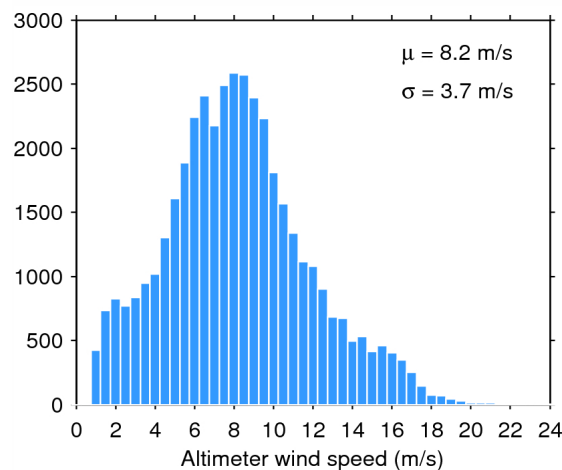
Figure 35. Histogram of science-valid wind over oceans and lakes for 12/06/2015. The mean ( \mu ) and standard deviation ( \sigma ) are also shown. Note that values larger than 24 m/s are excluded from the histogram for the sake of readability but not from the computation of \mu and \sigma .
