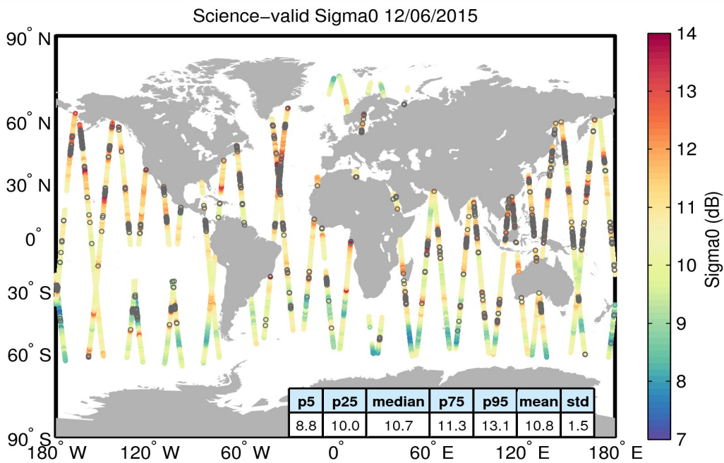
Figure 27. Geographical distribution of science-valid sigma0 data over oceans and lakes for 12/06/2015. The statistical values shown in the table refer to the sigma0 in dB and are calculated over all measurements shown in the figure. Gray circles denote records that have been rejected based on the editing criteria described in Table 4.
