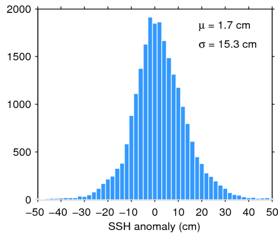
Figure 7. Histogram of flag-valid SSH anomaly over oceans and lakes for 12/06/2015. The mean ( \mu ) and standard deviation ( \sigma ) are also shown. Note that values outside [-50\ 50] cm are excluded from the histogram for the sake of readability but not from the computation of \mu and \sigma .
