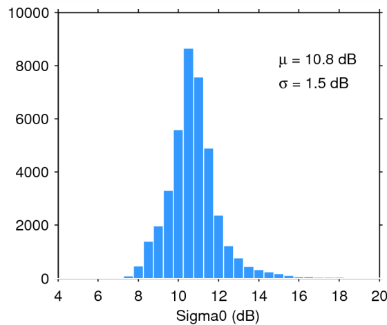
Figure 28. Histogram of science-valid sigma0 over oceans and lakes for 12/06/2015. The mean ( \mu ) and standard deviation ( \sigma ) are also shown. Note that values outside [4 20] dB are excluded from the histogram for the sake of readability but not from the computation of \mu and \sigma .
