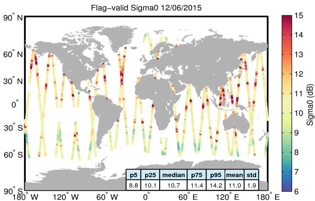
Figure 23. Geographical distribution of flag-valid sigma0 data over oceans and lakes for 12/06/2015. The statistical values shown in the table refer to the sigma0 in dB and are calculated over all measurements shown in the figure.
