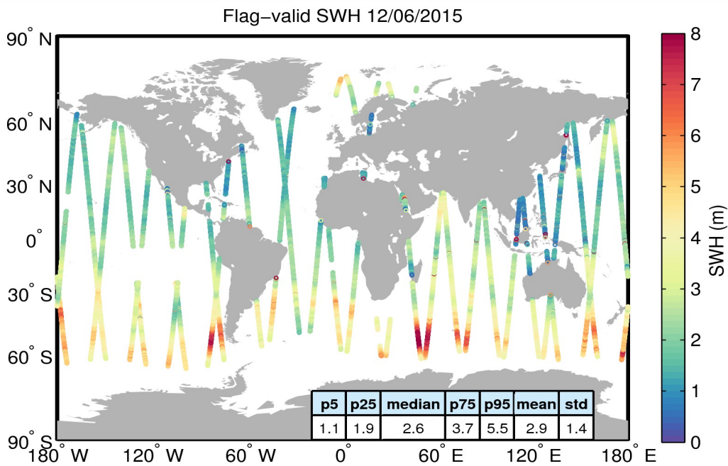
Figure 15. Geographical distribution of flag-valid SWH data over oceans and lakes for 12/06/2015. The statistical values shown in the table refer to the SWH in m and are calculated over all measurements shown in the figure.
