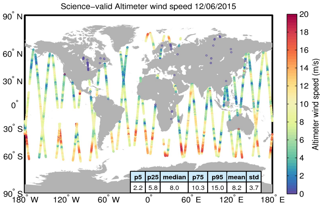
Figure 34. Geographical distribution of science-valid wind data over oceans and lakes for 12/06/2015. The statistical values shown in the table refer to the wind in m/s and are calculated over all measurements shown in the figure. Gray circles denote records that have been rejected based on the editing criteria described in Table 5.
