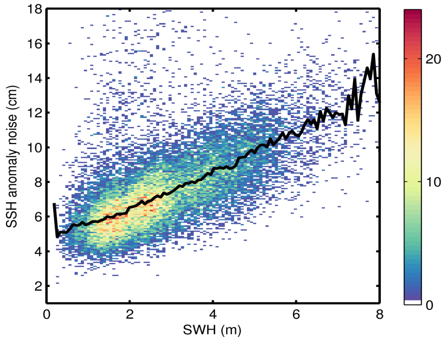
Figure 9. 2D histogram showing flag-valid SSH anomaly noise as a function of SWH for 12/06/2015. The black line denotes the median SSH anomaly as a function of SWH.
