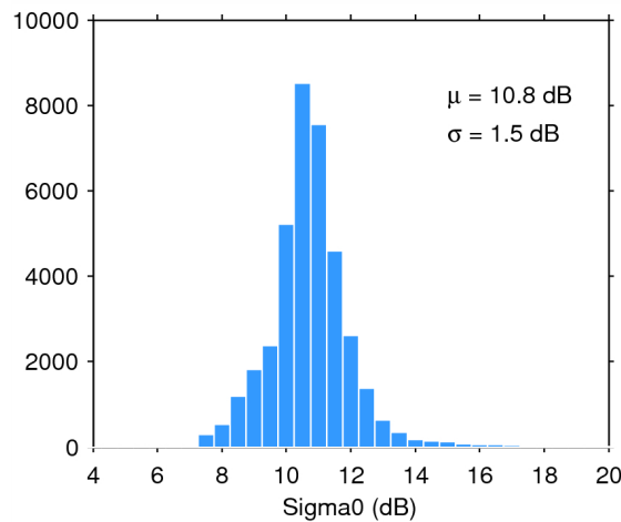
Figure 28. Histogram of science-valid sigma0 over oceans and lakes for 11/06/2015. The mean ( \mu ) and standard deviation ( \sigma ) are also shown. Note that values outside [4 20] dB are excluded from the histogram for the sake of readability but not from the computation of \mu and \sigma .
