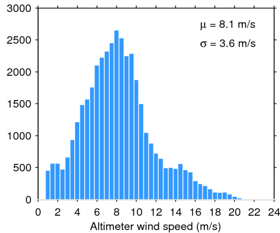
Figure 33. Histogram of flag-valid wind over oceans and lakes for 11/06/2015. The mean ( \mu ) and standard deviation ( \sigma ) are also shown. Note that values larger than 24 m/s are excluded from the histogram for the sake of readability but not from the computation of \mu and \sigma .
