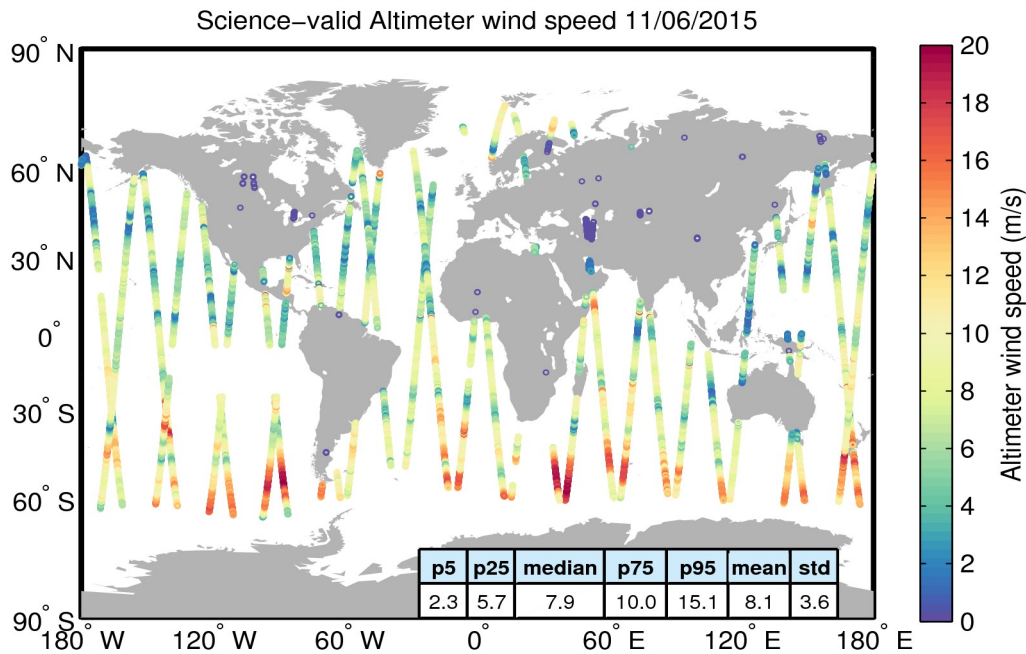
Figure 34. Geographical distribution of science-valid wind data over oceans and lakes for 11/06/2015. The statistical values shown in the table refer to the wind in m/s and are calculated over all measurements shown in the figure. Gray circles denote records that have been rejected based on the editing criteria described in Table 5.
