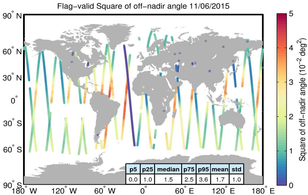
Figure 37. Geographical distribution of flag-valid mispointing data over oceans and lakes for 11/06/2015. The statistical values shown in the table refer to the mispointing in 10^{-2} \text{deg}^2 and are calculated over all measurements shown in the figure.
