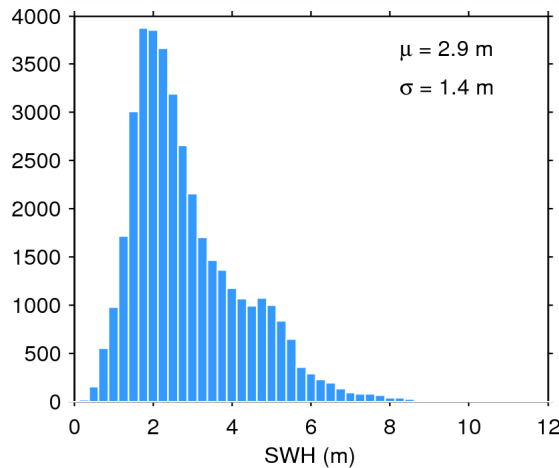
Figure 20. Histogram of science-valid SWH over oceans and lakes for 11/06/2015. The mean ( \mu ) and standard deviation ( \sigma ) are also shown. Note that values larger than 12 m are excluded from the histogram for the sake of readability but not from the computation of \mu and \sigma .
