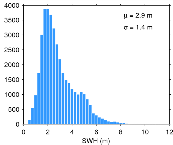
Figure 17. Histogram of flag-valid SWH over oceans and lakes for 11/06/2015. The mean ( \mu ) and standard deviation ( \sigma ) are also shown. Note that values larger than 12 m are excluded from the histogram for the sake of readability but not from the computation of \mu and \sigma .
