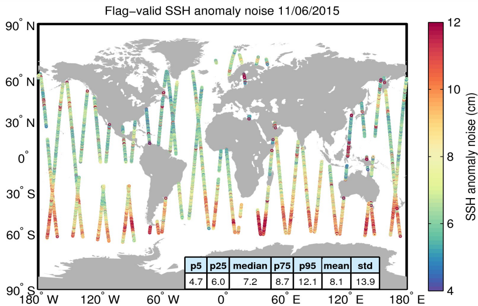
Figure 8. Geographical distribution of flag-valid 20-Hz SSH anomaly measurement noise over oceans and lakes for 11/06/2015. The statistical values shown in the table refer to the SSH anomaly noise and are calculated over all measurements shown in the figure.
