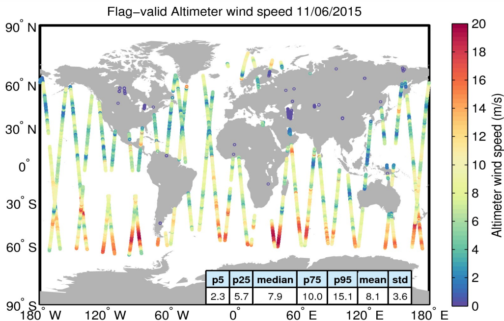
Figure 31. Geographical distribution of flag-valid wind data over oceans and lakes for 11/06/2015. The statistical values shown in the table refer to the wind in m/s and are calculated over all measurements shown in the figure.
