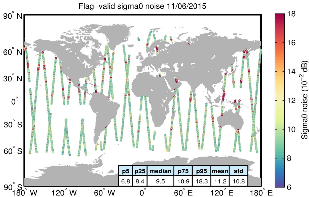
Figure 26. Geographical distribution of flag-valid 20-Hz sigma0 measurement noise over oceans and lakes for 11/06/2015. The statistical values shown in the table refer to the sigma0 noise and are calculated over all measurements shown in the figure.
