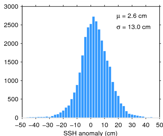
Figure 11. Histogram of science-valid SSH anomaly over oceans and lakes for 11/06/2015. The mean ( \mu ) and standard deviation ( \sigma ) are also shown. Note that values outside [-50, 50] cm are excluded from the histogram for the sake of readability but not from the computation of \mu and \sigma .
