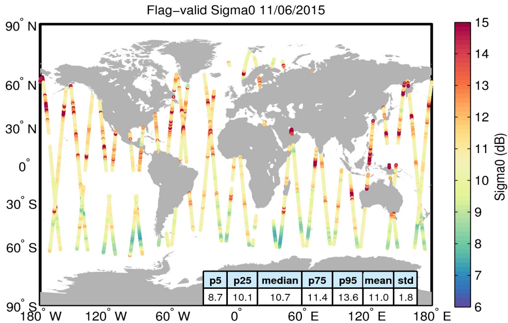
Figure 23. Geographical distribution of flag-valid sigma0 data over oceans and lakes for 11/06/2015. The statistical values shown in the table refer to the sigma0 in dB and are calculated over all measurements shown in the figure.
