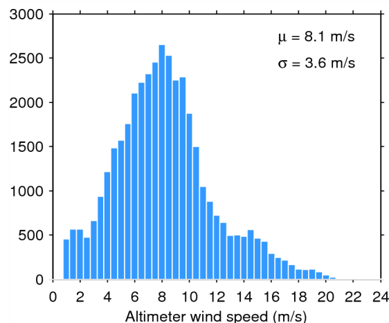
Figure 35. Histogram of science-valid wind over oceans and lakes for 11/06/2015. The mean ( \mu ) and standard deviation ( \sigma ) are also shown. Note that values larger than 24 m/s are excluded from the histogram for the sake of readability but not from the computation of \mu and \sigma .
