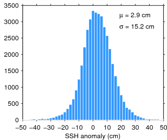
Figure 7. Histogram of flag-valid SSH anomaly over oceans and lakes for 10/06/2015. The mean ( \mu ) and standard deviation ( \sigma ) are also shown. Note that values outside [-50\ 50] cm are excluded from the histogram for the sake of readability but not from the computation of \mu and \sigma .
