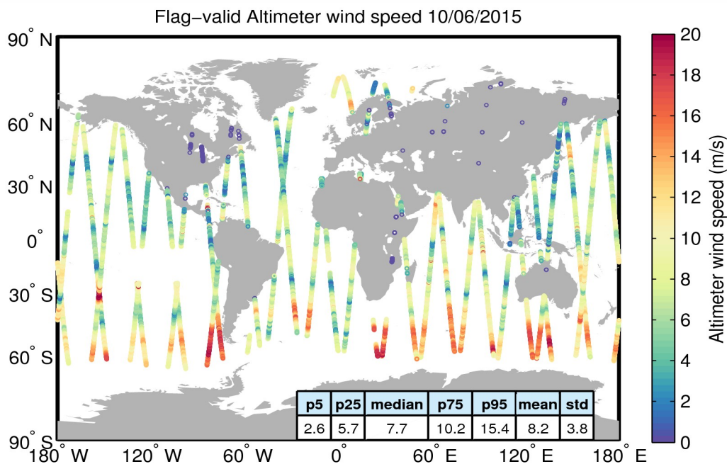
Figure 31. Geographical distribution of flag-valid wind data over oceans and lakes for 10/06/2015. The statistical values shown in the table refer to the wind in m/s and are calculated over all measurements shown in the figure.
