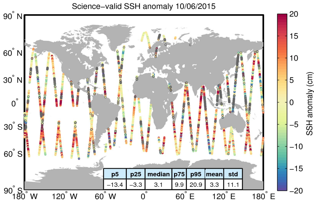
Figure 10. Geographical distribution of science-valid SSH anomaly data over oceans and lakes for 10/06/2015. The statistical values shown in the table refer to the SSH anomaly in cm and are calculated over all measurements shown in the figure. Gray circles denote records that have been rejected based on the editing criteria described in Table 2.
