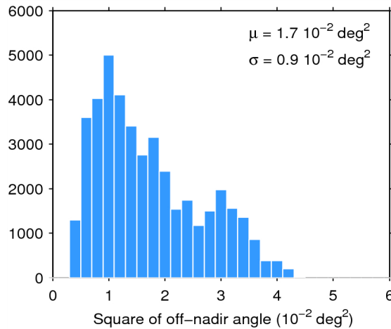
Figure 39. Histogram of flag-valid mispointing over oceans and lakes for 10/06/2015. The mean ( \mu ) and standard deviation ( \sigma ) are also shown. Note that values larger than 6 \cdot 10^{-2} \text{ deg}^2 are excluded from the histogram for the sake of readability but not from the computation of \mu and \sigma .
