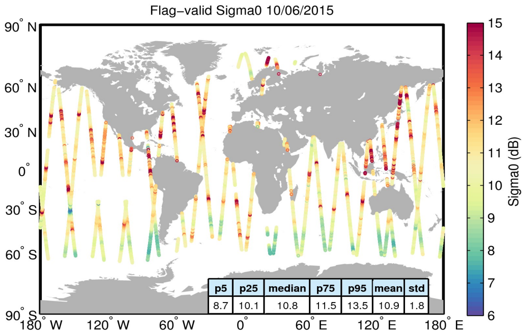
Figure 23. Geographical distribution of flag-valid sigma0 data over oceans and lakes for 10/06/2015. The statistical values shown in the table refer to the sigma0 in dB and are calculated over all measurements shown in the figure.
