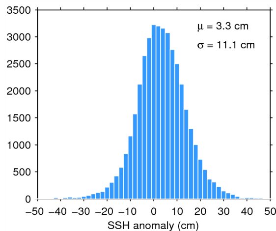
Figure 11. Histogram of science-valid SSH anomaly over oceans and lakes for 10/06/2015. The mean ( \mu ) and standard deviation ( \sigma ) are also shown. Note that values outside [-50 50] cm are excluded from the histogram for the sake of readability but not from the computation of \mu and \sigma .
