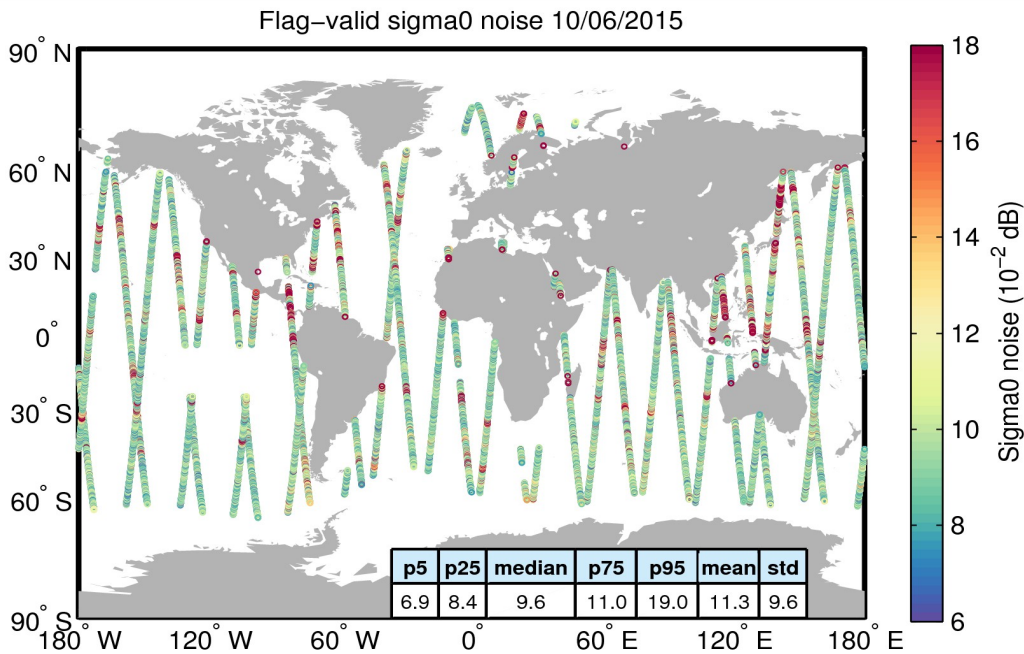
Figure 26. Geographical distribution of flag-valid 20-Hz sigma0 measurement noise over oceans and lakes for 10/06/2015. The statistical values shown in the table refer to the sigma0 noise and are calculated over all measurements shown in the figure.
