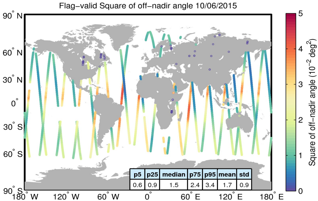
Figure 37. Geographical distribution of flag-valid mispointing data over oceans and lakes for 10/06/2015. The statistical values shown in the table refer to the mispointing in 10^{-2} \text{deg}^2 and are calculated over all measurements shown in the figure.
