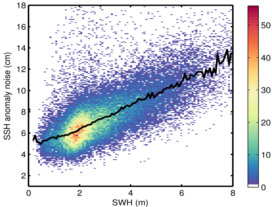
Figure 9. 2D histogram showing flag-valid SSH anomaly noise as a function of SWH for 10/06/2015. The black line denotes the median SSH anomaly as a function of SWH.
