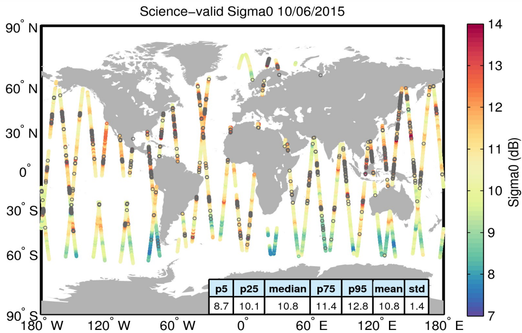
Figure 27. Geographical distribution of science-valid sigma0 data over oceans and lakes for 10/06/2015. The statistical values shown in the table refer to the sigma0 in dB and are calculated over all measurements shown in the figure. Gray circles denote records that have been rejected based on the editing criteria described in Table 4.
