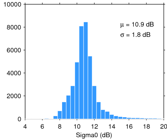
Figure 25. Histogram of flag-valid sigma0 over oceans and lakes for 10/06/2015. The mean ( \mu ) and standard deviation ( \sigma ) are also shown. Note that values outside [4 20] dB are excluded from the histogram for the sake of readability but not from the computation of \mu and \sigma .
