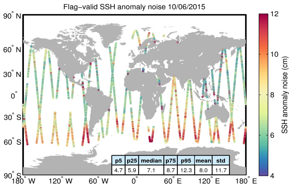
Figure 8. Geographical distribution of flag-valid 20-Hz SSH anomaly measurement noise over oceans and lakes for 10/06/2015. The statistical values shown in the table refer to the SSH anomaly noise and are calculated over all measurements shown in the figure.
