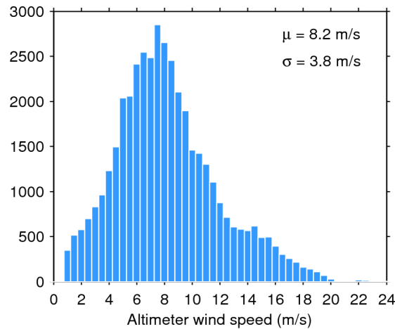
Figure 33. Histogram of flag-valid wind over oceans and lakes for 10/06/2015. The mean ( \mu ) and standard deviation ( \sigma ) are also shown. Note that values larger than 24 m/s are excluded from the histogram for the sake of readability but not from the computation of \mu and \sigma .
