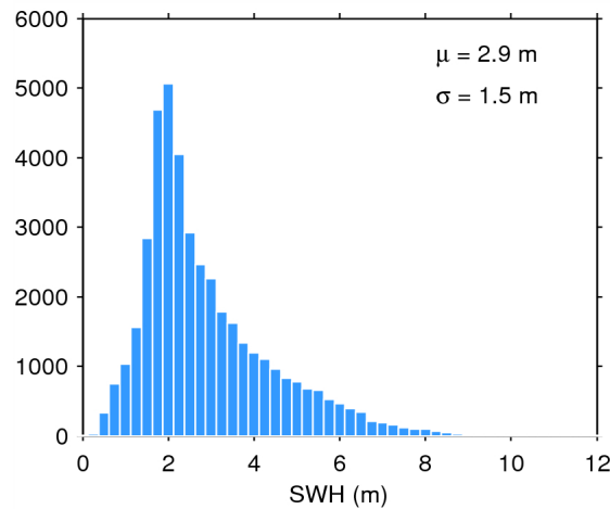
Figure 17. Histogram of flag-valid SWH over oceans and lakes for 10/06/2015. The mean ( \mu ) and standard deviation ( \sigma ) are also shown. Note that values larger than 12 m are excluded from the histogram for the sake of readability but not from the computation of \mu and \sigma .
