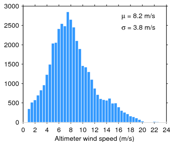
Figure 35. Histogram of science-valid wind over oceans and lakes for 10/06/2015. The mean ( \mu ) and standard deviation ( \sigma ) are also shown. Note that values larger than 24 m/s are excluded from the histogram for the sake of readability but not from the computation of \mu and \sigma .
