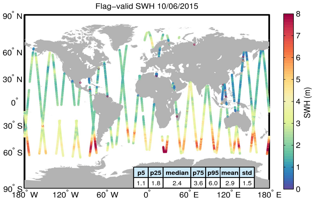
Figure 15. Geographical distribution of flag-valid SWH data over oceans and lakes for 10/06/2015. The statistical values shown in the table refer to the SWH in m and are calculated over all measurements shown in the figure.
