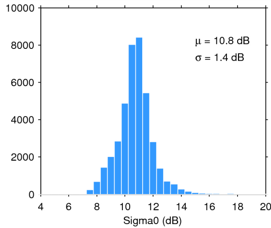
Figure 28. Histogram of science-valid sigma0 over oceans and lakes for 10/06/2015. The mean ( \mu ) and standard deviation ( \sigma ) are also shown. Note that values outside [4 20] dB are excluded from the histogram for the sake of readability but not from the computation of \mu and \sigma .
