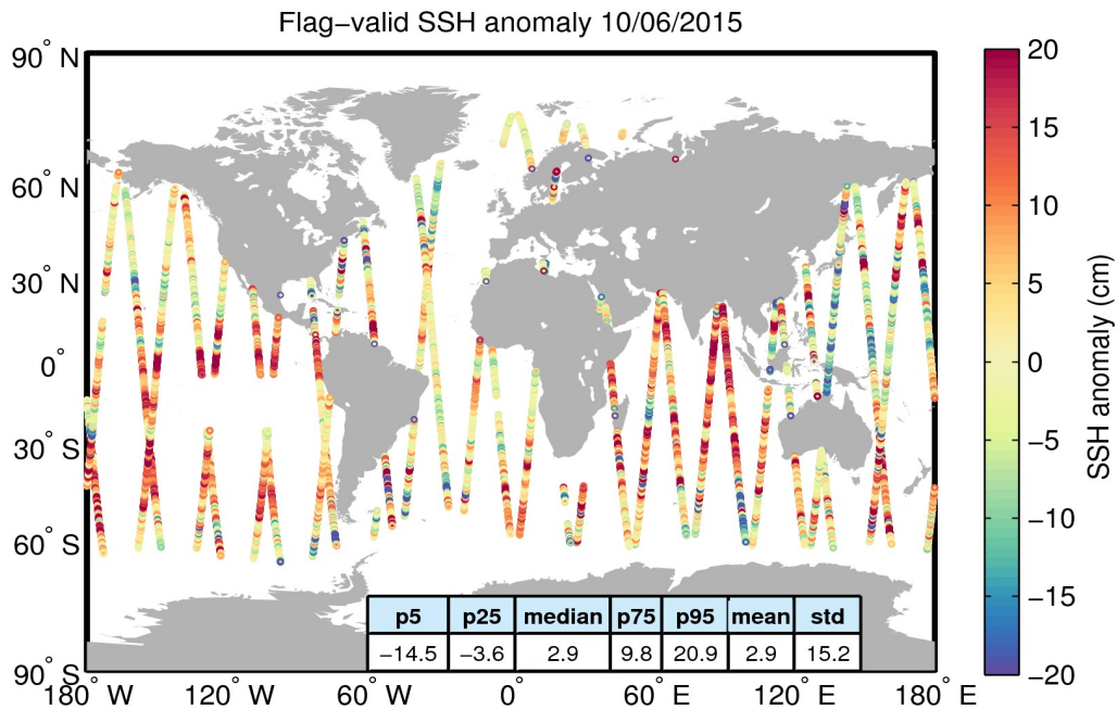
Figure 5. Geographical distribution of flag-valid 1-Hz SSH anomaly data over oceans and lakes for 10/06/2015. The statistical values shown in the table refer to the SSH anomaly in cm and are calculated over all measurements shown in the figure.
