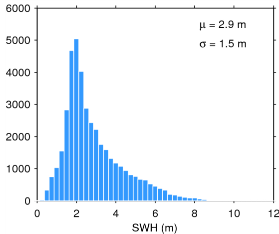
Figure 20. Histogram of science-valid SWH over oceans and lakes for 10/06/2015. The mean ( \mu ) and standard deviation ( \sigma ) are also shown. Note that values larger than 12 m are excluded from the histogram for the sake of readability but not from the computation of \mu and \sigma .
