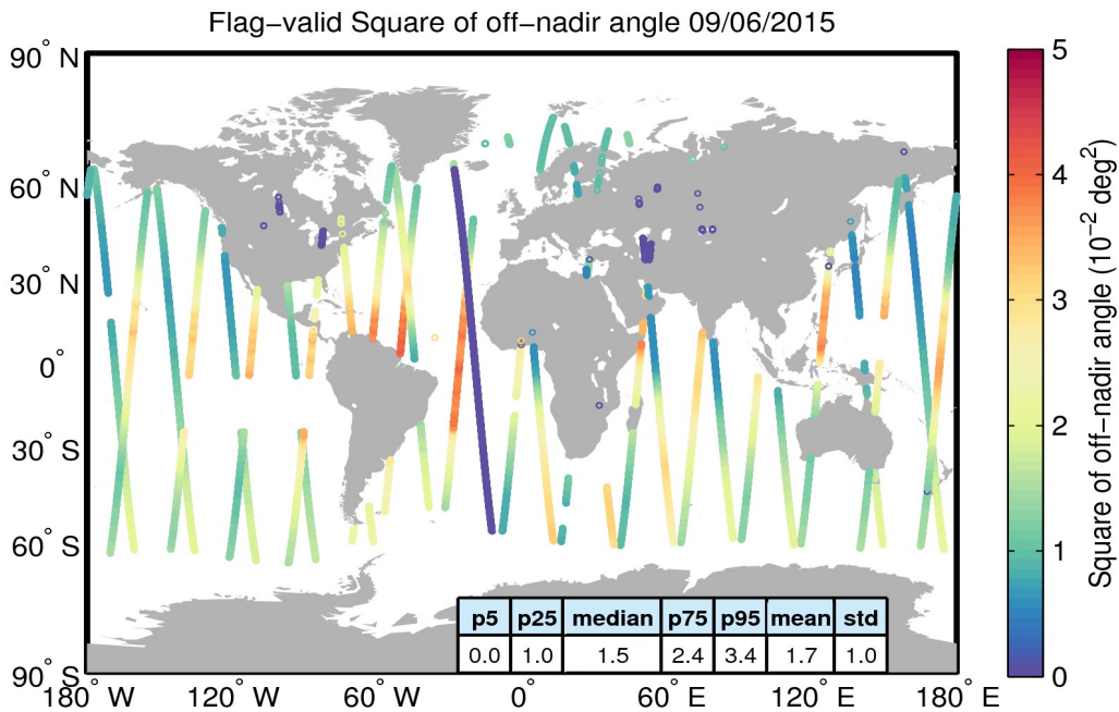
Figure 37. Geographical distribution of flag-valid mispointing data over oceans and lakes for 09/06/2015. The statistical values shown in the table refer to the mispointing in 10^{-2} \text{ deg}^2 and are calculated over all measurements shown in the figure.
