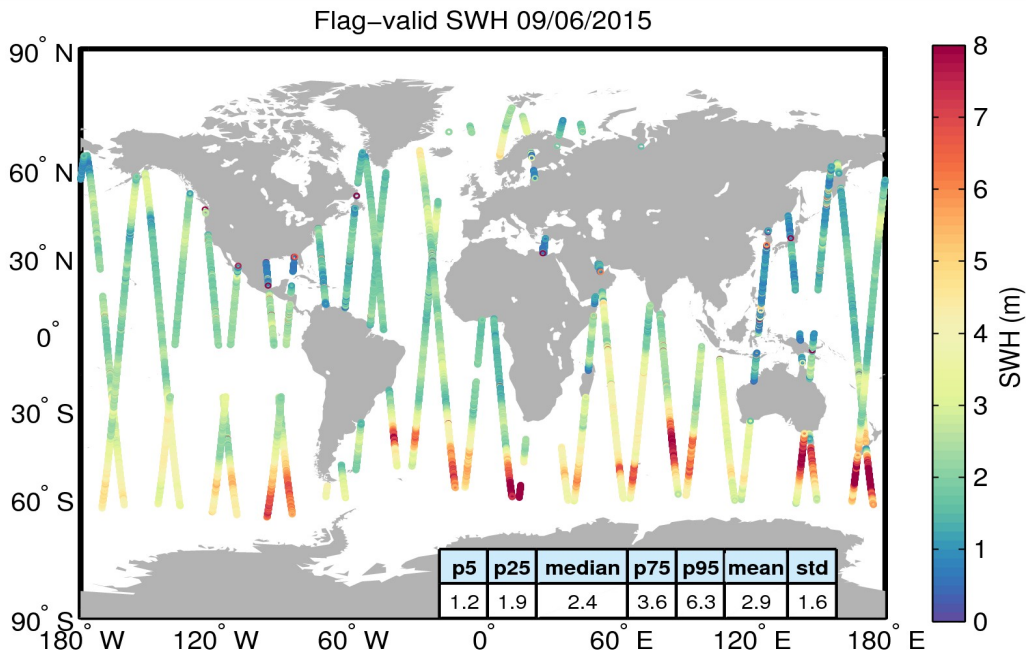
Figure 15. Geographical distribution of flag-valid SWH data over oceans and lakes for 09/06/2015. The statistical values shown in the table refer to the SWH in m and are calculated over all measurements shown in the figure.
