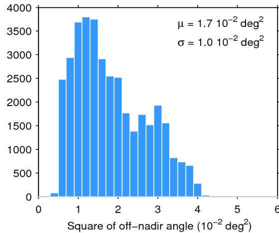
Figure 39. Histogram of flag-valid mispointing over oceans and lakes for 09/06/2015. The mean ( \mu ) and standard deviation ( \sigma ) are also shown. Note that values larger than 6 \cdot 10^{-2} \text{ deg}^2 are excluded from the histogram for the sake of readability but not from the computation of \mu and \sigma .
