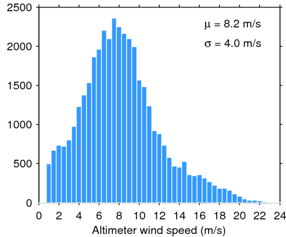
Figure 33. Histogram of flag-valid wind over oceans and lakes for 09/06/2015. The mean ( \mu ) and standard deviation ( \sigma ) are also shown. Note that values larger than 24 m/s are excluded from the histogram for the sake of readability but not from the computation of \mu and \sigma .
