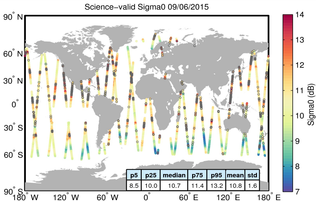
Figure 27. Geographical distribution of science-valid sigma0 data over oceans and lakes for 09/06/2015. The statistical values shown in the table refer to the sigma0 in dB and are calculated over all measurements shown in the figure. Gray circles denote records that have been rejected based on the editing criteria described in Table 4.
