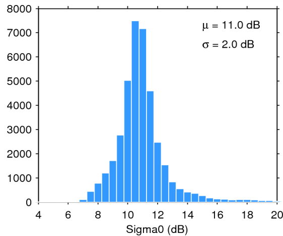
Figure 25. Histogram of flag-valid sigma0 over oceans and lakes for 09/06/2015. The mean ( \mu ) and standard deviation ( \sigma ) are also shown. Note that values outside [4 20] dB are excluded from the histogram for the sake of readability but not from the computation of \mu and \sigma .
