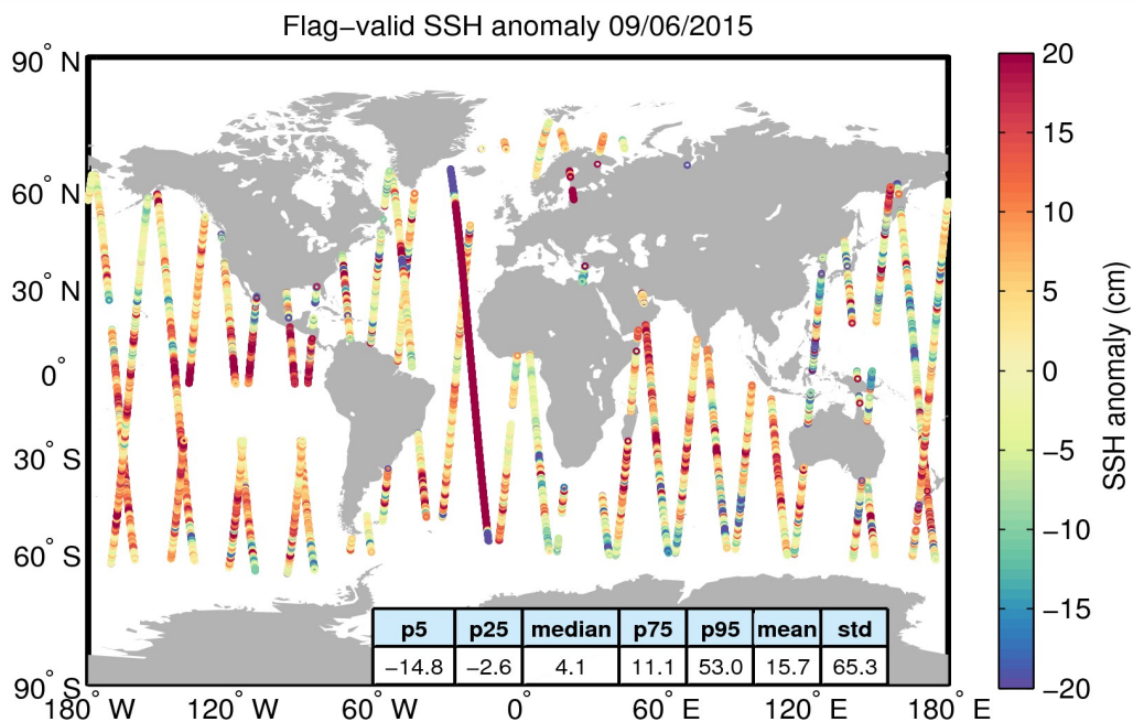
Figure 5. Geographical distribution of flag-valid 1-Hz SSH anomaly data over oceans and lakes for 09/06/2015. The statistical values shown in the table refer to the SSH anomaly in cm and are calculated over all measurements shown in the figure.
