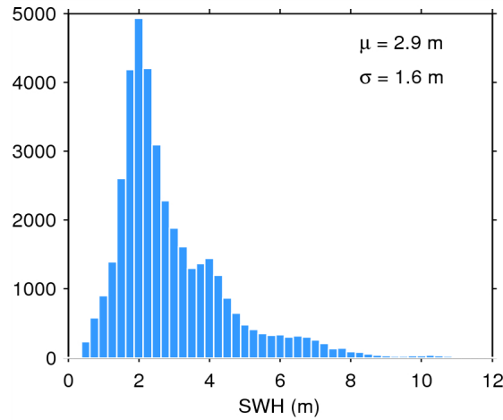
Figure 17. Histogram of flag-valid SWH over oceans and lakes for 09/06/2015. The mean ( \mu ) and standard deviation ( \sigma ) are also shown. Note that values larger than 12 m are excluded from the histogram for the sake of readability but not from the computation of \mu and \sigma .
