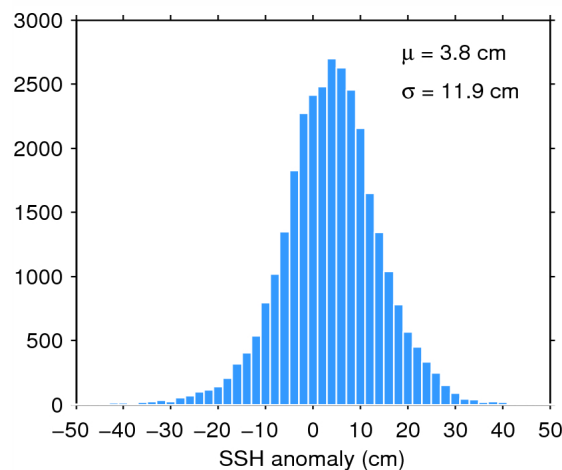
Figure 11. Histogram of science-valid SSH anomaly over oceans and lakes for 09/06/2015. The mean ( \mu ) and standard deviation ( \sigma ) are also shown. Note that values outside [-50 50] cm are excluded from the histogram for the sake of readability but not from the computation of \mu and \sigma .
