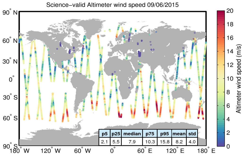
Figure 34. Geographical distribution of science-valid wind data over oceans and lakes for 09/06/2015. The statistical values shown in the table refer to the wind in m/s and are calculated over all measurements shown in the figure. Gray circles denote records that have been rejected based on the editing criteria described in Table 5.
