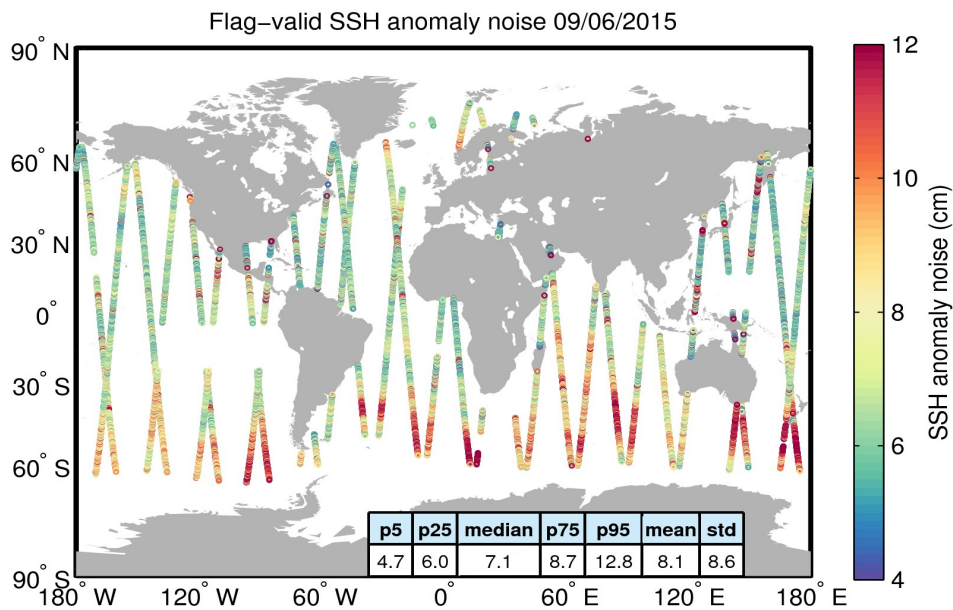
Figure 8. Geographical distribution of flag-valid 20-Hz SSH anomaly measurement noise over oceans and lakes for 09/06/2015. The statistical values shown in the table refer to the SSH anomaly noise and are calculated over all measurements shown in the figure.
