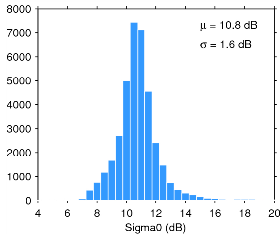
Figure 28. Histogram of science-valid sigma0 over oceans and lakes for 09/06/2015. The mean ( \mu ) and standard deviation ( \sigma ) are also shown. Note that values outside [4 20] dB are excluded from the histogram for the sake of readability but not from the computation of \mu and \sigma .
