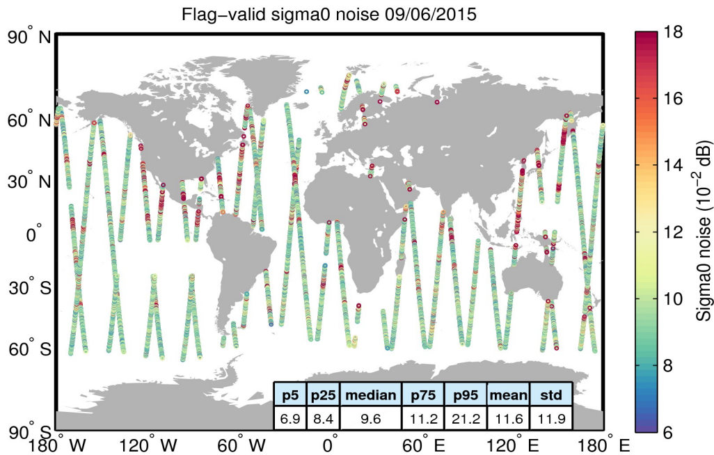
Figure 26. Geographical distribution of flag-valid 20-Hz sigma0 measurement noise over oceans and lakes for 09/06/2015. The statistical values shown in the table refer to the sigma0 noise and are calculated over all measurements shown in the figure.
