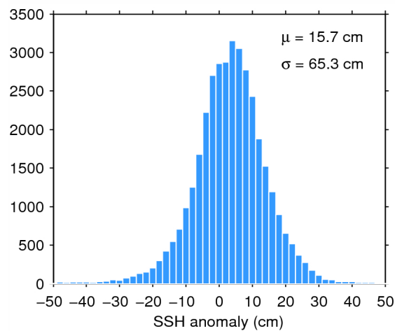
Figure 7. Histogram of flag-valid SSH anomaly over oceans and lakes for 09/06/2015. The mean ( \mu ) and standard deviation ( \sigma ) are also shown. Note that values outside [-50 50] cm are excluded from the histogram for the sake of readability but not from the computation of \mu and \sigma .
