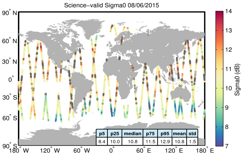
Figure 27. Geographical distribution of science-valid sigma0 data over oceans and lakes for 08/06/2015. The statistical values shown in the table refer to the sigma0 in dB and are calculated over all measurements shown in the figure. Gray circles denote records that have been rejected based on the editing criteria described in Table 4.
