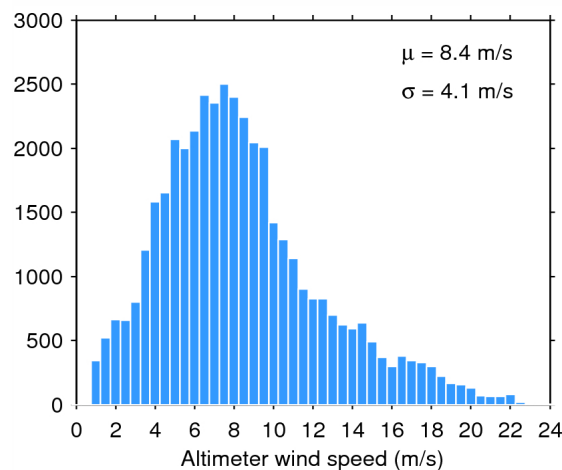
Figure 35. Histogram of science-valid wind over oceans and lakes for 08/06/2015. The mean ( \mu ) and standard deviation ( \sigma ) are also shown. Note that values larger than 24 m/s are excluded from the histogram for the sake of readability but not from the computation of \mu and \sigma .
