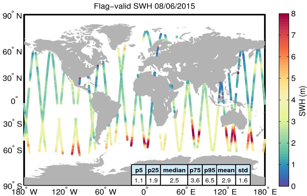
Figure 15. Geographical distribution of flag-valid SWH data over oceans and lakes for 08/06/2015. The statistical values shown in the table refer to the SWH in m and are calculated over all measurements shown in the figure.
