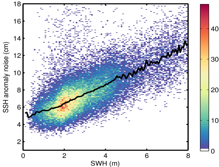
Figure 9. 2D histogram showing flag-valid SSH anomaly noise as a function of SWH for 08/06/2015. The black line denotes the median SSH anomaly as a function of SWH.
