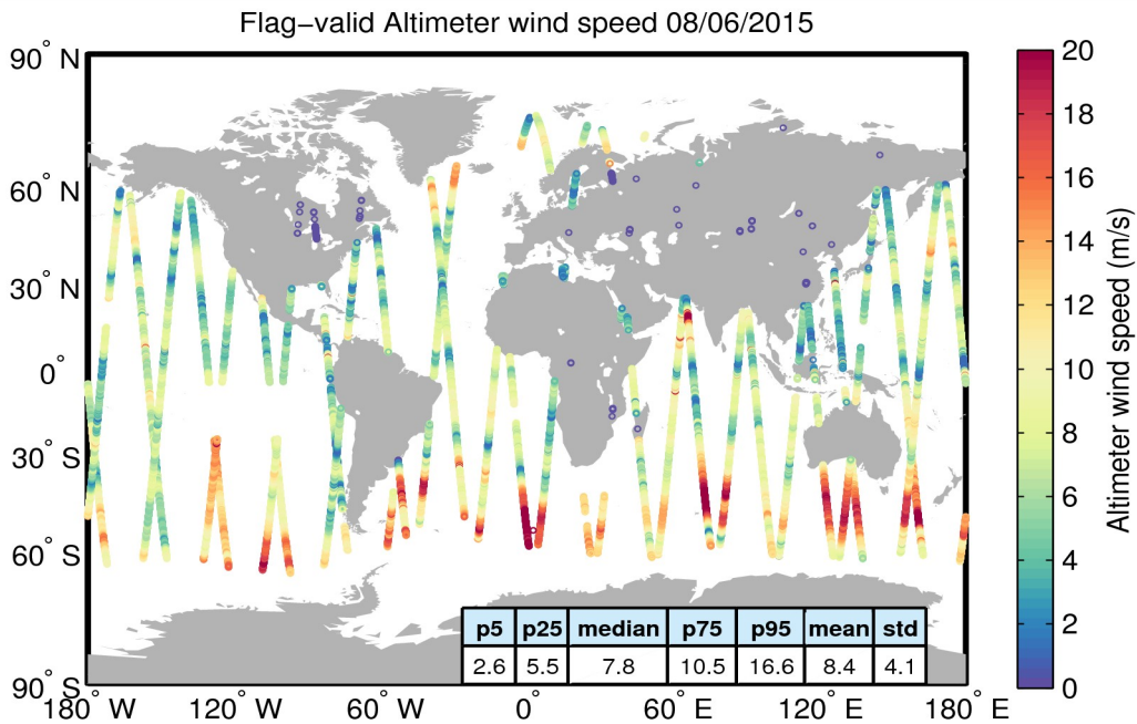
Figure 31. Geographical distribution of flag-valid wind data over oceans and lakes for 08/06/2015. The statistical values shown in the table refer to the wind in m/s and are calculated over all measurements shown in the figure.
