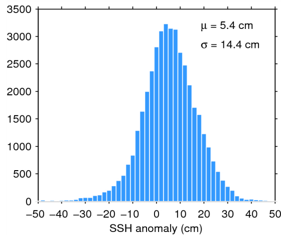
Figure 7. Histogram of flag-valid SSH anomaly over oceans and lakes for 08/06/2015. The mean ( \mu ) and standard deviation ( \sigma ) are also shown. Note that values outside [-50\ 50] cm are excluded from the histogram for the sake of readability but not from the computation of \mu and \sigma .
