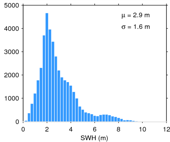
Figure 17. Histogram of flag-valid SWH over oceans and lakes for 08/06/2015. The mean ( \mu ) and standard deviation ( \sigma ) are also shown. Note that values larger than 12 m are excluded from the histogram for the sake of readability but not from the computation of \mu and \sigma .
