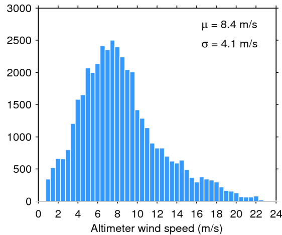
Figure 33. Histogram of flag-valid wind over oceans and lakes for 08/06/2015. The mean ( \mu ) and standard deviation ( \sigma ) are also shown. Note that values larger than 24 m/s are excluded from the histogram for the sake of readability but not from the computation of \mu and \sigma .
