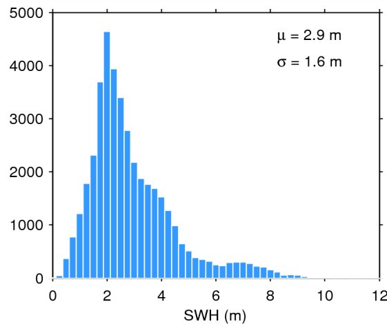
Figure 20. Histogram of science-valid SWH over oceans and lakes for 08/06/2015. The mean ( \mu ) and standard deviation ( \sigma ) are also shown. Note that values larger than 12 m are excluded from the histogram for the sake of readability but not from the computation of \mu and \sigma .
