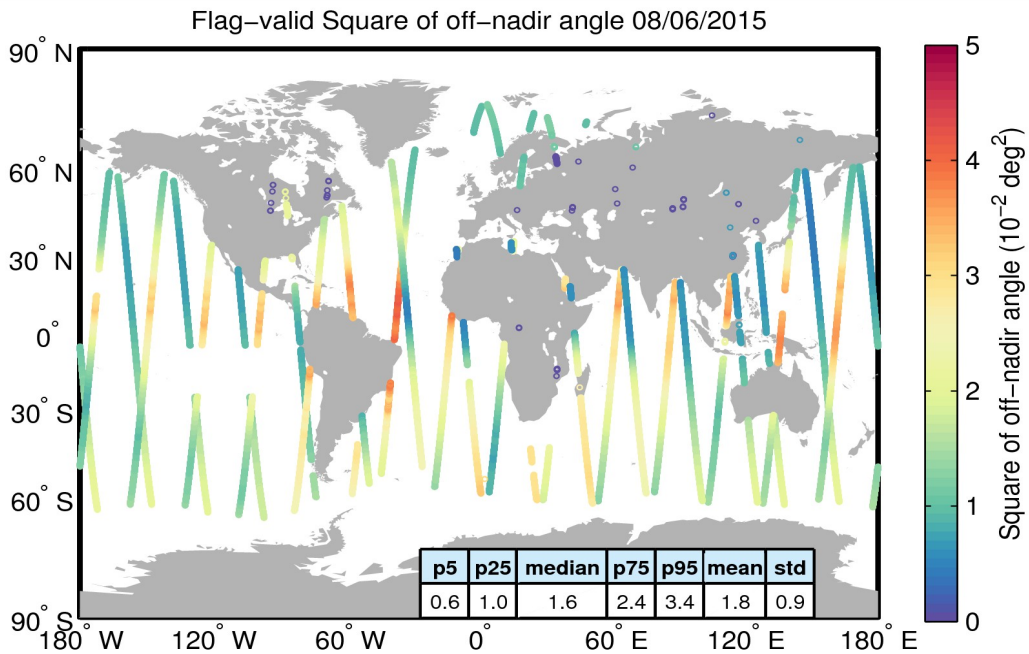
Figure 37. Geographical distribution of flag-valid mispointing data over oceans and lakes for 08/06/2015. The statistical values shown in the table refer to the mispointing in 10^{-2} \text{deg}^2 and are calculated over all measurements shown in the figure.
