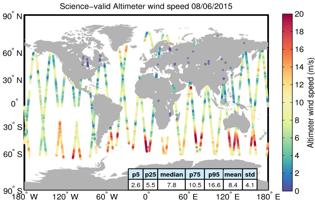
Figure 34. Geographical distribution of science-valid wind data over oceans and lakes for 08/06/2015. The statistical values shown in the table refer to the wind in m/s and are calculated over all measurements shown in the figure. Gray circles denote records that have been rejected based on the editing criteria described in Table 5.
