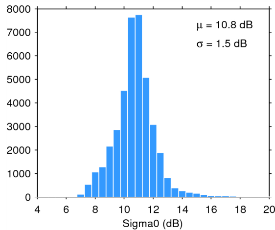
Figure 28. Histogram of science-valid sigma0 over oceans and lakes for 08/06/2015. The mean ( \mu ) and standard deviation ( \sigma ) are also shown. Note that values outside [4 20] dB are excluded from the histogram for the sake of readability but not from the computation of \mu and \sigma .
