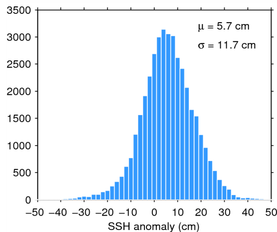
Figure 11. Histogram of science-valid SSH anomaly over oceans and lakes for 08/06/2015. The mean ( \mu ) and standard deviation ( \sigma ) are also shown. Note that values outside [-50 50] cm are excluded from the histogram for the sake of readability but not from the computation of \mu and \sigma .
