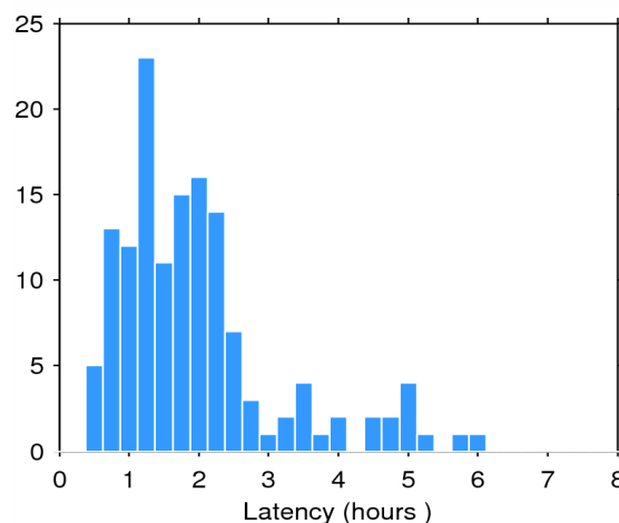
Figure 2. Histogram of the data latency for 08/06/2015. The y-axis denotes the number of files that are made available with a delay of x-hours with respect to the mean time of the records stored in the file.
