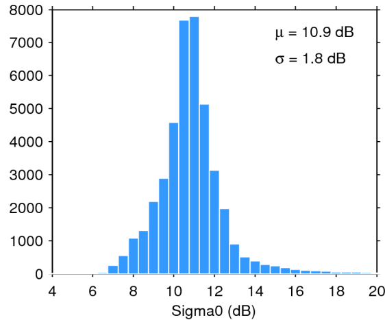
Figure 25. Histogram of flag-valid sigma0 over oceans and lakes for 08/06/2015. The mean ( \mu ) and standard deviation ( \sigma ) are also shown. Note that values outside [4 20] dB are excluded from the histogram for the sake of readability but not from the computation of \mu and \sigma .
