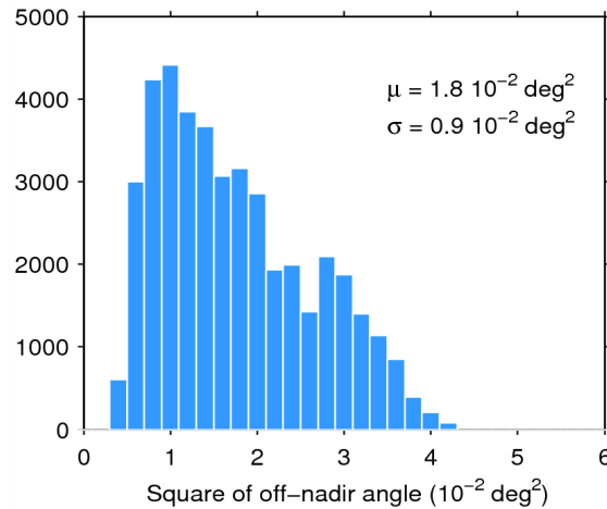
Figure 39. Histogram of flag-valid mispointing over oceans and lakes for 08/06/2015. The mean ( \mu ) and standard deviation ( \sigma ) are also shown. Note that values larger than 6 \cdot 10^{-2} \text{ deg}^2 are excluded from the histogram for the sake of readability but not from the computation of \mu and \sigma .
