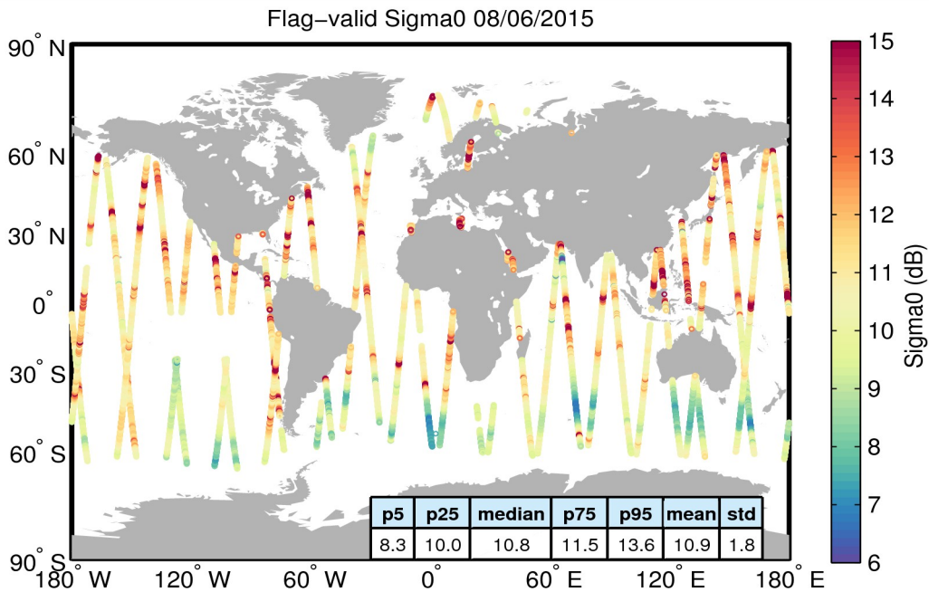
Figure 23. Geographical distribution of flag-valid sigma0 data over oceans and lakes for 08/06/2015. The statistical values shown in the table refer to the sigma0 in dB and are calculated over all measurements shown in the figure.
