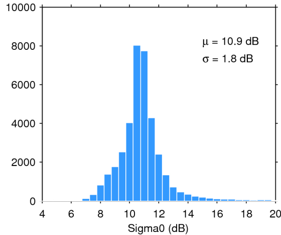
Figure 25. Histogram of flag-valid sigma0 over oceans and lakes for 07/06/2015. The mean ( \mu ) and standard deviation ( \sigma ) are also shown. Note that values outside [4 20] dB are excluded from the histogram for the sake of readability but not from the computation of \mu and \sigma .
