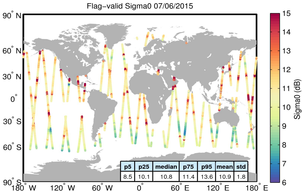
Figure 23. Geographical distribution of flag-valid sigma0 data over oceans and lakes for 07/06/2015. The statistical values shown in the table refer to the sigma0 in dB and are calculated over all measurements shown in the figure.
