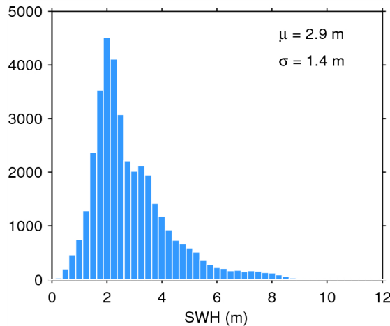
Figure 20. Histogram of science-valid SWH over oceans and lakes for 07/06/2015. The mean ( \mu ) and standard deviation ( \sigma ) are also shown. Note that values larger than 12 m are excluded from the histogram for the sake of readability but not from the computation of \mu and \sigma .
