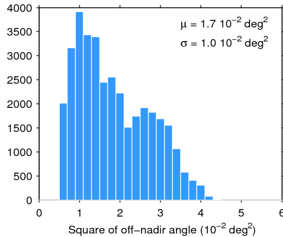
Figure 39. Histogram of flag-valid mispointing over oceans and lakes for 07/06/2015. The mean ( \mu ) and standard deviation ( \sigma ) are also shown. Note that values larger than 6 \cdot 10^{-2} \text{ deg}^2 are excluded from the histogram for the sake of readability but not from the computation of \mu and \sigma .
