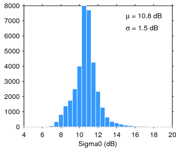
Figure 28. Histogram of science-valid sigma0 over oceans and lakes for 07/06/2015. The mean ( \mu ) and standard deviation ( \sigma ) are also shown. Note that values outside [4 20] dB are excluded from the histogram for the sake of readability but not from the computation of \mu and \sigma .
