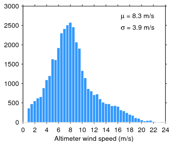
Figure 35. Histogram of science-valid wind over oceans and lakes for 07/06/2015. The mean ( \mu ) and standard deviation ( \sigma ) are also shown. Note that values larger than 24 m/s are excluded from the histogram for the sake of readability but not from the computation of \mu and \sigma .
