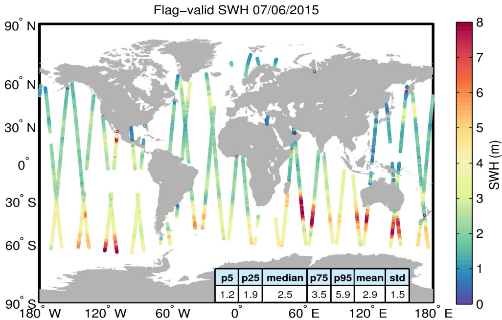
Figure 15. Geographical distribution of flag-valid SWH data over oceans and lakes for 07/06/2015. The statistical values shown in the table refer to the SWH in m and are calculated over all measurements shown in the figure.
