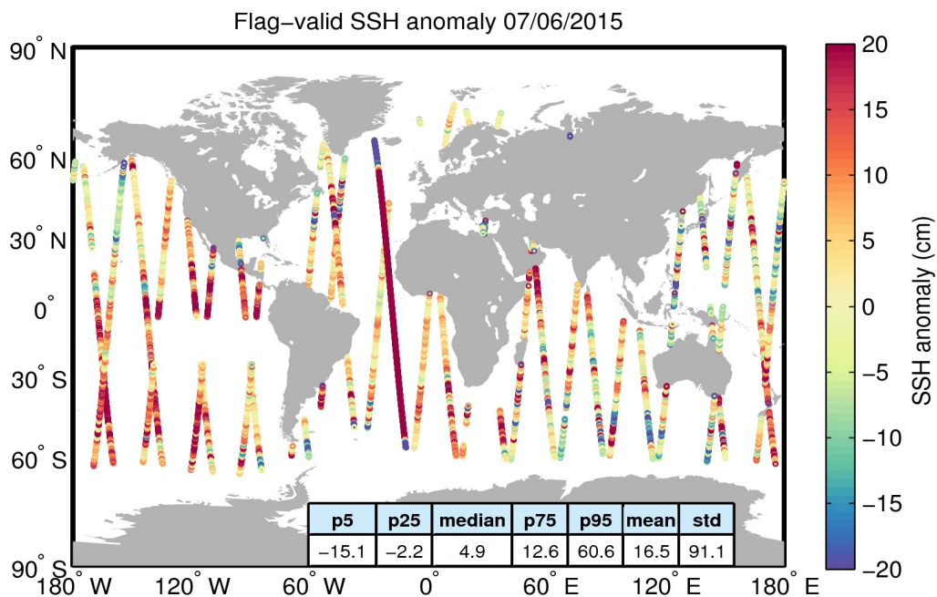
Figure 5. Geographical distribution of flag-valid 1-Hz SSH anomaly data over oceans and lakes for 07/06/2015. The statistical values shown in the table refer to the SSH anomaly in cm and are calculated over all measurements shown in the figure.
