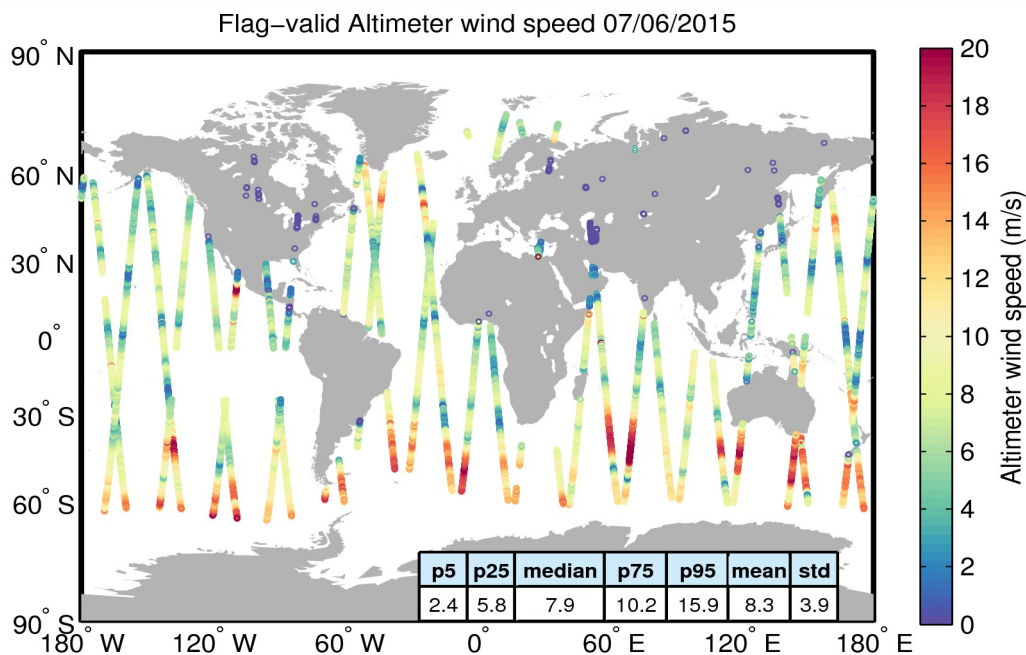
Figure 31. Geographical distribution of flag-valid wind data over oceans and lakes for 07/06/2015. The statistical values shown in the table refer to the wind in m/s and are calculated over all measurements shown in the figure.
