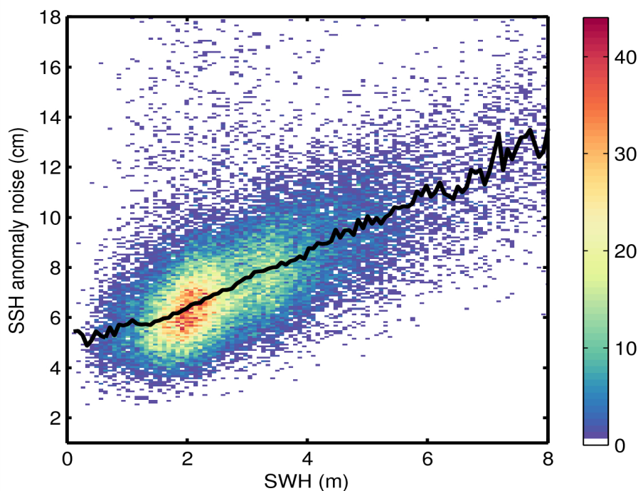
Figure 9. 2D histogram showing flag-valid SSH anomaly noise as a function of SWH for 07/06/2015. The black line denotes the median SSH anomaly as a function of SWH.
