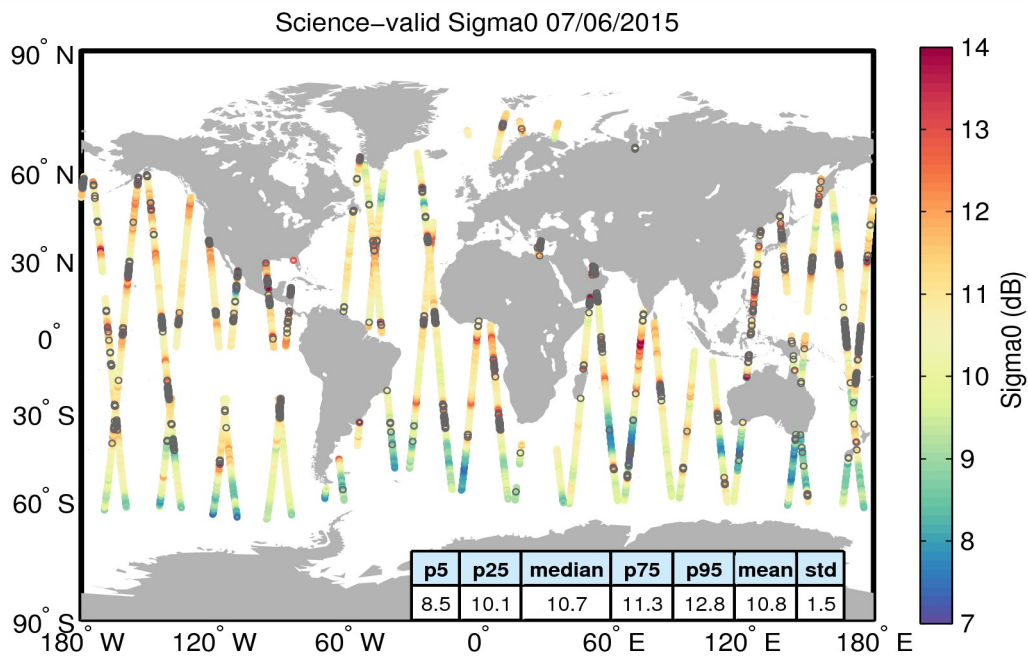
Figure 27. Geographical distribution of science-valid sigma0 data over oceans and lakes for 07/06/2015. The statistical values shown in the table refer to the sigma0 in dB and are calculated over all measurements shown in the figure. Gray circles denote records that have been rejected based on the editing criteria described in Table 4.
