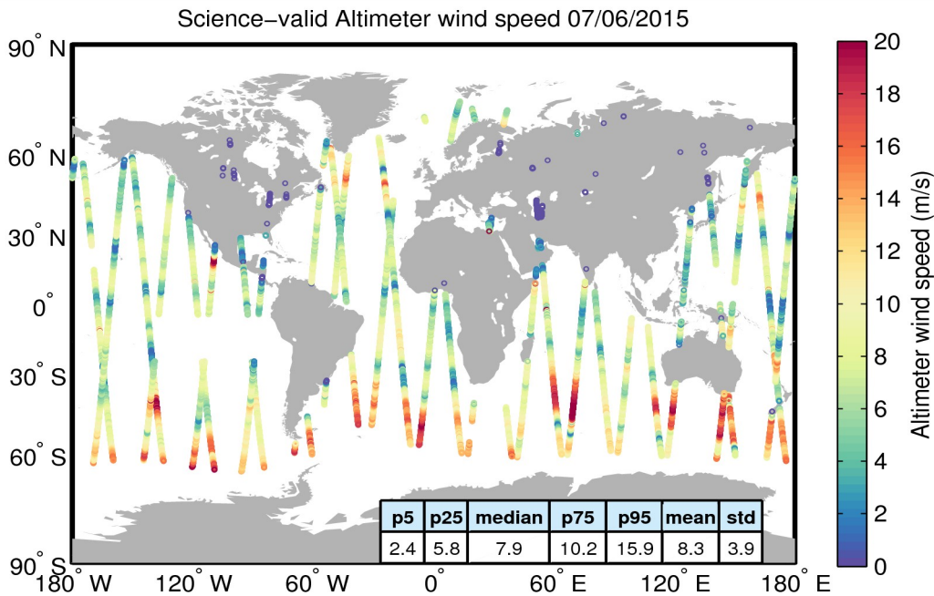
Figure 34. Geographical distribution of science-valid wind data over oceans and lakes for 07/06/2015. The statistical values shown in the table refer to the wind in m/s and are calculated over all measurements shown in the figure. Gray circles denote records that have been rejected based on the editing criteria described in Table 5.
