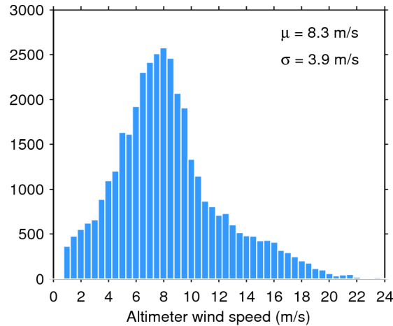
Figure 33. Histogram of flag-valid wind over oceans and lakes for 07/06/2015. The mean ( \mu ) and standard deviation ( \sigma ) are also shown. Note that values larger than 24 m/s are excluded from the histogram for the sake of readability but not from the computation of \mu and \sigma .
