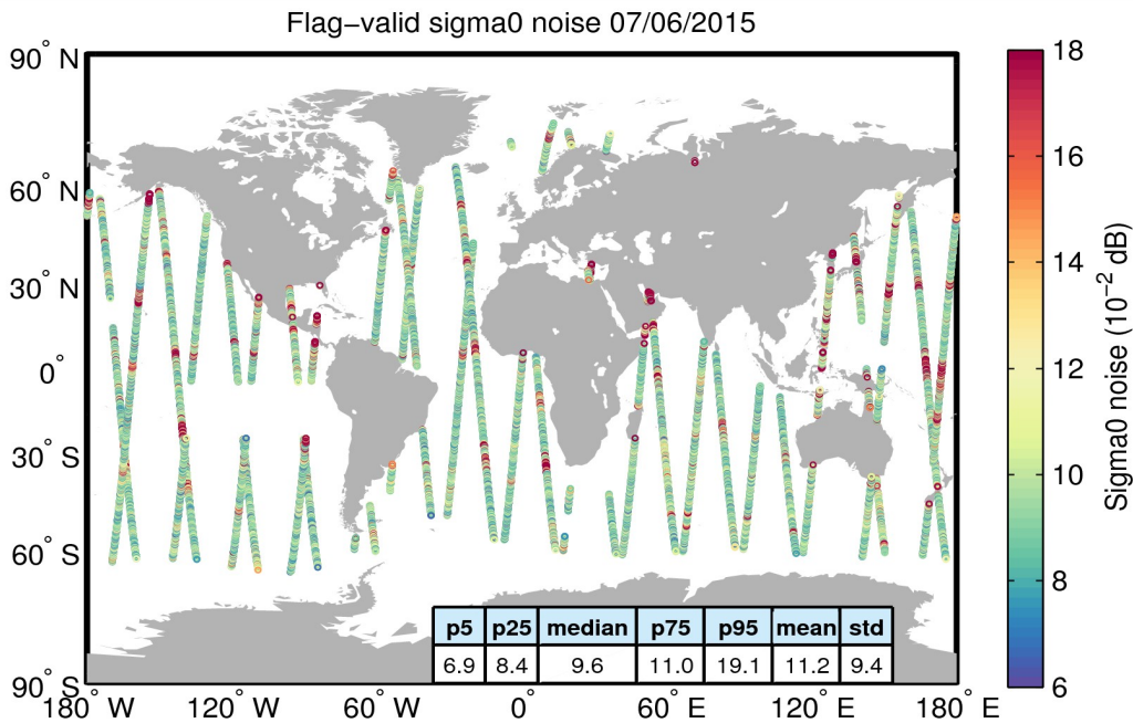
Figure 26. Geographical distribution of flag-valid 20-Hz sigma0 measurement noise over oceans and lakes for 07/06/2015. The statistical values shown in the table refer to the sigma0 noise and are calculated over all measurements shown in the figure.
