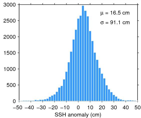
Figure 7. Histogram of flag-valid SSH anomaly over oceans and lakes for 07/06/2015. The mean ( \mu ) and standard deviation ( \sigma ) are also shown. Note that values outside [-50 50] cm are excluded from the histogram for the sake of readability but not from the computation of \mu and \sigma .
