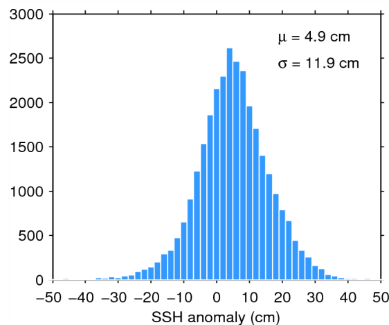
Figure 11. Histogram of science-valid SSH anomaly over oceans and lakes for 07/06/2015. The mean ( \mu ) and standard deviation ( \sigma ) are also shown. Note that values outside [-50 50] cm are excluded from the histogram for the sake of readability but not from the computation of \mu and \sigma .
