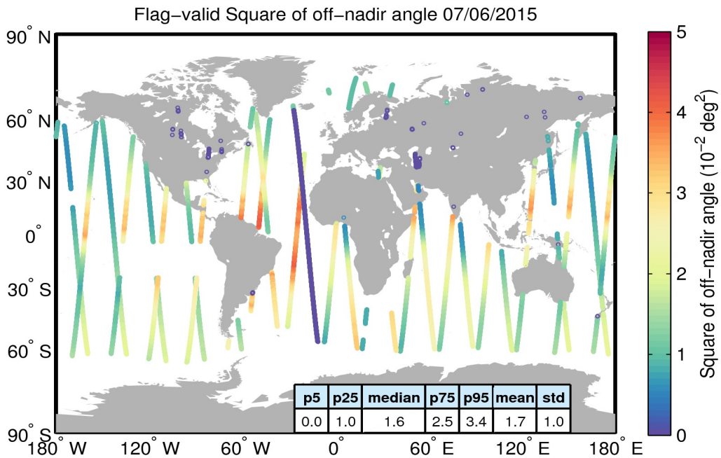
Figure 37. Geographical distribution of flag-valid mispointing data over oceans and lakes for 07/06/2015. The statistical values shown in the table refer to the mispointing in 10^{-2} \text{deg}^2 and are calculated over all measurements shown in the figure.
