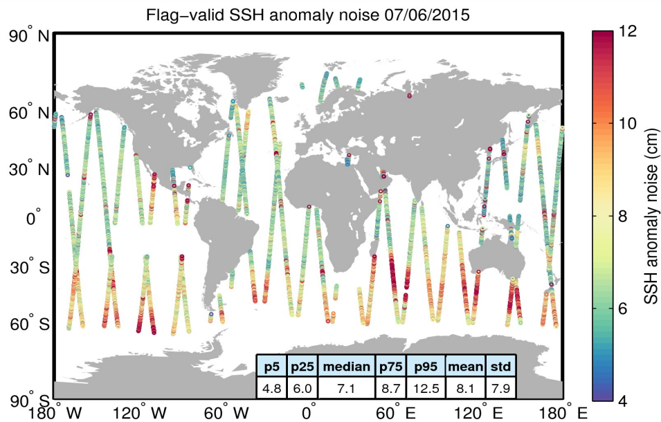
Figure 8. Geographical distribution of flag-valid 20-Hz SSH anomaly measurement noise over oceans and lakes for 07/06/2015. The statistical values shown in the table refer to the SSH anomaly noise and are calculated over all measurements shown in the figure.
