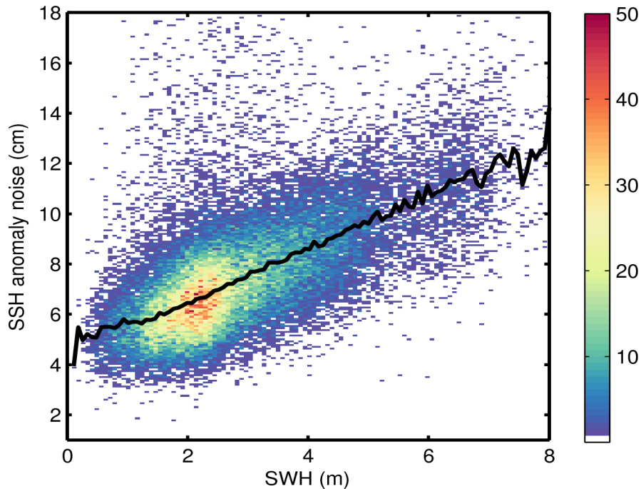
Figure 9. 2D histogram showing flag-valid SSH anomaly noise as a function of SWH for 06/06/2015. The black line denotes the median SSH anomaly as a function of SWH.
