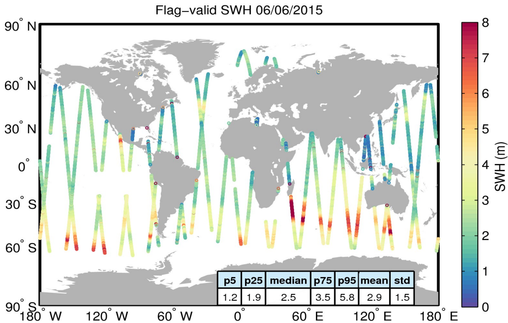
Figure 15. Geographical distribution of flag-valid SWH data over oceans and lakes for 06/06/2015. The statistical values shown in the table refer to the SWH in m and are calculated over all measurements shown in the figure.
