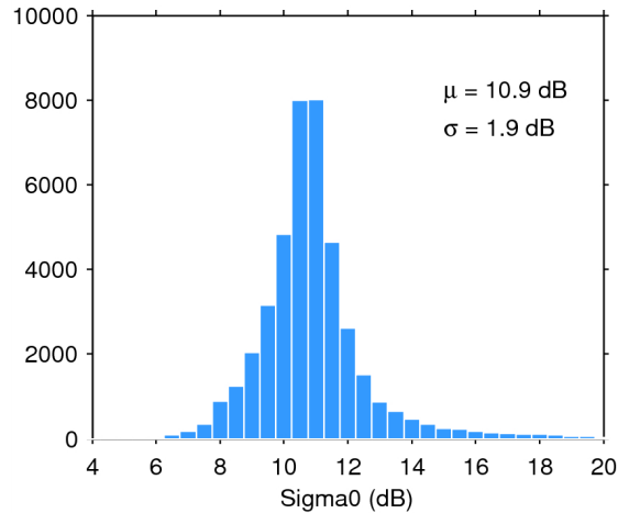
Figure 25. Histogram of flag-valid sigma0 over oceans and lakes for 06/06/2015. The mean ( \mu ) and standard deviation ( \sigma ) are also shown. Note that values outside [4 20] dB are excluded from the histogram for the sake of readability but not from the computation of \mu and \sigma .
