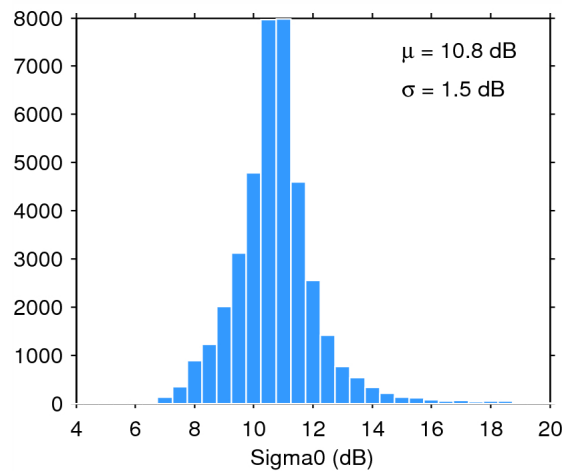
Figure 28. Histogram of science-valid sigma0 over oceans and lakes for 06/06/2015. The mean ( \mu ) and standard deviation ( \sigma ) are also shown. Note that values outside [4 20] dB are excluded from the histogram for the sake of readability but not from the computation of \mu and \sigma .
