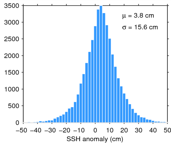
Figure 7. Histogram of flag-valid SSH anomaly over oceans and lakes for 06/06/2015. The mean ( \mu ) and standard deviation ( \sigma ) are also shown. Note that values outside [-50\ 50] cm are excluded from the histogram for the sake of readability but not from the computation of \mu and \sigma .
