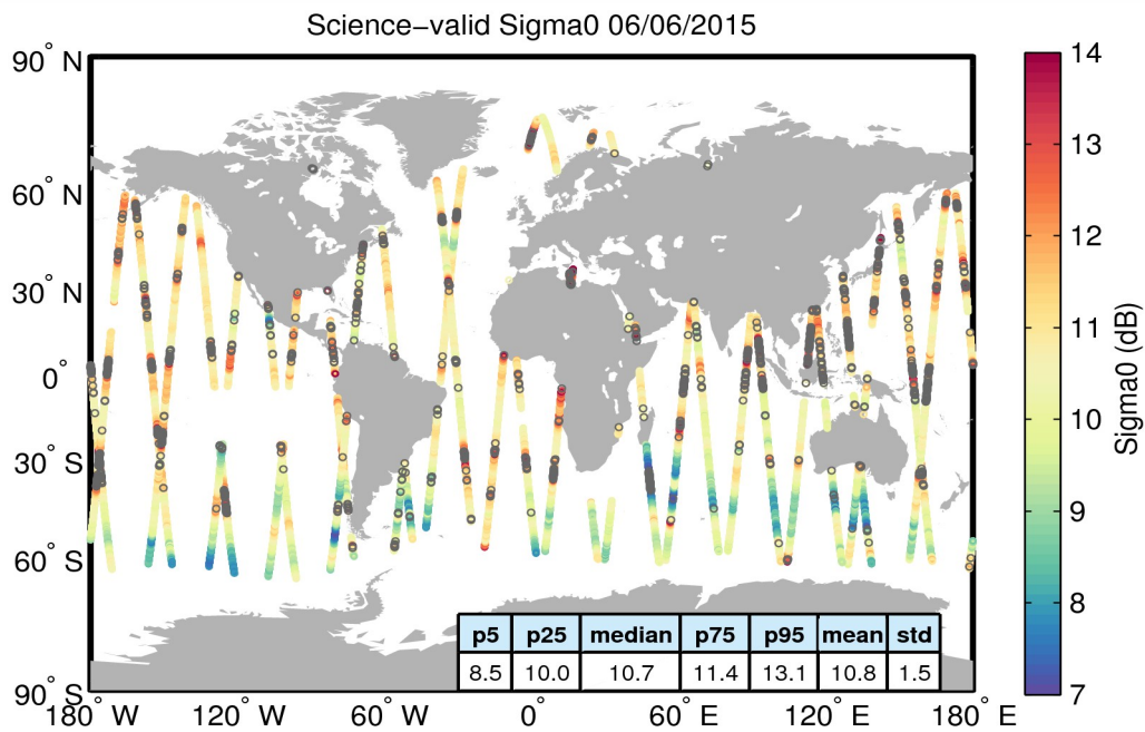
Figure 27. Geographical distribution of science-valid sigma0 data over oceans and lakes for 06/06/2015. The statistical values shown in the table refer to the sigma0 in dB and are calculated over all measurements shown in the figure. Gray circles denote records that have been rejected based on the editing criteria described in Table 4.
