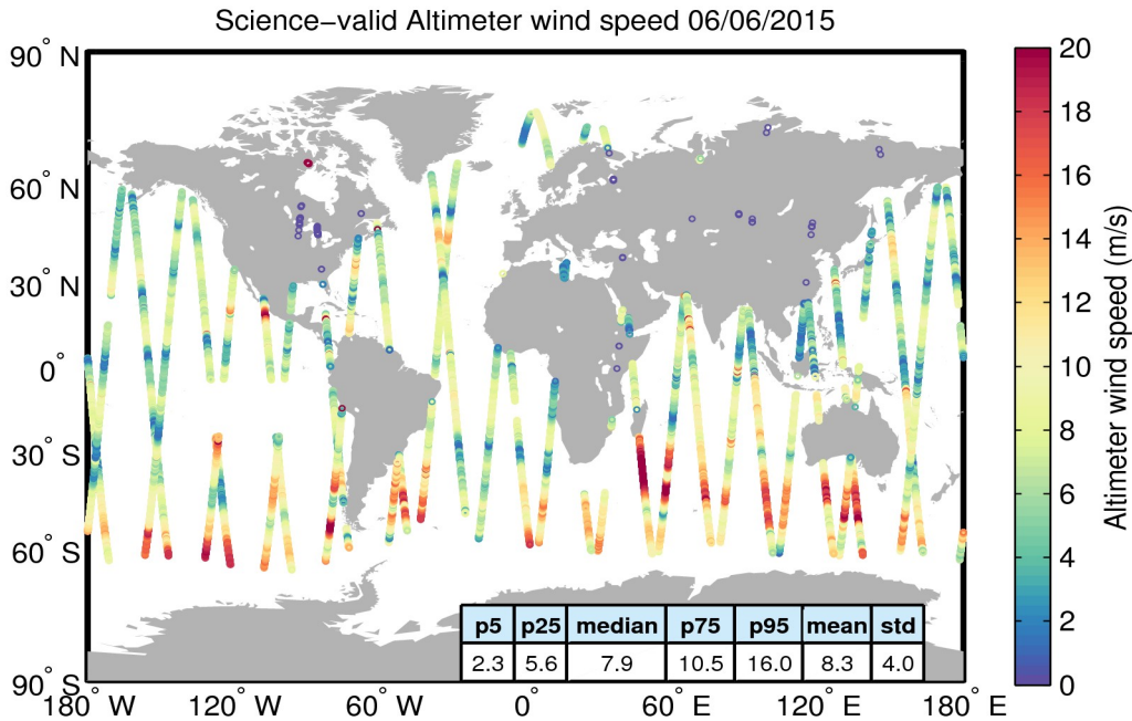
Figure 34. Geographical distribution of science-valid wind data over oceans and lakes for 06/06/2015. The statistical values shown in the table refer to the wind in m/s and are calculated over all measurements shown in the figure. Gray circles denote records that have been rejected based on the editing criteria described in Table 5.
