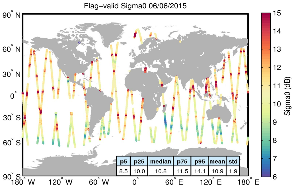
Figure 23. Geographical distribution of flag-valid sigma0 data over oceans and lakes for 06/06/2015. The statistical values shown in the table refer to the sigma0 in dB and are calculated over all measurements shown in the figure.
