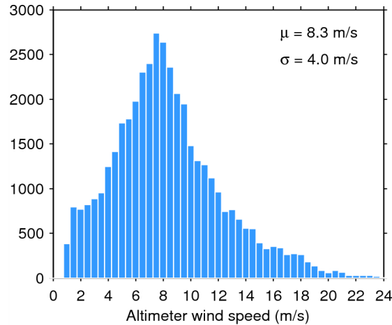
Figure 33. Histogram of flag-valid wind over oceans and lakes for 06/06/2015. The mean ( \mu ) and standard deviation ( \sigma ) are also shown. Note that values larger than 24 m/s are excluded from the histogram for the sake of readability but not from the computation of \mu and \sigma .
