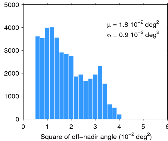
Figure 39. Histogram of flag-valid mispointing over oceans and lakes for 06/06/2015. The mean ( \mu ) and standard deviation ( \sigma ) are also shown. Note that values larger than 6 \cdot 10^{-2} \text{ deg}^2 are excluded from the histogram for the sake of readability but not from the computation of \mu and \sigma .
