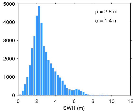
Figure 20. Histogram of science-valid SWH over oceans and lakes for 06/06/2015. The mean ( \mu ) and standard deviation ( \sigma ) are also shown. Note that values larger than 12 m are excluded from the histogram for the sake of readability but not from the computation of \mu and \sigma .
