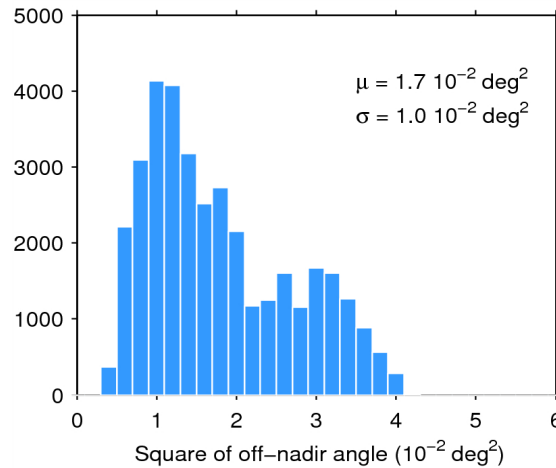
Figure 39. Histogram of flag-valid mispointing over oceans and lakes for 05/06/2015. The mean ( \mu ) and standard deviation ( \sigma ) are also shown. Note that values larger than 6 \cdot 10^{-2} \text{ deg}^2 are excluded from the histogram for the sake of readability but not from the computation of \mu and \sigma .
