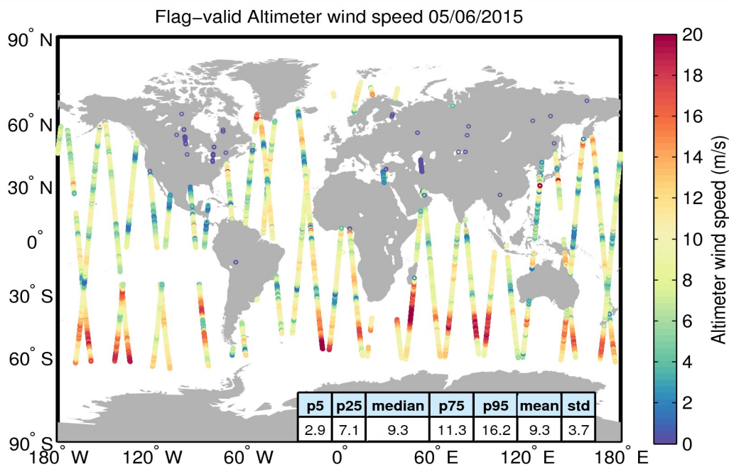
Figure 31. Geographical distribution of flag-valid wind data over oceans and lakes for 05/06/2015. The statistical values shown in the table refer to the wind in m/s and are calculated over all measurements shown in the figure.
