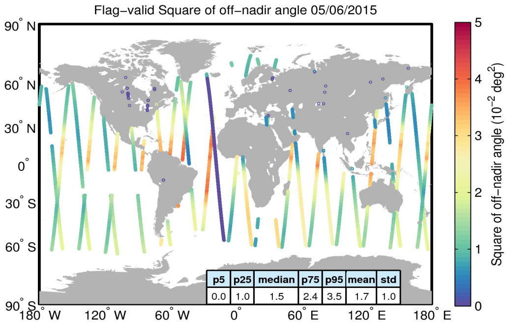
Figure 37. Geographical distribution of flag-valid mispointing data over oceans and lakes for 05/06/2015. The statistical values shown in the table refer to the mispointing in 10^{-2} \text{ deg}^2 and are calculated over all measurements shown in the figure.
