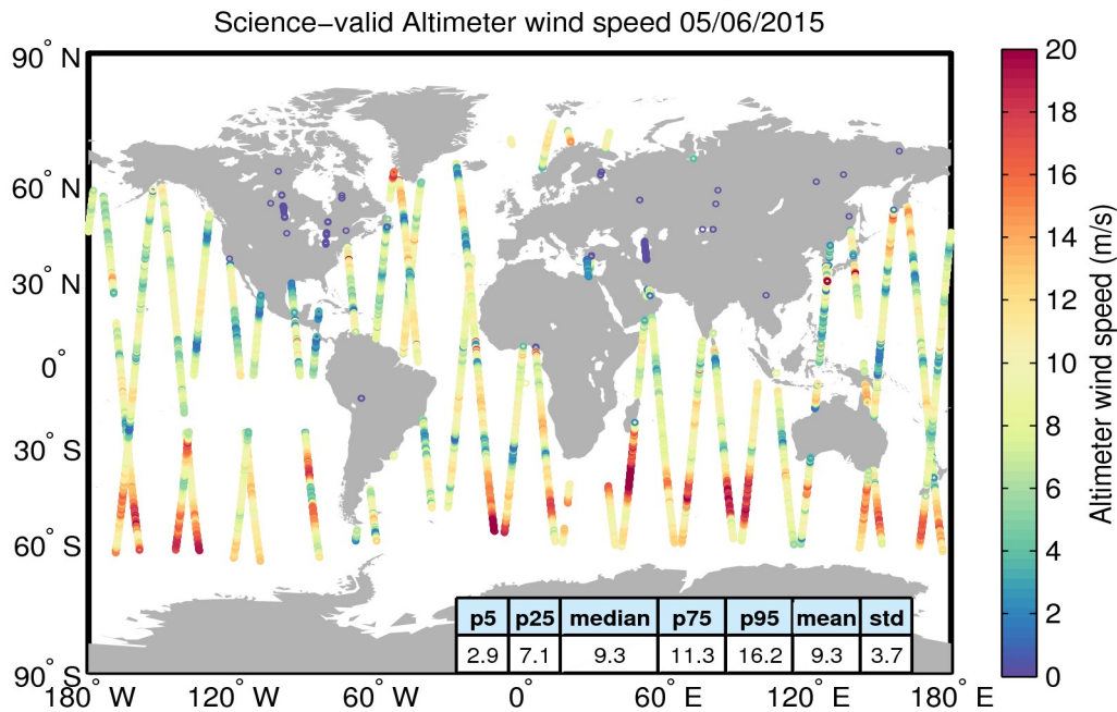
Figure 34. Geographical distribution of science-valid wind data over oceans and lakes for 05/06/2015. The statistical values shown in the table refer to the wind in m/s and are calculated over all measurements shown in the figure. Gray circles denote records that have been rejected based on the editing criteria described in Table 5.
