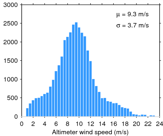
Figure 33. Histogram of flag-valid wind over oceans and lakes for 05/06/2015. The mean ( \mu ) and standard deviation ( \sigma ) are also shown. Note that values larger than 24 m/s are excluded from the histogram for the sake of readability but not from the computation of \mu and \sigma .
