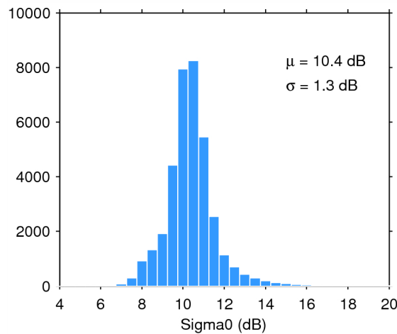
Figure 28. Histogram of science-valid sigma0 over oceans and lakes for 05/06/2015. The mean ( \mu ) and standard deviation ( \sigma ) are also shown. Note that values outside [4 20] dB are excluded from the histogram for the sake of readability but not from the computation of \mu and \sigma .
