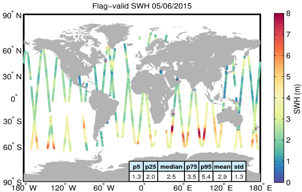
Figure 15. Geographical distribution of flag-valid SWH data over oceans and lakes for 05/06/2015. The statistical values shown in the table refer to the SWH in m and are calculated over all measurements shown in the figure.
