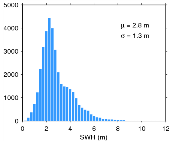
Figure 20. Histogram of science-valid SWH over oceans and lakes for 05/06/2015. The mean ( \mu ) and standard deviation ( \sigma ) are also shown. Note that values larger than 12 m are excluded from the histogram for the sake of readability but not from the computation of \mu and \sigma .
