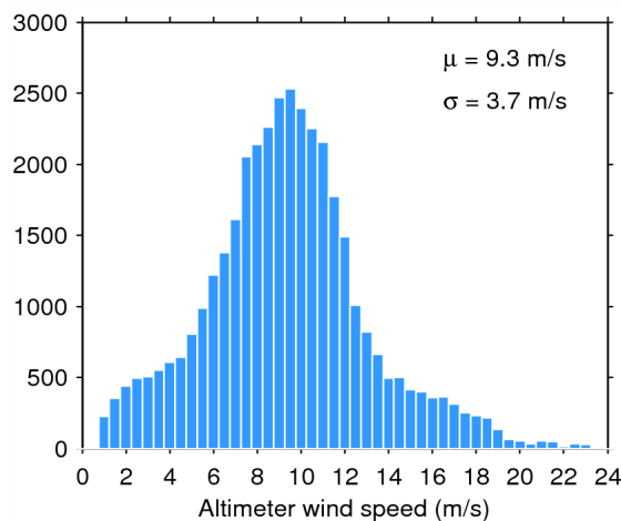
Figure 35. Histogram of science-valid wind over oceans and lakes for 05/06/2015. The mean ( \mu ) and standard deviation ( \sigma ) are also shown. Note that values larger than 24 m/s are excluded from the histogram for the sake of readability but not from the computation of \mu and \sigma .
