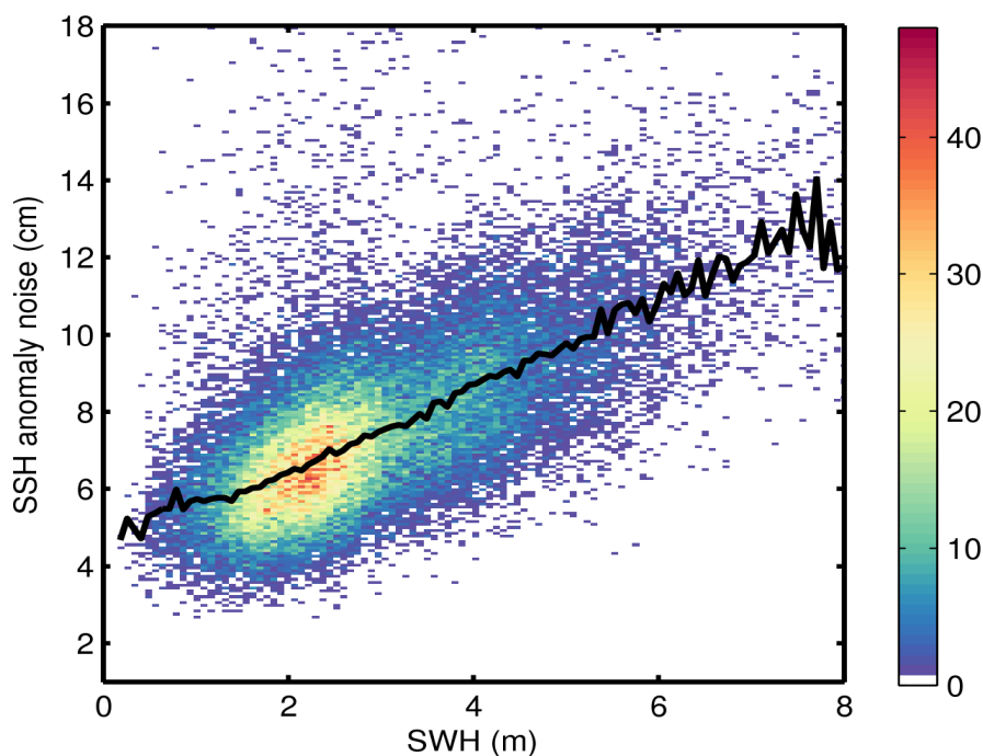
Figure 9. 2D histogram showing flag-valid SSH anomaly noise as a function of SWH for 05/06/2015. The black line denotes the median SSH anomaly as a function of SWH.
