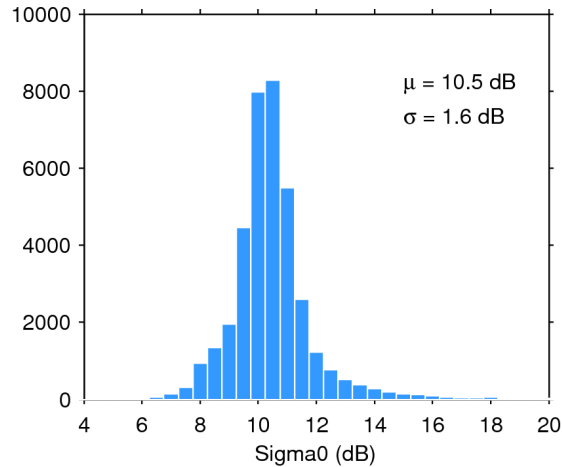
Figure 25. Histogram of flag-valid sigma0 over oceans and lakes for 05/06/2015. The mean ( \mu ) and standard deviation ( \sigma ) are also shown. Note that values outside [4 20] dB are excluded from the histogram for the sake of readability but not from the computation of \mu and \sigma .
