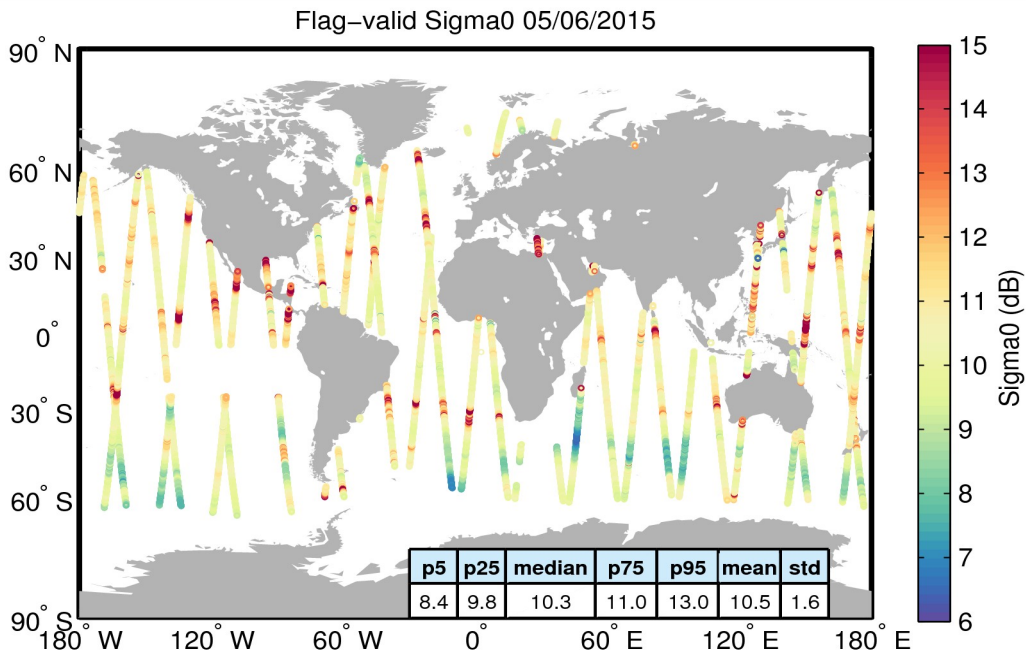
Figure 23. Geographical distribution of flag-valid sigma0 data over oceans and lakes for 05/06/2015. The statistical values shown in the table refer to the sigma0 in dB and are calculated over all measurements shown in the figure.
