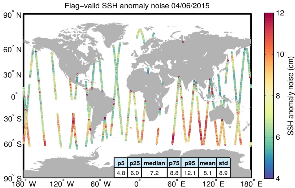
Figure 8. Geographical distribution of flag-valid 20-Hz SSH anomaly measurement noise over oceans and lakes for 04/06/2015. The statistical values shown in the table refer to the SSH anomaly noise and are calculated over all measurements shown in the figure.
