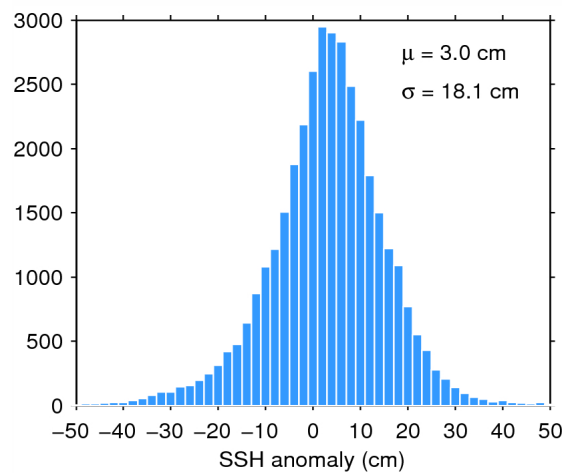
Figure 7. Histogram of flag-valid SSH anomaly over oceans and lakes for 04/06/2015. The mean ( \mu ) and standard deviation ( \sigma ) are also shown. Note that values outside [-50 50] cm are excluded from the histogram for the sake of readability but not from the computation of \mu and \sigma .
