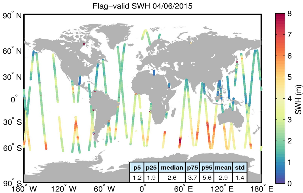
Figure 15. Geographical distribution of flag-valid SWH data over oceans and lakes for 04/06/2015. The statistical values shown in the table refer to the SWH in m and are calculated over all measurements shown in the figure.
