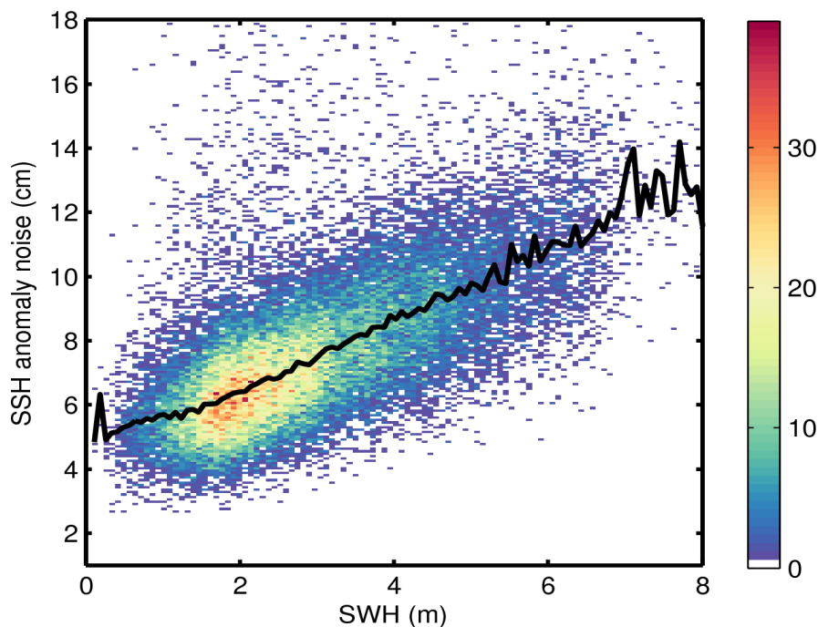
Figure 9. 2D histogram showing flag-valid SSH anomaly noise as a function of SWH for 04/06/2015. The black line denotes the median SSH anomaly as a function of SWH.
