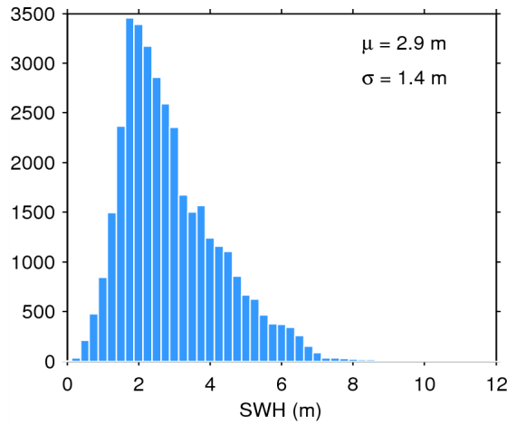
Figure 17. Histogram of flag-valid SWH over oceans and lakes for 04/06/2015. The mean ( \mu ) and standard deviation ( \sigma ) are also shown. Note that values larger than 12 m are excluded from the histogram for the sake of readability but not from the computation of \mu and \sigma .
