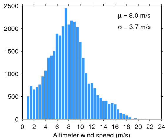
Figure 35. Histogram of science-valid wind over oceans and lakes for 04/06/2015. The mean ( \mu ) and standard deviation ( \sigma ) are also shown. Note that values larger than 24 m/s are excluded from the histogram for the sake of readability but not from the computation of \mu and \sigma .
