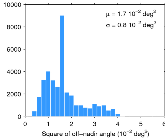
Figure 39. Histogram of flag-valid mispointing over oceans and lakes for 04/06/2015. The mean ( \mu ) and standard deviation ( \sigma ) are also shown. Note that values larger than 6 \cdot 10^{-2} \text{ deg}^2 are excluded from the histogram for the sake of readability but not from the computation of \mu and \sigma .
