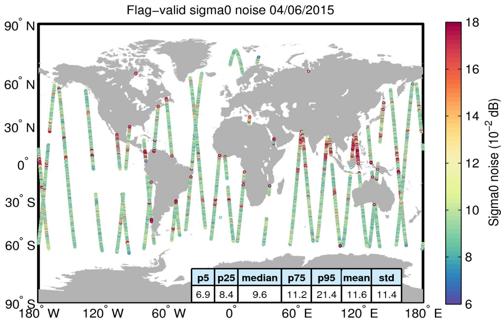
Figure 26. Geographical distribution of flag-valid 20-Hz sigma0 measurement noise over oceans and lakes for 04/06/2015. The statistical values shown in the table refer to the sigma0 noise and are calculated over all measurements shown in the figure.
