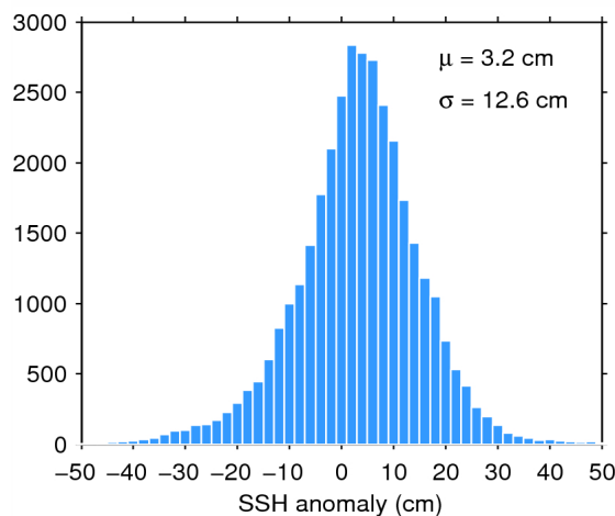
Figure 11. Histogram of science-valid SSH anomaly over oceans and lakes for 04/06/2015. The mean ( \mu ) and standard deviation ( \sigma ) are also shown. Note that values outside [-50 50] cm are excluded from the histogram for the sake of readability but not from the computation of \mu and \sigma .
