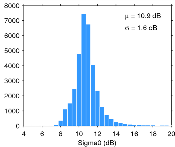
Figure 28. Histogram of science-valid sigma0 over oceans and lakes for 04/06/2015. The mean ( \mu ) and standard deviation ( \sigma ) are also shown. Note that values outside [4 20] dB are excluded from the histogram for the sake of readability but not from the computation of \mu and \sigma .
