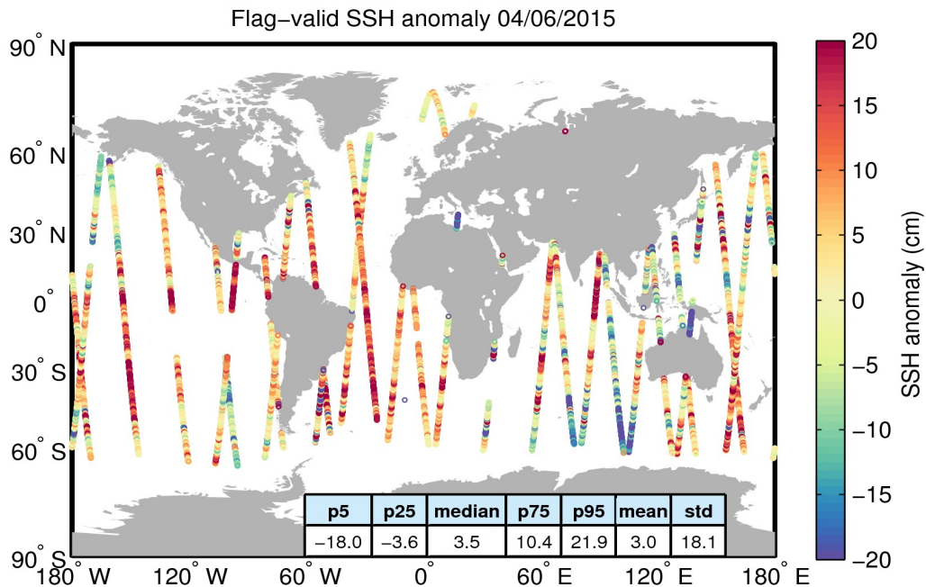
Figure 5. Geographical distribution of flag-valid 1-Hz SSH anomaly data over oceans and lakes for 04/06/2015. The statistical values shown in the table refer to the SSH anomaly in cm and are calculated over all measurements shown in the figure.
