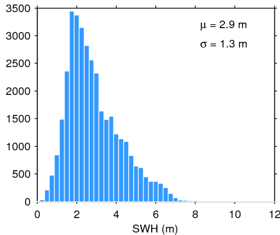
Figure 20. Histogram of science-valid SWH over oceans and lakes for 04/06/2015. The mean ( \mu ) and standard deviation ( \sigma ) are also shown. Note that values larger than 12 m are excluded from the histogram for the sake of readability but not from the computation of \mu and \sigma .
