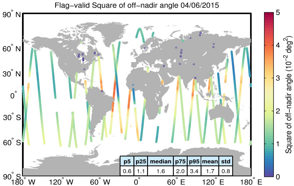
Figure 37. Geographical distribution of flag-valid mispointing data over oceans and lakes for 04/06/2015. The statistical values shown in the table refer to the mispointing in 10^{-2} \text{deg}^2 and are calculated over all measurements shown in the figure.
