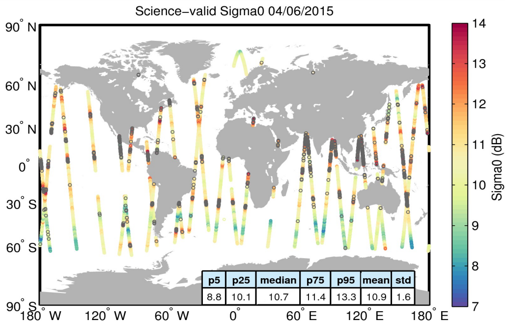
Figure 27. Geographical distribution of science-valid sigma0 data over oceans and lakes for 04/06/2015. The statistical values shown in the table refer to the sigma0 in dB and are calculated over all measurements shown in the figure. Gray circles denote records that have been rejected based on the editing criteria described in Table 4.
