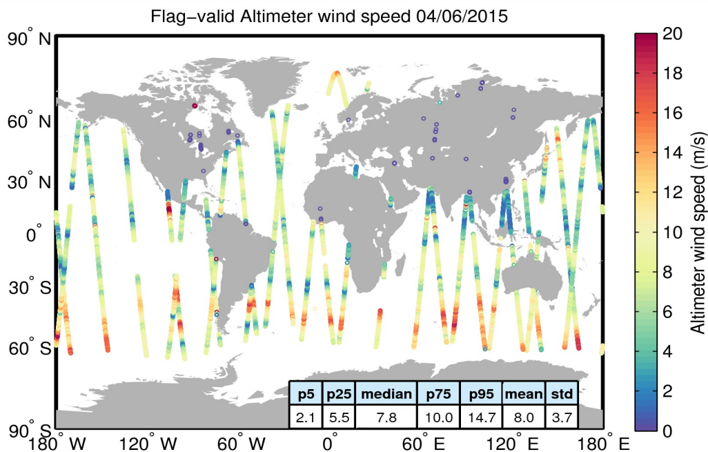
Figure 31. Geographical distribution of flag-valid wind data over oceans and lakes for 04/06/2015. The statistical values shown in the table refer to the wind in m/s and are calculated over all measurements shown in the figure.
