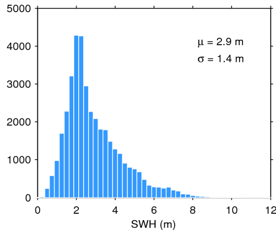
Figure 20. Histogram of science-valid SWH over oceans and lakes for 03/06/2015. The mean ( \mu ) and standard deviation ( \sigma ) are also shown. Note that values larger than 12 m are excluded from the histogram for the sake of readability but not from the computation of \mu and \sigma .
