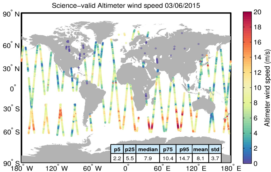
Figure 34. Geographical distribution of science-valid wind data over oceans and lakes for 03/06/2015. The statistical values shown in the table refer to the wind in m/s and are calculated over all measurements shown in the figure. Gray circles denote records that have been rejected based on the editing criteria described in Table 5.
