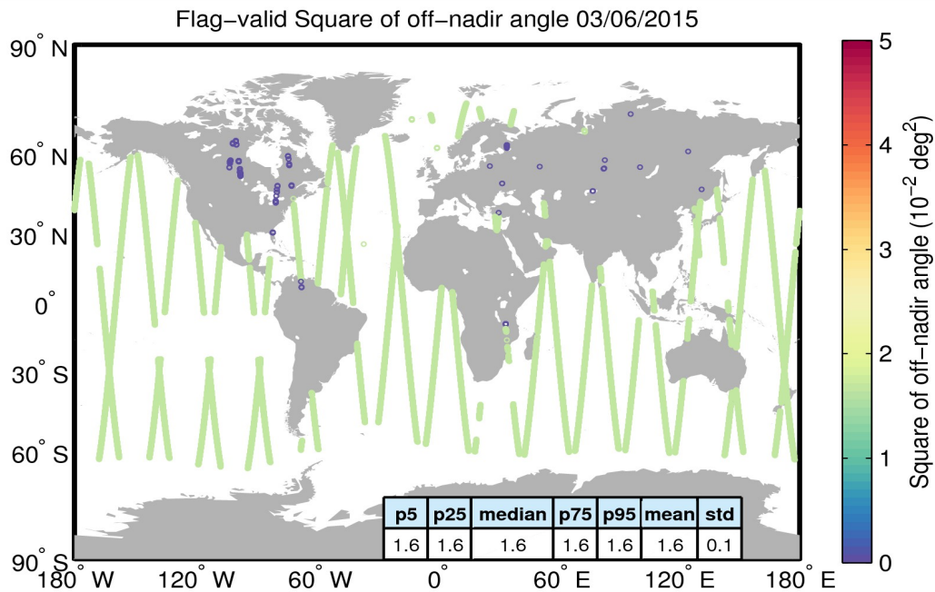
Figure 37. Geographical distribution of flag-valid mispointing data over oceans and lakes for 03/06/2015. The statistical values shown in the table refer to the mispointing in 10^{-2} \text{ deg}^2 and are calculated over all measurements shown in the figure.
