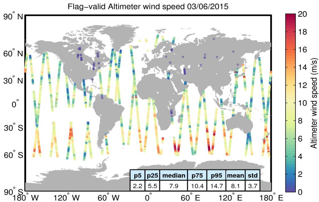
Figure 31. Geographical distribution of flag-valid wind data over oceans and lakes for 03/06/2015. The statistical values shown in the table refer to the wind in m/s and are calculated over all measurements shown in the figure.
