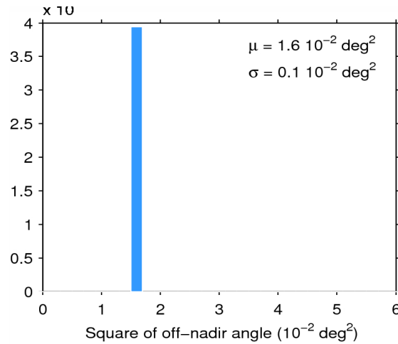
Figure 39. Histogram of flag-valid mispointing over oceans and lakes for 03/06/2015. The mean ( \mu ) and standard deviation ( \sigma ) are also shown. Note that values larger than 6 \cdot 10^{-2} \text{ deg}^2 are excluded from the histogram for the sake of readability but not from the computation of \mu and \sigma .
