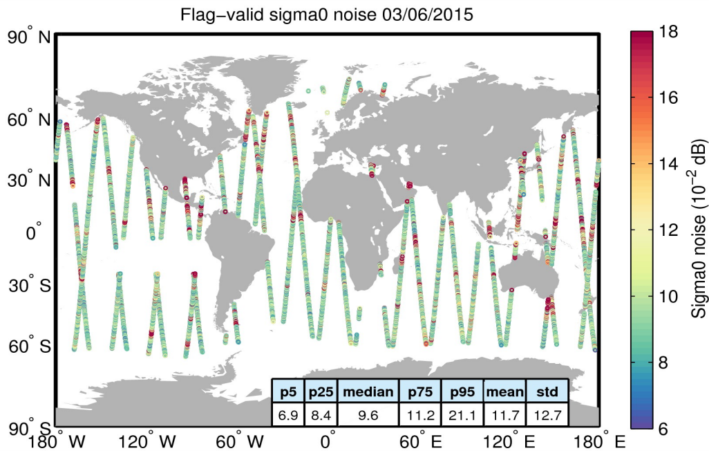
Figure 26. Geographical distribution of flag-valid 20-Hz sigma0 measurement noise over oceans and lakes for 03/06/2015. The statistical values shown in the table refer to the sigma0 noise and are calculated over all measurements shown in the figure.
