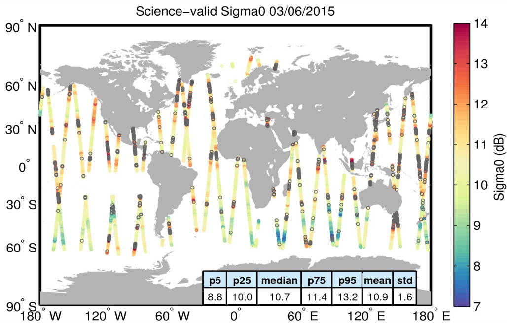
Figure 27. Geographical distribution of science-valid sigma0 data over oceans and lakes for 03/06/2015. The statistical values shown in the table refer to the sigma0 in dB and are calculated over all measurements shown in the figure. Gray circles denote records that have been rejected based on the editing criteria described in Table 4.
