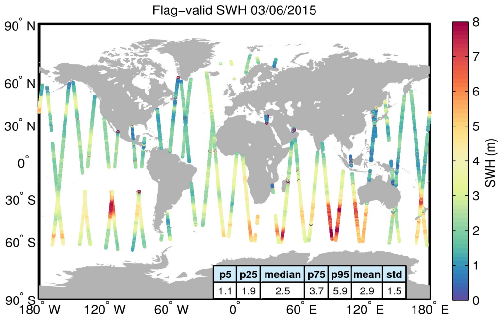
Figure 15. Geographical distribution of flag-valid SWH data over oceans and lakes for 03/06/2015. The statistical values shown in the figure refer to the SWH in m and are calculated over all measurements shown in the figure.
