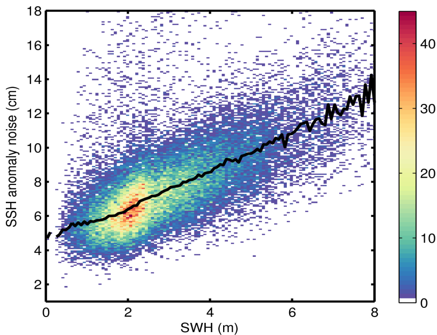
Figure 9. 2D histogram showing flag-valid SSH anomaly noise as a function of SWH for 03/06/2015. The black line denotes the median SSH anomaly as a function of SWH.
