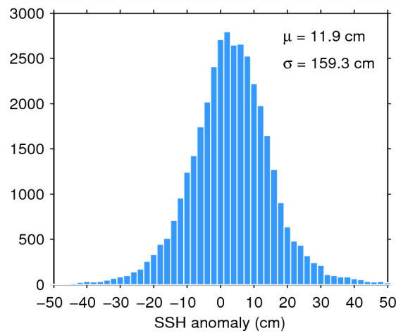
Figure 7. Histogram of flag-valid SSH anomaly over oceans and lakes for 03/06/2015. The mean ( \mu ) and standard deviation ( \sigma ) are also shown. Note that values outside [-50 50] cm are excluded from the histogram for the sake of readability but not from the computation of \mu and \sigma .
