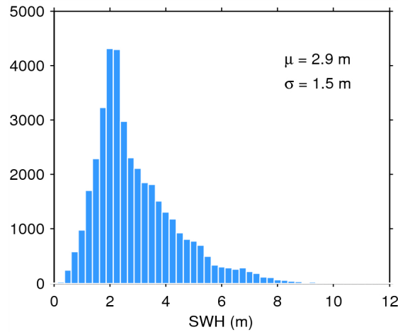
Figure 17. Histogram of flag-valid SWH over oceans and lakes for 03/06/2015. The mean ( \mu ) and standard deviation ( \sigma ) are also shown. Note that values larger than 12 m are excluded from the histogram for the sake of readability but not from the computation of \mu and \sigma .
