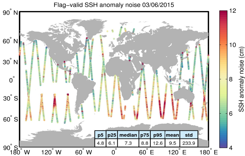
Figure 8. Geographical distribution of flag-valid 20-Hz SSH anomaly measurement noise over oceans and lakes for 03/06/2015. The statistical values shown in the table refer to the SSH anomaly noise and are calculated over all measurements shown in the figure.
