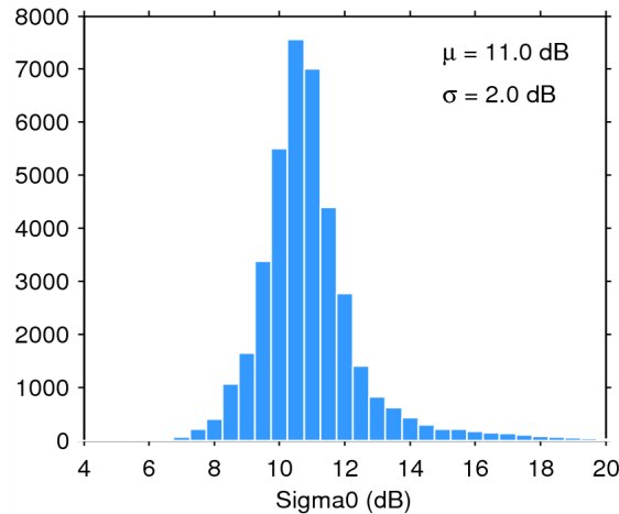
Figure 25. Histogram of flag-valid sigma0 over oceans and lakes for 03/06/2015. The mean ( \mu ) and standard deviation ( \sigma ) are also shown. Note that values outside [4 20] dB are excluded from the histogram for the sake of readability but not from the computation of \mu and \sigma .
