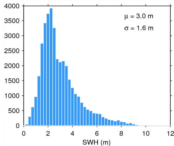
Figure 20. Histogram of science-valid SWH over oceans and lakes for 02/06/2015. The mean ( \mu ) and standard deviation ( \sigma ) are also shown. Note that values larger than 12 m are excluded from the histogram for the sake of readability but not from the computation of \mu and \sigma .
