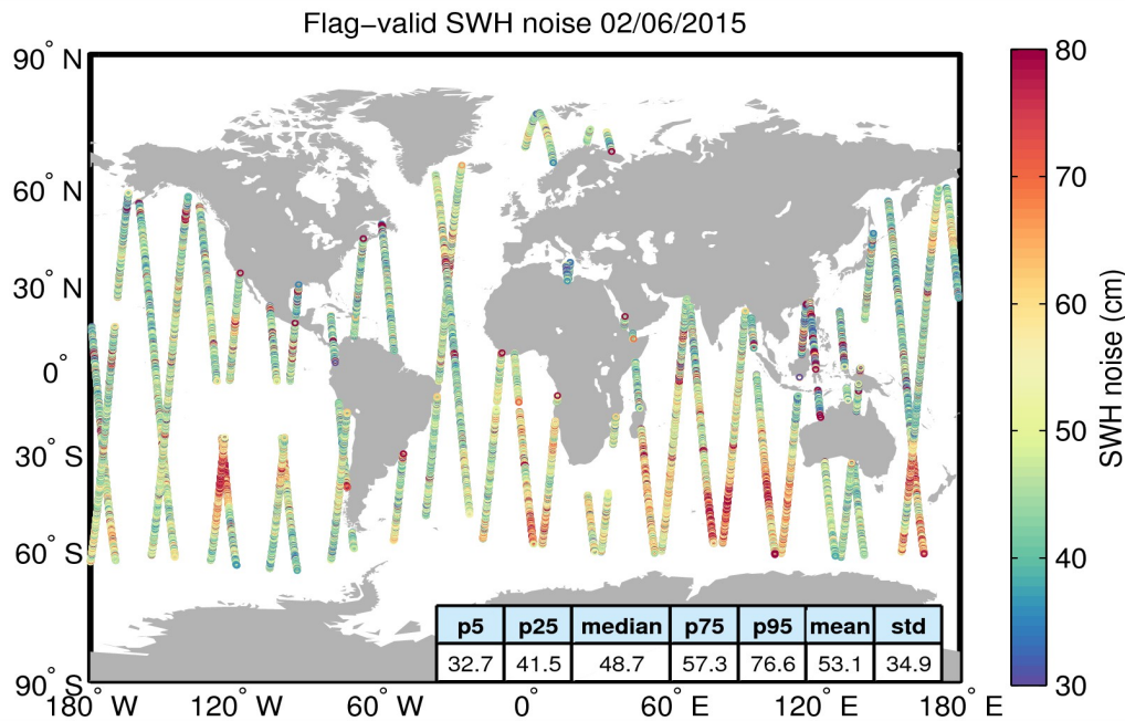
Figure 18. Geographical distribution of flag-valid 20-Hz SWH measurement noise over oceans and lakes for 02/06/2015. The statistical values shown in the figure refer to the SWH noise and are calculated over all measurements shown in the figure.
