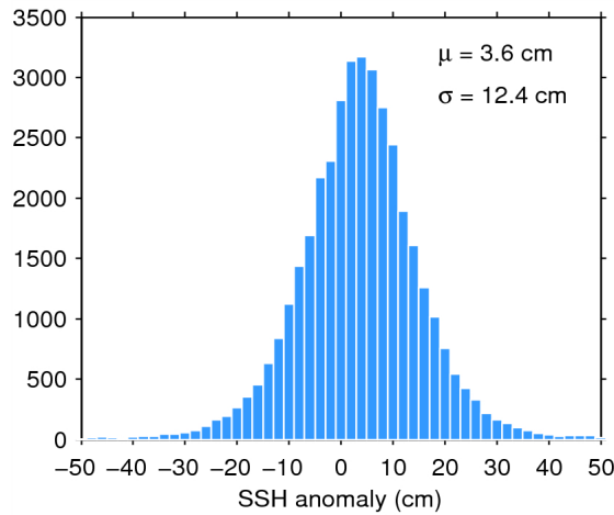
Figure 11. Histogram of science-valid SSH anomaly over oceans and lakes for 02/06/2015. The mean ( \mu ) and standard deviation ( \sigma ) are also shown. Note that values outside [-50 50] cm are excluded from the histogram for the sake of readability but not from the computation of \mu and \sigma .
