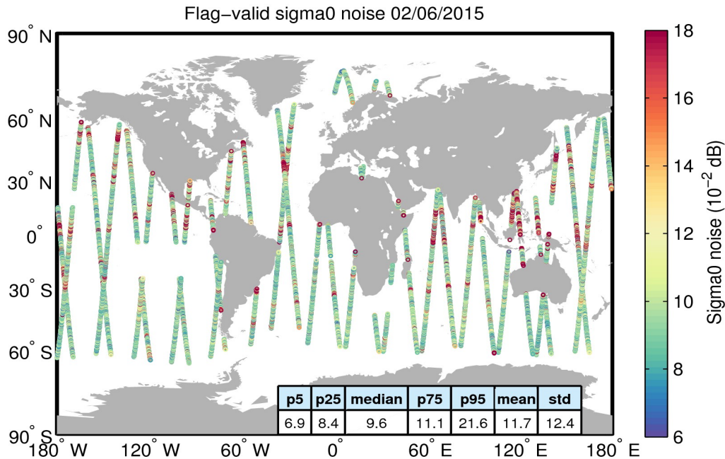
Figure 26. Geographical distribution of flag-valid 20-Hz sigma0 measurement noise over oceans and lakes for 02/06/2015. The statistical values shown in the table refer to the sigma0 noise and are calculated over all measurements shown in the figure.
