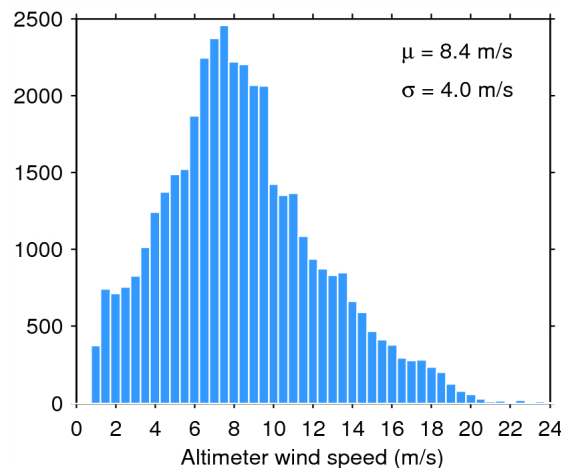
Figure 35. Histogram of science-valid wind over oceans and lakes for 02/06/2015. The mean ( \mu ) and standard deviation ( \sigma ) are also shown. Note that values larger than 24 m/s are excluded from the histogram for the sake of readability but not from the computation of \mu and \sigma .
