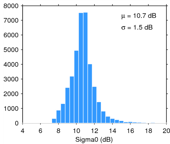
Figure 28. Histogram of science-valid sigma0 over oceans and lakes for 02/06/2015. The mean ( \mu ) and standard deviation ( \sigma ) are also shown. Note that values outside [4 20] dB are excluded from the histogram for the sake of readability but not from the computation of \mu and \sigma .
