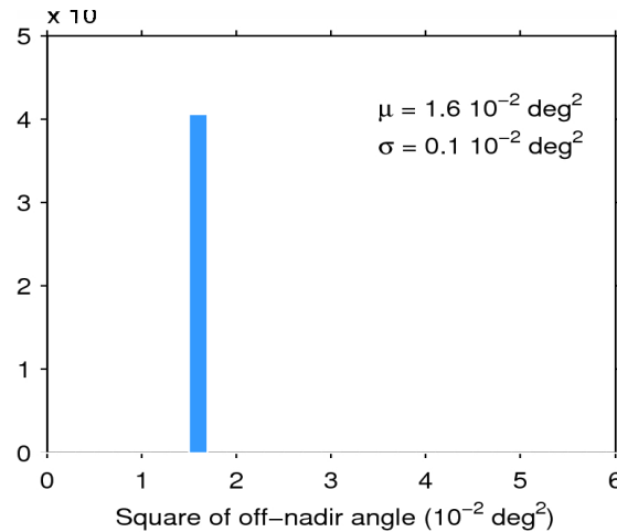
Figure 39. Histogram of flag-valid mispointing over oceans and lakes for 02/06/2015. The mean ( \mu ) and standard deviation ( \sigma ) are also shown. Note that values larger than 6 \cdot 10^{-2} \text{ deg}^2 are excluded from the histogram for the sake of readability but not from the computation of \mu and \sigma .
