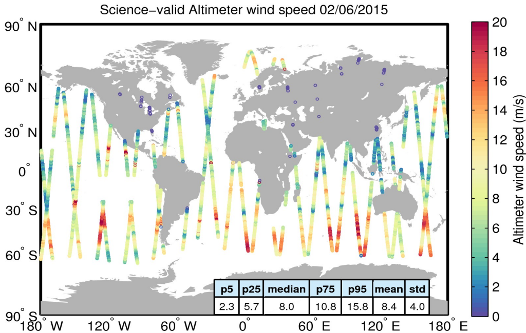
Figure 34. Geographical distribution of science-valid wind data over oceans and lakes for 02/06/2015. The statistical values shown in the table refer to the wind in m/s and are calculated over all measurements shown in the figure. Gray circles denote records that have been rejected based on the editing criteria described in Table 5.
