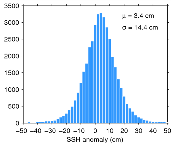
Figure 7. Histogram of flag-valid SSH anomaly over oceans and lakes for 02/06/2015. The mean ( \mu ) and standard deviation ( \sigma ) are also shown. Note that values outside [-50\ 50] cm are excluded from the histogram for the sake of readability but not from the computation of \mu and \sigma .
