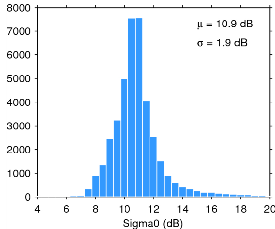
Figure 25. Histogram of flag-valid sigma0 over oceans and lakes for 02/06/2015. The mean ( \mu ) and standard deviation ( \sigma ) are also shown. Note that values outside [4 20] dB are excluded from the histogram for the sake of readability but not from the computation of \mu and \sigma .
