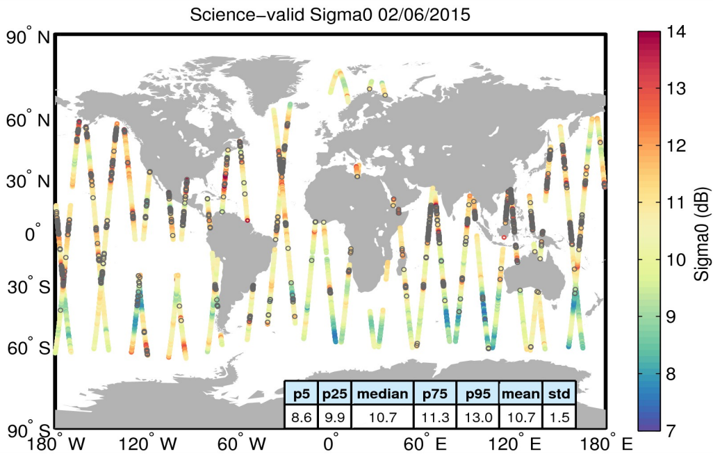
Figure 27. Geographical distribution of science-valid sigma0 data over oceans and lakes for 02/06/2015. The statistical values shown in the table refer to the sigma0 in dB and are calculated over all measurements shown in the figure. Gray circles denote records that have been rejected based on the editing criteria described in Table 4.
