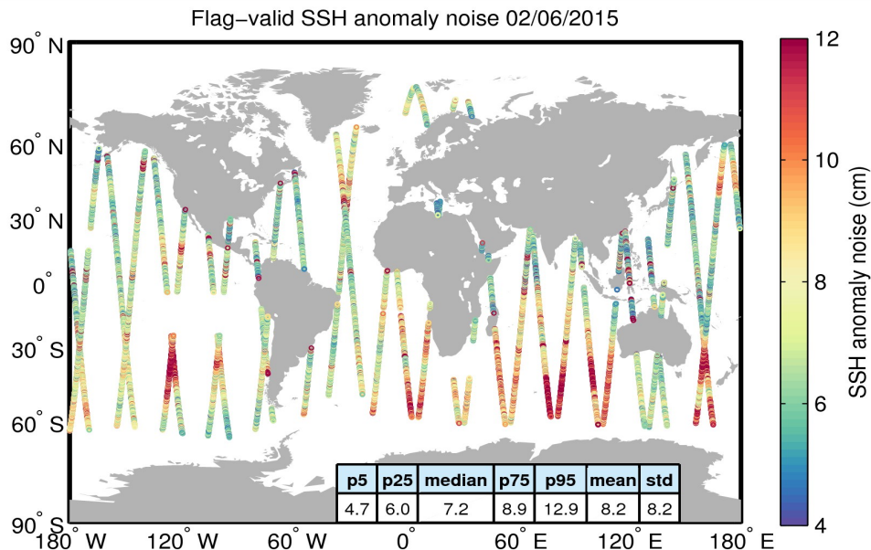
Figure 8. Geographical distribution of flag-valid 20-Hz SSH anomaly measurement noise over oceans and lakes for 02/06/2015. The statistical values shown in the table refer to the SSH anomaly noise and are calculated over all measurements shown in the figure.
