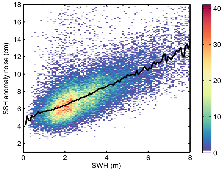
Figure 9. 2D histogram showing flag-valid SSH anomaly noise as a function of SWH for 02/06/2015. The black line denotes the median SSH anomaly as a function of SWH.
