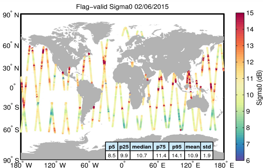
Figure 23. Geographical distribution of flag-valid sigma0 data over oceans and lakes for 02/06/2015. The statistical values shown in the table refer to the sigma0 in dB and are calculated over all measurements shown in the figure.
