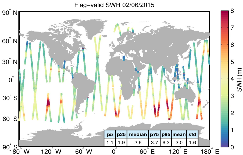
Figure 15. Geographical distribution of flag-valid SWH data over oceans and lakes for 02/06/2015. The statistical values shown in the table refer to the SWH in m and are calculated over all measurements shown in the figure.
