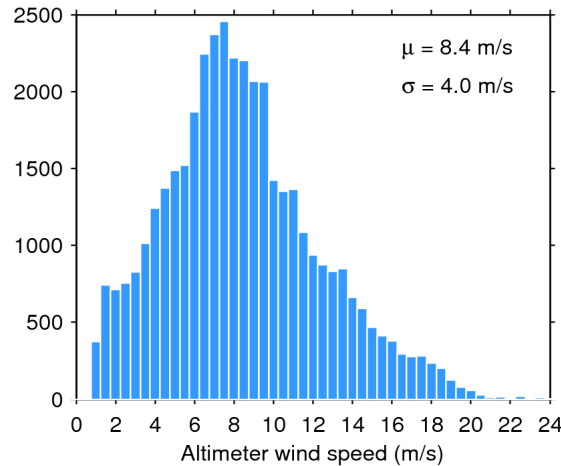
Figure 33. Histogram of flag-valid wind over oceans and lakes for 02/06/2015. The mean ( \mu ) and standard deviation ( \sigma ) are also shown. Note that values larger than 24 m/s are excluded from the histogram for the sake of readability but not from the computation of \mu and \sigma .
