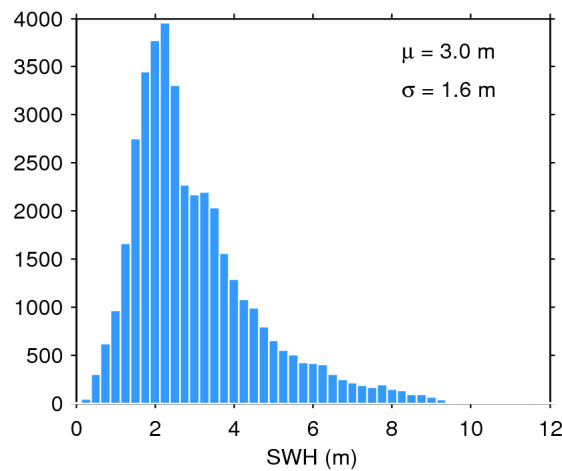
Figure 17. Histogram of flag-valid SWH over oceans and lakes for 02/06/2015. The mean ( \mu ) and standard deviation ( \sigma ) are also shown. Note that values larger than 12 m are excluded from the histogram for the sake of readability but not from the computation of \mu and \sigma .
