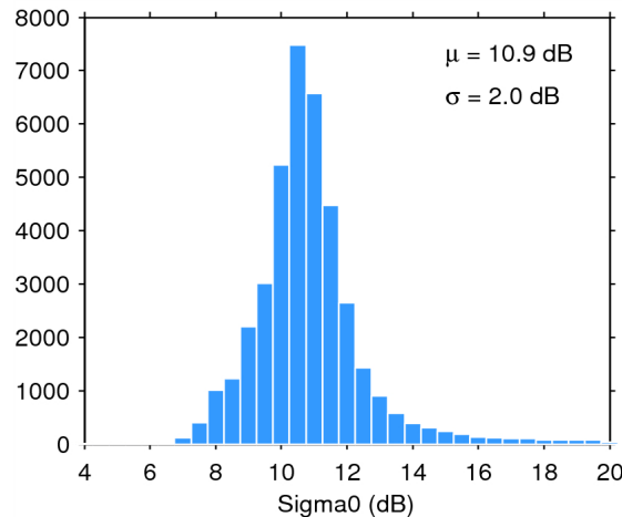
Figure 25. Histogram of flag-valid sigma0 over oceans and lakes for 01/06/2015. The mean ( \mu ) and standard deviation ( \sigma ) are also shown. Note that values outside [4 20] dB are excluded from the histogram for the sake of readability but not from the computation of \mu and \sigma .
