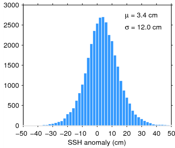
Figure 11. Histogram of science-valid SSH anomaly over oceans and lakes for 01/06/2015. The mean ( \mu ) and standard deviation ( \sigma ) are also shown. Note that values outside [-50 50] cm are excluded from the histogram for the sake of readability but not from the computation of \mu and \sigma .
