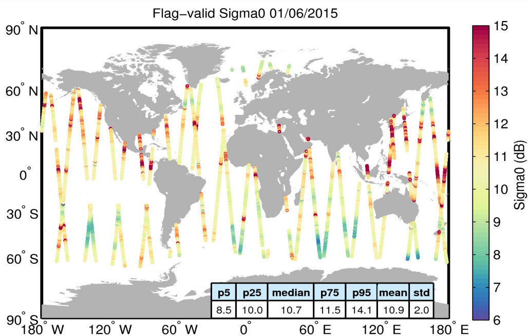
Figure 23. Geographical distribution of flag-valid sigma0 data over oceans and lakes for 01/06/2015. The statistical values shown in the table refer to the sigma0 in dB and are calculated over all measurements shown in the figure.
