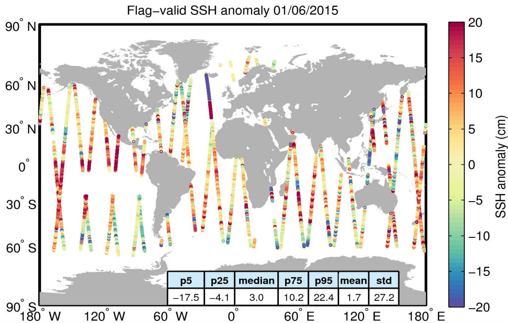
Figure 5. Geographical distribution of flag-valid 1-Hz SSH anomaly data over oceans and lakes for 01/06/2015. The statistical values shown in the table refer to the SSH anomaly in cm and are calculated over all measurements shown in the figure.
