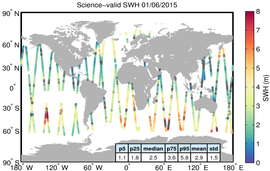
Figure 19. Geographical distribution of science-valid SWH data over oceans and lakes for 01/06/2015. The statistical values shown in the table refer to the SWH in m and are calculated over all measurements shown in the figure. Gray circles denote records that have been rejected based on the editing criteria described in Table 3.
