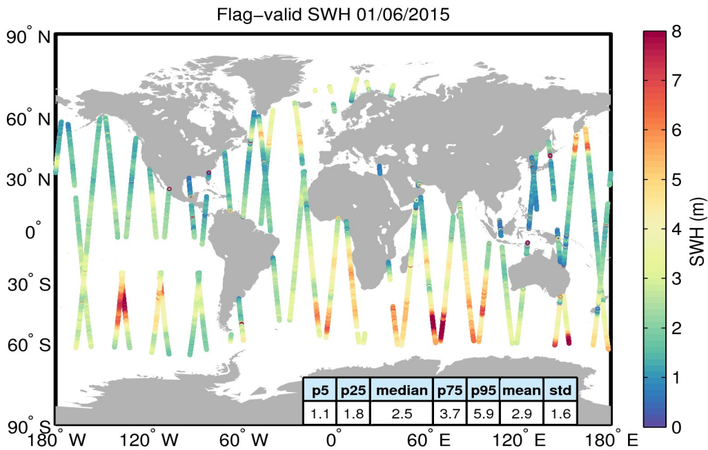
Figure 15. Geographical distribution of flag-valid SWH data over oceans and lakes for 01/06/2015. The statistical values shown in the table refer to the SWH in m and are calculated over all measurements shown in the figure.
