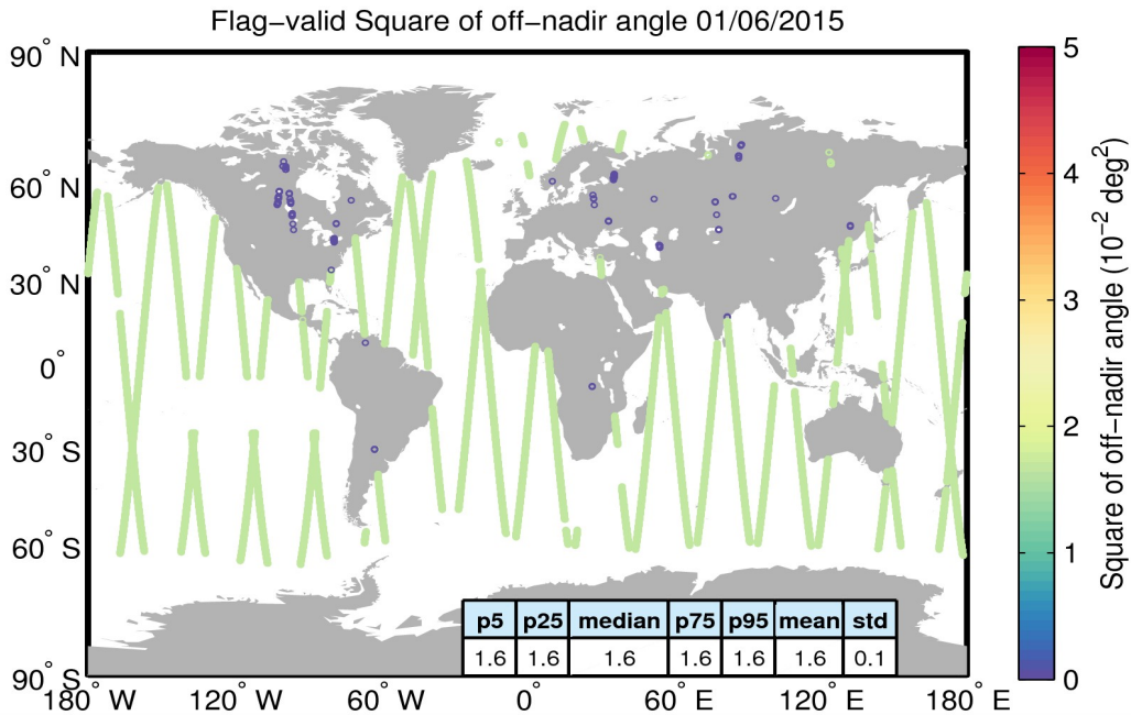
Figure 37. Geographical distribution of flag-valid mispointing data over oceans and lakes for 01/06/2015. The statistical values shown in the table refer to the mispointing in 10^{-2} \text{ deg}^2 and are calculated over all measurements shown in the figure.
