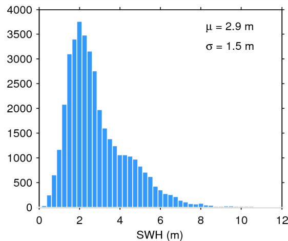
Figure 20. Histogram of science-valid SWH over oceans and lakes for 01/06/2015. The mean ( \mu ) and standard deviation ( \sigma ) are also shown. Note that values larger than 12 m are excluded from the histogram for the sake of readability but not from the computation of \mu and \sigma .
