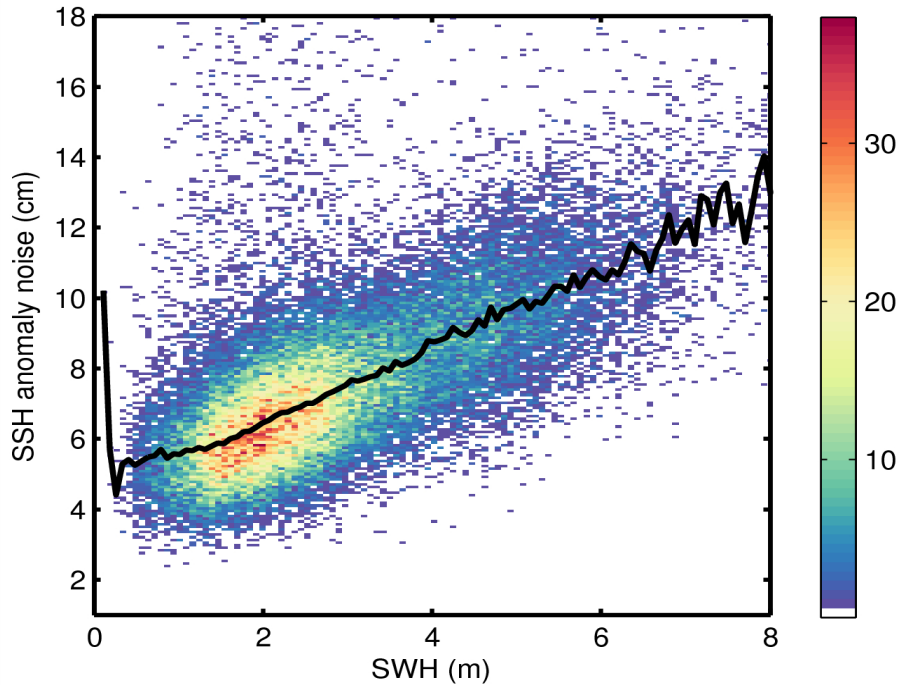
Figure 9. 2D histogram showing flag-valid SSH anomaly noise as a function of SWH for 01/06/2015. The black line denotes the median SSH anomaly as a function of SWH.
