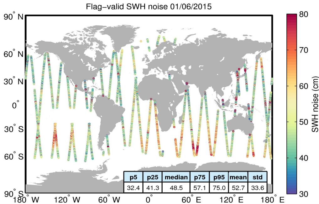
Figure 18. Geographical distribution of flag-valid 20-Hz SWH measurement noise over oceans and lakes for 01/06/2015. The statistical values shown in the figure refer to the SWH noise and are calculated over all measurements shown in the figure.
