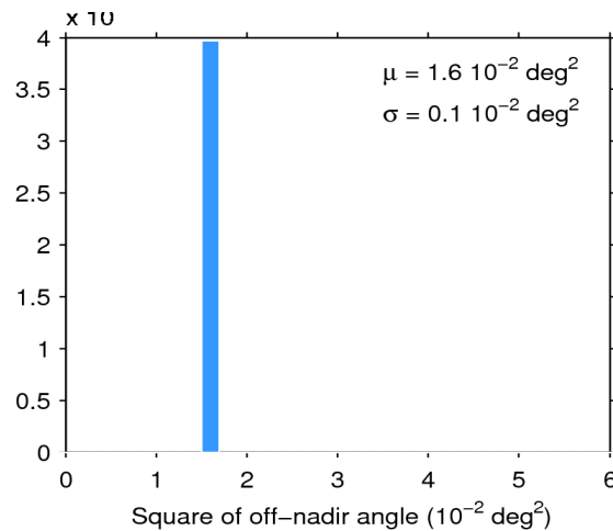
Figure 39. Histogram of flag-valid mispointing over oceans and lakes for 01/06/2015. The mean ( \mu ) and standard deviation ( \sigma ) are also shown. Note that values larger than 6 \cdot 10^{-2} \text{ deg}^2 are excluded from the histogram for the sake of readability but not from the computation of \mu and \sigma .
