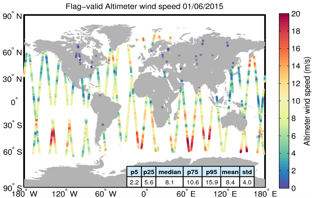
Figure 31. Geographical distribution of flag-valid wind data over oceans and lakes for 01/06/2015. The statistical values shown in the table refer to the wind in m/s and are calculated over all measurements shown in the figure.
