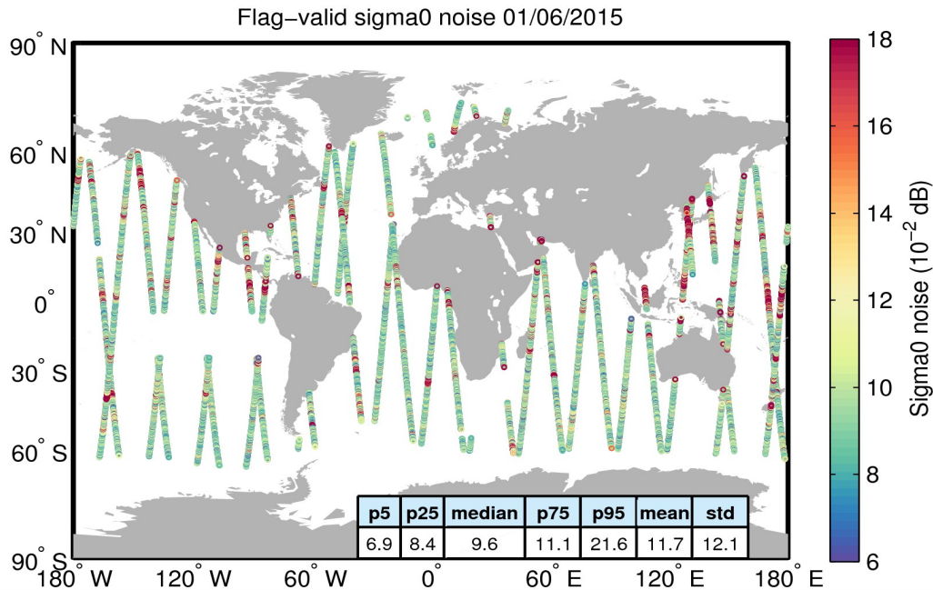
Figure 26. Geographical distribution of flag-valid 20-Hz sigma0 measurement noise over oceans and lakes for 01/06/2015. The statistical values shown in the table refer to the sigma0 noise and are calculated over all measurements shown in the figure.
