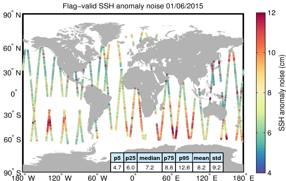
Figure 8. Geographical distribution of flag-valid 20-Hz SSH anomaly measurement noise over oceans and lakes for 01/06/2015. The statistical values shown in the table refer to the SSH anomaly noise and are calculated over all measurements shown in the figure.
