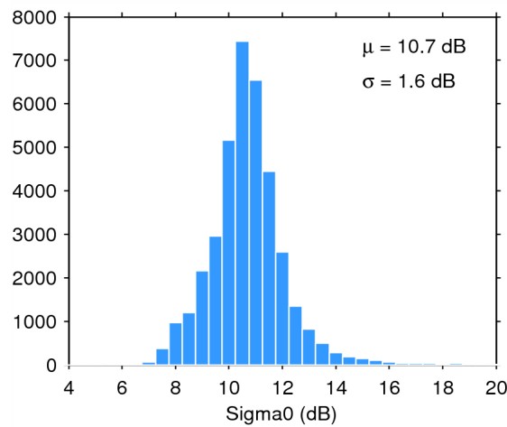
Figure 28. Histogram of science-valid sigma0 over oceans and lakes for 01/06/2015. The mean ( \mu ) and standard deviation ( \sigma ) are also shown. Note that values outside [4 20] dB are excluded from the histogram for the sake of readability but not from the computation of \mu and \sigma .
